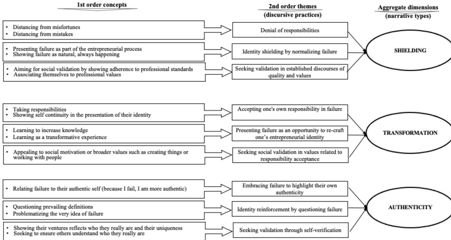
Figure 1: Data Structure
