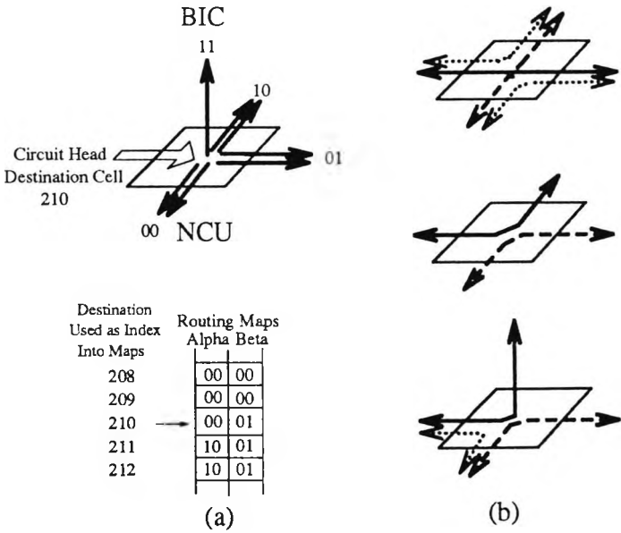
Figure 5.19: Circuit-Switched Routing
