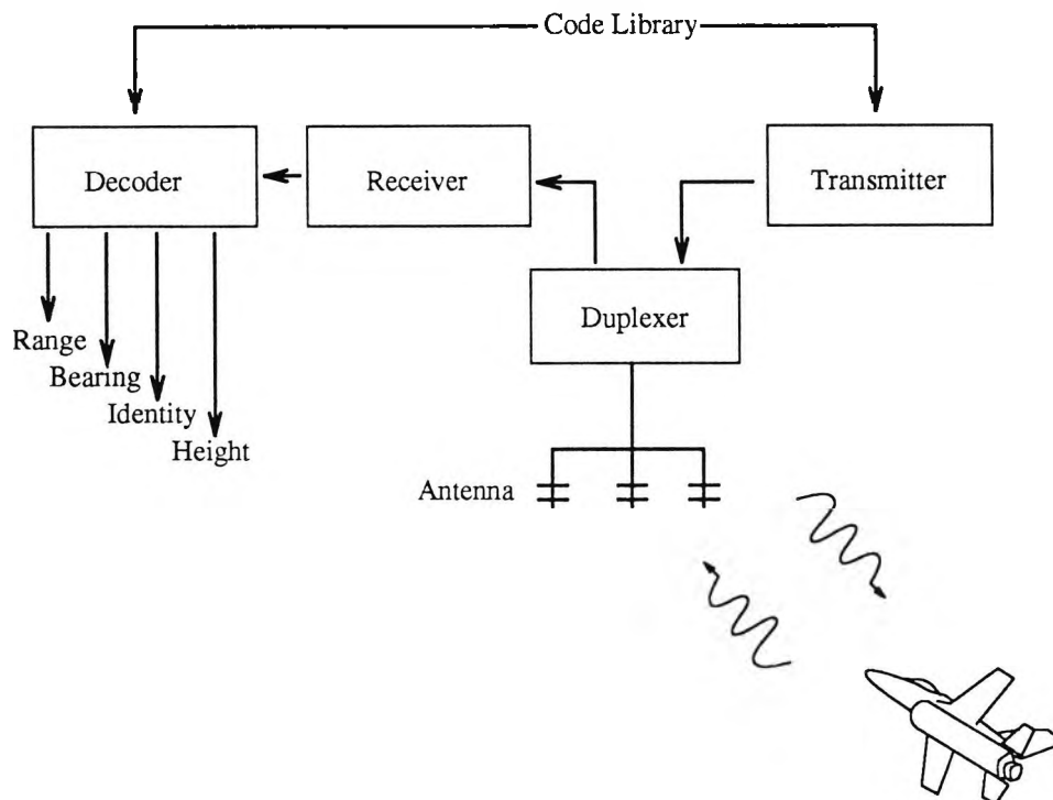
Figure B.5: The Identification, Friend or Foe (IFF) System
