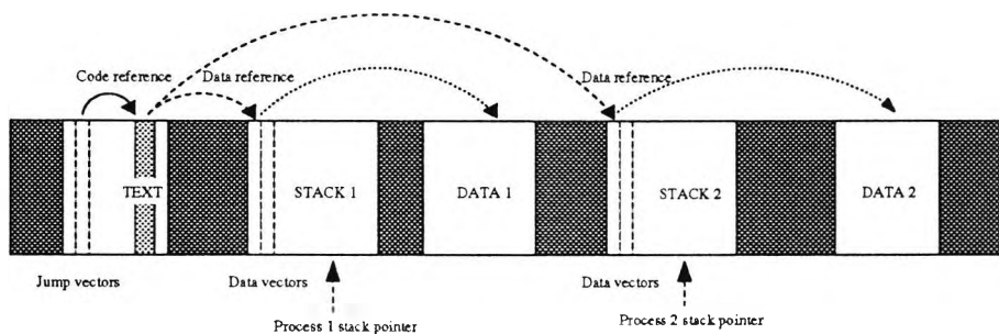
Figure 2.4: Using Indirection to Allow Code Sharing
