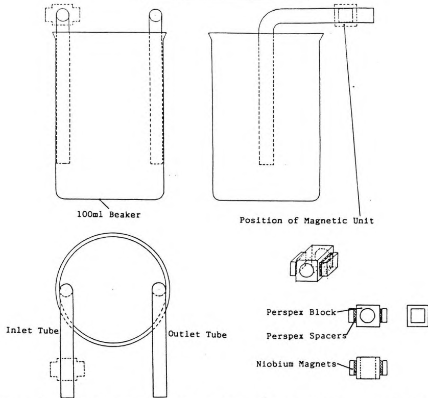
Vessels and Magnetic Units Used for Multiple Test Rig.
