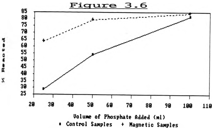
Percentage Calcium Reacted Results for Experiment 3.
