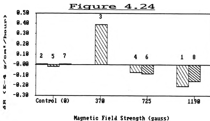
Graph of Corrosion Rate Results for Experiment 27.
