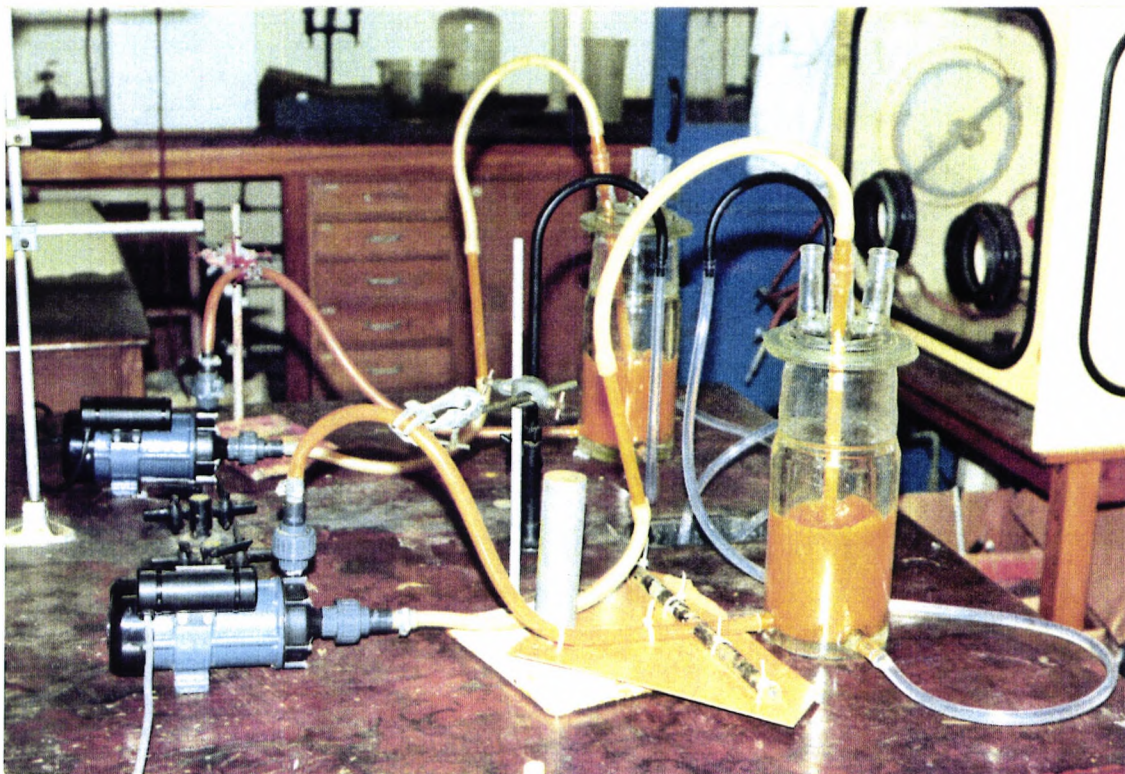
Corrosion Testing Apparatus (Single Test Rigs).
