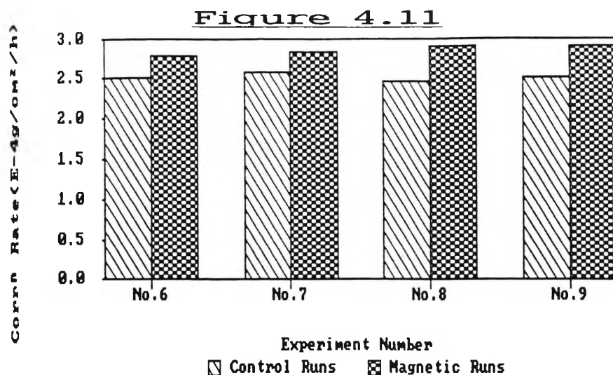
Comparison of Corrosion Rates Determined for Experiments 6 to 9.
