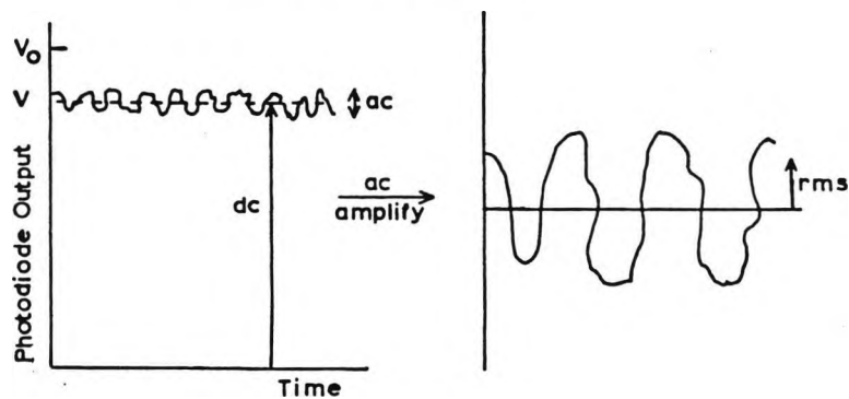
a.c. and d.c. Components of Photodiode Output.
