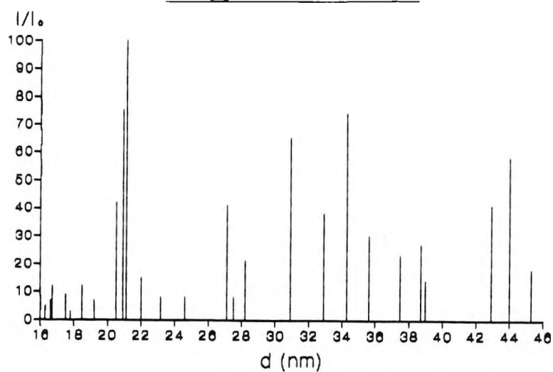
X-ray Diffractogram for O-O* Run Sample.
