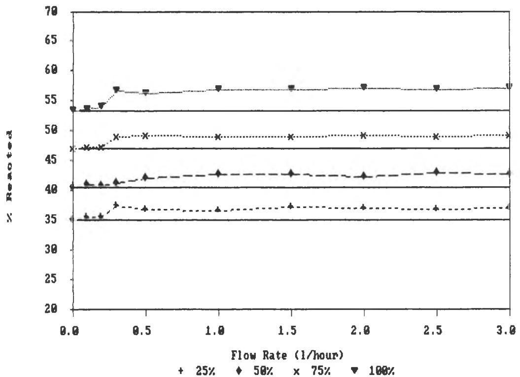
Percentage Magnesium Reacted Results for Experiment 8. (Single Pass - Narrow Tube)
