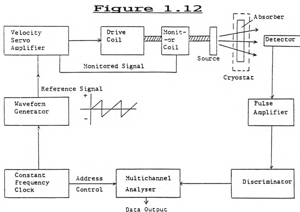
Schematic Diagram of a Mössbauer Spectrometer.
