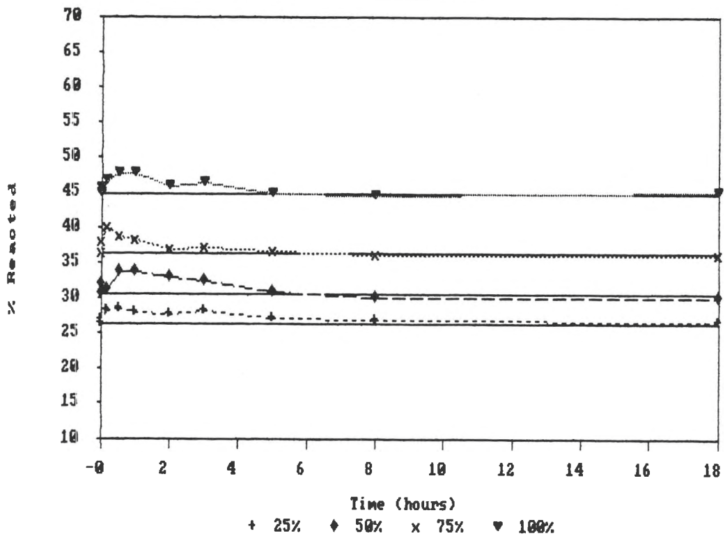
Percentage Magnesium Reacted Results for Experiment 5.
