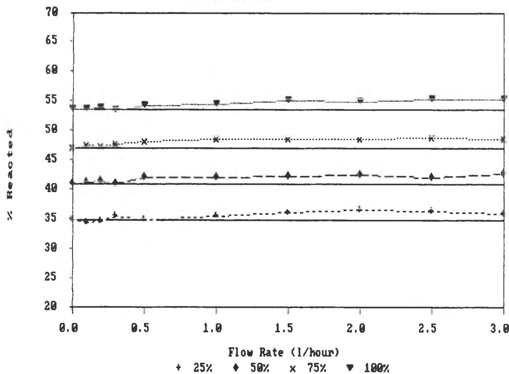
Percentage Magnesium Reacted Results for Experiment 7. (Recirculating - Wide Tube)
