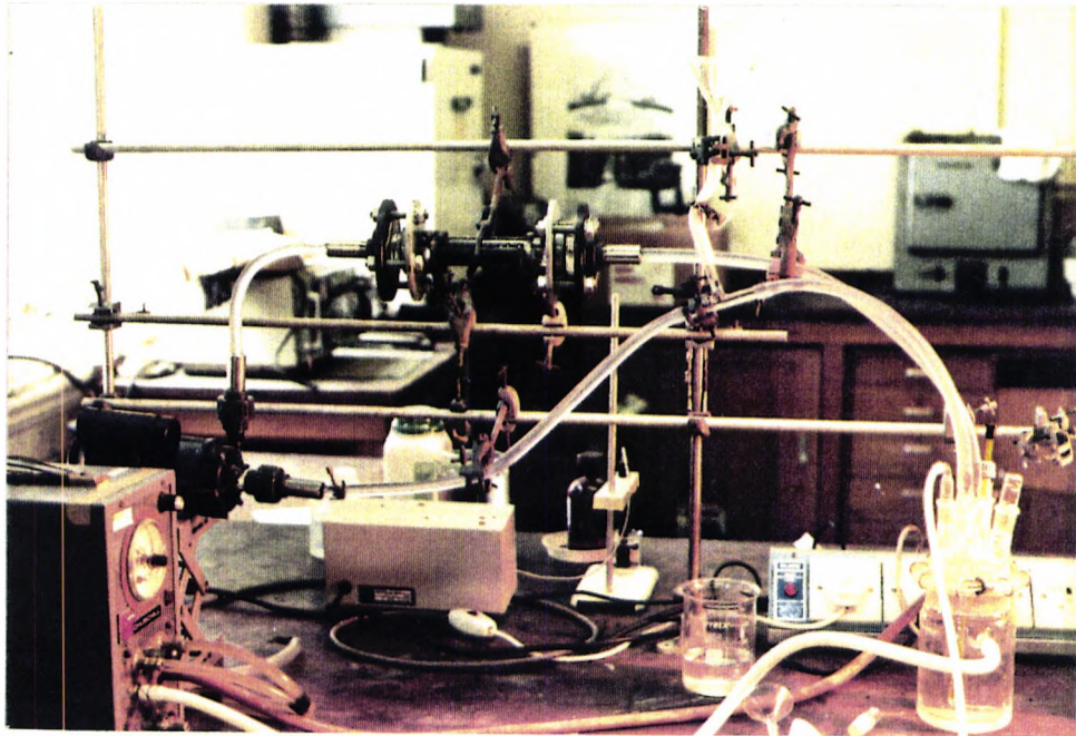
Photograph of Jacketed Vessel Test Rig.
