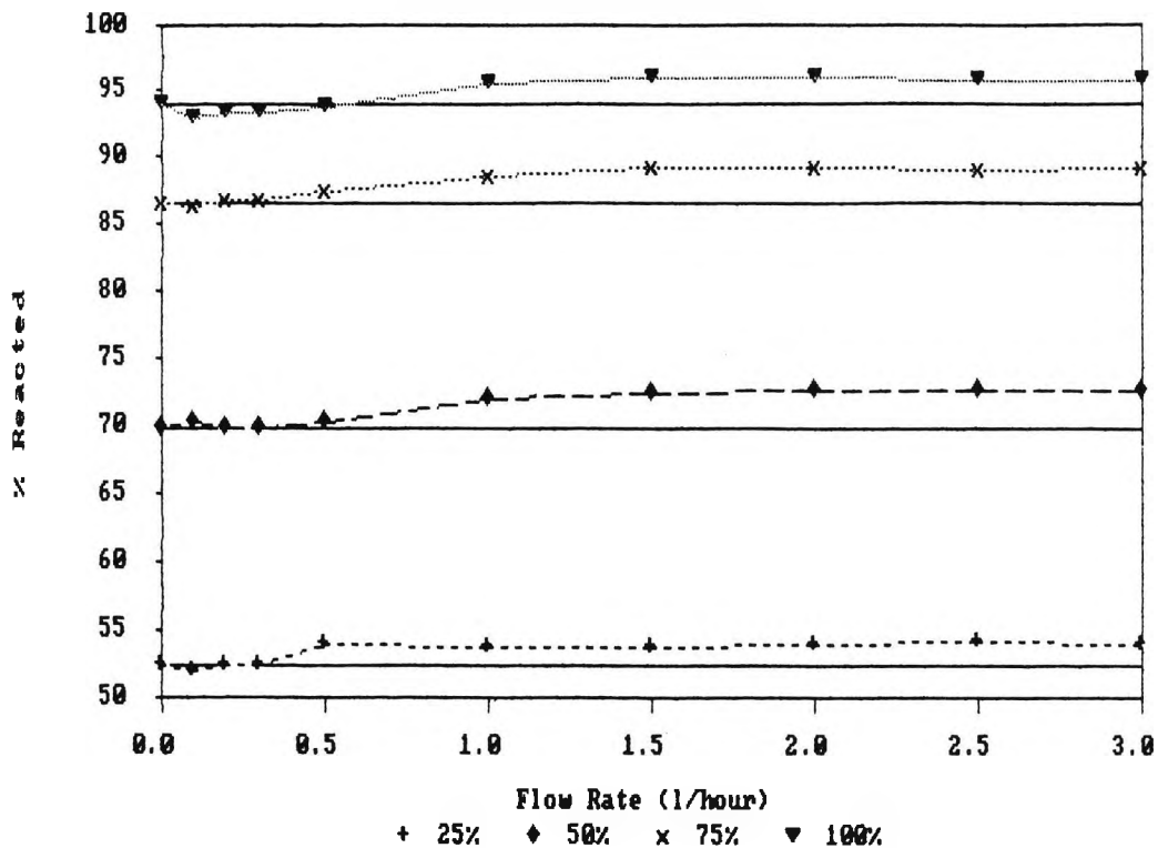
Percentage Calcium Reacted Results for Experiment 9. (Single Pass - Wide Tube)
