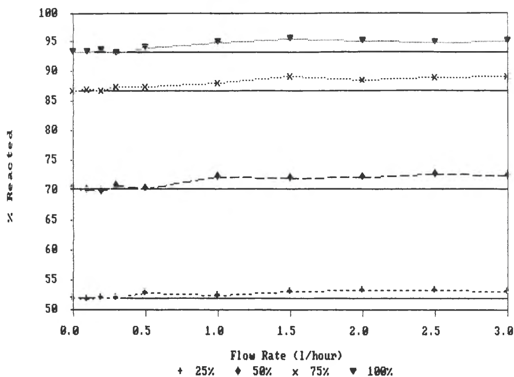
Percentage Calcium Reacted Results for Experiment 7. (Recirculating - Wide Tube)
