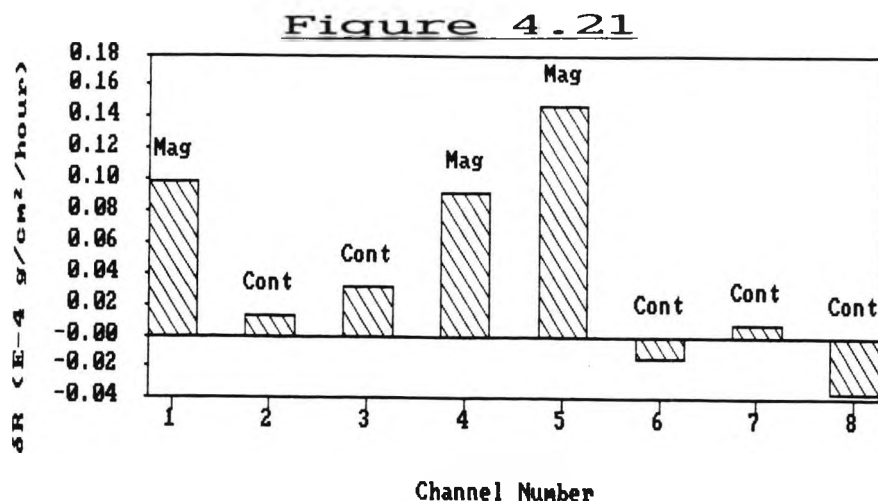
Graph of Corrosion Rate Results for Experiment 24.
