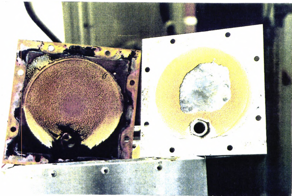
Boiler Top Plates After One Month.
