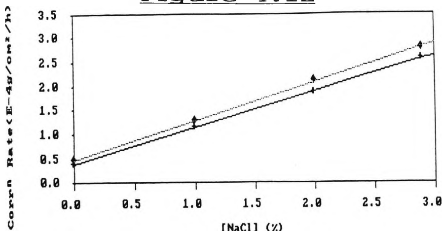
+ Control Runs ♦ Magnetic Runs Corrosion Rates at Different [NaCl] Concentrations (5.0mm Diameter Balls).
