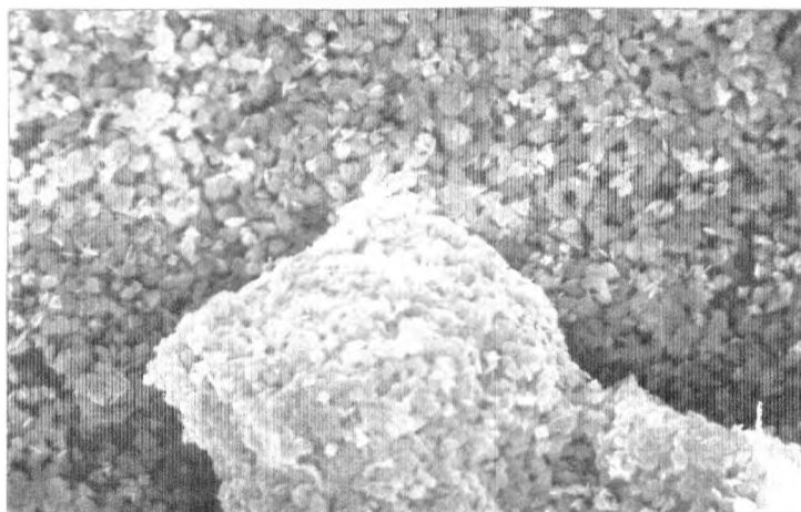
Electron Micrograph (x300) of **M Run Sample.
