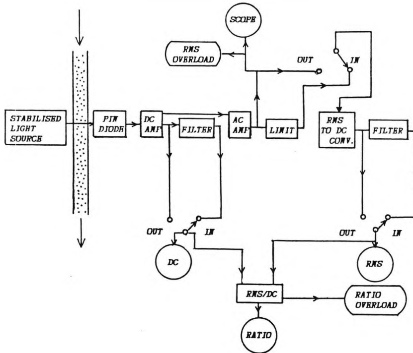
Schematic Diagram of PDA2000 Photometric Dispersion Analyzer.
