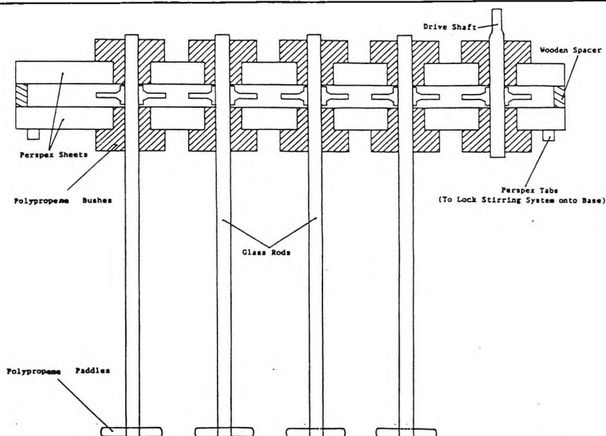
Section A - A of Stirring System Used with Multiple Test Rig.
