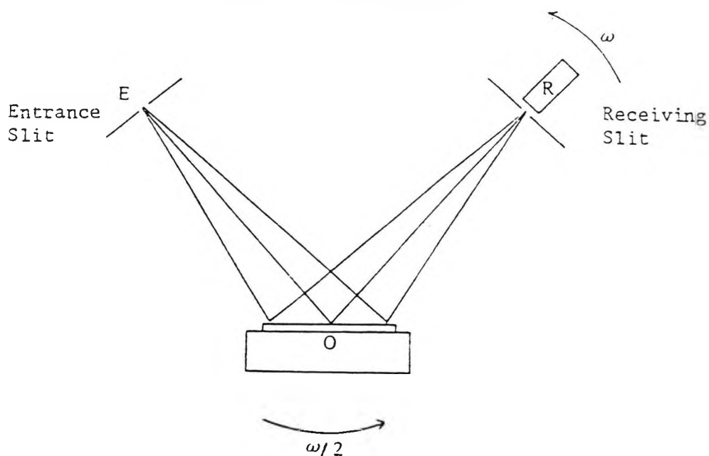
Schematic Diagram of a X-Ray Diffractometer.
