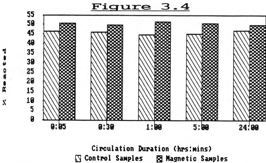
Percentage Calcium Reacted Results for Experiment 2.
