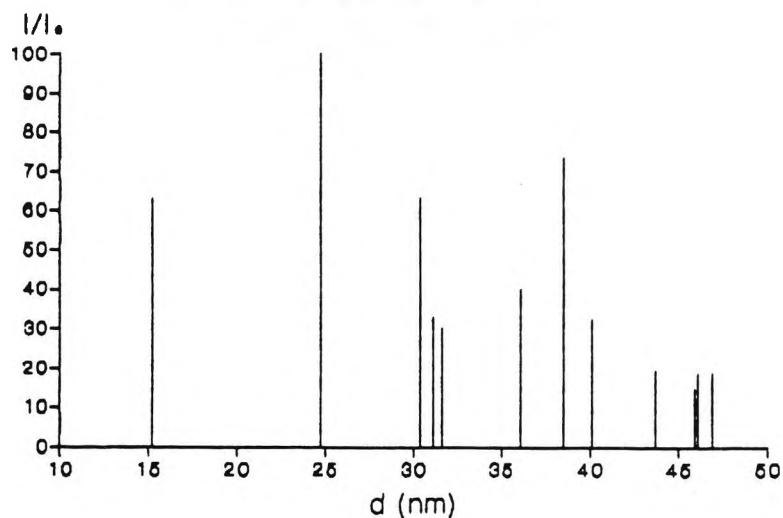
X-ray Diffractogram - Control Run Sample.
