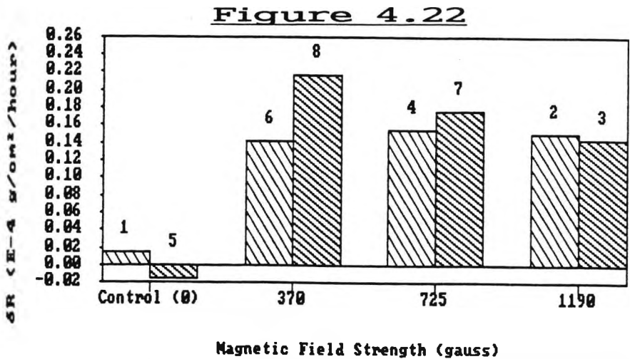
Graph of Corrosion Rate Results for Experiment 25.
