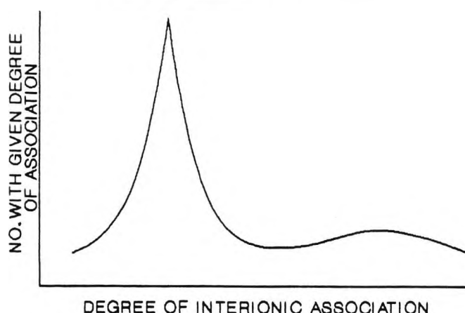
Distribution of Degree of Association After Recirculating Tests.
