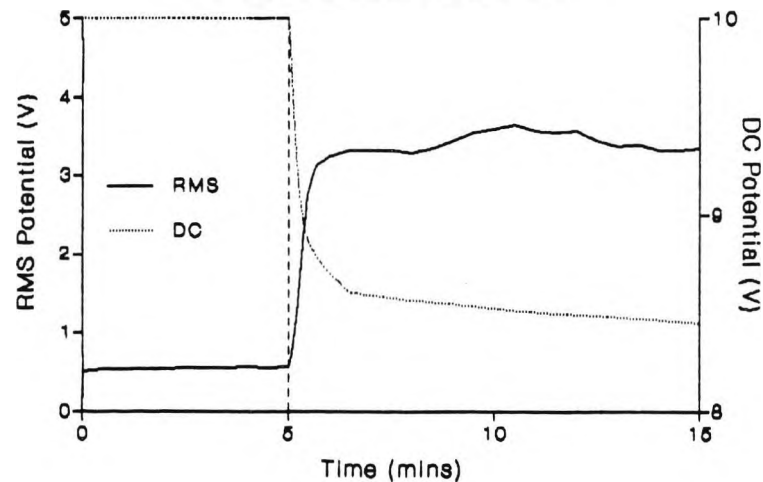
PDA2000 Graph - Control Run.
