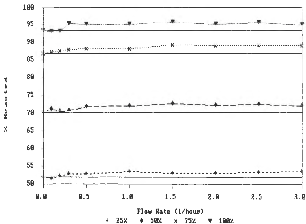
Percentage Calcium Reacted Results for Experiment 6. (Recirculating - Narrow Tube)
