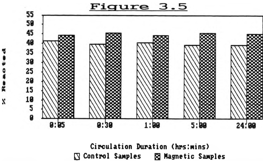
Percentage Magnesium Reacted Results for Experiment 2.
