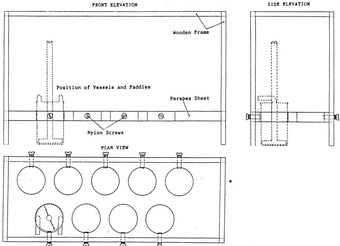
Multiple Test Rig Base and Vessel Holder.
