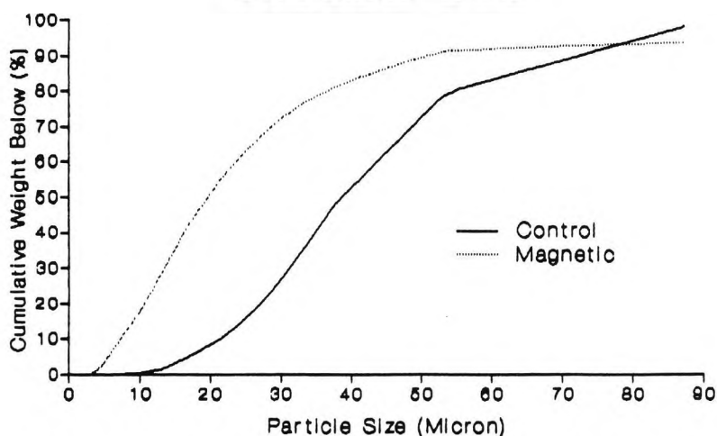
Particle Size Distribution - Cumulative Weight Below.
