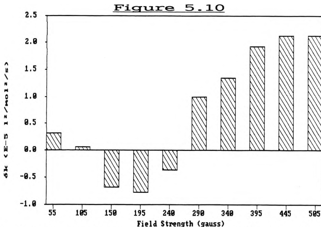
Graph of \Delta k against Magnetic Field Strength - Recirculating Tests.
