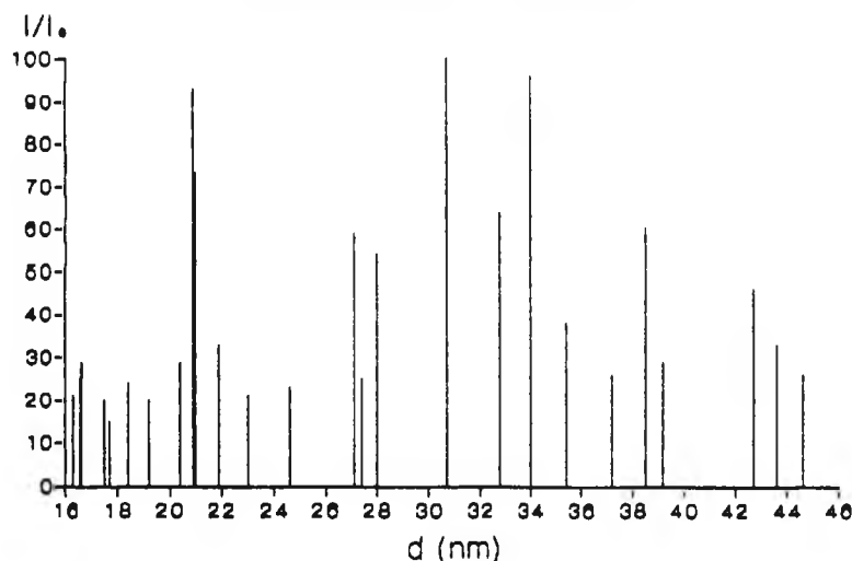
X-ray Diffractogram for X-ray Grade Barium Sulphate.
