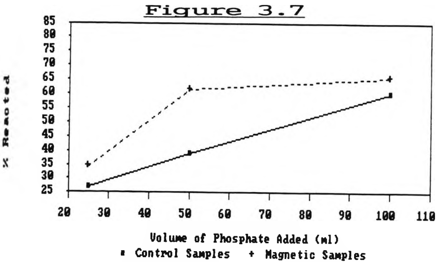
Percentage Magnesium Reacted Results for Experiment 3.
