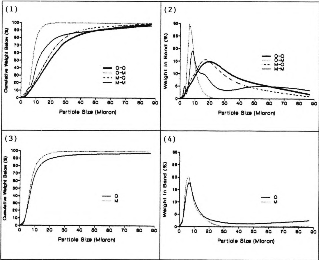
Particle Size Distribution Graphs - Barium in Aqueous Sol n and Sulphate in 2.9% NaCl (aq) (X-Y*).
