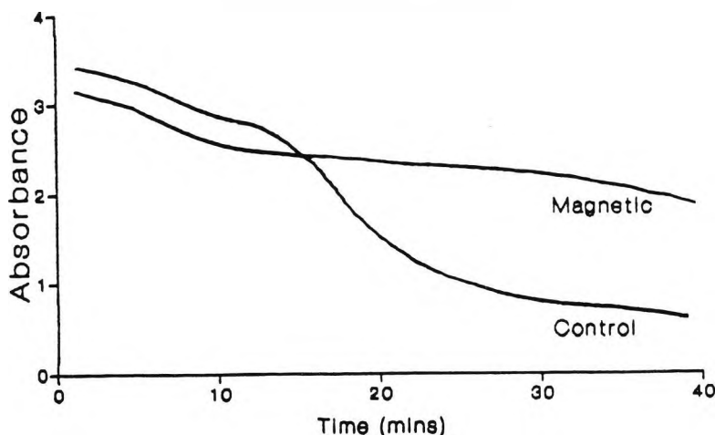
Graph of Absorbance vs. Time for Precipitate Settling Rate.
