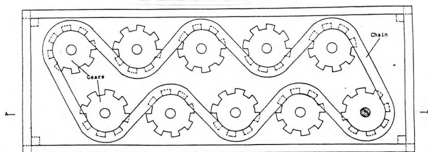
Plan View of the Stirring System Used with the Multiple Test Rig. (N.B. Lid Removed).
