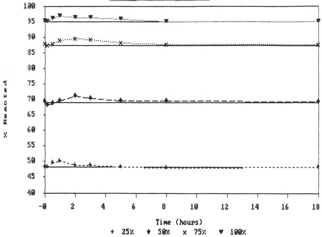
Percentage Calcium Reacted Results for Experiment 5.
