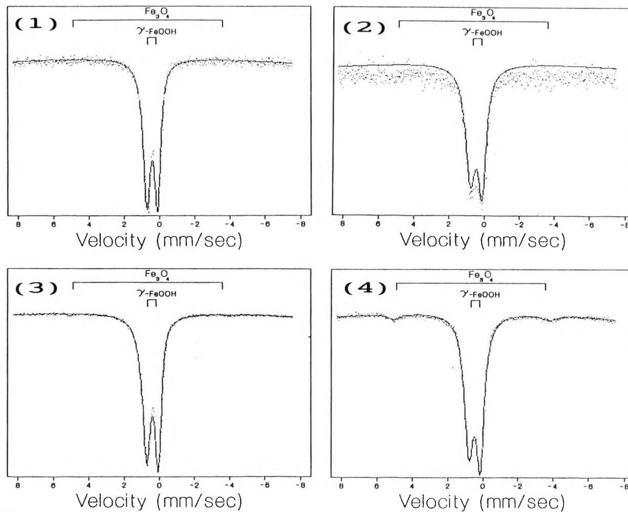
Room Temperature Mössbauer Spectra of Corrosion Products from Experiment 16 (1) Bulk Control (2) Bulk Magnetic (3) Surface Control (4) Surface Magnetic.
