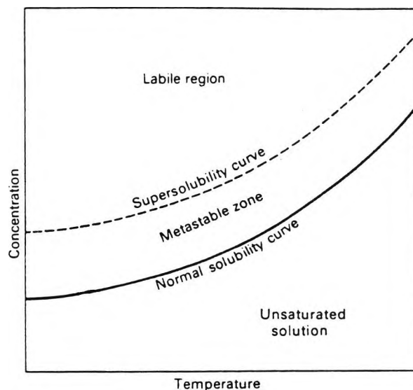
Solubility Curves.
