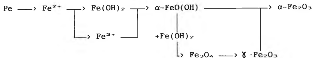
Hiller's Scheme for the Mechanism of Corrosion.
