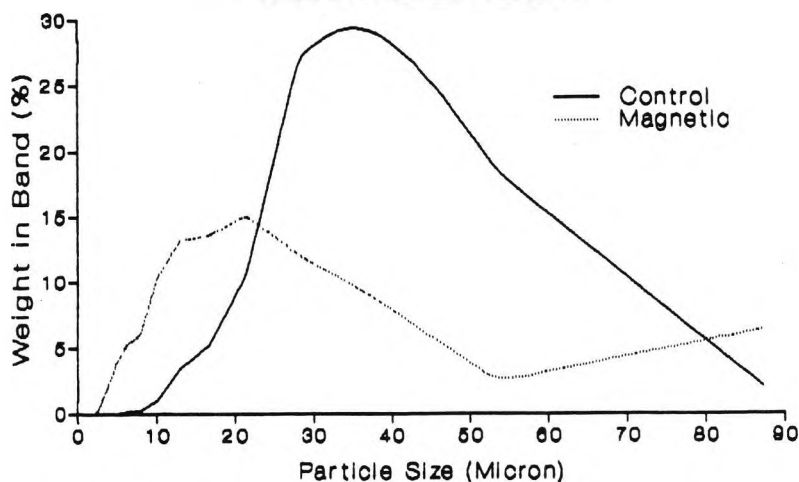
Particle Size Distribution - Weight in Band.
