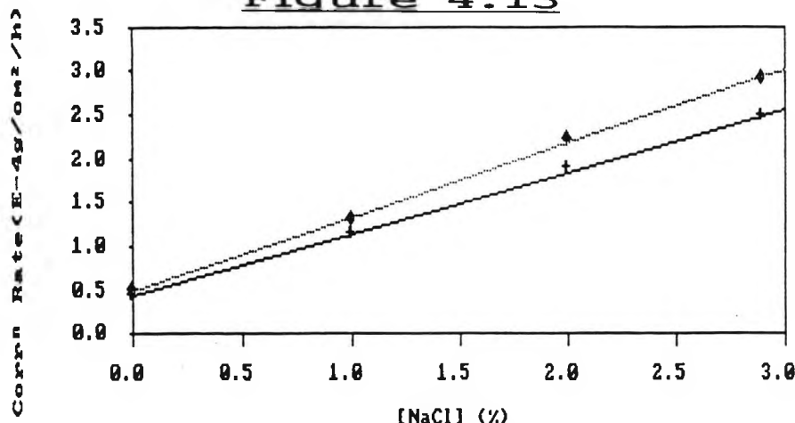
+ Control Runs ♦ Magnetic Runs Corrosion Rates at Different [NaCl] Concentrations (6.0mm Diameter Balls).
