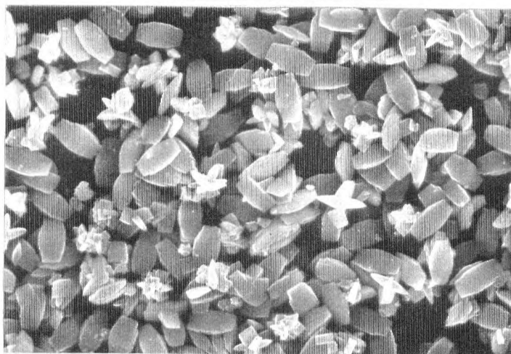
Electron Micrograph (x1000) of O-M* Run Sample.
