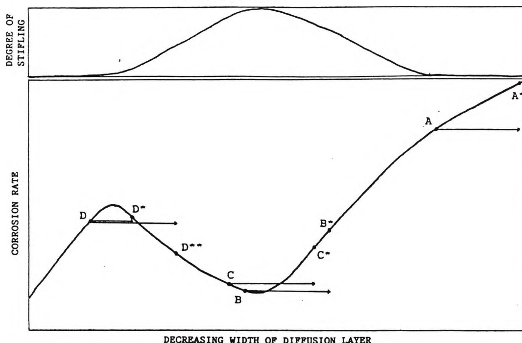
Effect of Decreasing Diffusion Layer Width on Stifling and Corrosion.
