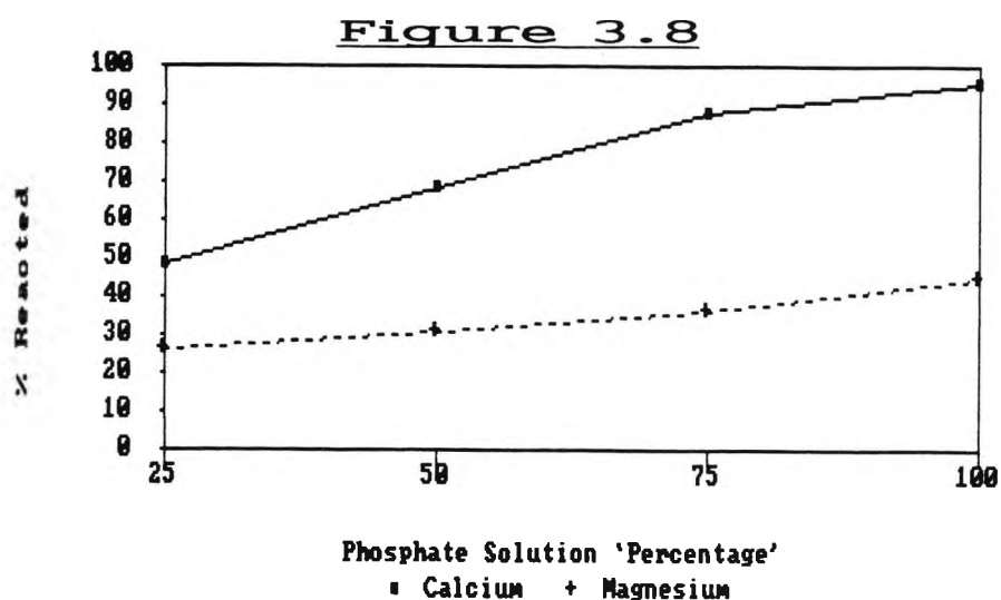
Graphs of Average Replicate Control Runs for Experiment 4.
