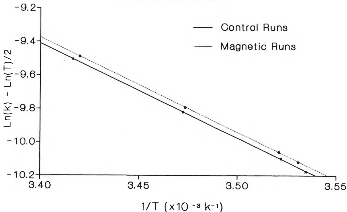
Graph of Results of Experiment 2 for the Determination of E and A' .
