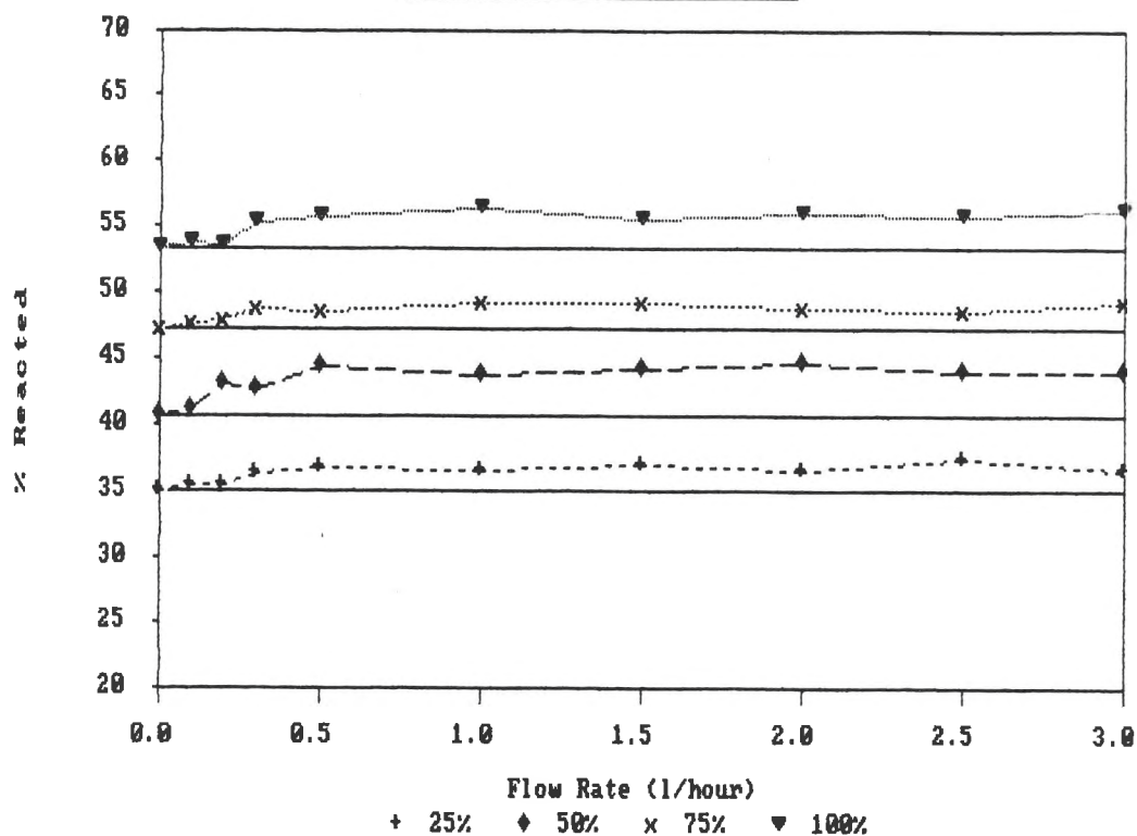
Percentage Magnesium Reacted Results for Experiment 6. (Recirculating - Narrow Tube)
