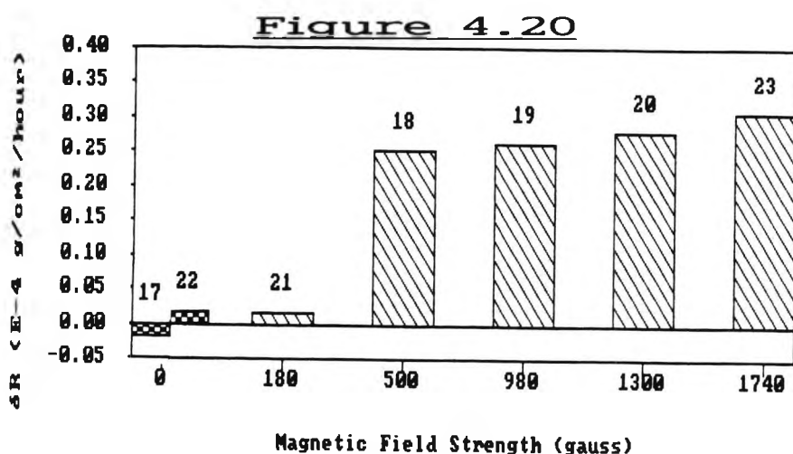
Results of Experiments 17 to 23 Against Field Strength.
