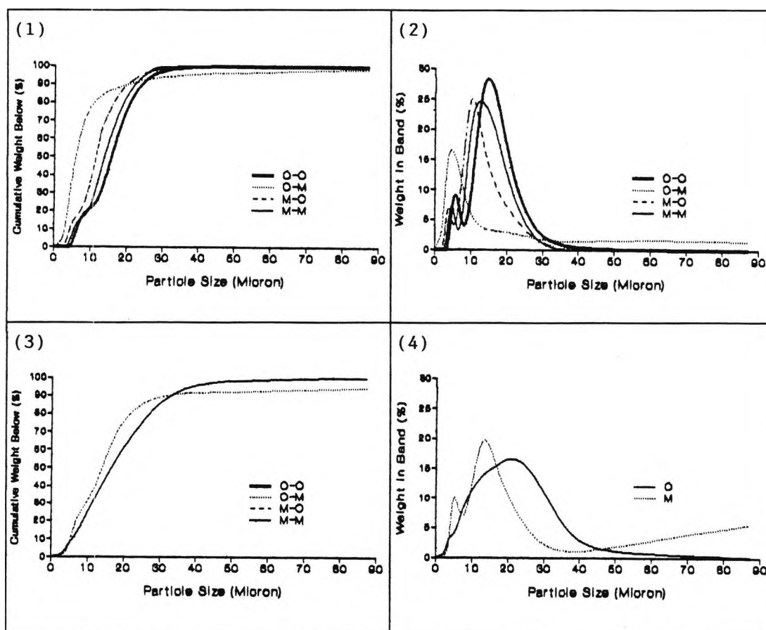
Particle Size Distribution Graphs - Both Barium and Sulphate in Aqueous Solution (X-Y).
