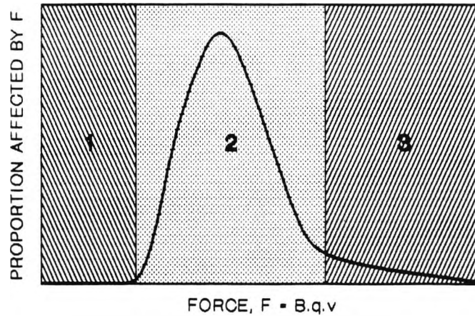
Theoretical Distribution of Energy of Interionic Associations.
