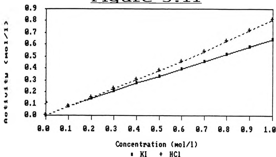
Graphs of Activity Against Concentration for KI (aq) and HCl (aq) .
