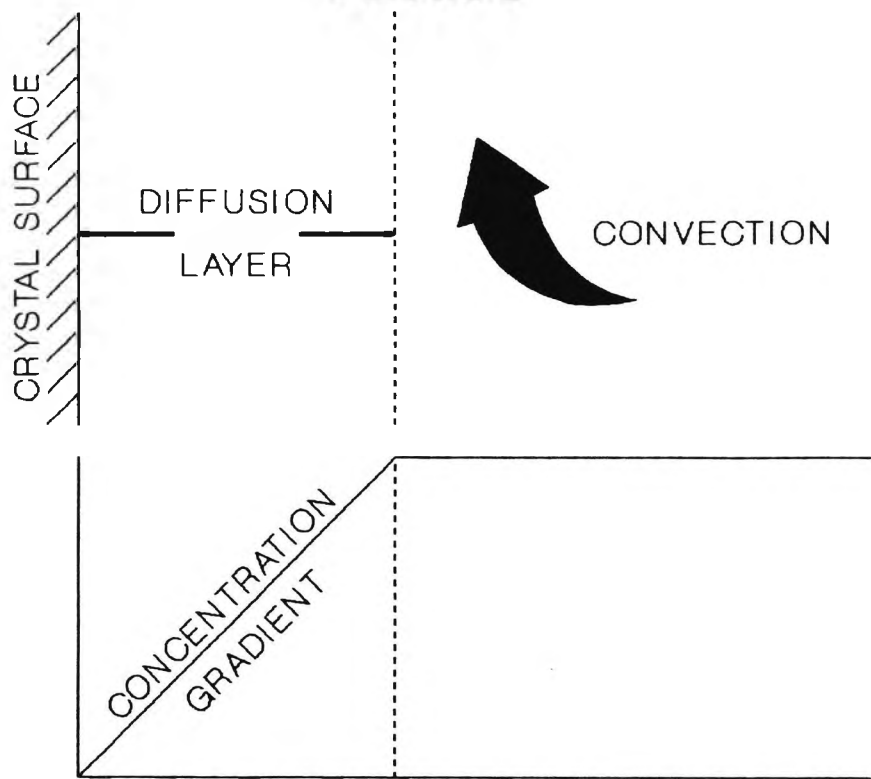
Diagram of Diffusion Layer Near to a Crystal/Solution Interface.
