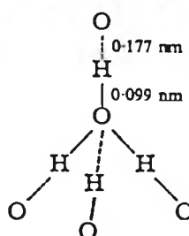
Tetragonal Structure of Water Molecules in Ice.
