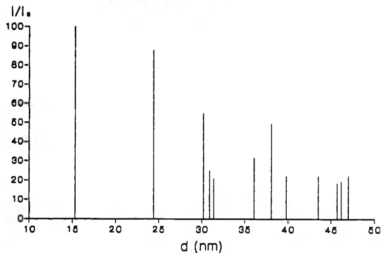
X-ray Diffractogram - Magnetic Run Sample.
