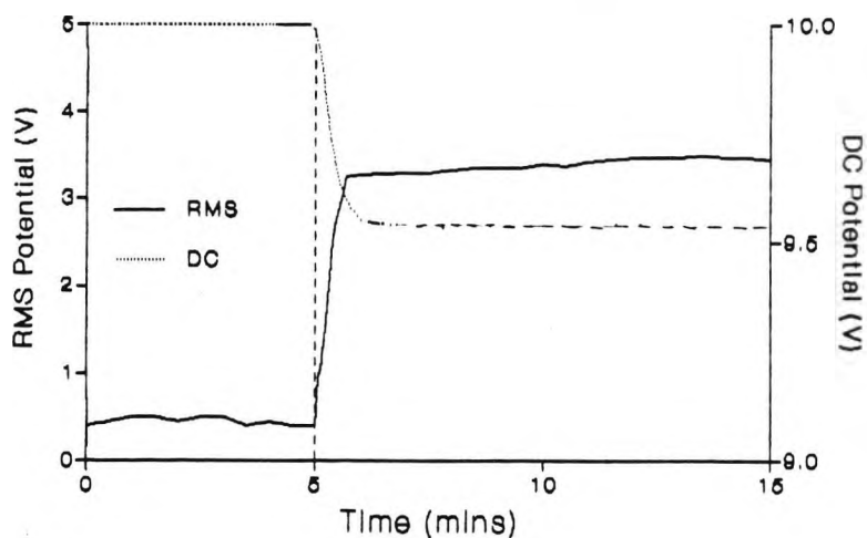
PDA2000 Graph - Magnetic Run.
