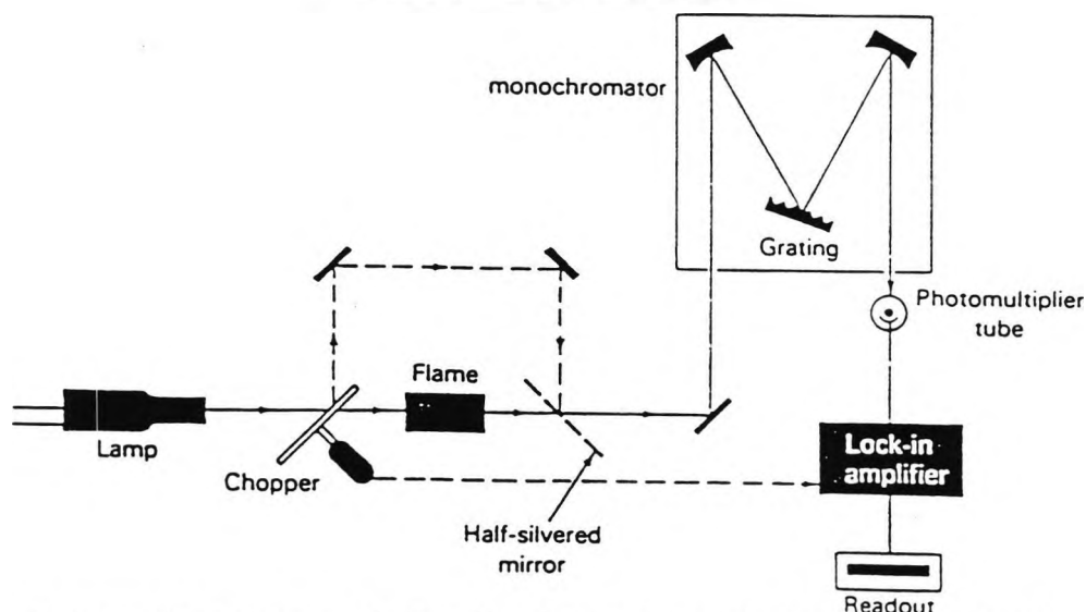
Schematic Diagram of Double Beam A.A. Spectrophotometer.
