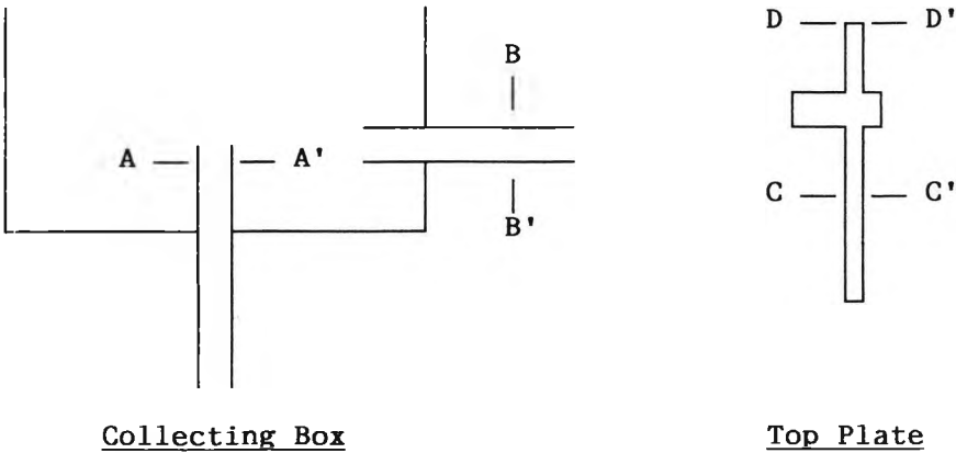
Position of Measurements for Degree of Scaling Determination.
