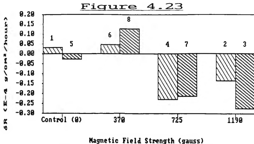
Graph of Corrosion Rate Results for Experiment 26.
