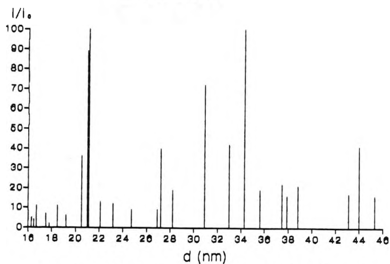
X-ray Diffractogram for M-M* Run Sample.
