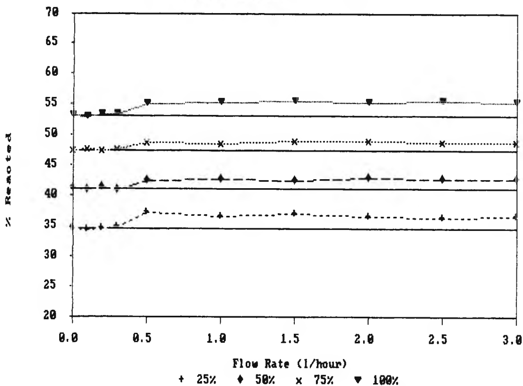
Percentage Magnesium Reacted Results for Experiment 9. (Single Pass - Wide Tube)
