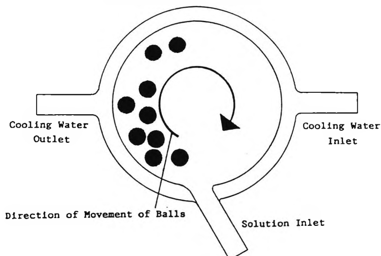
Modified Jacketed Vessel used in Corrosion Experiments.
