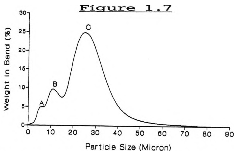
Particle Size Analysis as Weight in Band vs. Particle Size.
