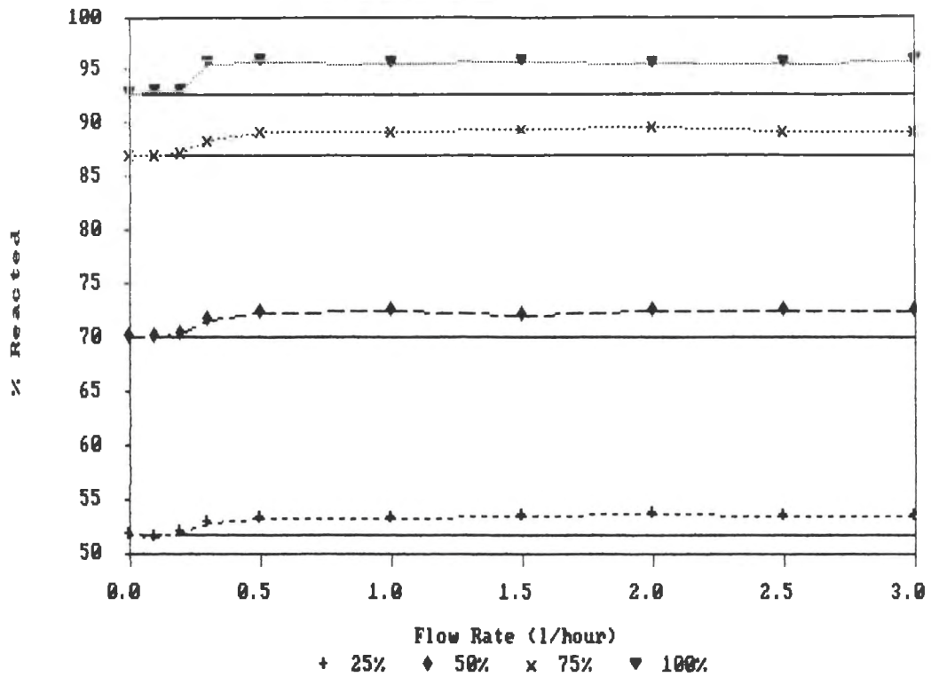
Percentage Calcium Reacted Results for Experiment 8. (Single Pass - Narrow Tube)
