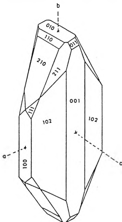
Crystal Growth Habit of Barium Sulphate.
