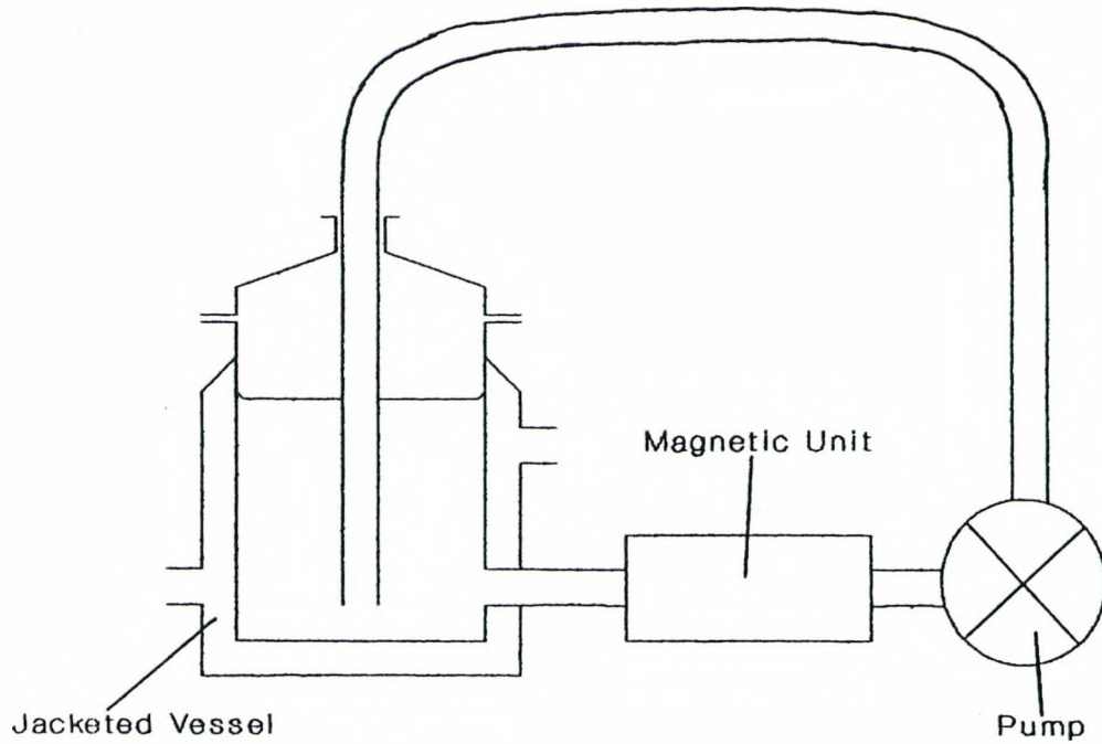
Schematic Diagram of Jacketed Vessel Test Rig.
