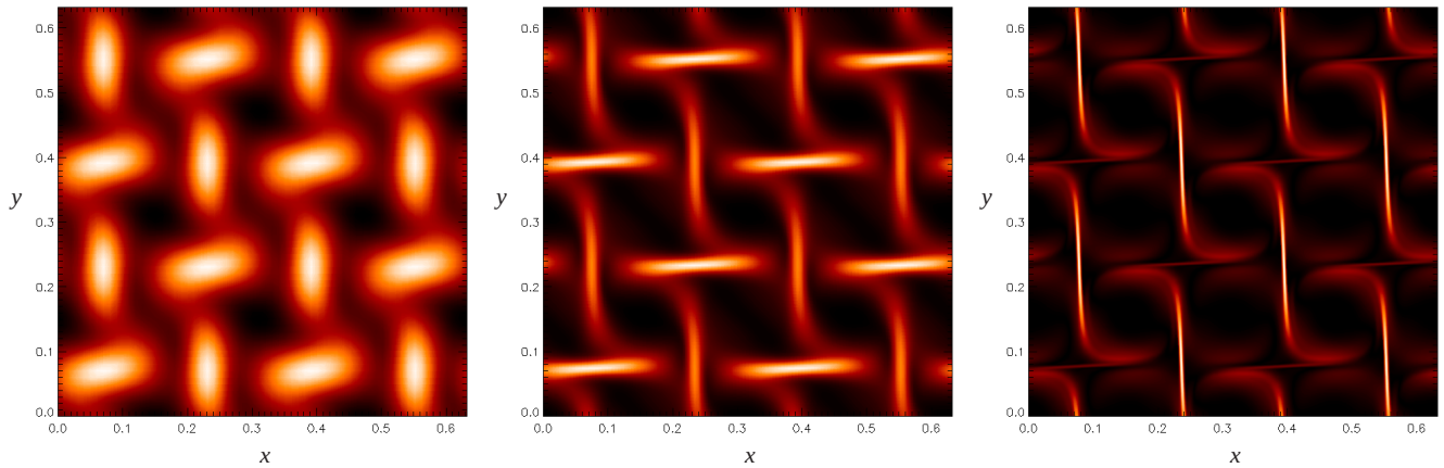
FIG. 5. Magnetic energy B^2 in a horizontal plane located at z = 0.25 . For the sake of clarity, the aspect ratio has been multiplied by two by plotting four copies of the domain side by side. Bright and dark tones correspond to opposite polarity. From left to right, \eta = 10^{-2} (close to the critical value for dynamo action), \eta = 10^{-3} and \eta = 5 \times 10^{-5} (small-scale dynamo action is possible). The horizontally-averaged magnetic field is oriented in the same direction in all cases.
