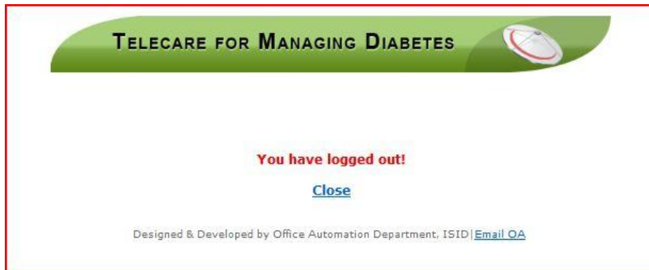
Figure 7.17: Logout webpage
