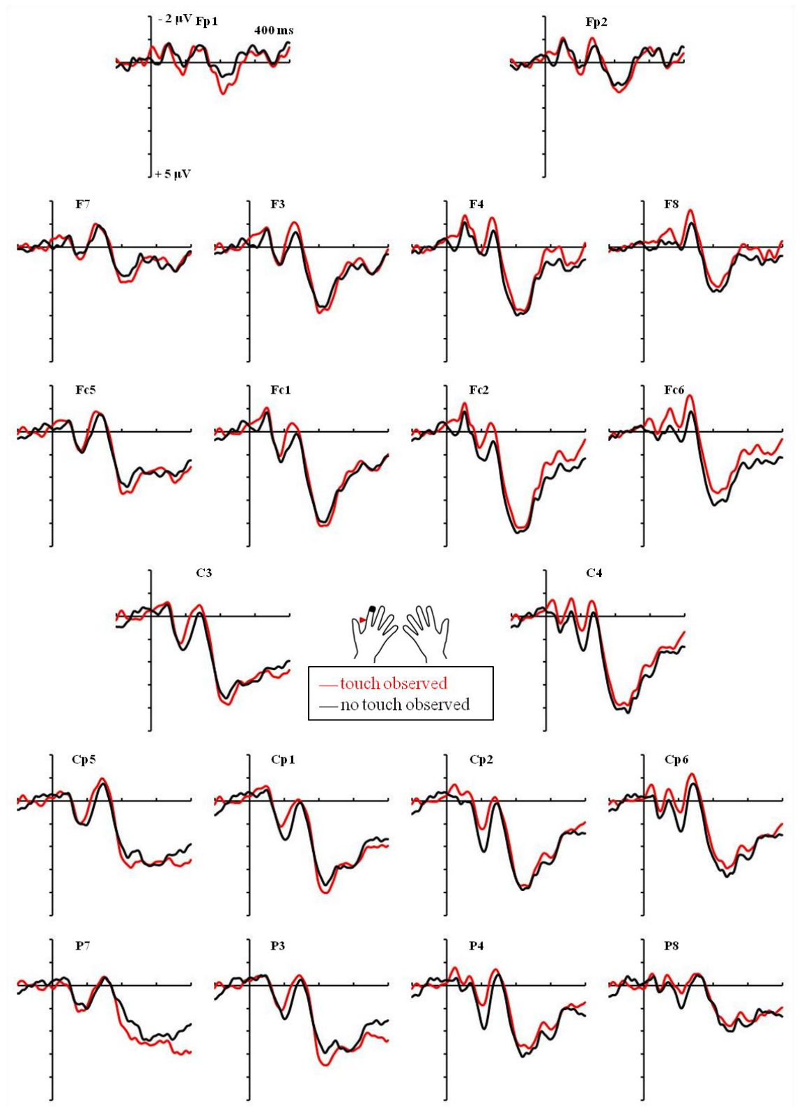
Fig. 2.3.c. Grand-averaged ERP waveforms in response to tactile stimuli to the base segment of the left index finger (IndexBase left ) during the observation of touch (red line) resp. no touch (black line) on the model's index finger tip. Shown are all electrode sites included in the statistical analysis.
