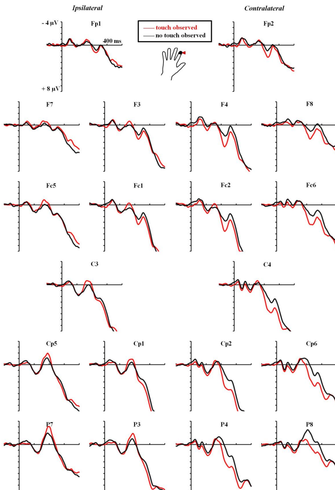
Fig. 3.5.a. Grand-averaged ERP waveforms in response to tactile stimuli to the left index finger tip during the observation of the model's index finger tip touch the object (red line) rather than merely the empty space next to it (black line). Shown are all electrode sites included in the statistical analysis.
