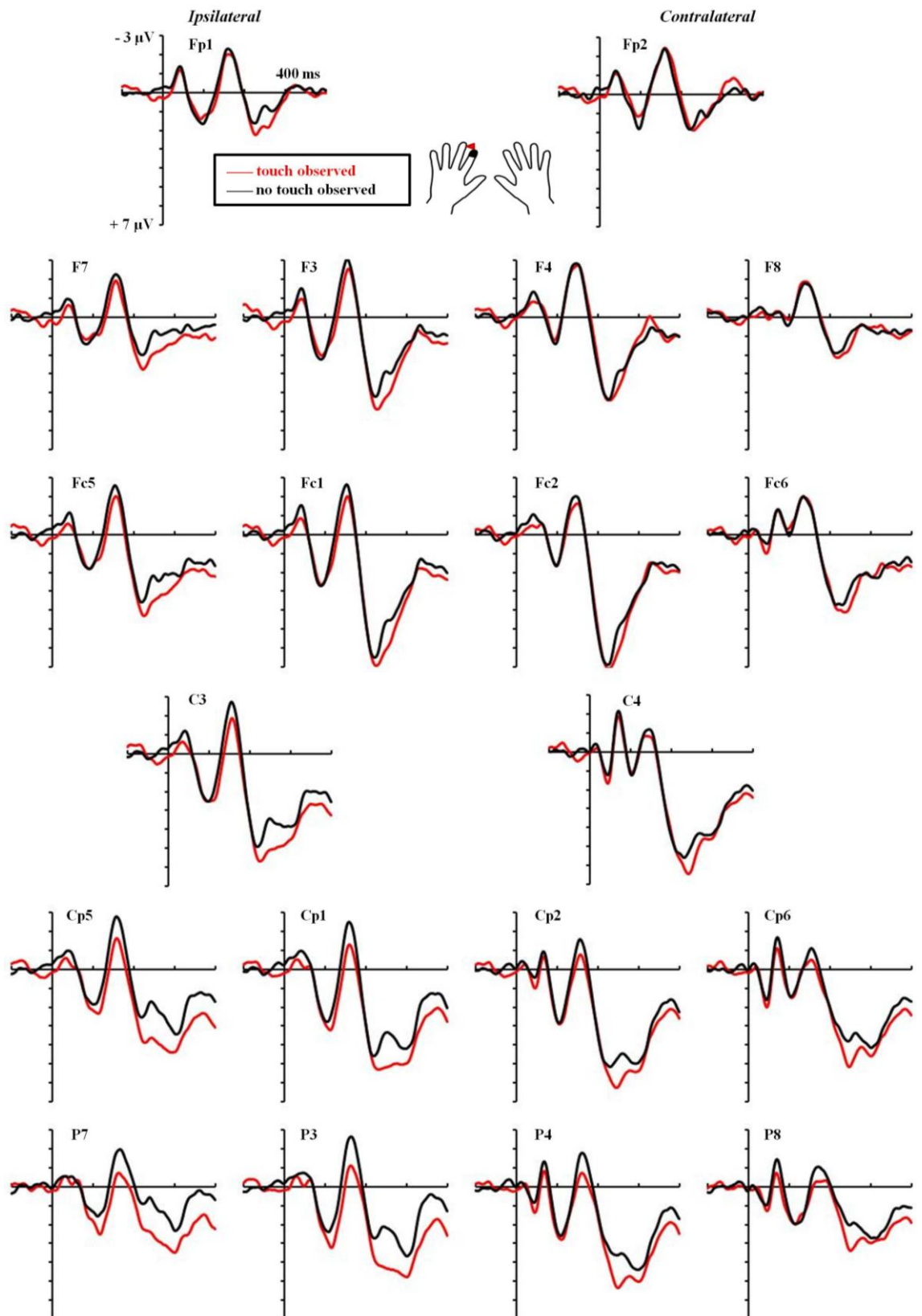
Fig. 3.2.d. Grand-averaged ERP waveforms in response to tactile stimuli to the left middle finger tip (MiddleTip left ) during the observation of the model's index finger tip touch the object (red line) rather than merely the empty space next to it (black line). Shown are all electrode sites included in the statistical analysis.
