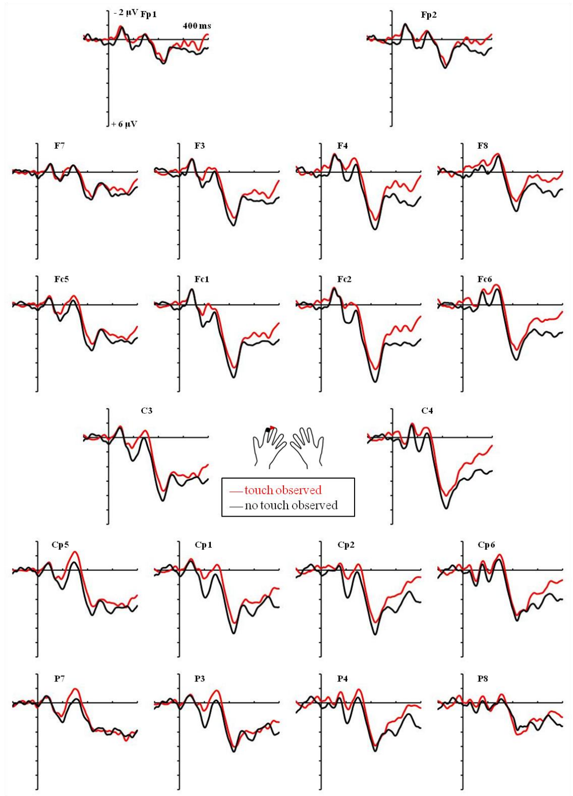
Fig. 2.3.d. Grand-averaged ERP waveforms in response to tactile stimuli to the left middle finger tip (MiddleTip left ) during the observation of touch (red line) resp. no touch (black line) on the model's index finger tip. Shown are all electrode sites included in the statistical analysis.
