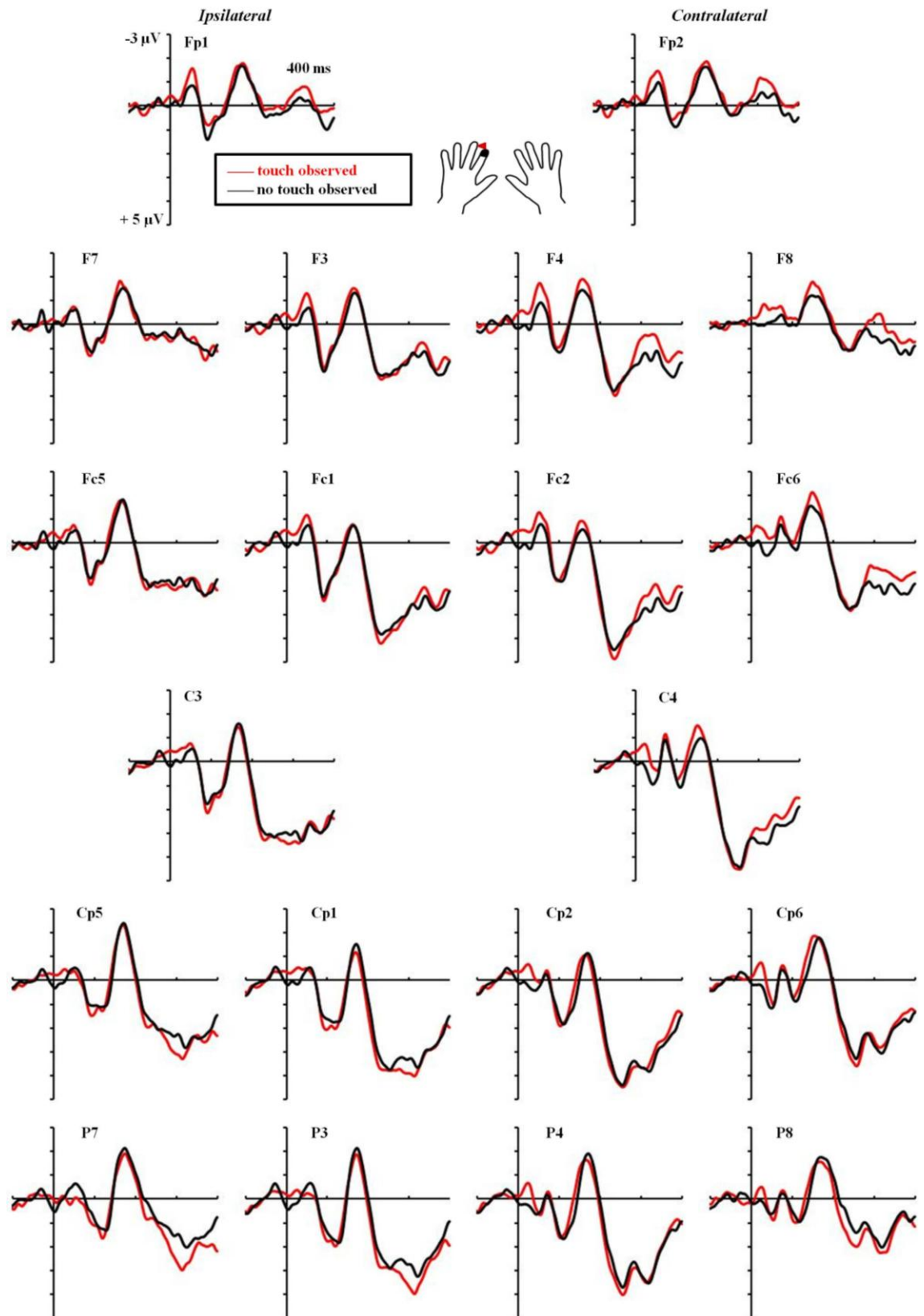
Fig. 3.3.c. Grand-averaged ERP waveforms in response to tactile stimuli to the left middle finger tip (MiddleTip left ) during the observation of the model's index finger tip touch the object (red line) rather than merely the empty space next to it (black line). Shown are all electrode sites included in the statistical analysis.
