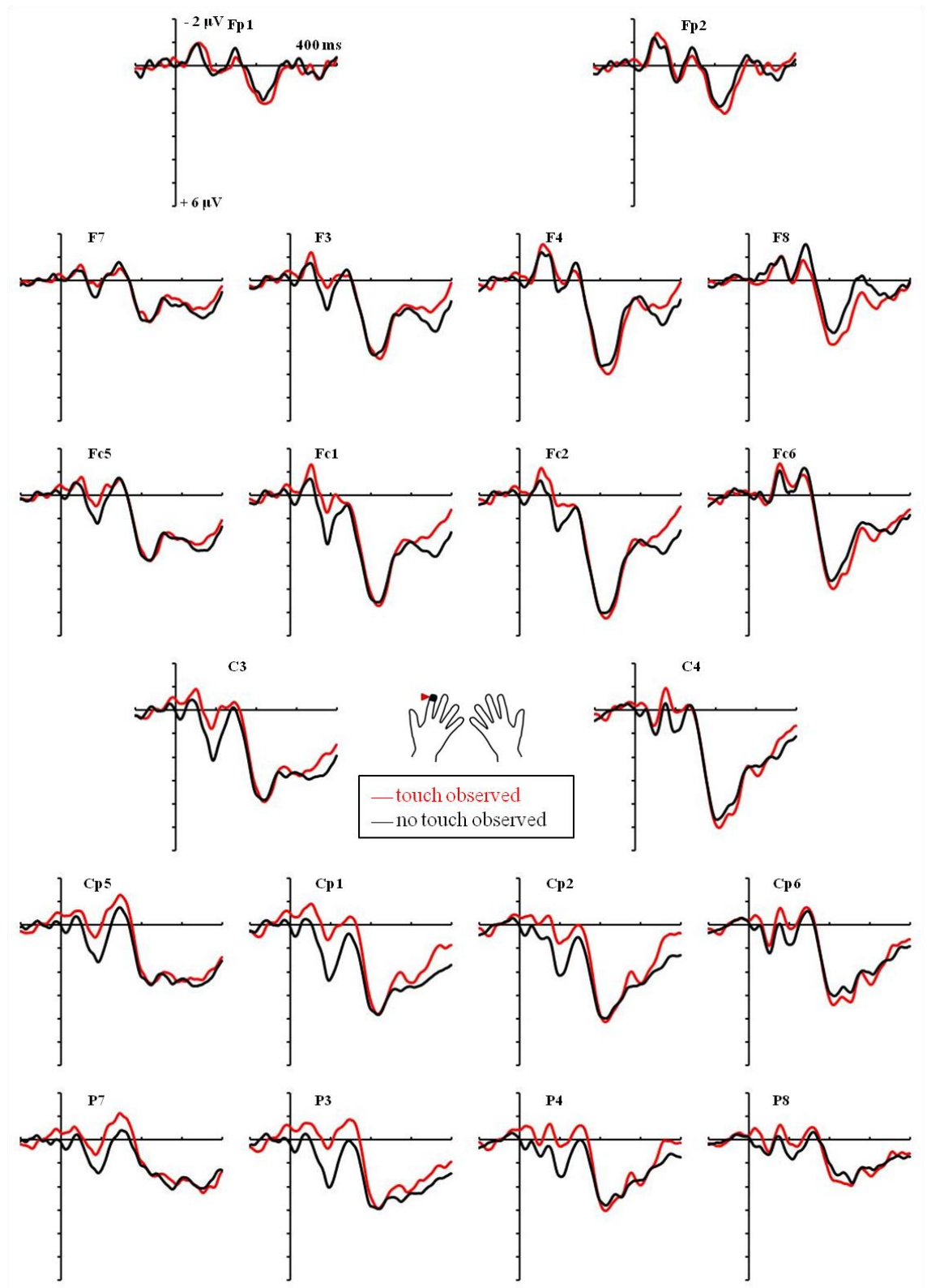
Fig. 2.3.b. Grand-averaged ERP waveforms in response to tactile stimuli to the left index finger tip (IndexTip left ) during the observation of touch (red line) resp. no touch (black line) on the model's index finger tip. Shown are all electrode sites included in the statistical analysis.
