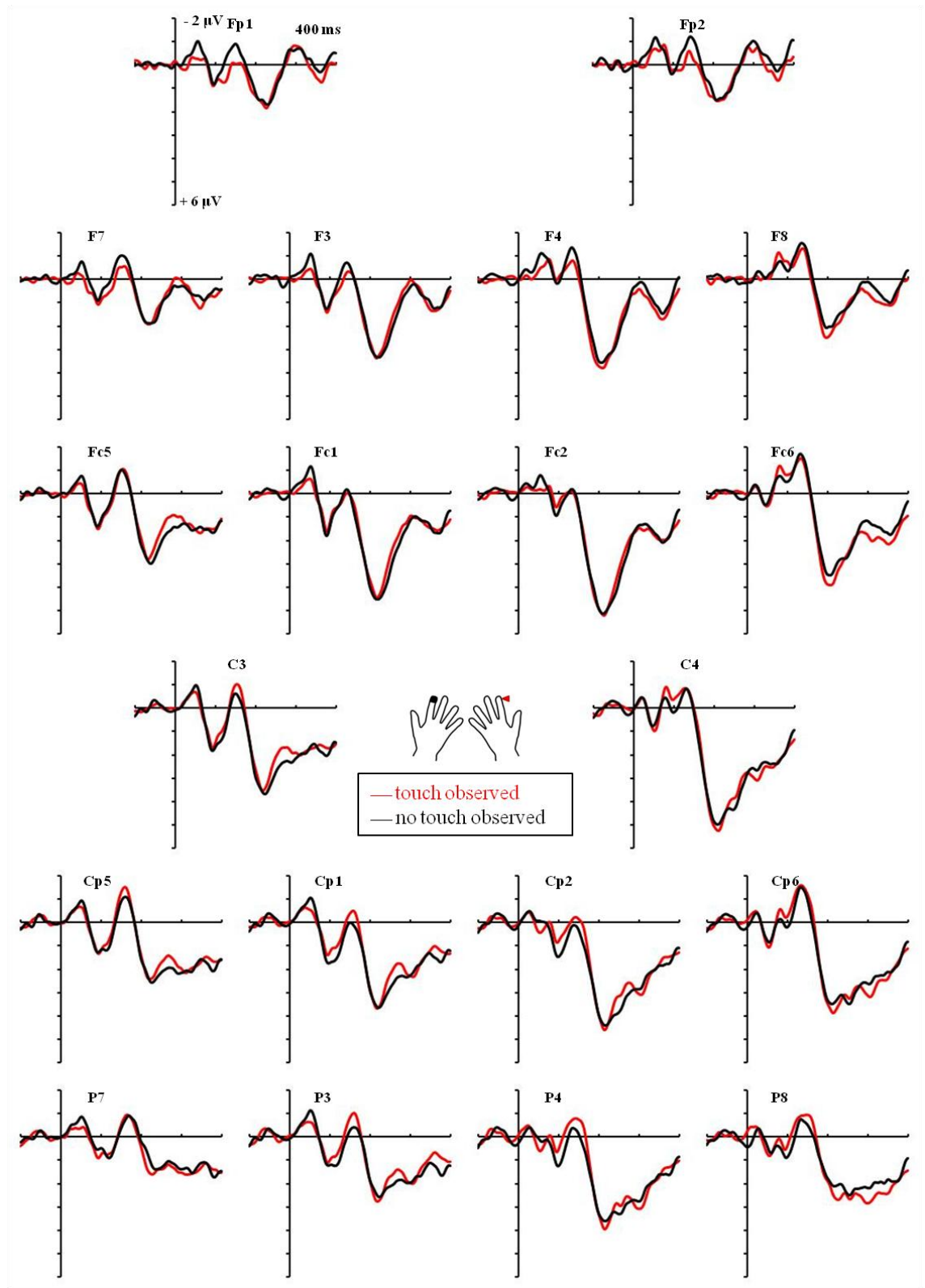
Fig. 2.3.e. Grand-averaged ERP waveforms in response to tactile stimuli to the right index finger tip (IndexTip right ) during the observation of touch (red line) resp. no touch (black line) on the model's index finger tip. Shown are all electrode sites included in the statistical analysis.
