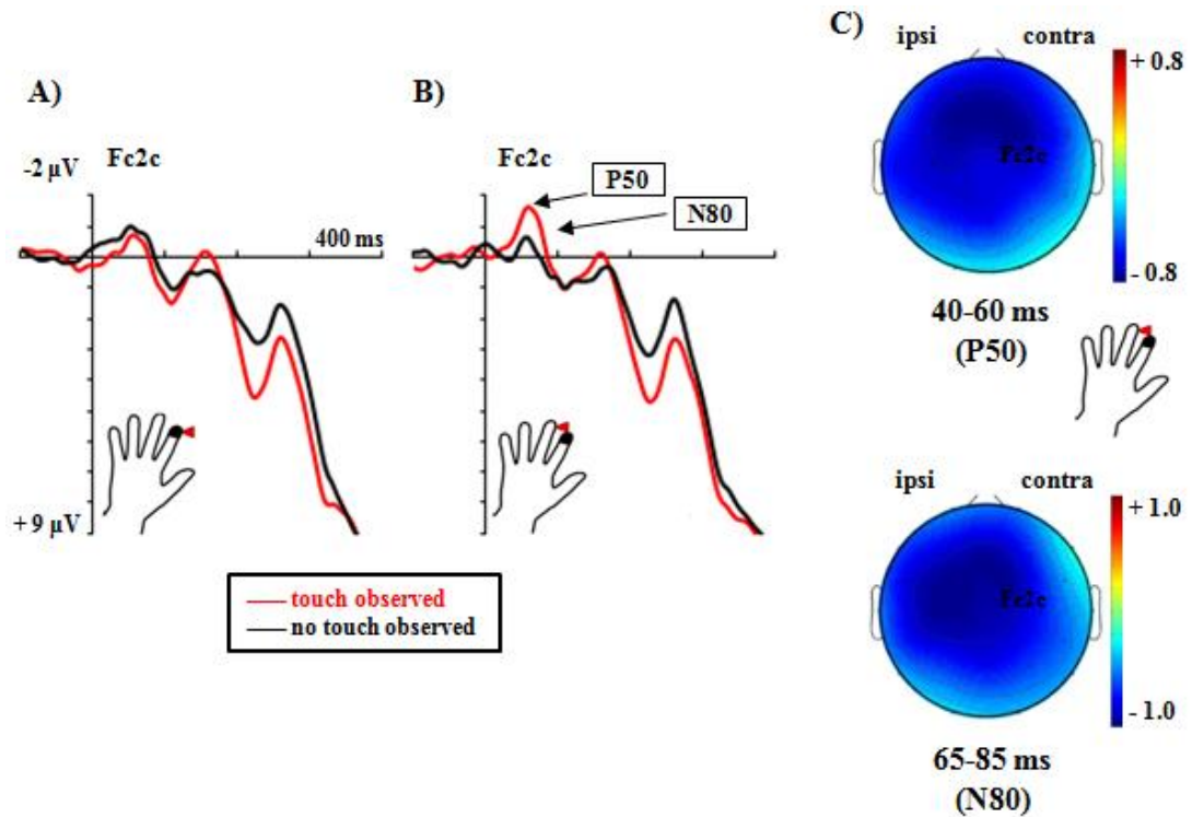
Fig. 3.5.c. Grand-averaged ERP waveforms in response to tactile stimuli to the anatomically congruent index finger (A) and the adjacent middle finger (B) during the observation of the model's index finger tip touch the object (red line) rather than merely the empty space next to it (black line), at a representative fronto-central electrode over the hemisphere contralateral to the stimulated hand (Fc2c). The scalp maps in (C) show the topographic distribution of the significant touch observation-related ERP amplitude differences in the P50 and N80 latency range during tactile stimulation of the adjacent middle finger. Note that a negative difference indicates an increased negativity for both the P50 (whose polarity is reversed to negative at anterior electrodes) and the N80 amplitude during the sight of touch.
