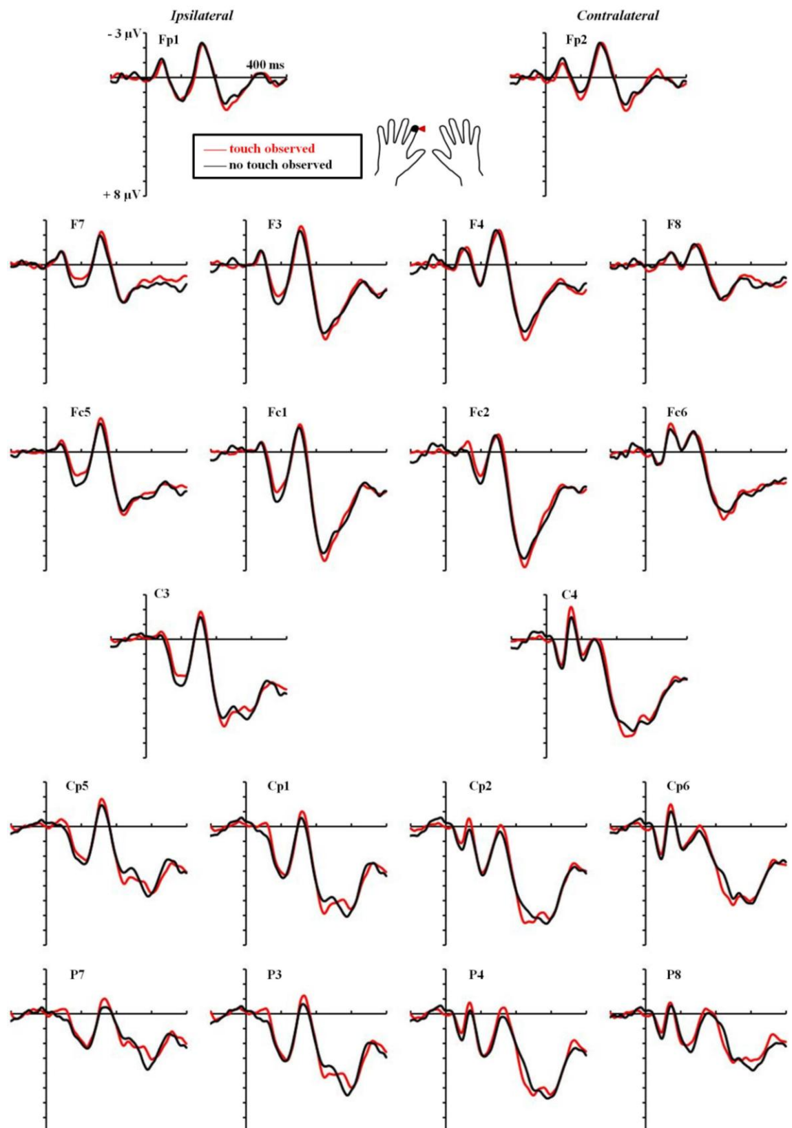
Fig. 3.2.b. Grand-averaged ERP waveforms in response to tactile stimuli to the left index finger tip (IndexTip left ) during the observation of the model's index finger tip touch the object (red line) rather than merely the empty space next to it (black line). Shown are all electrode sites included in the statistical analysis.
