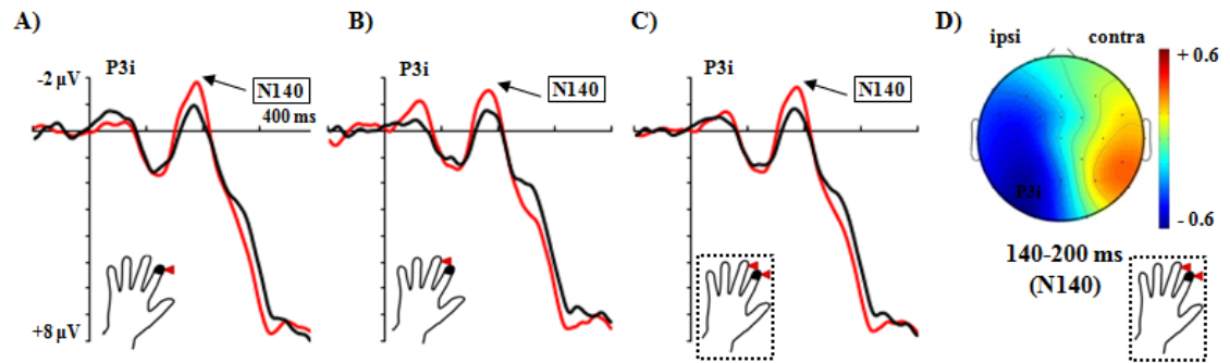
Fig. 3.5.d. Grand-averaged ERP waveforms in response to tactile stimuli to the anatomically congruent index finger ( A ), the adjacent middle finger ( B ) and when collapsing across both stimulated fingers ( C ) during the observation of the model's index finger tip touch the object (red line) rather than merely the empty space next to it (black line), at a representative parietal electrode over the hemisphere ipsilateral to the stimulated hand (P3i). The scalp map in ( D ) shows the topographic distribution of the significant touch observation-related ERP amplitude differences (touch – not touch) in the N140 latency range when averaged across both tactually stimulated fingers. Note that a negative difference reflects an increased N140 amplitude during the sight of touch.
