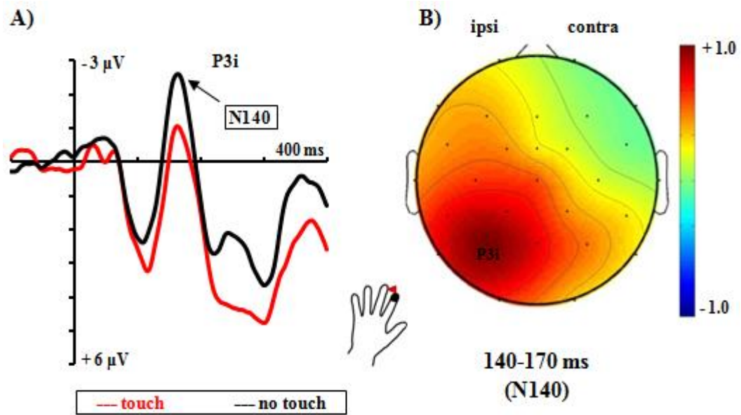
Fig. 3.2.g. A) Grand-averaged ERP waveforms in response to tactile stimuli to the left middle finger tip (MiddleTip left ) during the observation of the model's index finger tip touch the object (red line) rather than merely the empty space next to it (black line), at a representative parietal electrode (P3i) over the hemisphere ipsilateral to the stimulated finger. B) Topographic distribution of the difference in SEP mean amplitude for the two observational conditions for the 140-170 ms post-stimulus latency range during tactile stimulation of the left middle finger tip. Note that a positive difference indicates a decreased N140 amplitude during the sight of touch.
