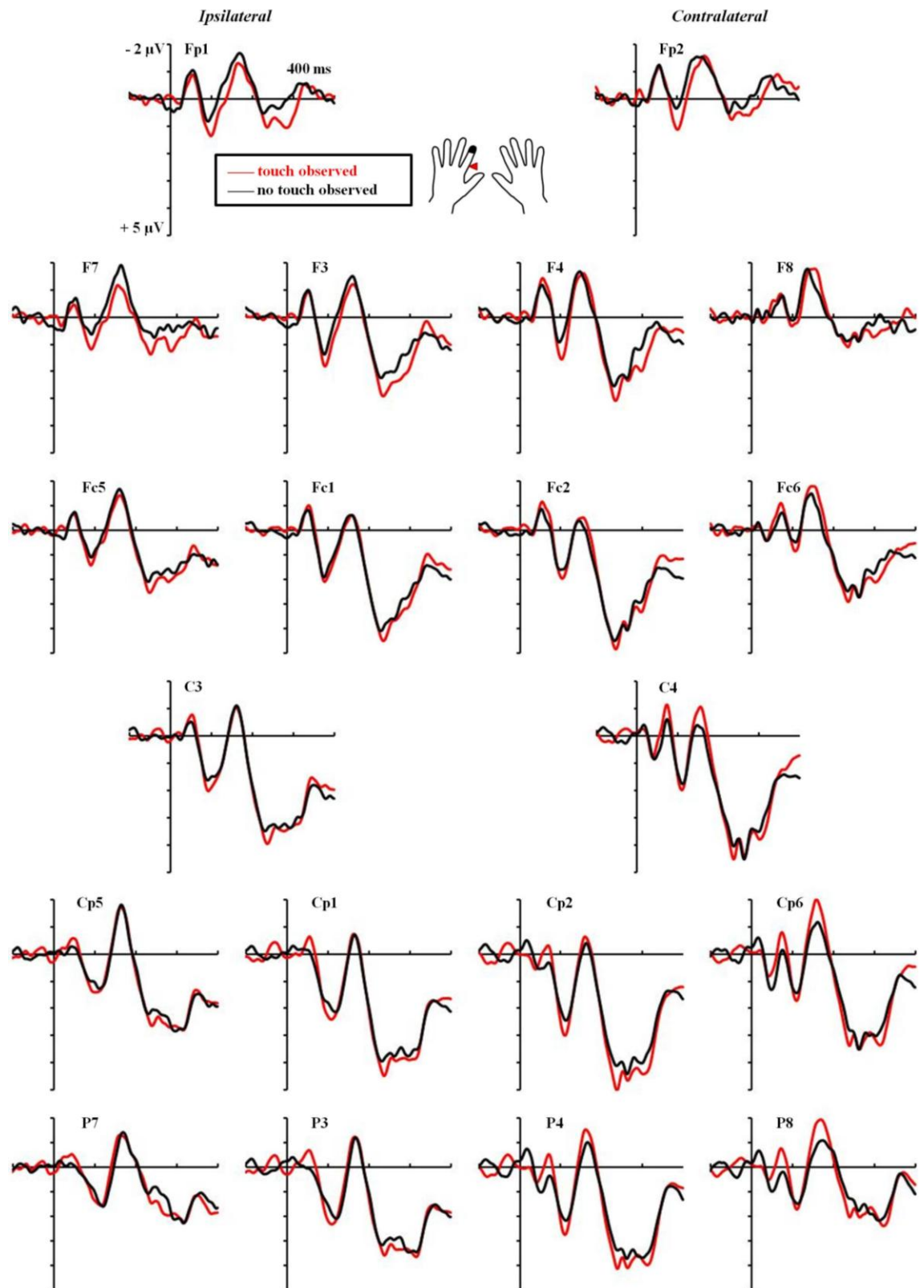
Fig. 3.3.b. Grand-averaged ERP waveforms in response to tactile stimuli to the base segment of the left index finger (IndexBase left ) during the observation of the model's index finger tip touch the object (red line) rather than merely the empty space next to it (black line). Shown are all electrode sites included in the statistical analysis.
