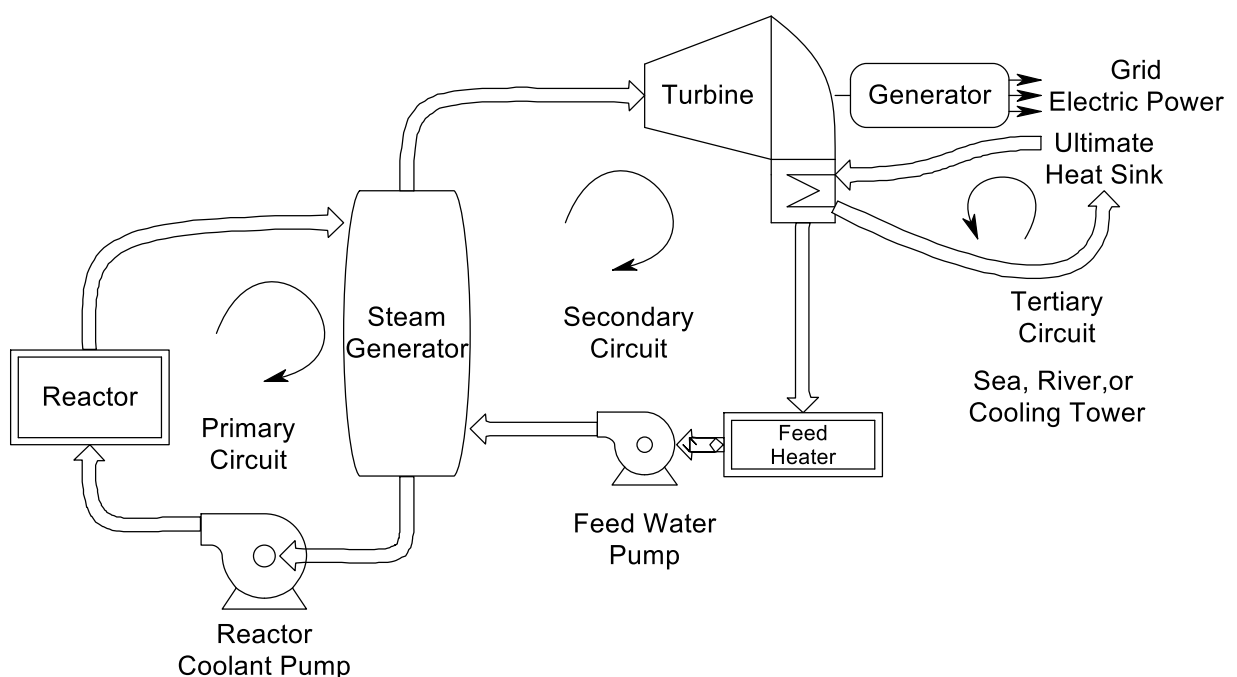
Figure 2.5 Typical NPP Layout of Heat Transfer Circuits
