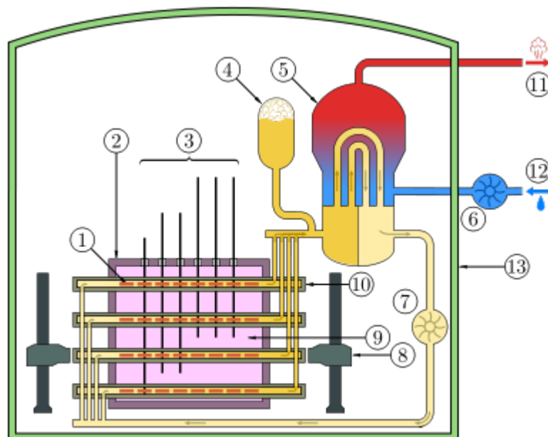
Figure 2.14 Schematic of the Primary Loop of a CANDU Reactor (Wikipedia.org)
