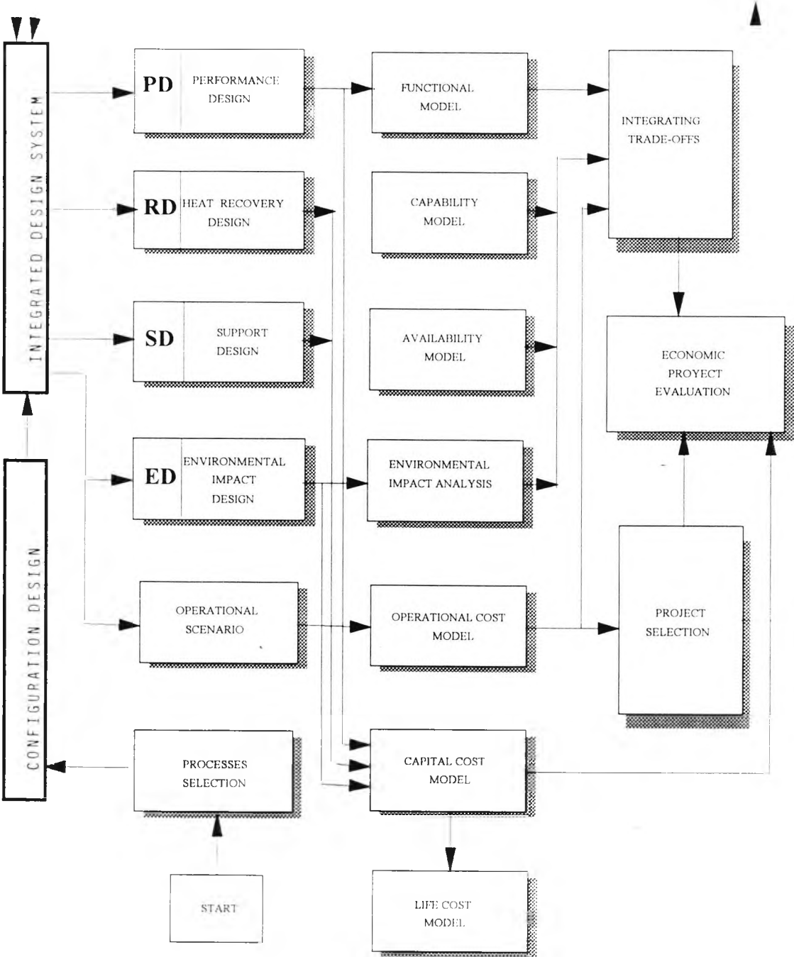
FIGURE 4.7.a. FRAMEWORK FOR INTEGRATED REFINERY DESIGN TO IMPROVE ENERGY USAGE PRODUCTIVITY
