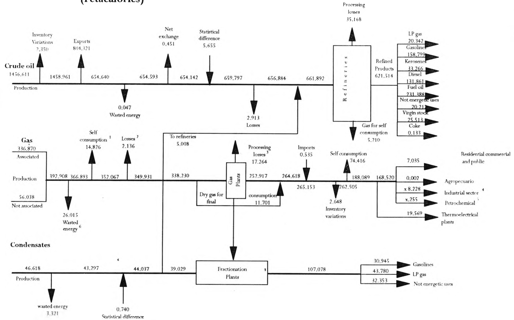
Diagram 2.3.d.2 Hydrocarbons balance 1985 8 / / (Petacalories)
