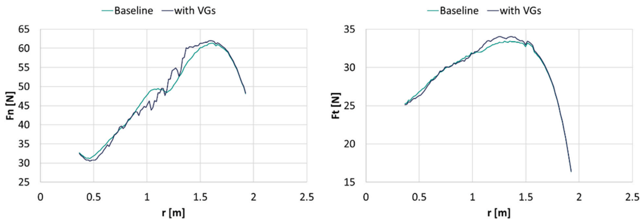
Fig. 27. Normal and tangential forces on the full-size turbine blade with and without vortex generators for \lambda = 3 and an inflow velocity of V_\infty = 2.0 \text{ m/s} .
