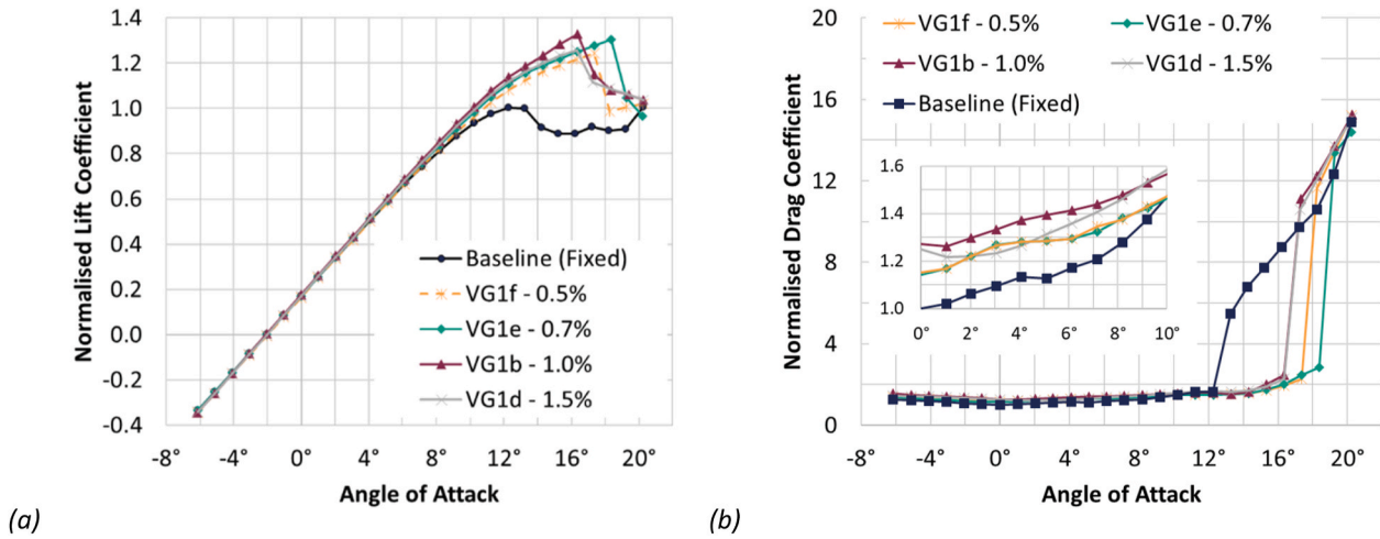
Fig. 10. Normalised lift (a) and drag coefficient (b) variation with angle of attack for varying vortex generator vane heights while testing at Reynolds number of Re = 10^6 under fixed transition conditions.
