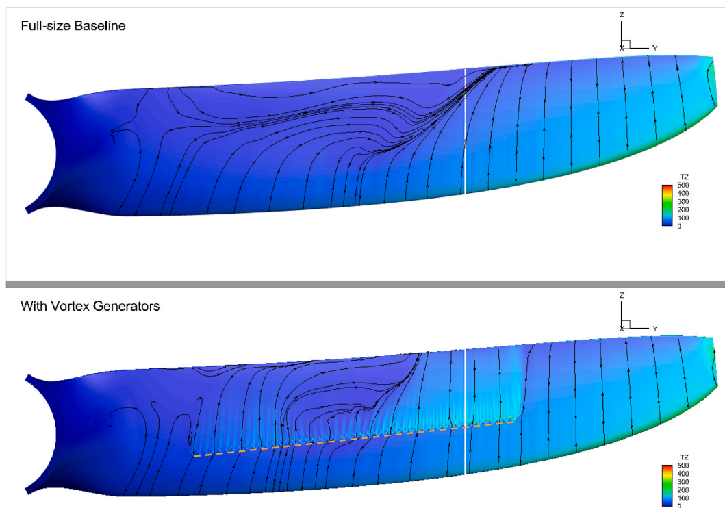
Fig. 23. Chordwise skin friction ( TZ ) contour on the full-size blade suction side without (top) and with vortex generators (bottom) for \lambda = 3 and an inflow velocity of V_\infty = 2.0 m/s. TZ units are N/m^2 . The solid white and the dashed orange line indicate the y = 0.65R and the Vortex Generators' location, respectively.
