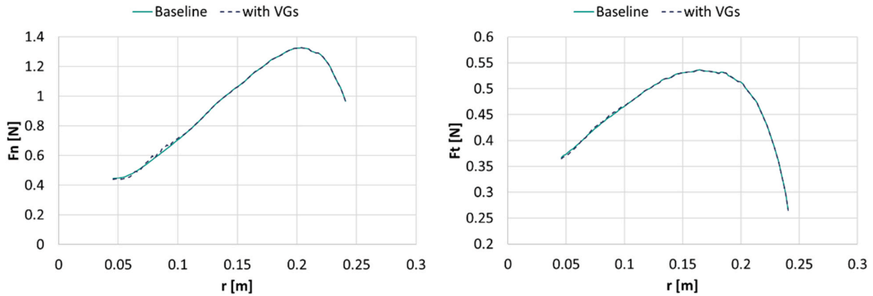
Fig. 20. Normal and tangential forces on the turbine blade with and without vortex generators for \lambda = 4 and an inflow velocity of V_\infty = 2.0 m/s.
