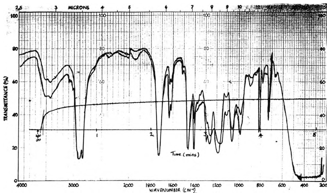
Spectrum 5: RTIR spectrum, showing the polymerization of 2-ethyl-2(hydroxymethyl)-1,3 propanediol triacrylate in the presence of 2,3-bis(4-methoxyphenyl) quinoxaline and N-methyldiethanolamine, under anaerobic conditions.
