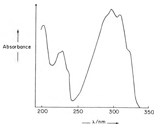
Fig.1.6 Electronic absorption spectrum of trans-stilbene
