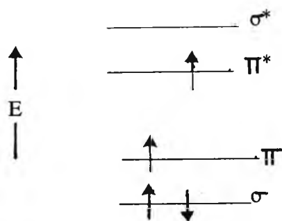
Fig. 1.7 Electronic configuration of the (\pi, \pi^*) triplet state of an alkene.
