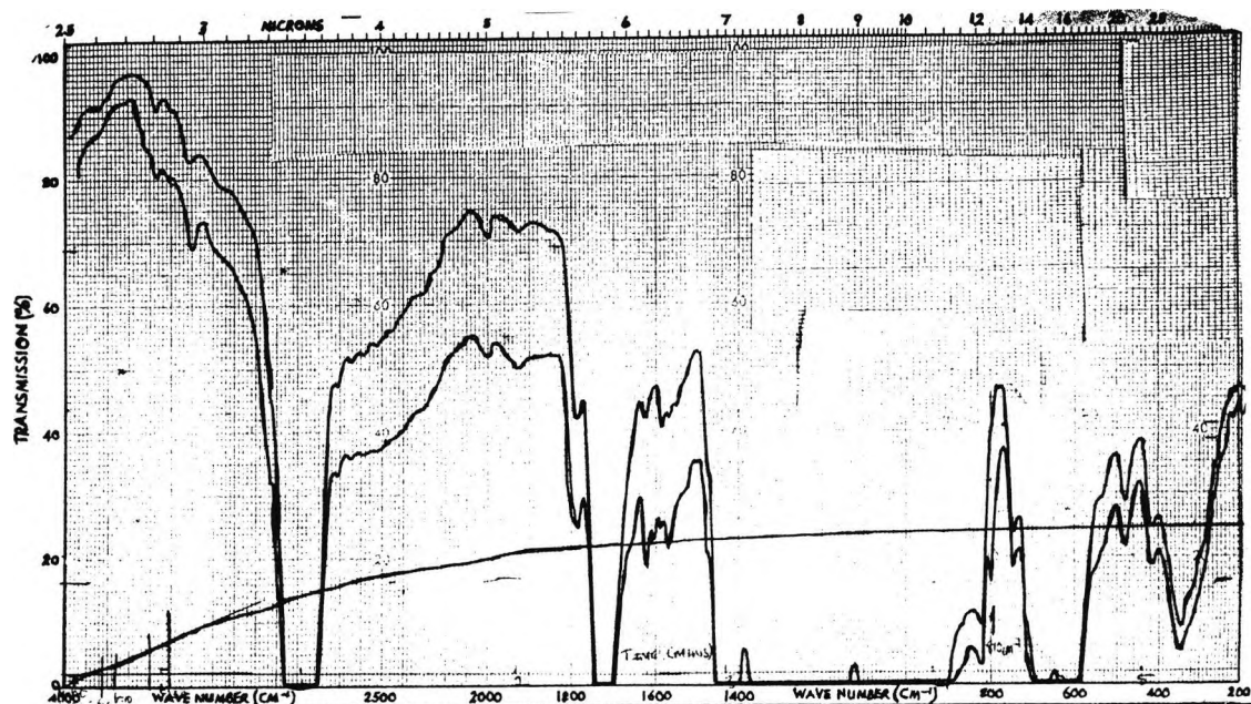
Spectrum 3:- RTIR spectrum, showing the polymerization of 3,6-dithia - 1,8 octane diacrylate in the presence of Irgacure 907 and N-methyldiethanolamine, under anaerobic conditions.
