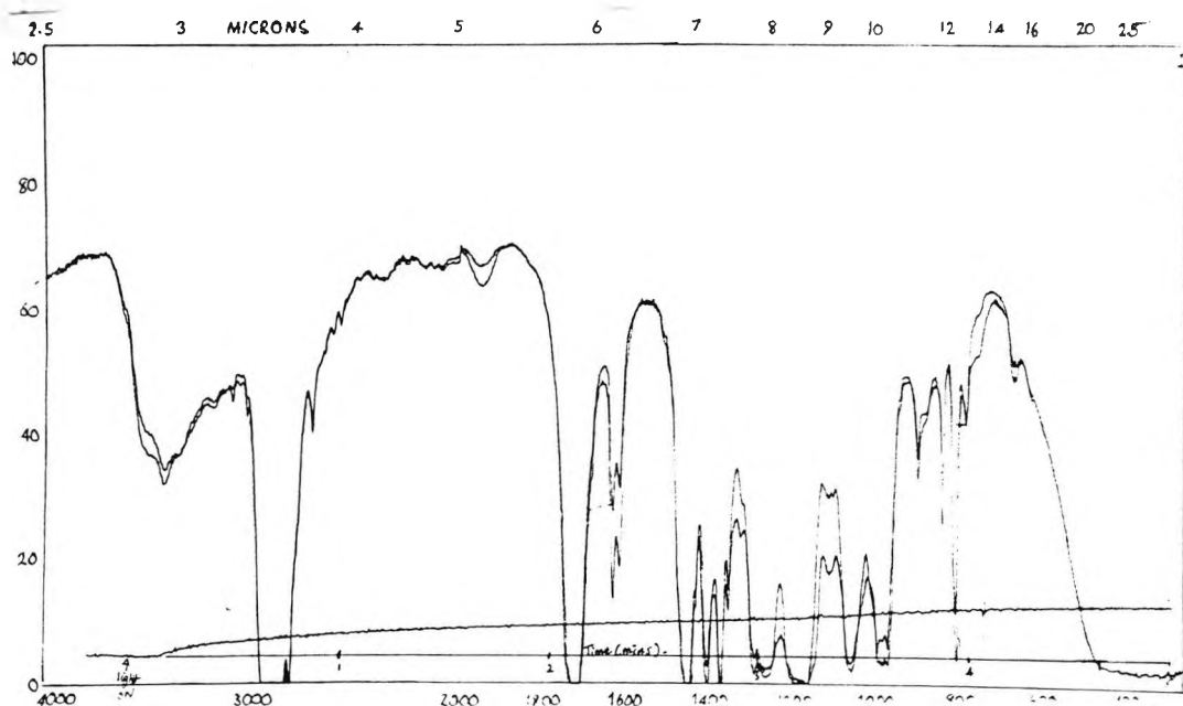
Spectrum 4: RTIR spectrum, showing the polymerization of 2-ethyl-2(hydroxymethyl)-1,3-propanediol triacrylate in the presence of 2,3-bis (4-hydroxyphenyl) quinoxaline and N-methyldiethanolamine, under anaerobic conditions
