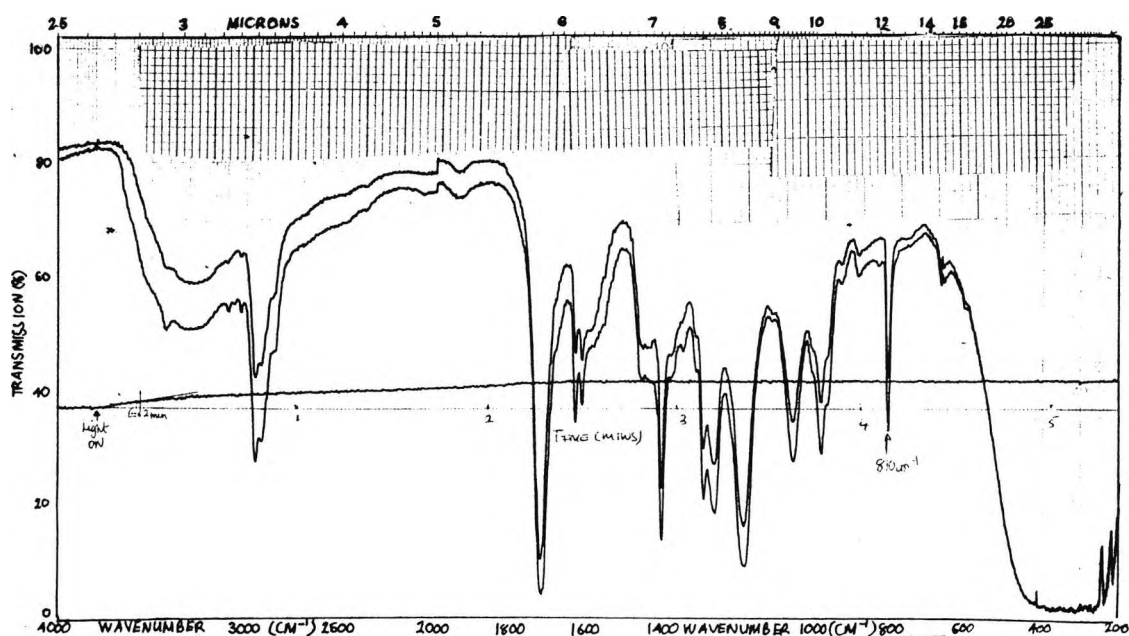
Spectrum 4:- RTIR spectrum, showing the polymerization of 3,6-dithia - 1,8 octane diacrylate in the presence of Irgacure 907 and N-methyldiethanolamine, under aerobic conditions.
