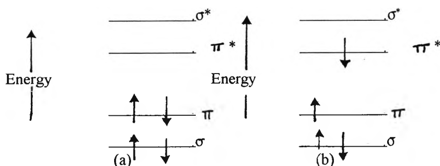
Fig1.5:- Electronic configuration of an alkene, showing the occupancy of the carbon-carbon bond orbitals (a) In the ground state (b) in the ( \pi , \pi^* ) excited single state.
