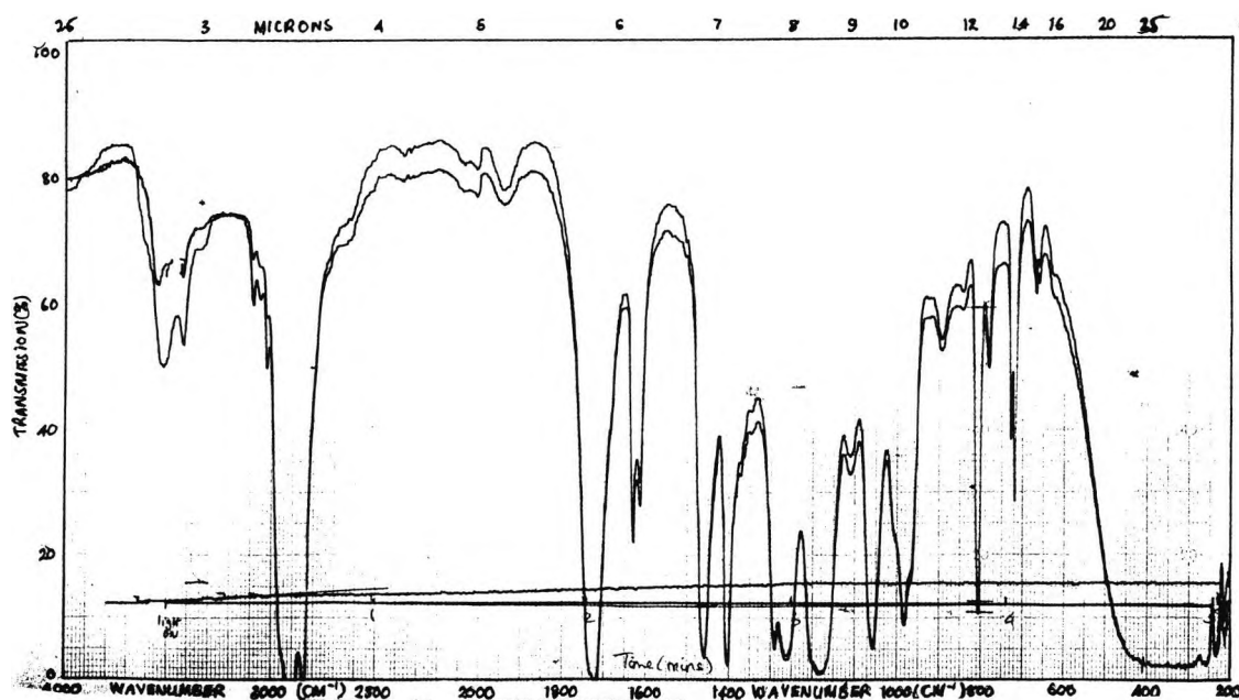
Spectrum 4:- RTIR spectrum, showing the polymerization of 2-ethyl-2(hydroxymethyl)-1,3-propanediol triacrylate in the presence of n^6 -dichlorobenzene- n^5 -cyclopentadienyliron(II)- n -butyltriphenylborate, under aerobic conditions.
