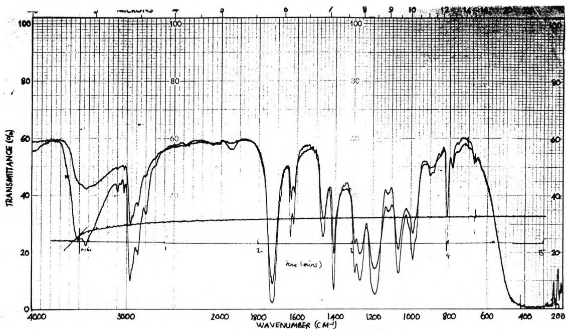
Spectrum 2: RTIR spectrum, showing the polymerization of 2-ethyl-2-(hydroxymethyl)-1,3-propanediol triacrylate in the presence of 7-benzoyl-2,3-diphenylquinoxaline and N-methyldiethanolamine, under aerobic conditions.
