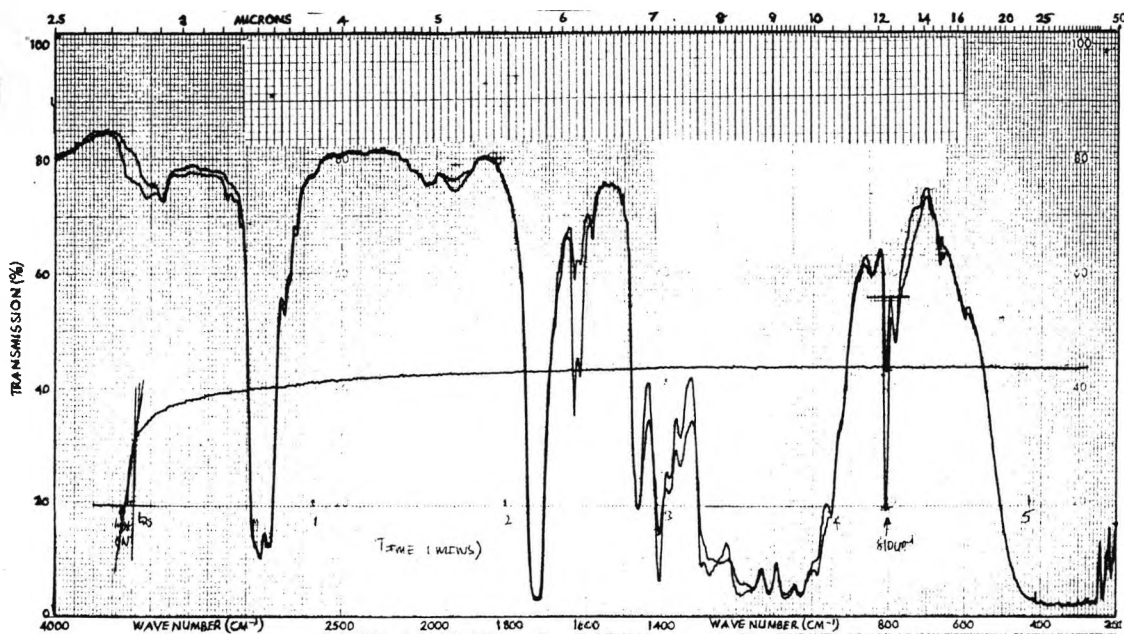
Spectrum 2:- RTIR spectrum, showing the polymerization of ZL1866 in the presence of Irgacure 907 under aerobic conditions.
