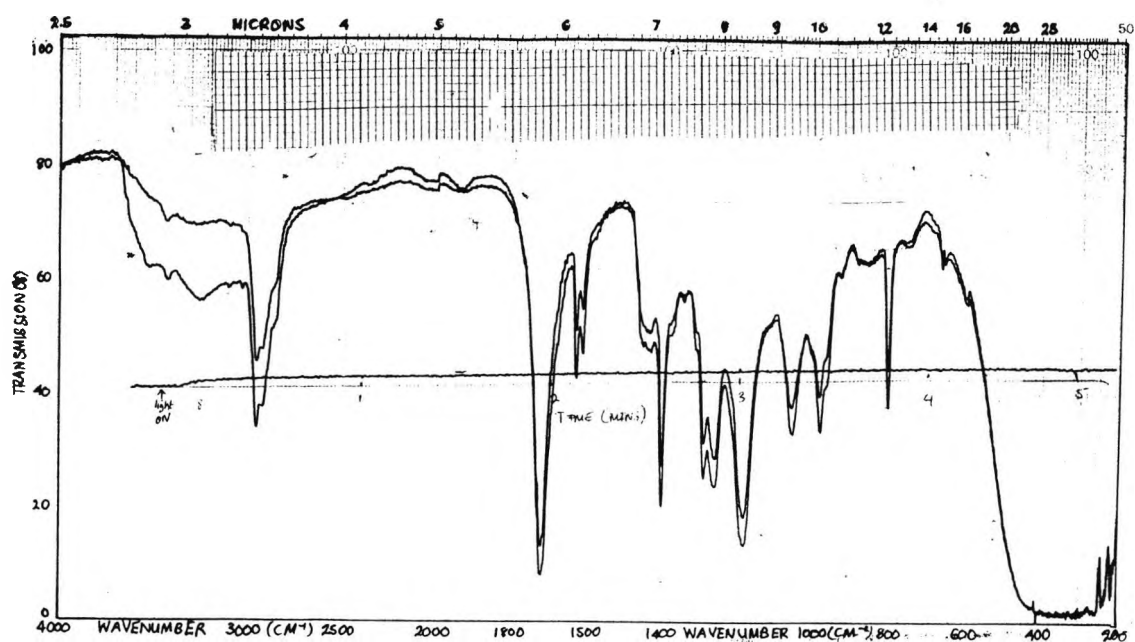
Spectrum 6:- RTIR spectrum showing the polymerization of 2,2-thiodiethyl diacrylate in the presence of Irgacure 907, under aerobic conditions.
