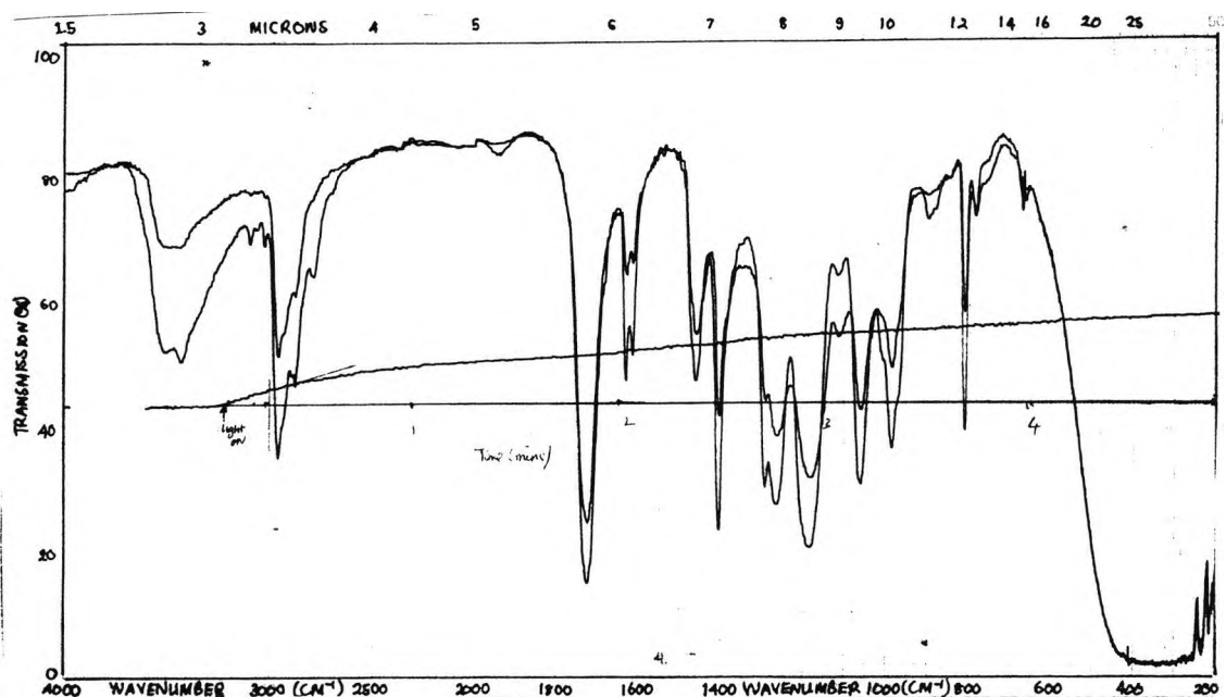
Spectrum 1:- RTIR spectrum, showing the polymerization of 2-ethyl-2(hydroxymethyl)-1,3-propanediol triacrylate in the presence of n^6 -dichlorobenzene- n^5 -cyclopentadienyliron(II)- n -butyltriphenylborate and N -methyldiethanolamine, under anaerobic conditions.
