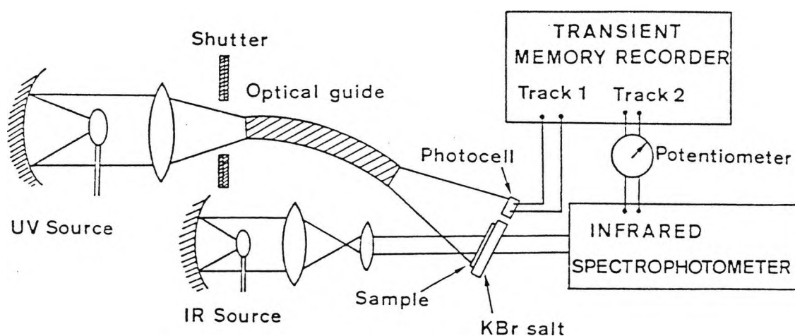
Fig. 2.1 Experimental device for real-time monitoring of uv curing reactions.
