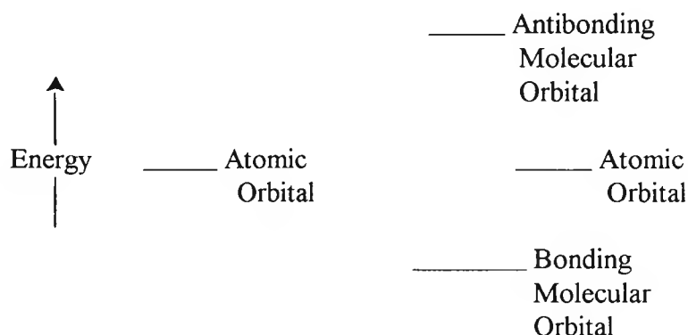
Fig 1.4:- Effect on orbital energy of a linear combination of atomic orbitals.
