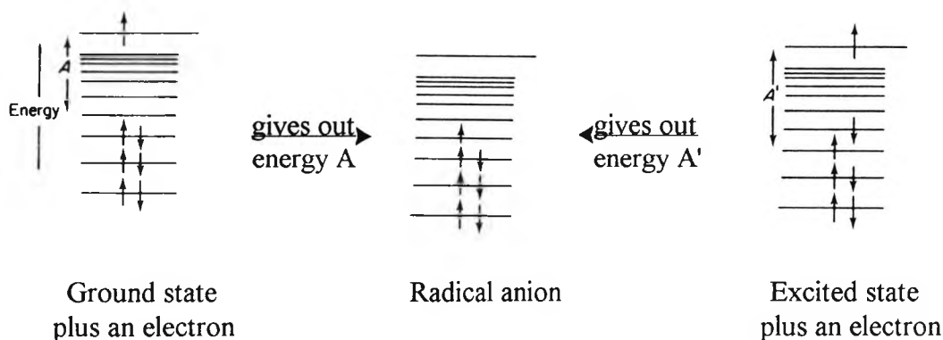
Fig 1.3:- Diagrammatic rationalization of the better electron-acceptor properties of an excited state.
