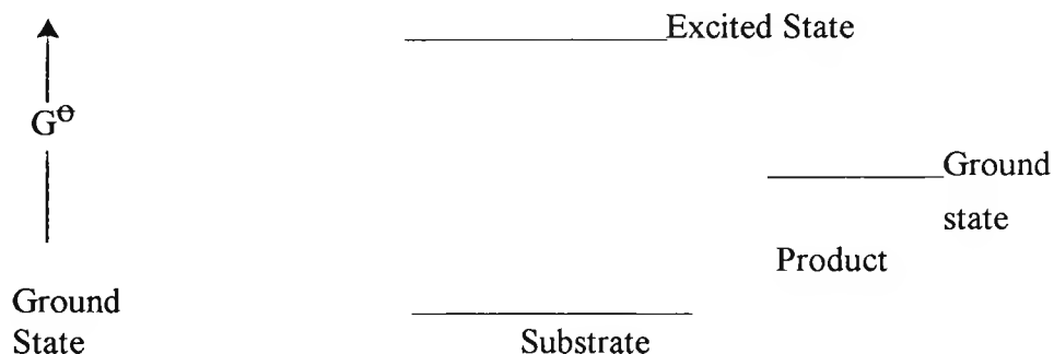
Figure 1.1 :- is a standard free-energy diagram showing the ground state of a molecule, an excited state of the same molecule and a potential product of a chemical reaction.
