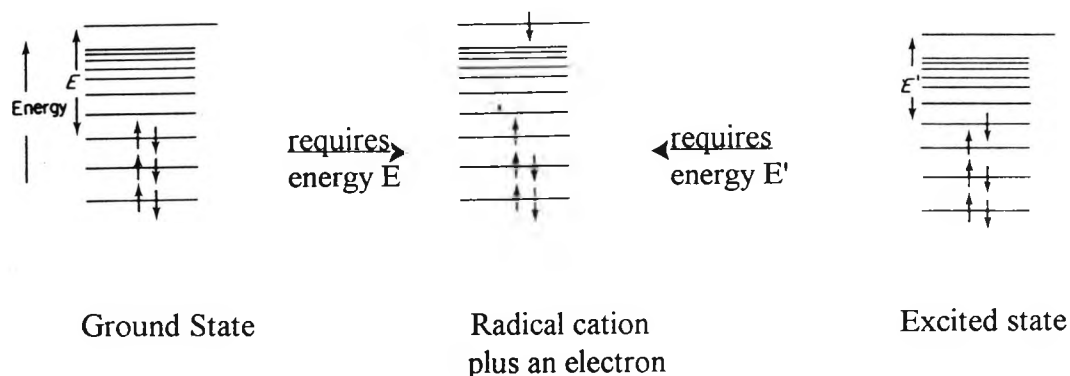
Fig 1.2:- Diagrammatic rationalization of the better electron-donor properties of an excited state.
