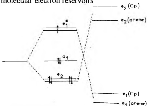
Fig. 1. - Molecular - orbital diagram for transition metal sandwiches d^7 , 19 electron \text{CpFe(I)(arene)} complex
