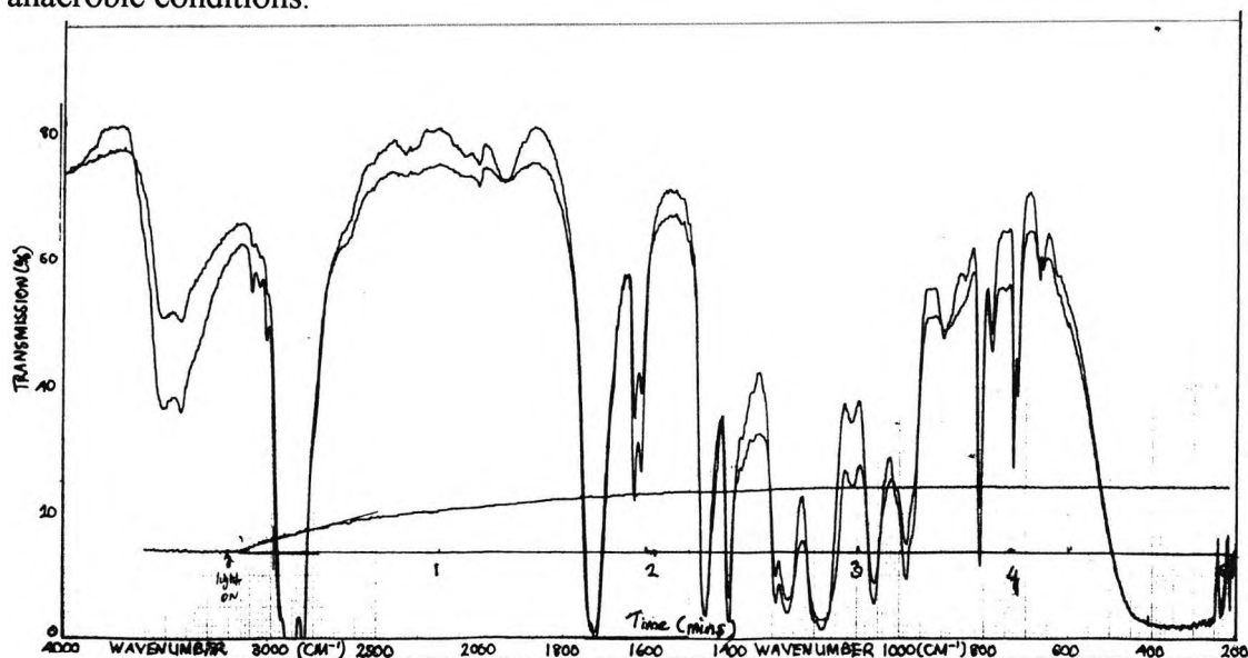
Spectrum 2:- RTIR spectrum, showing the polymerization of 2-ethyl-2(hydroxymethyl)-1,3-propanediol triacrylate in the presence of n^6 -dichlorobenzene- n^5 -cyclopentadienyliron(II)- n -butyltriphenylborate and N -methyldiethanolamine, under aerobic conditions.
