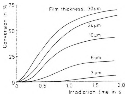
Fig 2.3 Effect of film thickness on the photopolymerization profiles recorded by RTIR spectroscopy for a polyurethane-acrylate.
