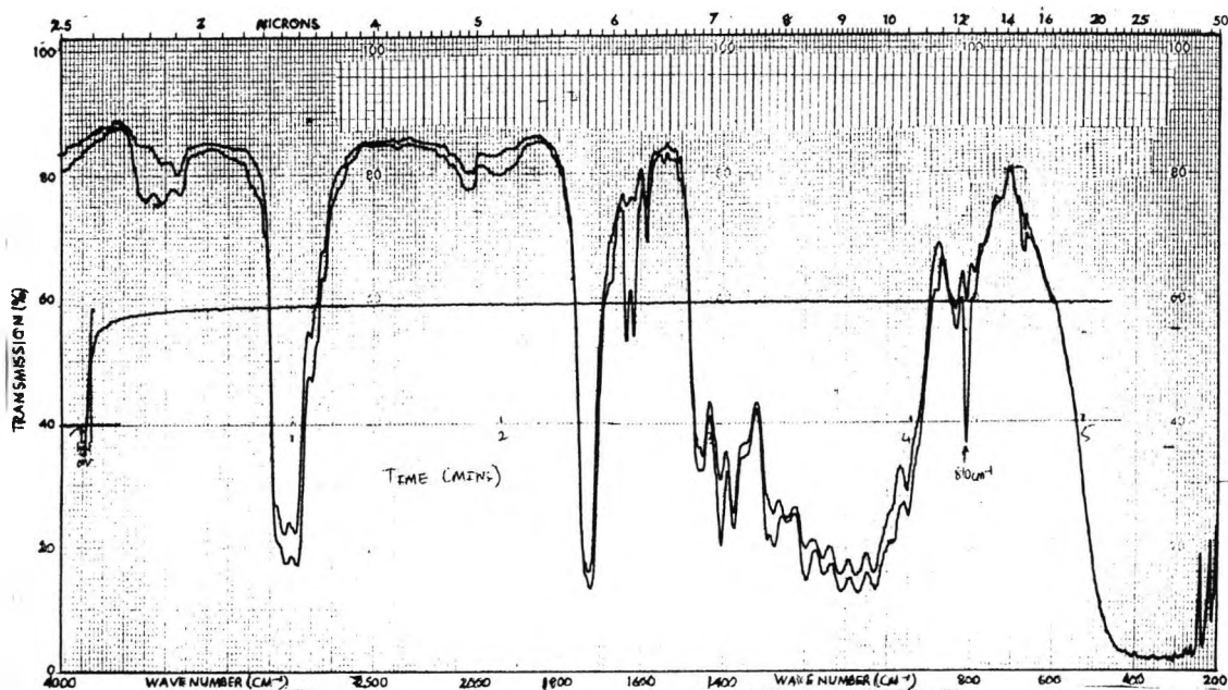
Spectrum 1:- RTIR spectrum, showing the polymerization of ZL2244 in the presence of Irgacure 907 under aerobic conditions.
