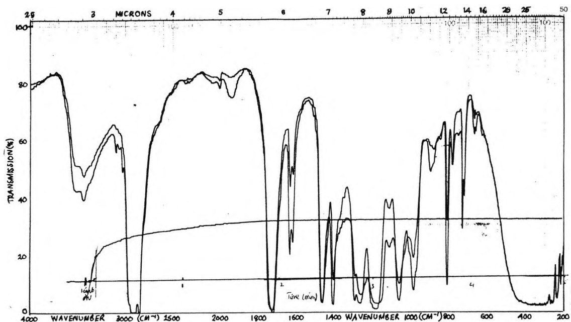
Spectrum 1: RTIR spectrum, showing the polymerization of 2-ethyl-2(hydroxymethyl)-1,3-propanediol triacrylate in the presence of an amine and pyrenediazonium tetrafluoroborate, under anaerobic conditions.
