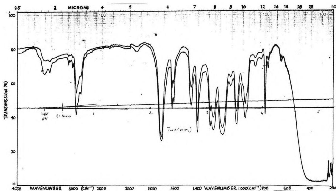
Spectrum 3:- RTIR spectrum, showing the polymerization of 2-ethyl-2(hydroxymethyl)-1,3-propanediol triacrylate in the presence of n^6 -dichlorobenzene- n^5 -cyclopentadienyliron(II)- n -butyltriphenylborate, under anaerobic conditions.
