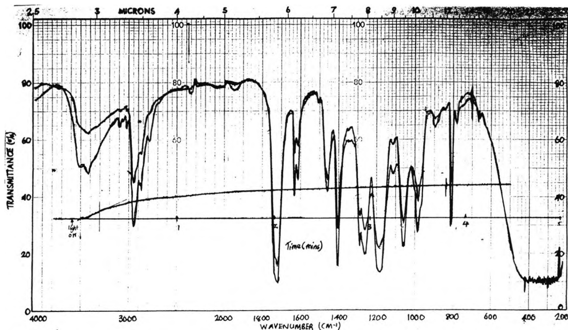
Spectrum 6: RTIR spectrum, showing the polymerization of 2-ethyl-2(hydroxymethyl)-1,3-propanediol triacrylate in the presence of 2,3-bis(4-methoxyphenyl) quinoxaline and N-methyldiethanolamine, under aerobic conditions.
