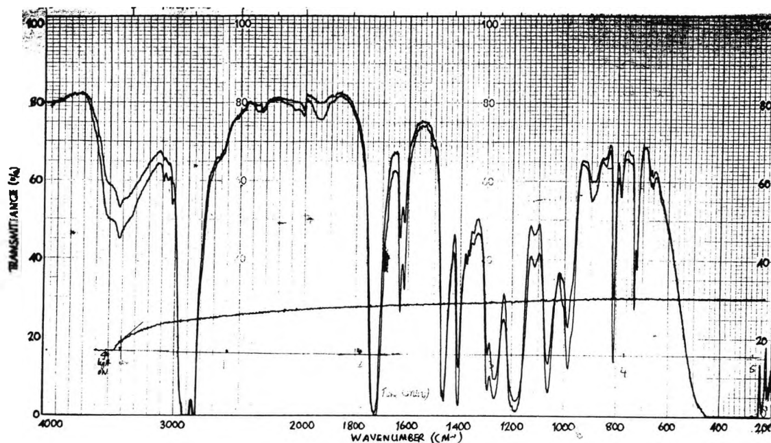
Spectrum 3: RTIR spectrum showing the polymerization of 2-ethyl-2(hydroxymethyl)-1,3-propanediol triacrylate in the presence of 7-benzoyl-2,3-bis(4-hydroxyphenyl)-quinoxaline and N-methyldiethanolamine, under anaerobic conditions.
