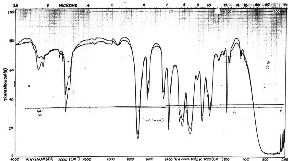
Spectrum 4:- RTIR spectrum showing the polymerization of 2-ethyl-2(hydroxymethyl)-1,3-propanediol triacrylate in the presence of pyrenediazonium tetrafluoroborate, under aerobic conditions.
