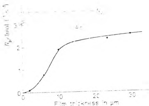
Fig. 2.4 Dependence of the rate of polymerization R_p on the film thickness.
