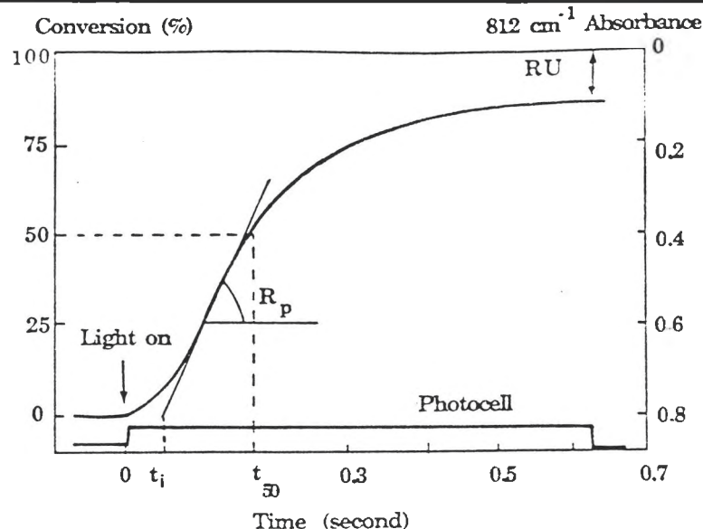
Figure 2.2 Typical cure profile recorded by RTIR spectroscopy for an acrylic coating exposed to u.v. radiation.
