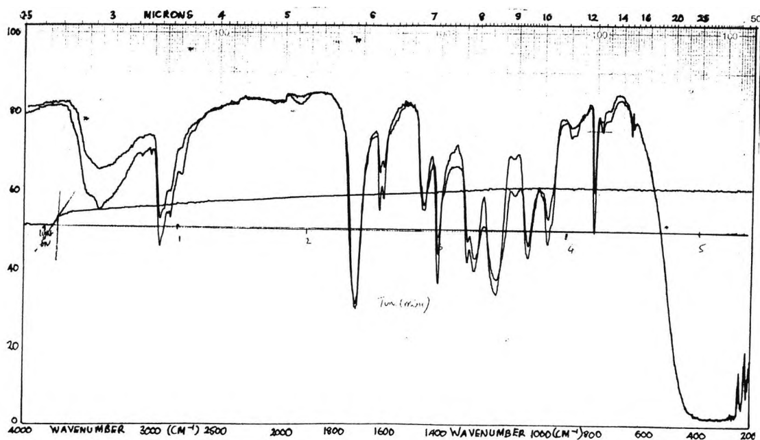
Spectrum 2:- RTIR spectrum, showing the polymerization of 2-ethyl-2(hydroxymethyl)-1,3-propanediol triacrylate in the presence of an amine and pyrenediazonium tetrafluoroborate, under aerobic conditions.
