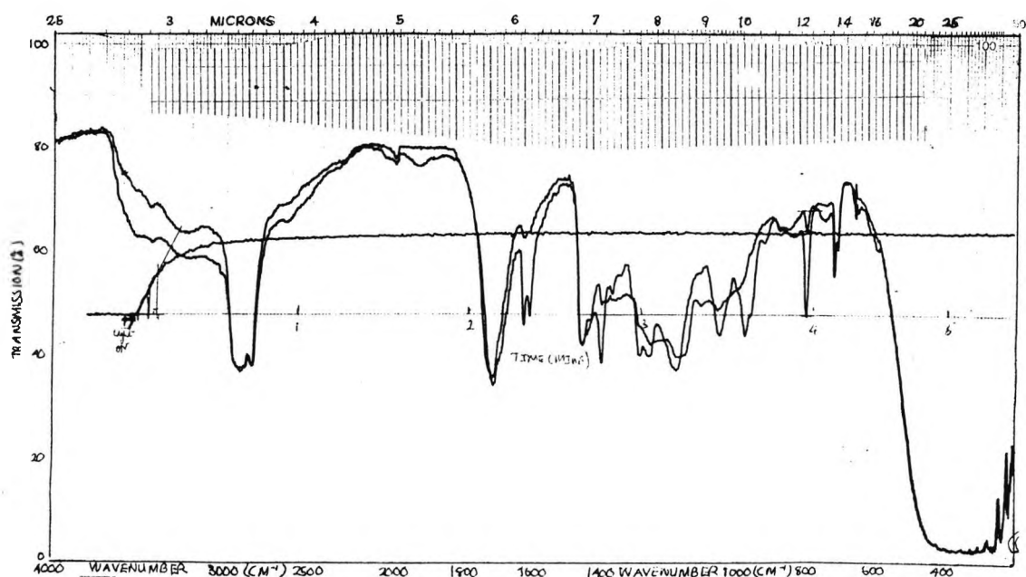
Spectrum 5:- RTIR spectrum showing the polymerization of 2,2-thiodiethyl diacrylate in the presence of Irgacure 907, under anaerobic conditions.
