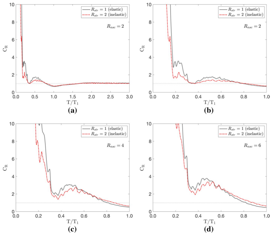
Fig. 10 Mean inelastic displacement ratios at roof level as a function of T/T_1 for different levels of lateral strength; Considering Set C subjected to NF: a R_{nsc}=2 , b R_{nsc}=2 , c R_{nsc}=4 , and d R_{nsc}=6
