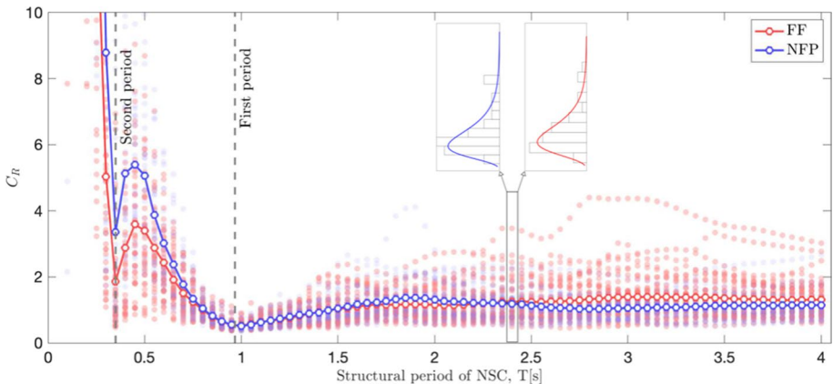
Fig. 15 Representative full C_R response versus T of the NSC components on the roof of a given building. Solid-dotted lines correspond to mean C_R values for a given period T , whose sample distributions are schematically shown for an arbitrarily selected period of 2.4 s
