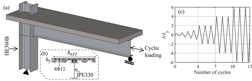
Fig. 3. Schematic test details of CS1 [47]: a) test configuration, b) composite beam cross-section, and c) applied loading history.
