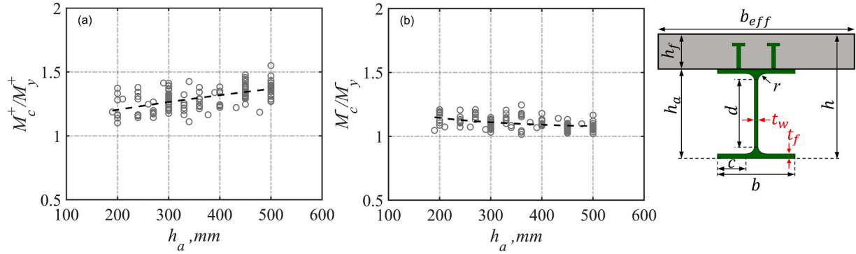
Fig. 25. Ratio of ultimate strength of composite beam to its yield strength for: a) positive and b) negative bending.
