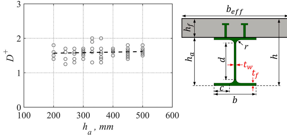
Fig. 22. Rate of cyclic degradation vs steel beam depth.
