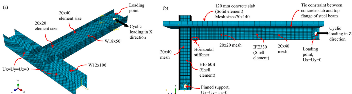
Fig. 7. Examples of continuum models: a) BS1 and b) CS1.
