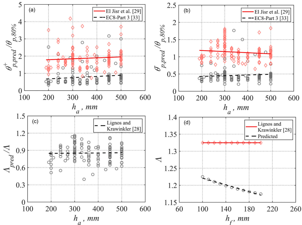
Fig. 28. Comparison of plastic rotation and cyclic deterioration parameter vs steel beam depth: a) \theta_p^+ , b) \theta_p^- , c) \Lambda , as well as d) cyclic deterioration parameter for IPE300 vs slab thickness.
