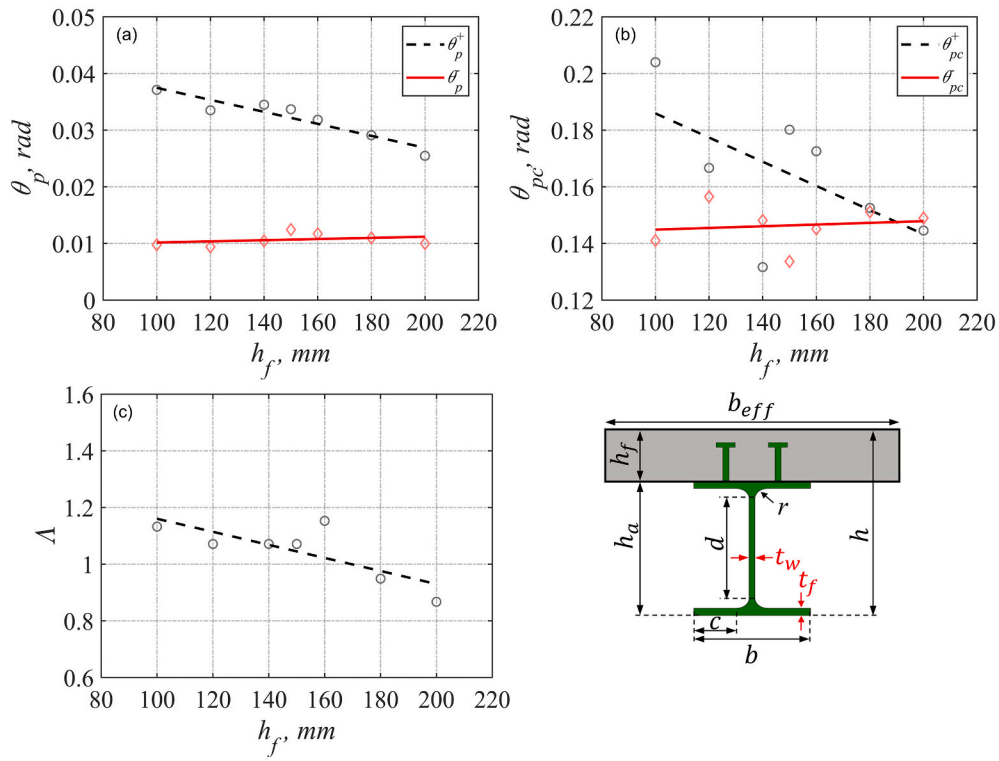
Fig. 20. Dependency of modelling parameters on slab thickness, h_f for IPE500: a) \theta_p , b) \theta_{pc} , c) \Lambda .
