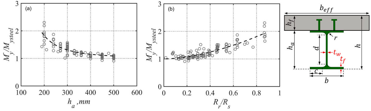
Fig. 24. Ratio of yield strength of composite beam to that of steel beam under negative bending vs: a) h_a and b) R_r/R_s .
