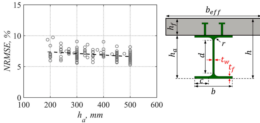
Fig. 16. Normalised root-mean-square error (NRMSE) versus steel section depth ( h_a ).
