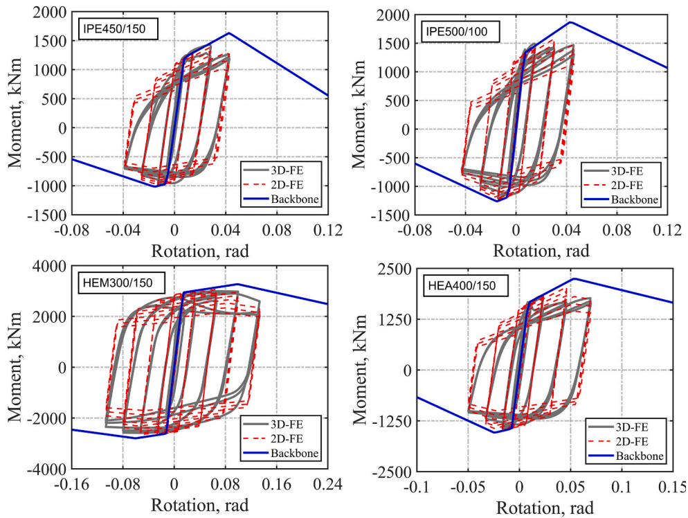
Fig. 17. Examples of IMK model calibration (initial backbone curve from 2D-FE model).
