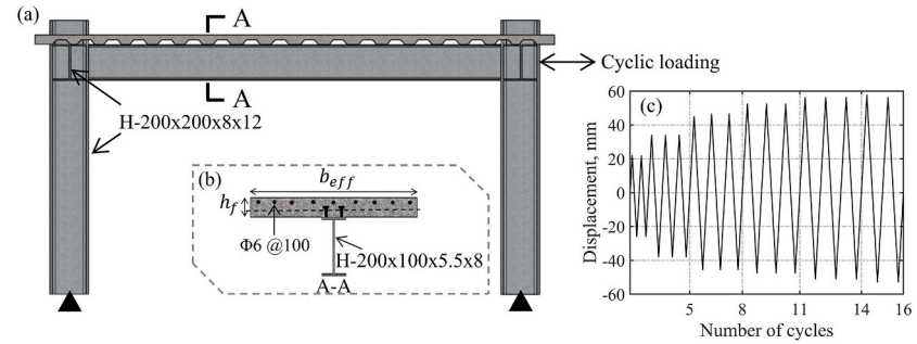
Fig. 5. Schematic test details of CS3 [49]: a) test configuration, b) composite beam cross-section, and c) applied loading history.
