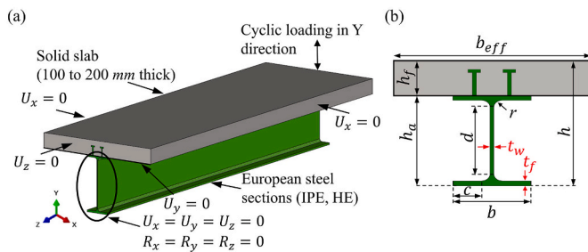
Fig. 13. Schematic view of parametric investigation: a) typical composite specimen and b) cross-section.
