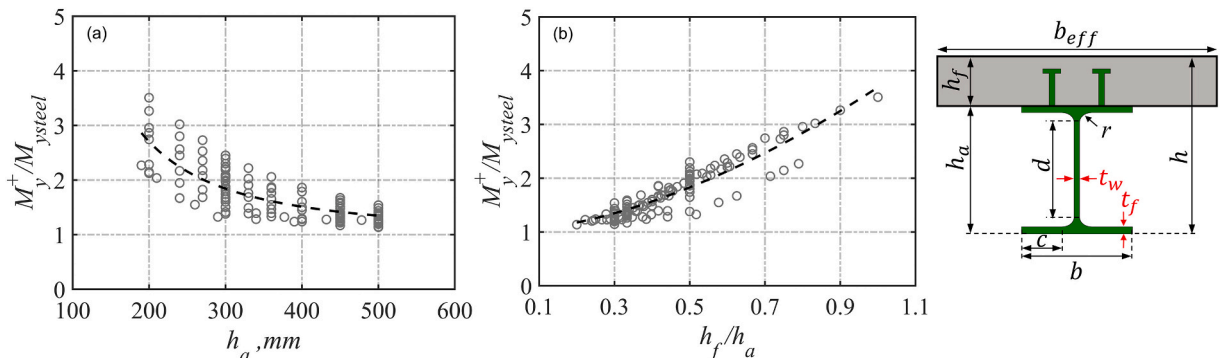
Fig. 23. Ratio of yield strength of composite beam to that of steel beam under positive bending vs: a) h_a and b) h_f/h_a .
