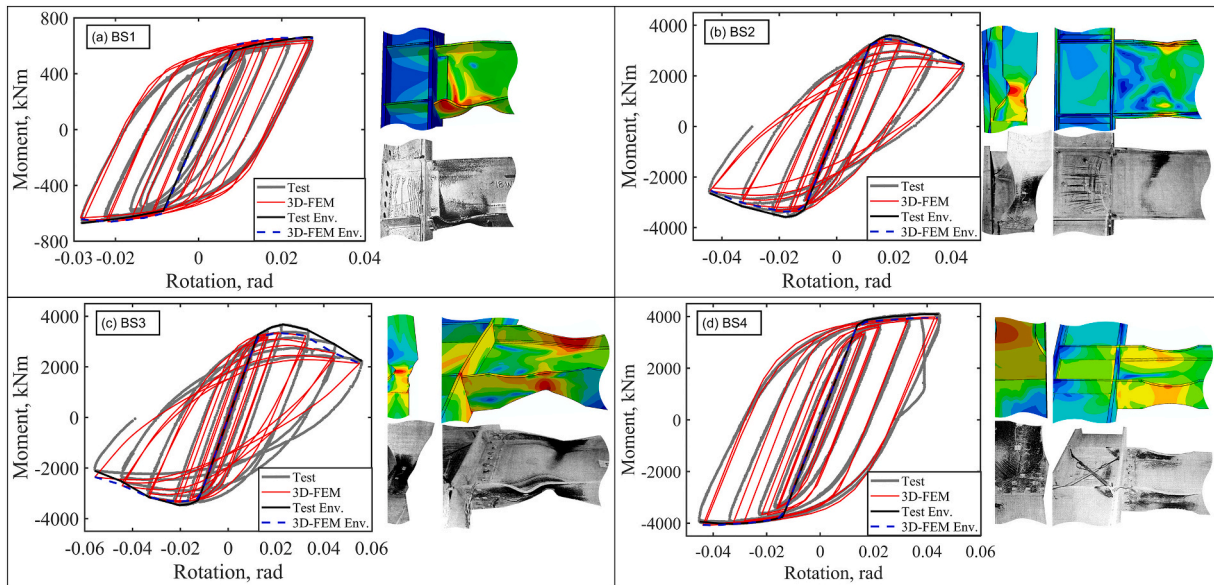
Fig. 10. Comparison between experimental and numerical results for (a) BS1, (b) BS2, (c) BS3, and (d) BS4.
