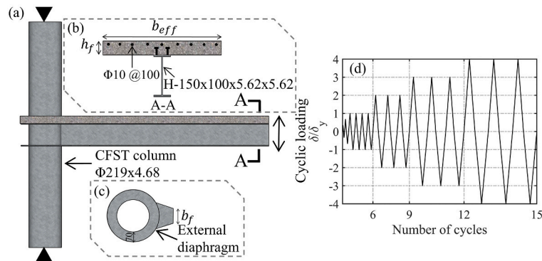
Fig. 6. Schematic test details of CS4 [50]: a) test configuration, b) composite beam cross-section, c) connection details, and d) applied loading history.
