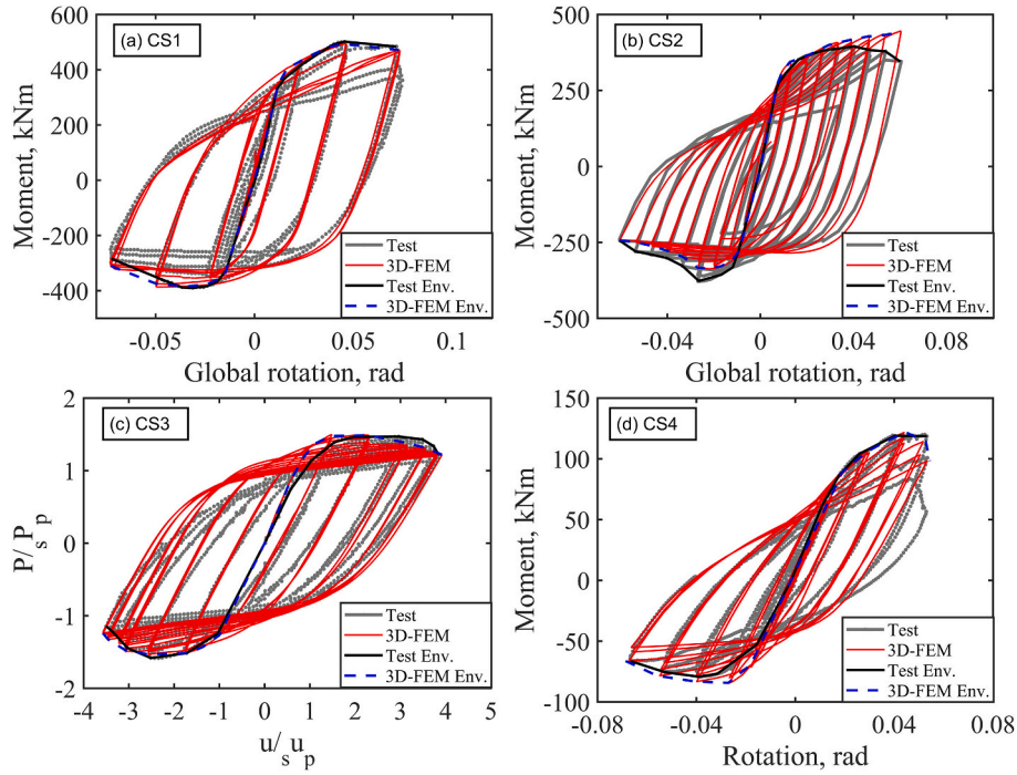
Fig. 11. Comparison between experimental and numerical results for: (a) CS1, (b) CS2, (c) CS3, (d) CS4.
