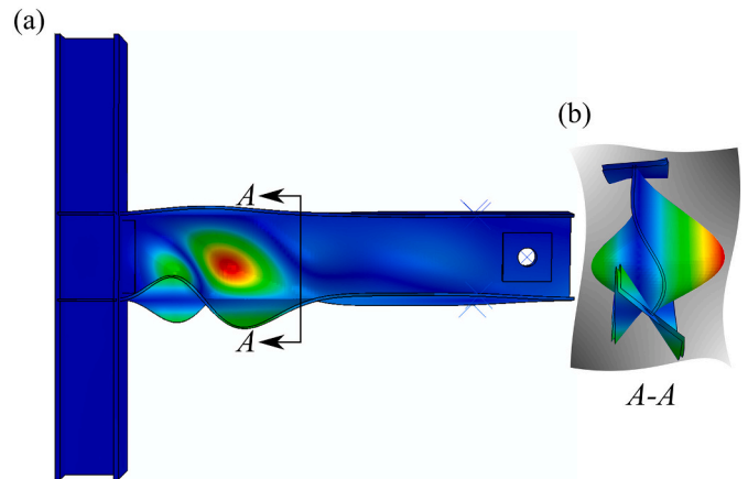
Fig. 8. Example of critical buckling mode for BS1: a) side view and b) cross-section.
