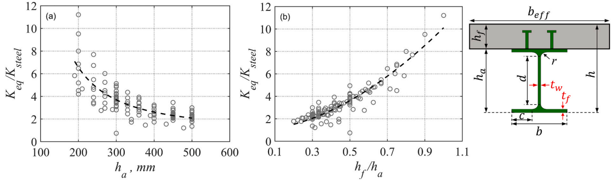
Fig. 26. Equivalent initial stiffness of composite members normalised by that of bare steel beams vs: a) h_a and b) h_f/h_a .
