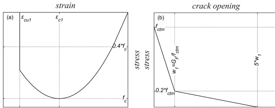
Fig. 9. Material model for concrete: (a) compression and (b) tension.
