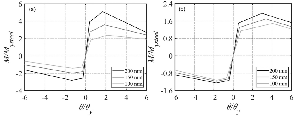
Fig. 27. Examples of backbone curves for various slab thicknesses, h_f , (as 200 mm, 150 mm, and 100 mm) plotted via proposed formulations: a) IPE200, and b) IPE500.
