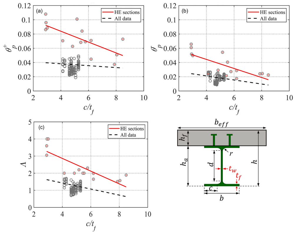
Fig. 19. Dependency of modelling parameters on flange slenderness, c/t_f : a) \theta_p^+ , b) \theta_p^- , c) \Lambda .
