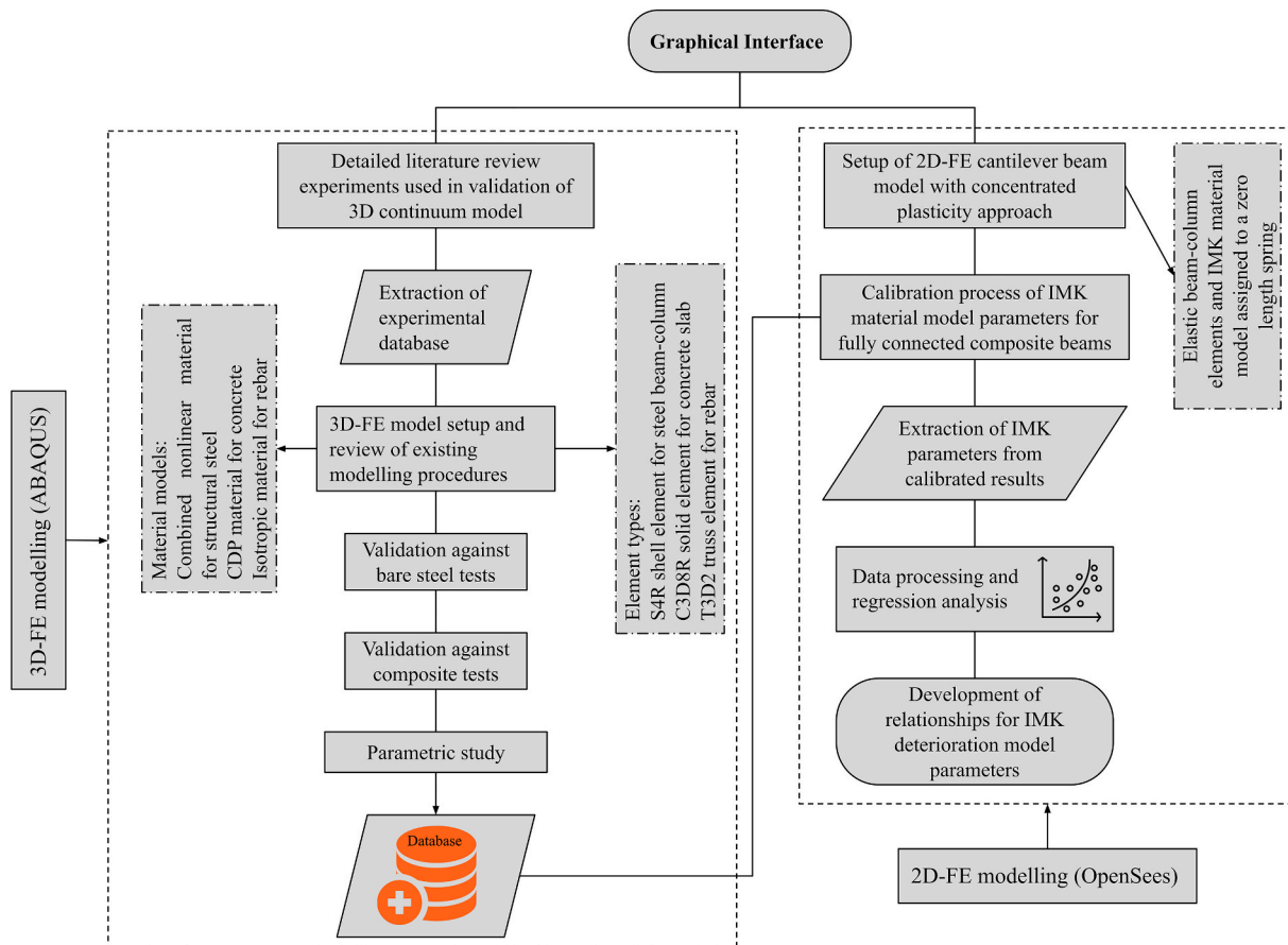
Fig. 1. Flowchart of the methodology used in this study.
