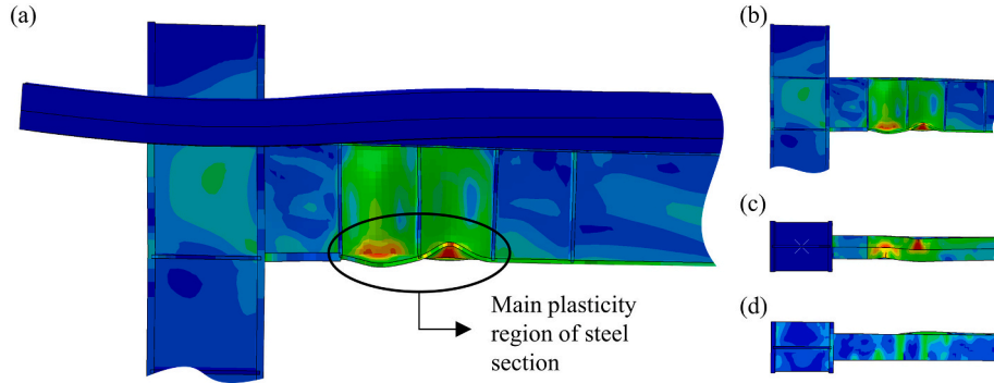
Fig. 12. Deformed shape from the analysis for Specimen CS1: a) side view of composite member, b) side view of steel component, c) bottom view of steel component, and d) top view of steel part.
