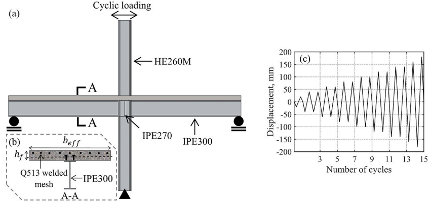
Fig. 4. Schematic test details of CS2 [48]: a) test configuration, b) composite beam cross-section, and c) applied loading history.
