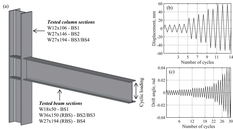
Fig. 2. Schematic test details of bare steel experimental specimens: a) typical test configuration and applied loading histories: b) BS1 [44], and c) BS2 to BS4 [45].
