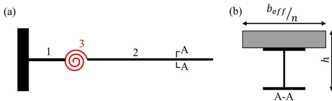
Fig. 15. 2D-FE lumped plasticity model: a) typical 2D composite specimen and b) cross-section - Elements 1 and 2: elastic beam-column; Element 3: rotational spring.
