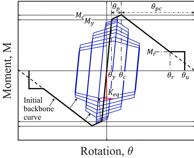
Fig. 14. Modified IMK cyclic degradation model and initial backbone curve.
