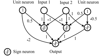
Fig. 3. Extended equality module
