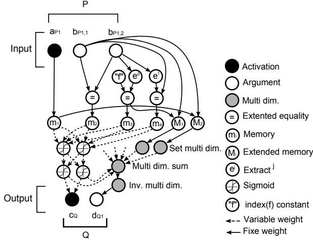
Fig. 6. Illustration of the PAN
