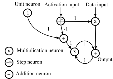
Fig. 4. Extended memory module
