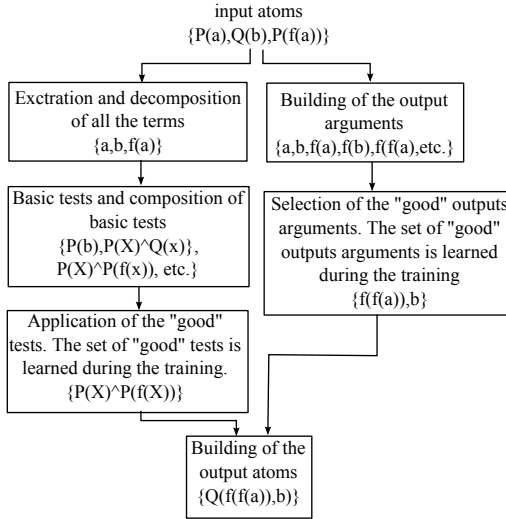
Fig. 2. Run of PAN after learning the rule P(X) \wedge P(f(X)) \Rightarrow Q(f(f(X)))
