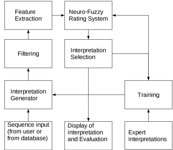
Figure 2: Modules of the ISSM.
