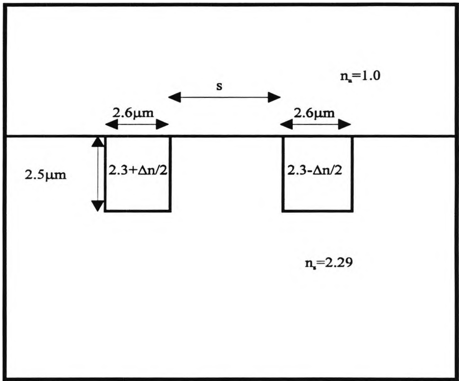
Fig. 9.1 Schematic diagram of channel waveguides directional coupler.
