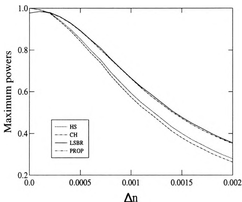
Fig. 6.10 Maximum power transfer between two coupled waveguides.
