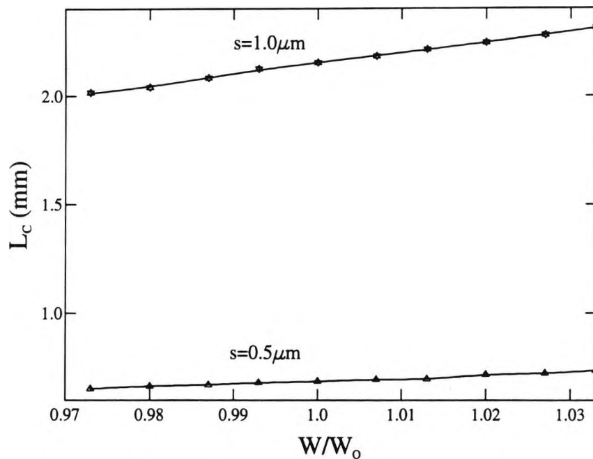
Fig. 8.9 Variation of the coupling length with W/W_o for different half-separation distances.
