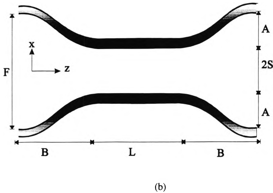
Fig. 8.13 Input and output sections of directional couplers (a) straight line approach (b) curved S shaped approach.
