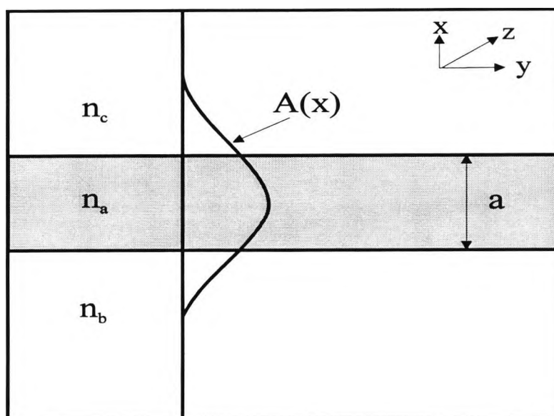
Fig. 1.2 Schematic of a slab waveguide, showing waveguide of thickness a , and refractive index n_a confined by two semi-infinitely thick layers of refractive indices n_c and n_b supporting a TE mode.
