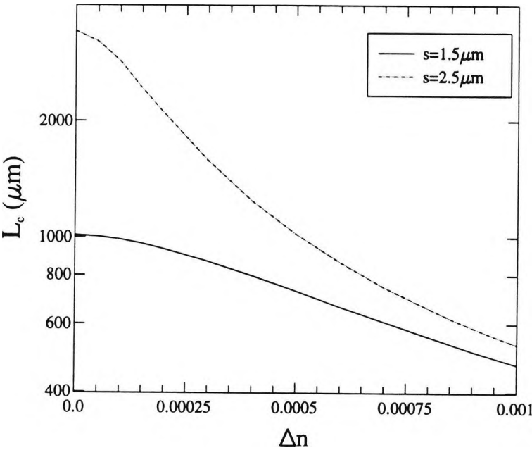
Fig. 9.7 Variation of the coupling length with \Delta n for different separation distances, s .
