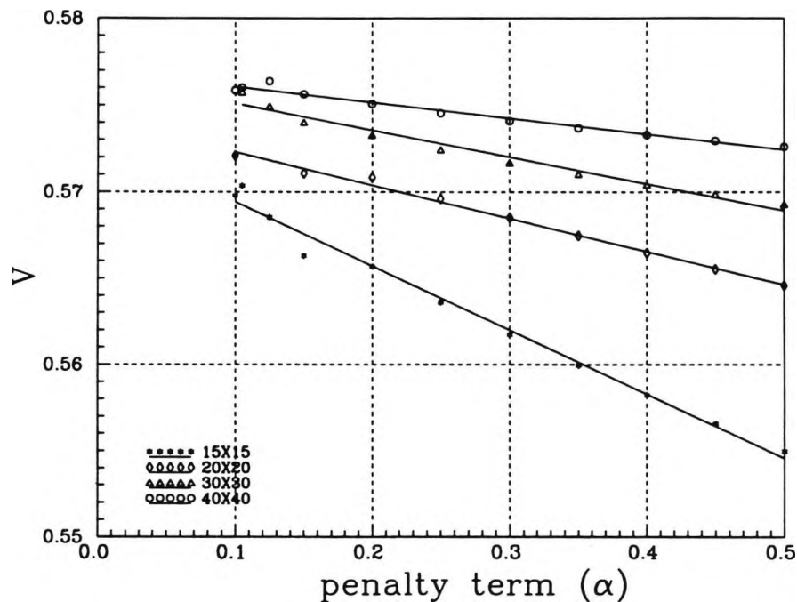
Fig. 8.4 Effect of the penalty parameter for the H_{11}^y mode with mesh division.
