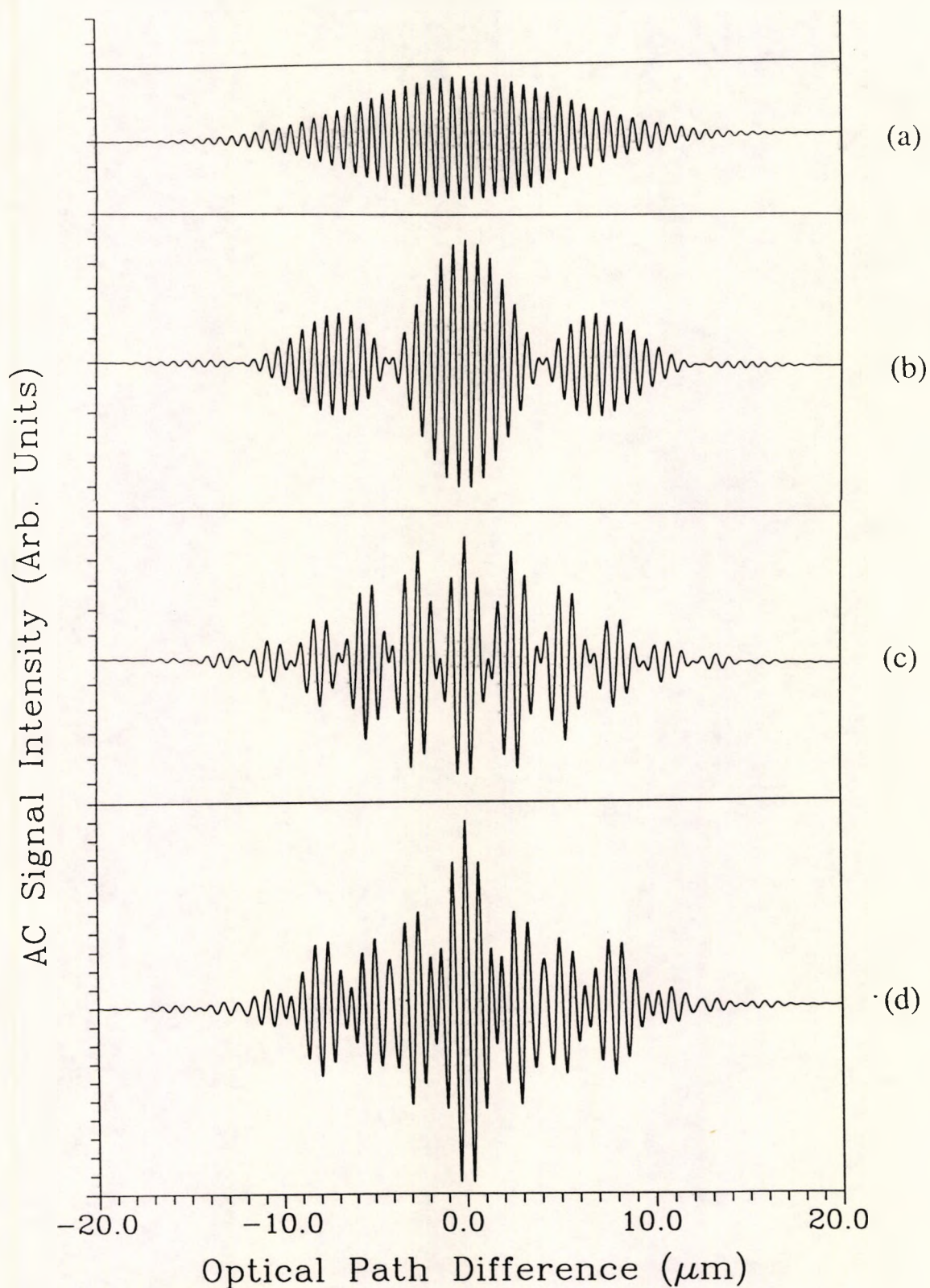
Fig.4.2 Computer Simulated Interference Fringe Patterns
