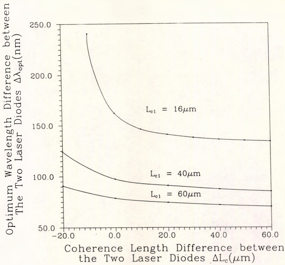
Fig.3.8 The Optimum Wavelength Difference for two Laser Diodes with Different Coherence Lengths \Delta L_c = L_{c2} - L_{c1} ( \lambda_1 = 635nm )
