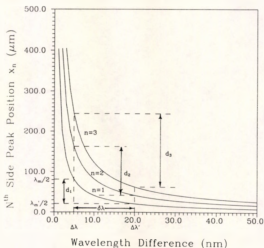
Fig.6.3 The Variation of the N^{\text{th}} Side Packet Peak Position with the Initial Wavelength Difference, \Delta\lambda
