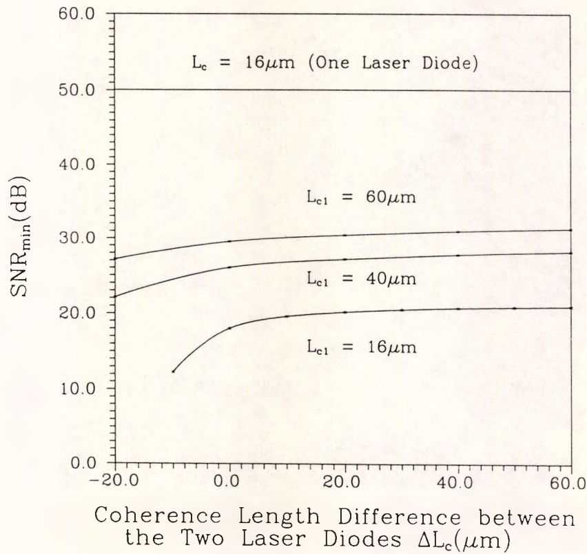
Fig.3.9 The SNR_{min} for two Laser Diodes with Different Coherence Lengths \Delta L_c = L_{c2} - L_{c1} ( \lambda_1 = 635nm )
