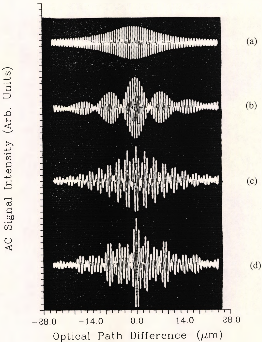
Fig.4.10 Experimentally Obtained Interference Fringe Patterns
