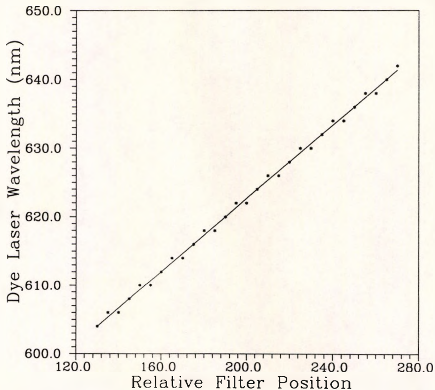
Fig.6.6 Dye Laser Wavelength Versus The Filter Calibration
