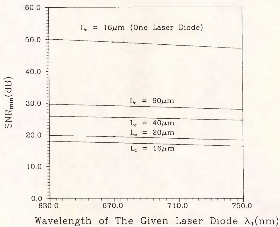
Fig. 3.7 The SNR_{min} at Optimum Wavelength Combinations
