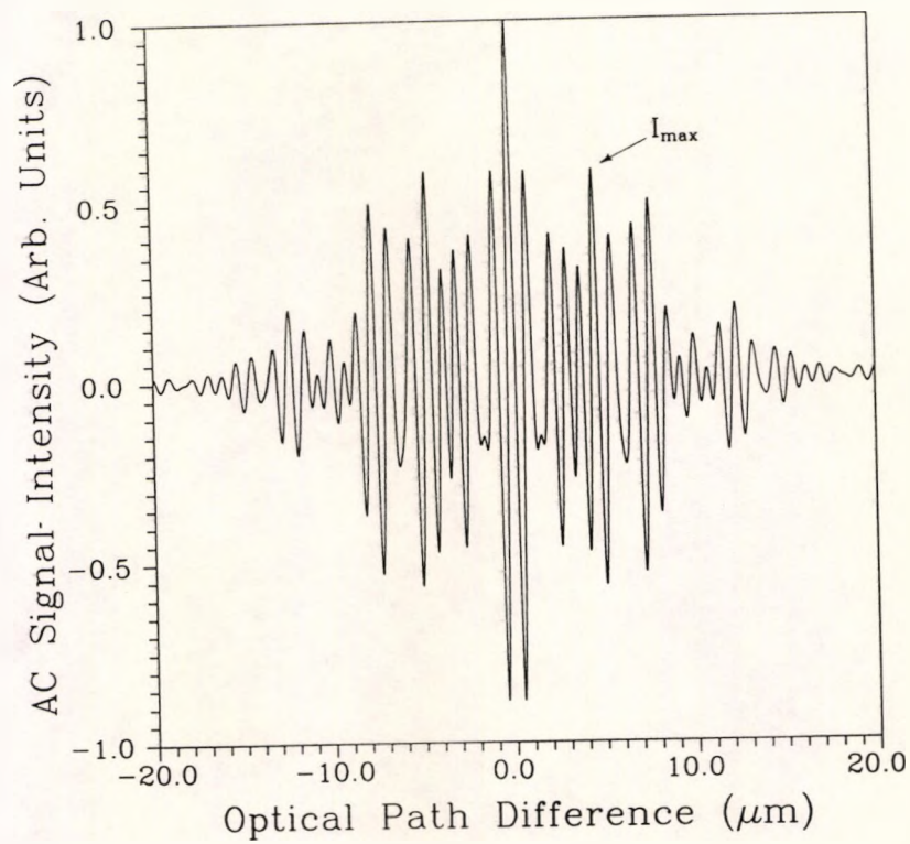
(a) \lambda = 770\text{nm} , L_c = 20\mu\text{m} , a_{\text{opt}} = 1.24 , b_{\text{opt}} = 1.45
