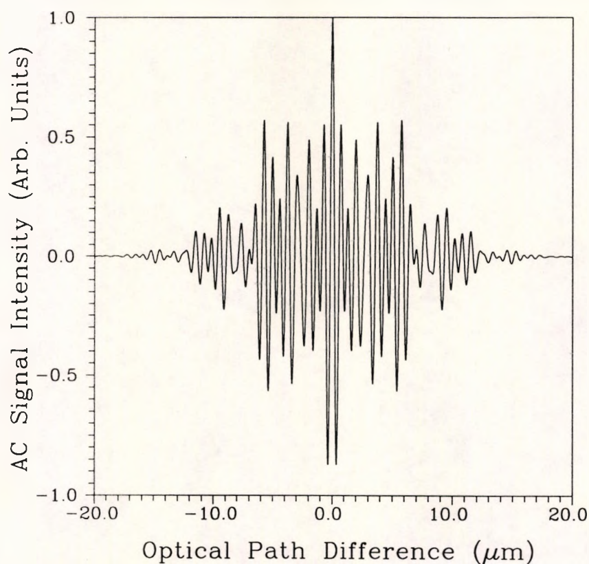
(b) \lambda_1 = 635\text{nm} , \lambda_2 = 724\text{nm} , \lambda_3 = 959\text{nm} , L_c = 16\mu\text{m}
