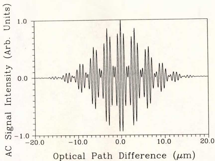
(a) \lambda_1 = 635\text{nm} , \lambda_2 = 797\text{nm} , L_c = 16\mu\text{m}
