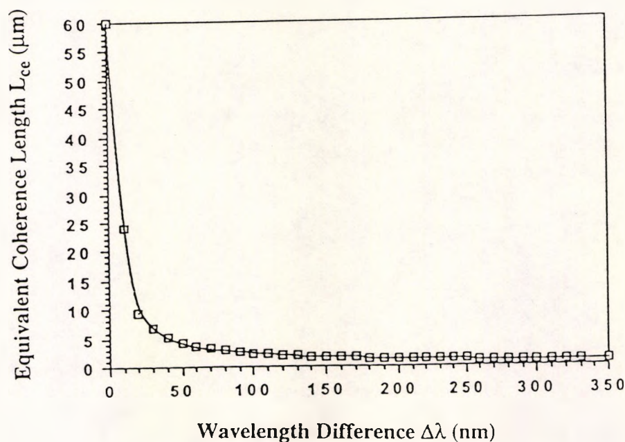
Fig.3.10 The Variation of Equivalent Coherence Length, L_{ce} , with Wavelength Difference
