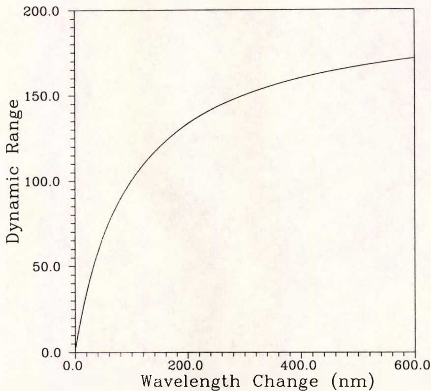
Fig.6.4 The Variation of the Dynamic Range with the Initial Wavelength Difference, \Delta\lambda ( \delta\lambda_{\max} = 100\text{nm} and \delta\lambda_{\min} = 0.5\text{nm} )
