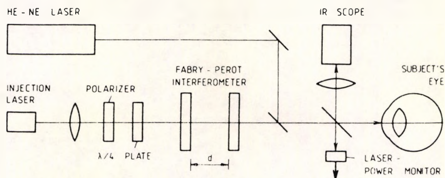
Fig.7.4 Optics of the Interferometer Used to Measure the Length of the Optic Axis of the Human Eye In Vivo , after Fercher et al [8]
