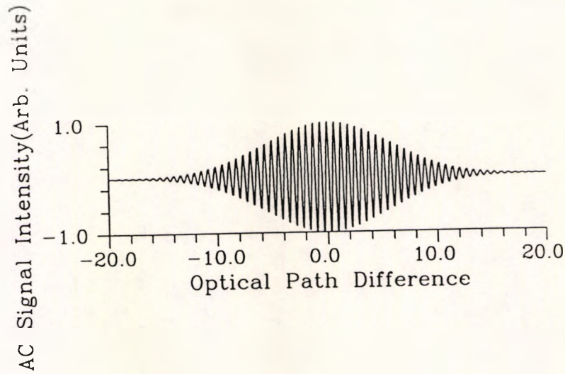
Fig.3.1 Interference Fringe Pattern for One Multimode Laser
