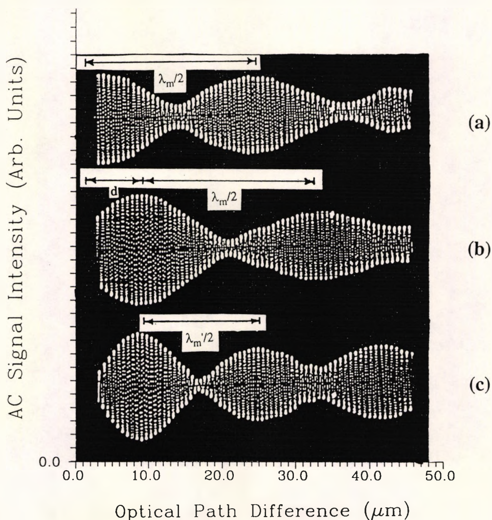
Fig.6.7 Experimentally obtained Interference Fringe Patterns
