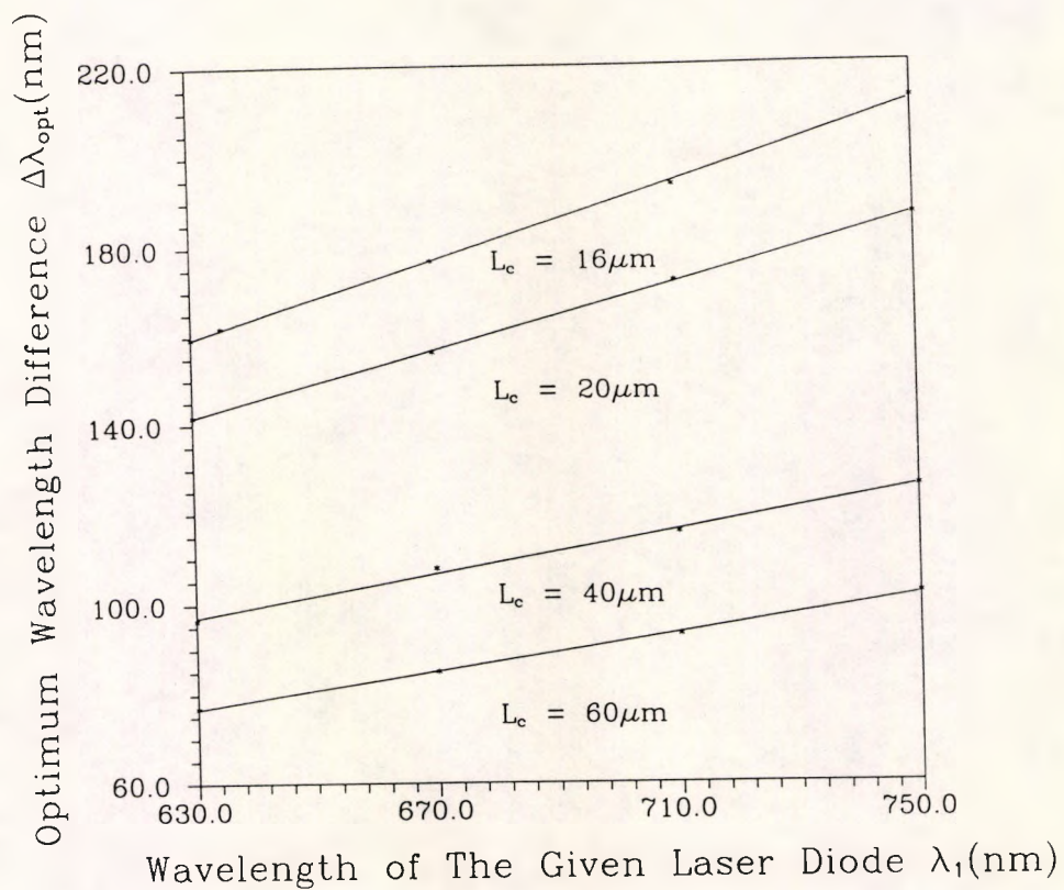
Fig. 3.6 The Optimum Wavelength Difference for a Given Wavelength
