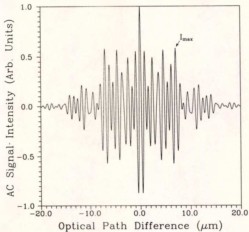
(b) \lambda = 780\text{nm} , L_c = 20\mu\text{m} , a_{\text{opt}} = 1.14 , b_{\text{opt}} = 1.51
