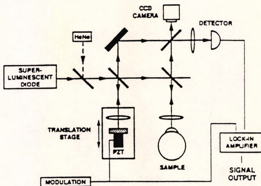
Fig.7.3 Schematic of Optical Coherence Domain Reflectometer Setup for Ranging Experiments, after Huang et al [17]
