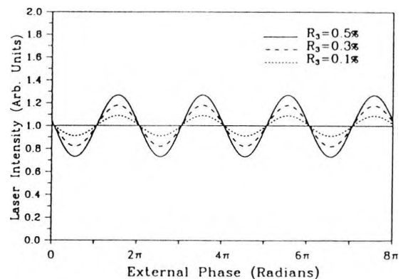
Fig. 12. Power-modulation dependence on external phase and reflectivity in self-mixing interference obtained from a theoretical model.
