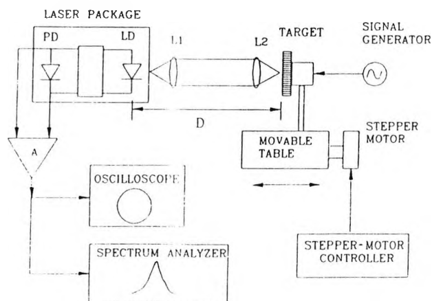
Fig. 1 Schematic experimental arrangement: PD, photodiode (integral); LD, laser diode; A, amplifier; D, distance; L1, L2, lenses.
