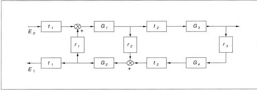
Figure 4.2 Block diagram of self-mixing feedback system
