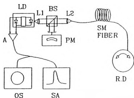
Fig. 2. Experimental arrangement for self-mixing LDV. LD, laser diode; BS, beam splitter; L_1 , L_2 , lenses; OS, oscilloscope; SA, spectrum analyzer; A, amplifier; PM, power meter; SM, single mode; RD, rotating disk.
