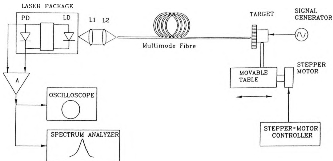
Fig. 5. Schematic experimental arrangement with a long multimode fiber between a laser and target. PD, photodiode; LD, laser diode; L1, L2, lenses; A, amplifier.
