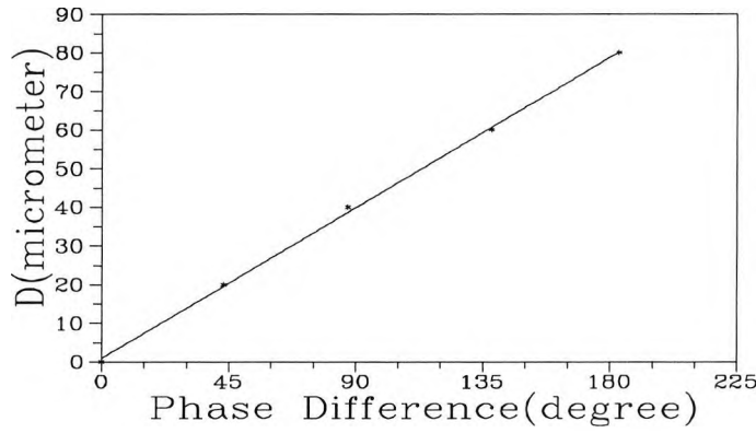
Figure 6.16 Displacement of target mirror dependence on the phase difference, \Delta\phi , of the two output signals of the lasers.
