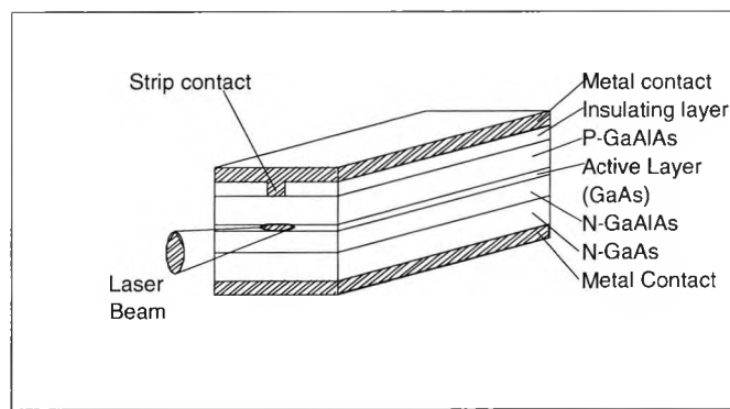
Figure 3.8 A schematic of a stripe-geometry double heterostructure semiconductor laser
