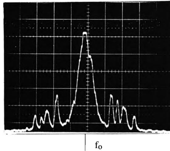
Figure 6.5 Signal spectrum with strong feedback level
