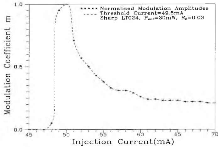
Figure 5.7 Dependence of modulation coefficient on laser injection current
