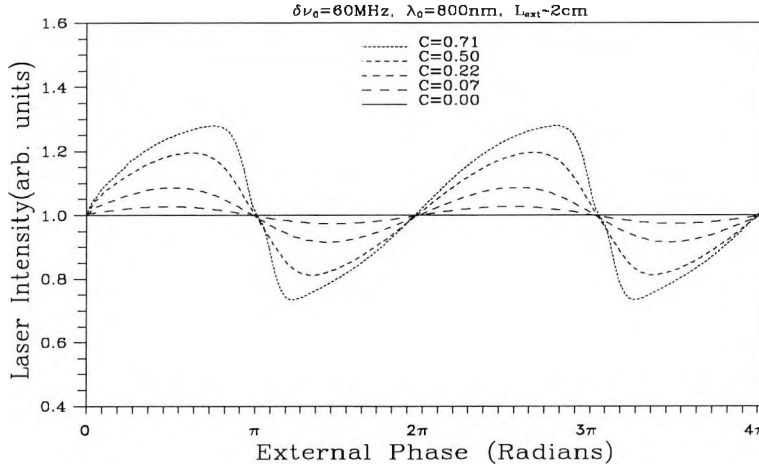
Figure 4.8 Optical intensity versus external phase change
