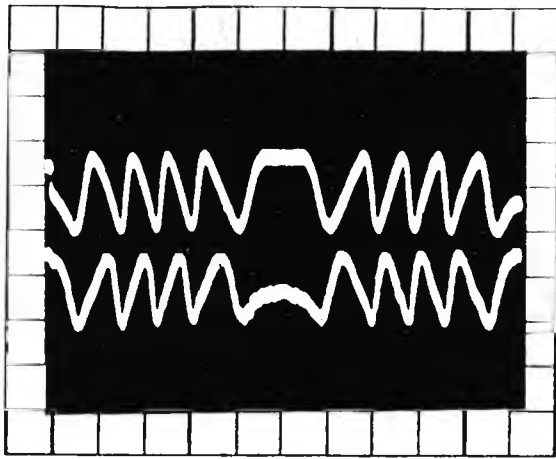
Fig. 10. Self-mixing interference signals observed in two emission directions of a laser.
