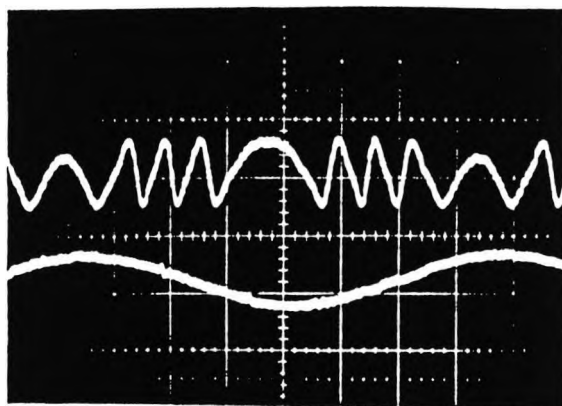
Figure 3: Experimental observation of self-mixing interference
