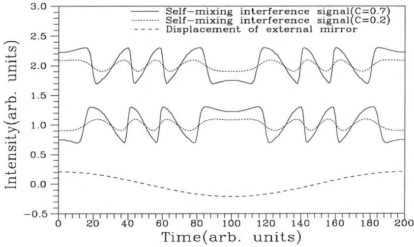
Figure 4.12 Waveform sign inversion of self-mixing interference between two emission directions
