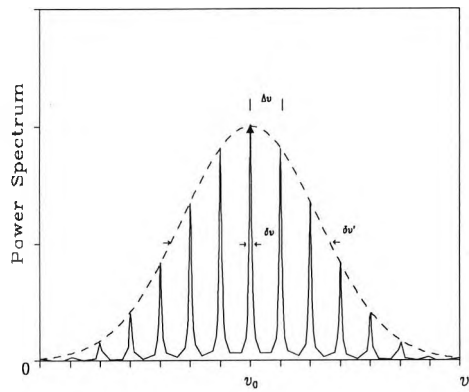
(c1) A multi-mode spectrum
