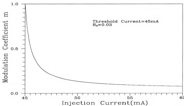
Figure 4.14 Modulation coefficient versus injection current
