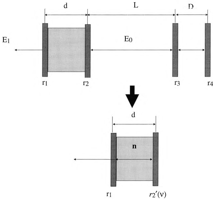
Figure 6.12 Geometry of a four-mirror Fabry-Perot type
