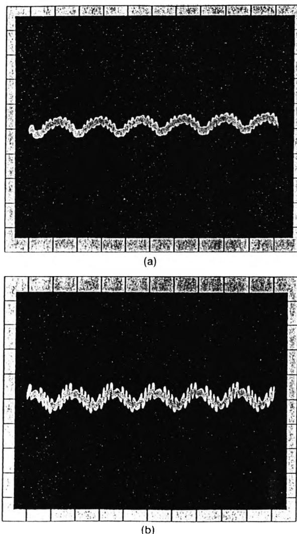
Fig. 6. Current modulation and beat signals (a) without and (b) with mirror reflection (Vertical scale, arbitrary units; horizontal axis, 1.0 ms/division).
