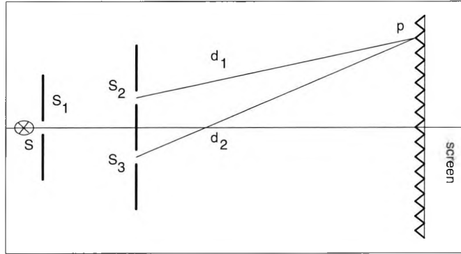
Figure 2.1 Young's experiment of two beam interference
