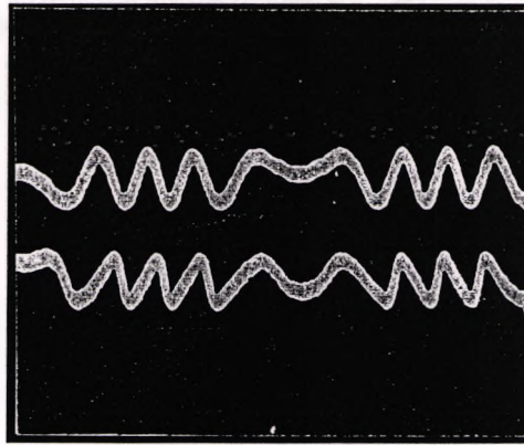
Figure 5.13 Conventional interference pattern(upper trace) compared with self-mixing interference pattern(lower trace) Vertical axis, arbitrary units, horizontal axis, 0.2 ms/division.
