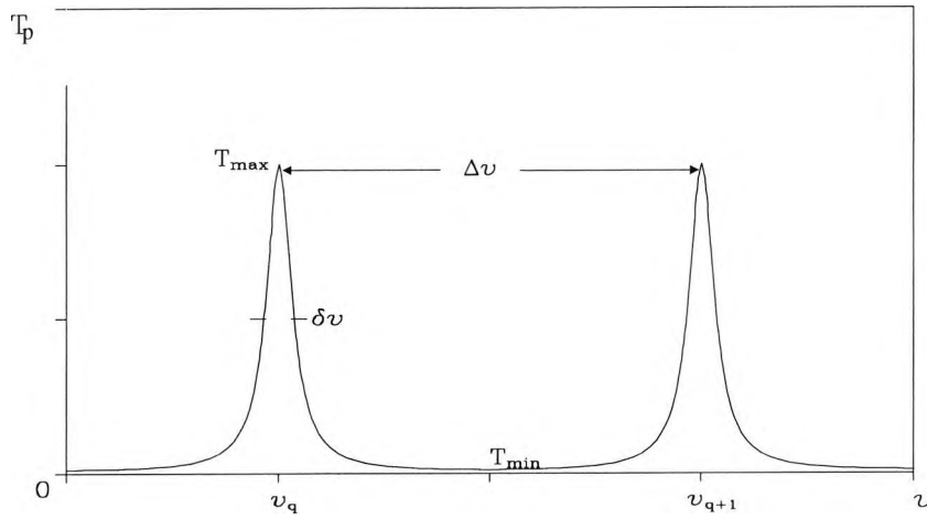
Figure 2.8 Intensity transmission vs. incident frequency
