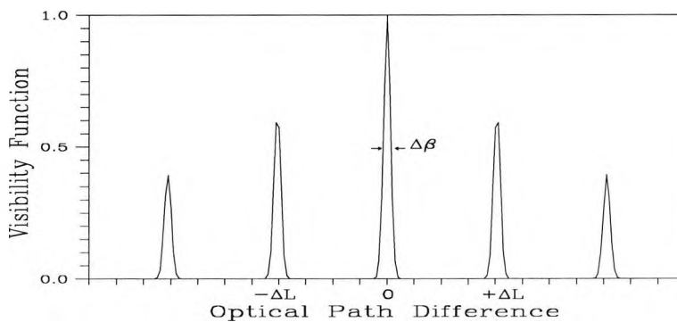
Figure 4.13(b) Visibility function of a multi-mode laser
