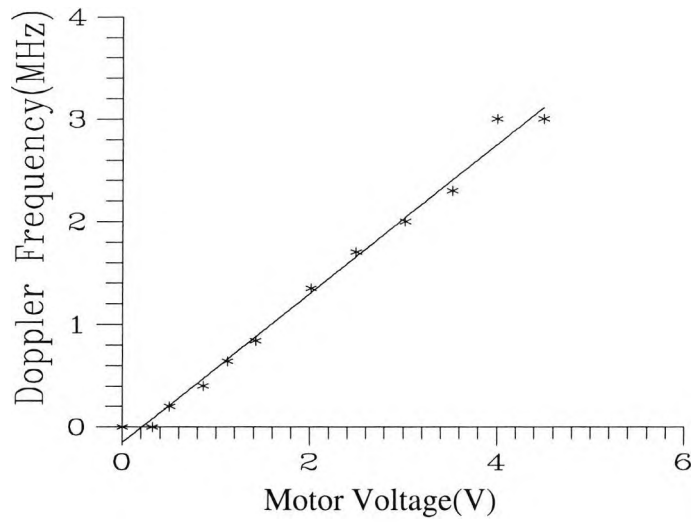
Figure 6.4(a) Doppler frequency dependence on motor voltage (where the motor voltage is proportional to the rotation speed)
