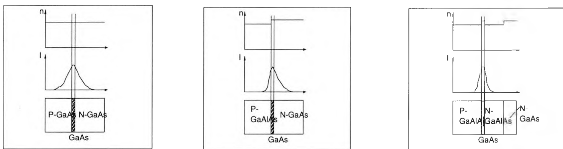
(a) Homostructure laser (b) Single-heterostructure laser (c) Double-heterostructure
