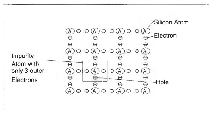
Figure 3.2(b) Bonding in doped p-type silicon
