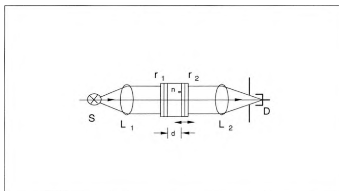
Figure 2.6 The Fabry-Perot interferometer
