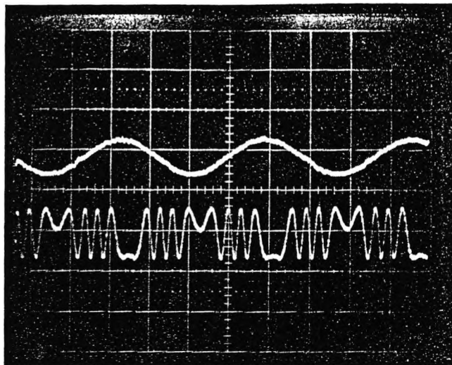
Fig. 2. Typical interference signals observed from self-mixing (vertical axis, arbitrary units; horizontal axis, 0.2 ms/division).
