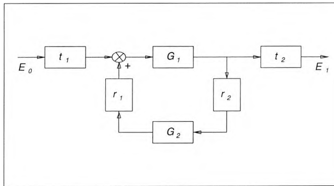
Figure 2.7 Block diagram of the FP feedback system
