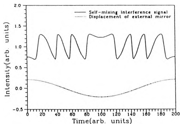
Figure 1 Intensity modulation by self-mixing interference
