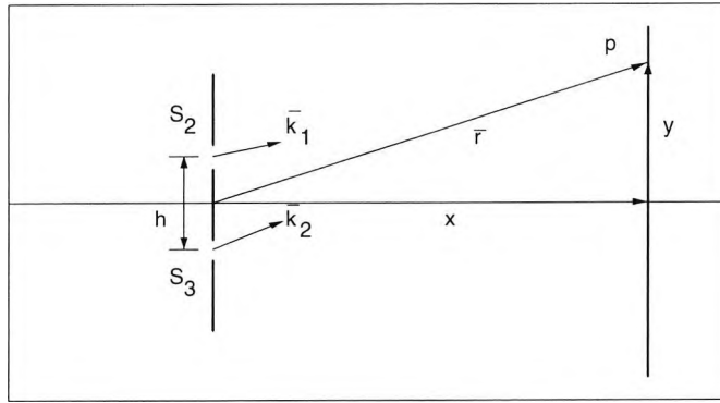
Figure 2.2 Geometry for analyzing two beam interference
