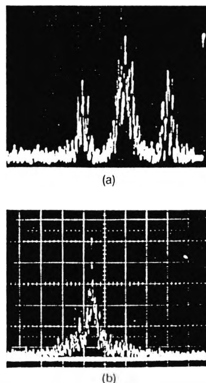
Fig. 3. Output spectra: (a) Doppler spectrum produced by Doppler-shifted frequency, (b) noise spectrum without rotation of the target. Vertical logarithmic scale, arbitrary units [same for (a) and (b)]; horizontal scale, 0.5 MHz per division [same for (a) and (b)]; central peak, zero frequency (dc) [same for (a) and (b)].
