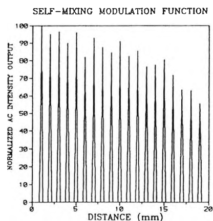
Fig. 4. Dependence of a self-mixing interference profile (for a multimode laser diode) on the distance of the external reflector from the laser.
