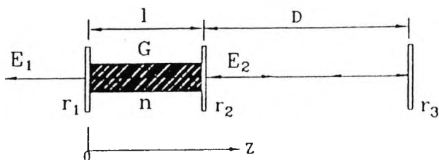
Fig. 1. Schematic of a diode laser with external optical feedback. r_1 , r_2 , laser facet amplitude reflectivities; r_3 , target amplitude reflectivity; G , single-pass gain transfer function; and n , effective refractive index of gain medium.
