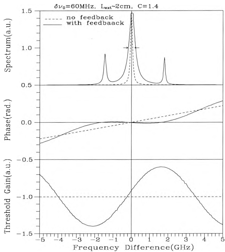
Figure 4.5 A schematic of lasing condition at multiple solutions for phase change, threshold gain and optical frequency
