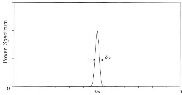
Figure 3.13 The power spectrum of a semiconductor laser below threshold
