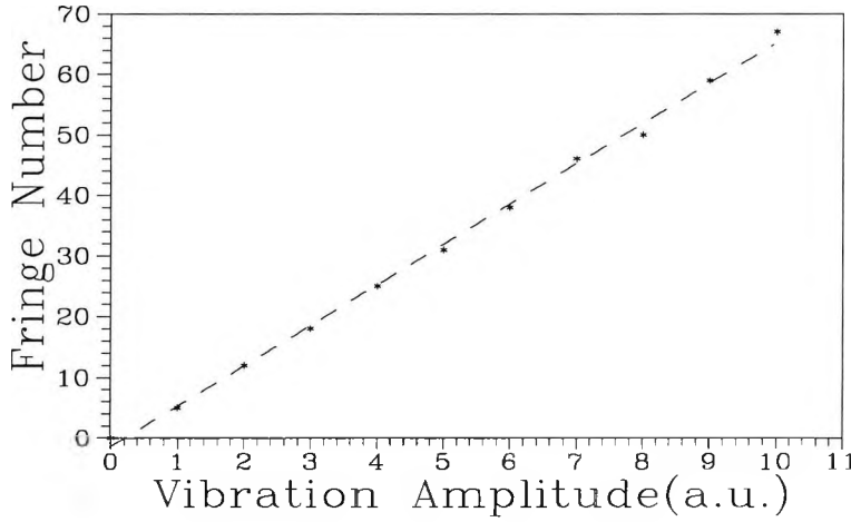
Figure 6.10 Fringe number dependence on vibrational amplitude
