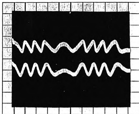
Fig. 9. Self-mixing interference patterns (upper trace) compared with conventional interference patterns (lower trace) (vertical axis, arbitrary units, horizontal axis, 0.2 ms/division).
