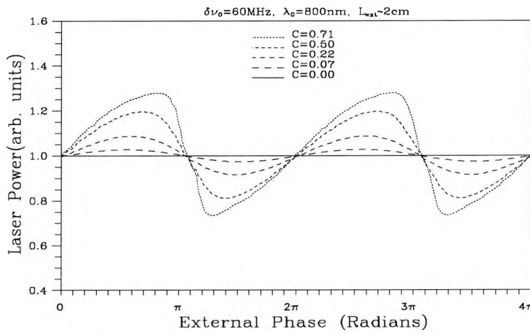
Figure 4.10 Optical power versus external phase change
