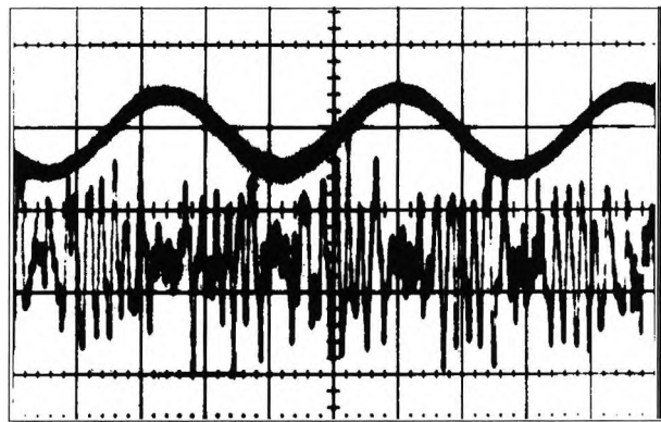
Figure 6.7 Beat frequency(lower trace) produced by current modulation of diode laser against upper trace(current modulation signal applied to LD).
