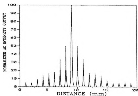
Fig.5 Visibility function of laser used for ranging experiments obtained from a two beam Michelson interferometer
