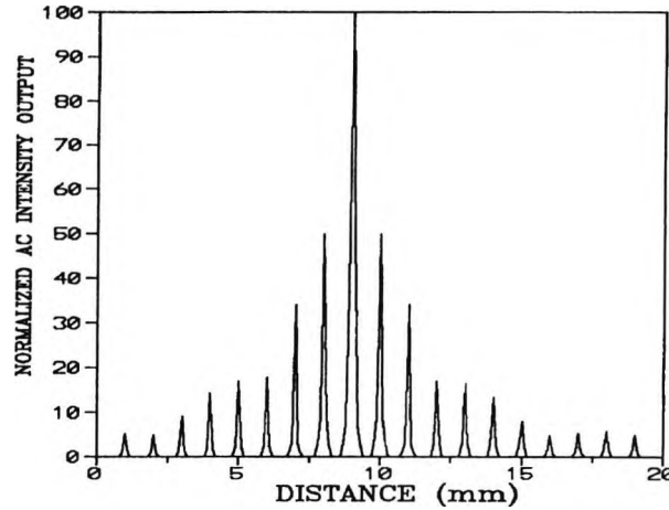
Figure 5.8 Visibility function of the diode laser used
