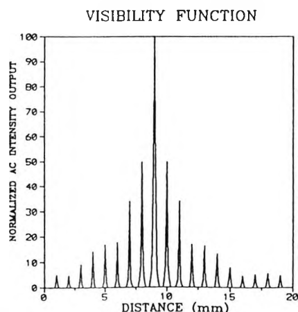
Fig. 3. Visibility function obtained from the multimode laser diode (with output power of 2.5 mW) and determined with a Michelson interferometer
