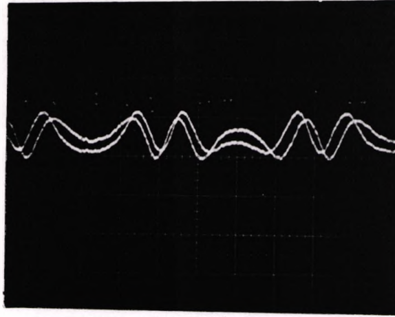
Figure 6.15 Output signals from two diode lasers
