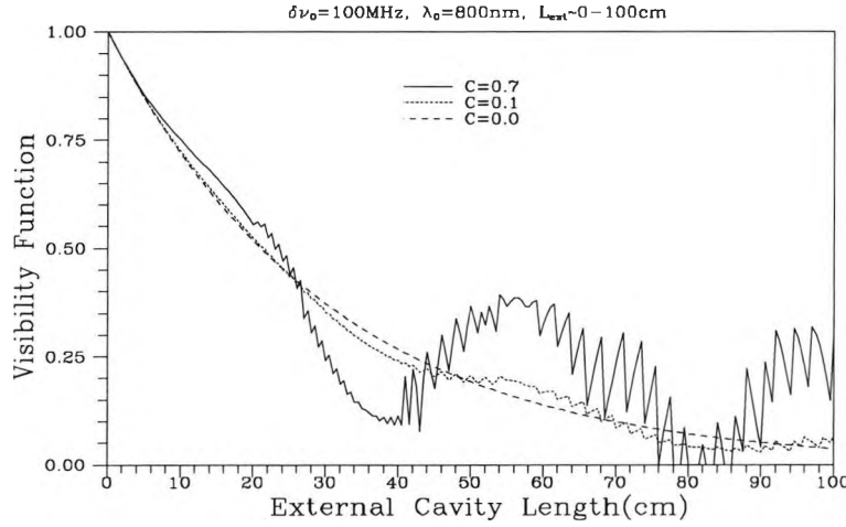
Figure 4.9 Visibility function of the laser with feedback
