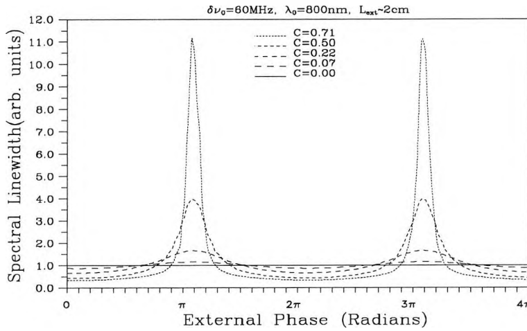
Figure 4.6 Spectral linewidth versus external phase change
