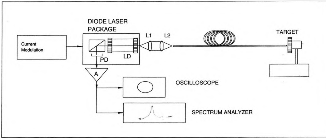
Figure 6.6 Experimental arrangement for self-mixing ranging
