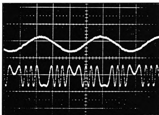
Figure 5.4 Self-mixing interference signal with weak feedback coefficient(upper trace—displacement of external mirror, lower trace—self-mixing interference signal) Vertical axis, arbitrary units; horizontal axis, 0.5 ms/division.
