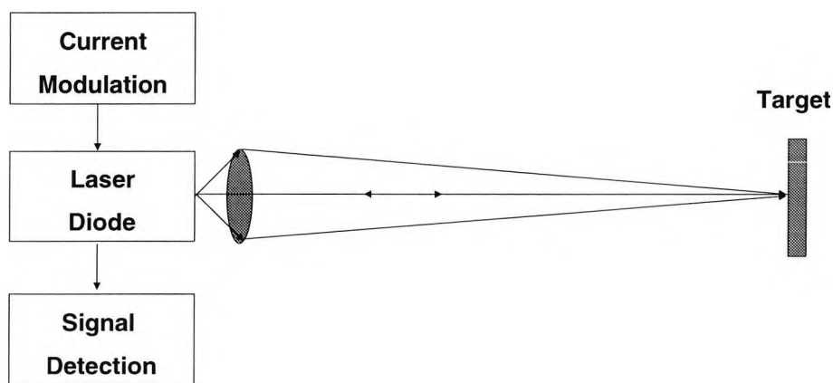
Figure 5.10 Block diagram of self-mixing ranging scheme
