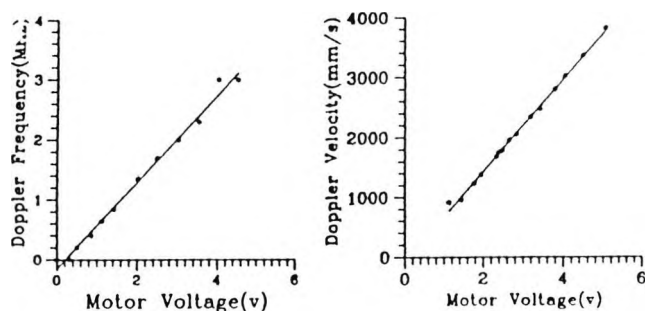
Fig. 4. Measured velocity of rotation disk dependence on the Doppler-shifted frequency.
