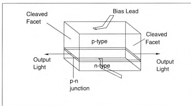
Figure 3.6 Typical broad-area p-n homojunction GaAs Laser
