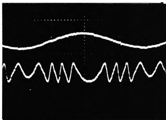
Figure 5.3 A typical self-mixing interference signal Upper trace—Voltage signal of external target mirror vibration, Lower trace—intensity modulation detected from laser output. (vertical axis, arbitrary units; horizontal axis 0.2 ms/division).
