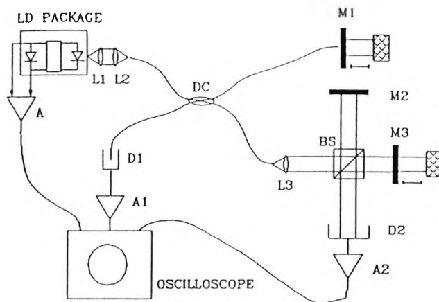
Fig. 8. Schematic experimental arrangement for a comparison between self-mixing interference and conventional two-beam interference: LD, laser diode; D1, D2, photodiodes, L1-L3, lenses; A, A1, A2, amplifiers; M1-M3, mirrors; BS, beam splitter.
