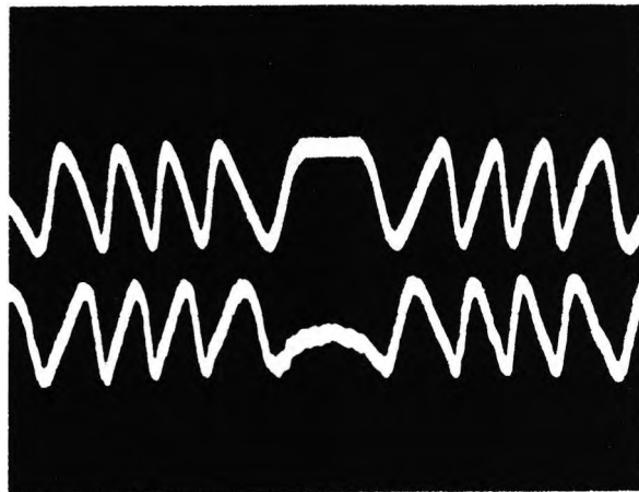
Figure 5.6 Sign inversion of self-mixing interference signal
