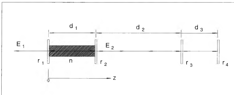
Figure 6.2 Schematic of self-mixing LDV system
