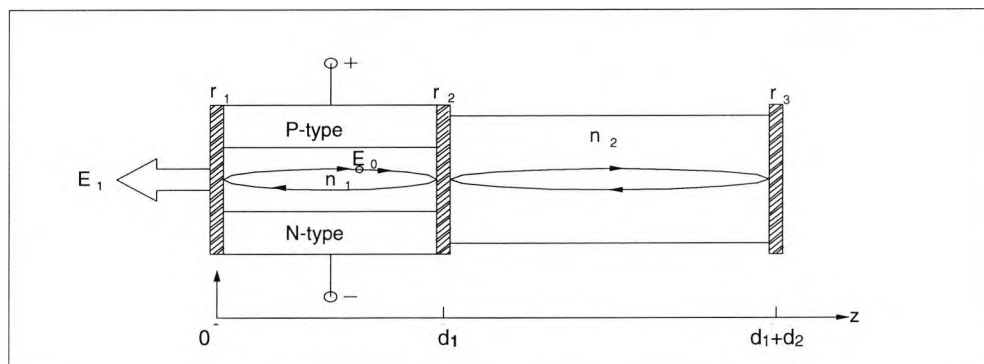
Figure 4.1 Schematic arrangement of a diode laser with external optical feedback
