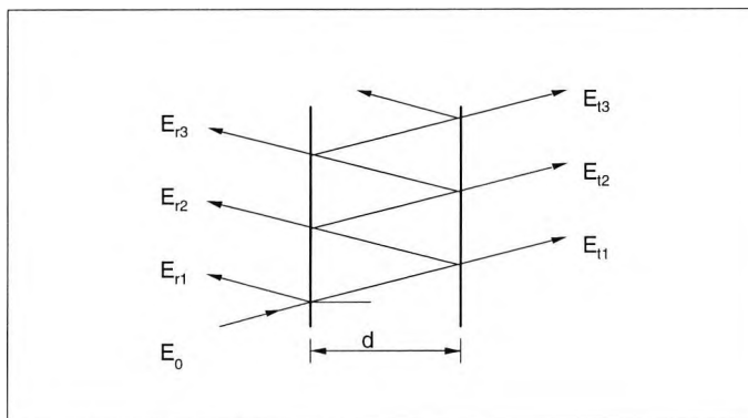
Figure 2.3 Multiple reflection between two parallel mirrors separated by a distance d
