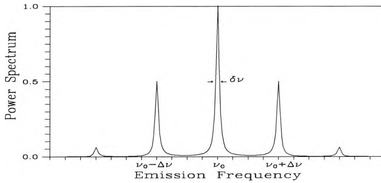
Figure 4.13(a) Schematic of a multi-mode laser spectrum
