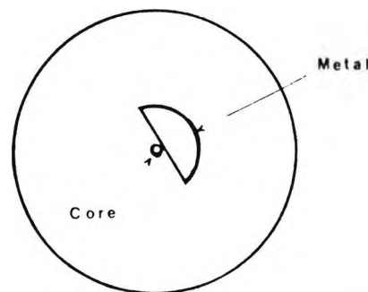
Fig. 4. Schematic diagram of a composite metal-glass polarizer.
