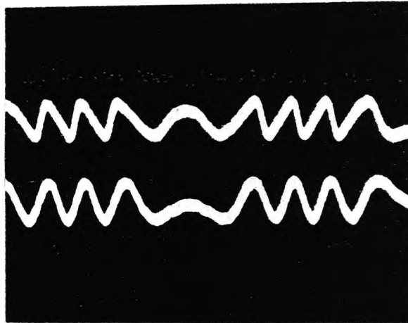
Figure 5.5 Asymmetric feature of Self-mixing interference
