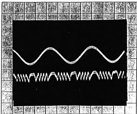
Fig. 7. Sawtoothlike signal-output dependence on direction of phase variation.
