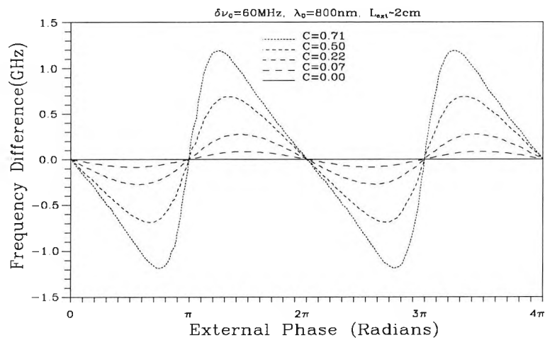
Figure 4.4 Frequency shifts versus external phase change
