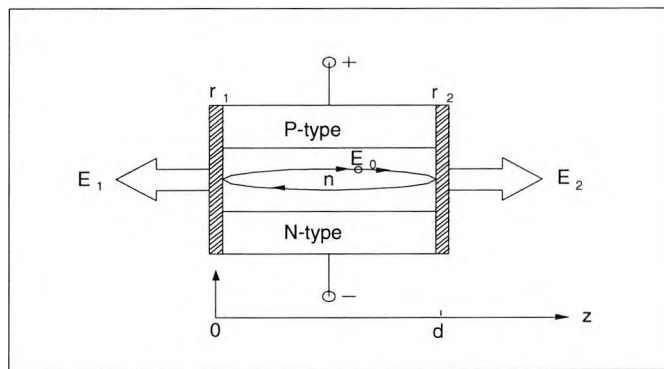
Figure 3.12 Fabry-Perot cavity structure of a diode laser
