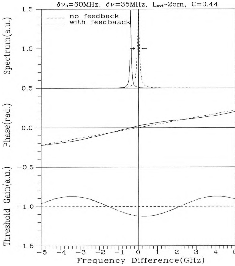
Figure 4.3 Schematics of optical spectrum, phase change and threshold gain versus optical frequency difference
