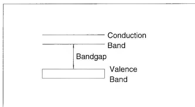
Figure 3.1 Energy-level diagram in a pure semiconductor
