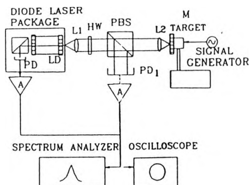
Figure 2 Experimental arrangement for self-mixing interference
