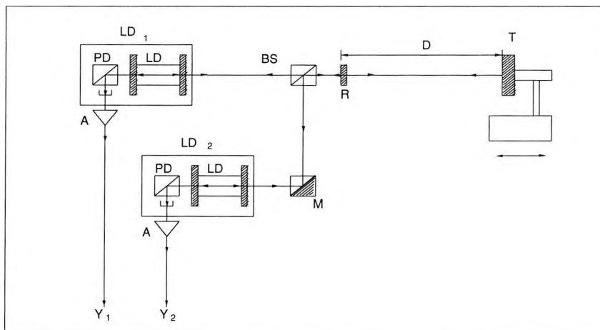
Figure 6.11 Schematic of two diode laser self-mixing system
