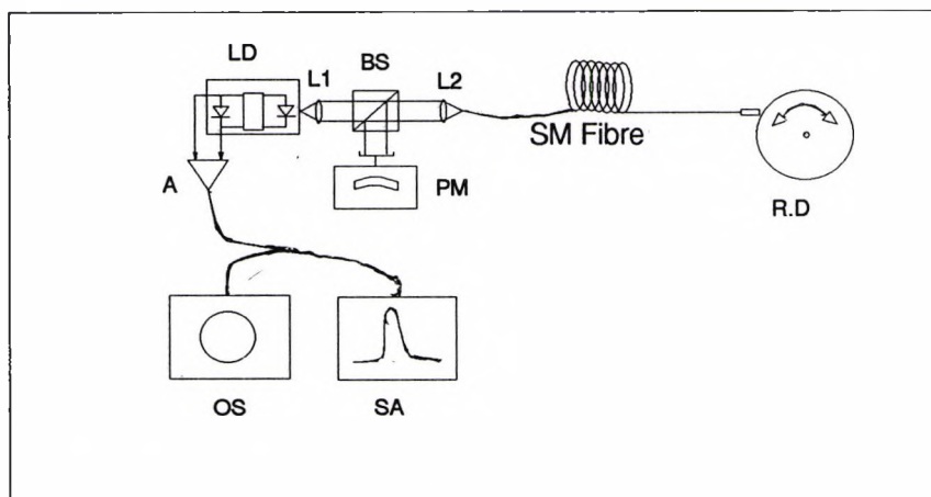
Figure 6.1 Experimental arrangement for self-mixing LDV
