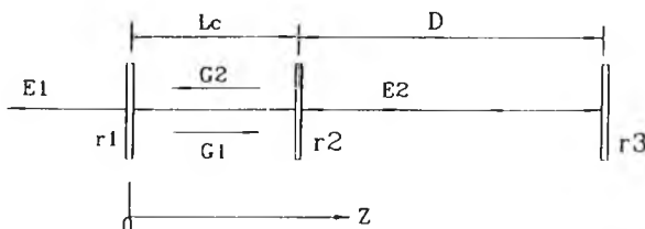
Fig. 11. Schematic of a simple laser with external optical feedback: L_c , laser-cavity length; D , distance from laser-cavity front face to target; E_1 , electric field from back face; E_2 , combined electric field from front face and reflected from target; G_1 , G_2 , forward and backward gain coefficients in the laser cavity; r_1 – r_3 , reflectivities of the laser-cavity ends and the target; Z , direction.
