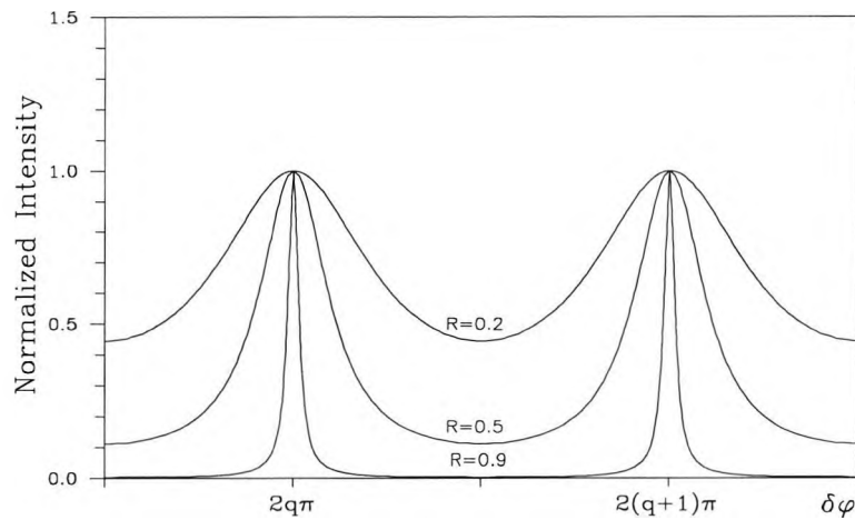
Figure 2.4 Intensity distribution of multi-beam interference
