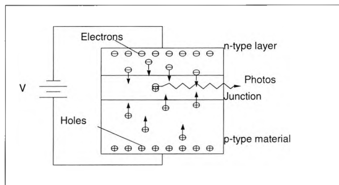
Figure 3.4 Forward-biasing p-n junction in a semiconductor
