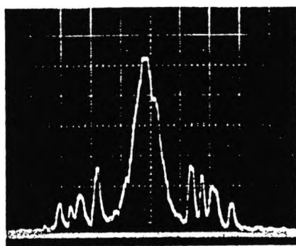
Fig. 5. Higher harmonics of Doppler-shifted frequency in self-mixing spectrum. Vertical logarithmic scale, arbitrary units; horizontal scale, 0.1 MHz per division and with video filter of 10 Hz; central peak, zero frequency (dc).
