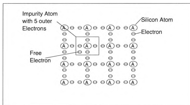
Figure 3.2(a) Bonding in doped n-type silicon
