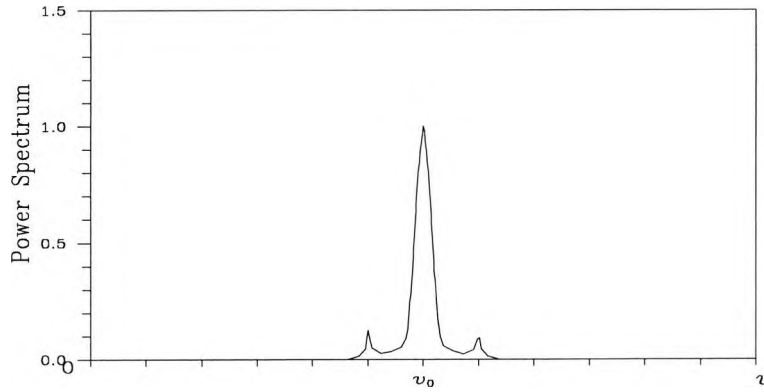
Figure 3.11 The laser spectrum with satellite side peaks
