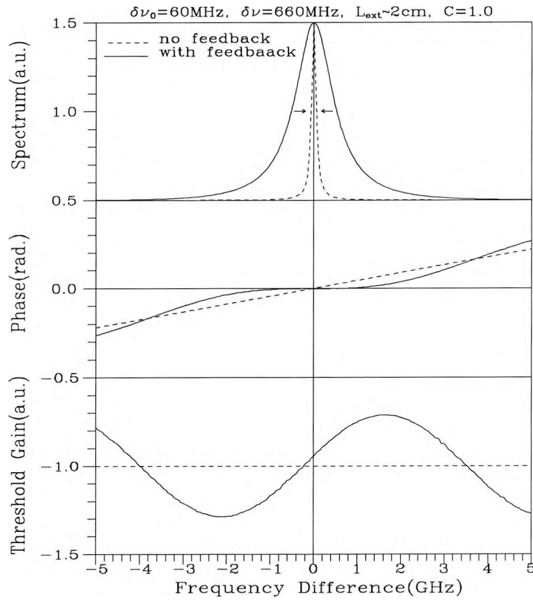
Figure 4.7 A schematic of lasing condition at C=1
