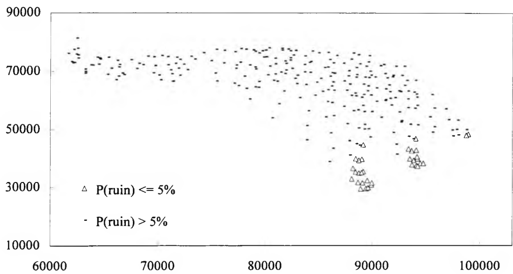
Figure 7.18. Graph of S.D. vs. Mean for all 286 portfolios; a mix of 20 year endowments and 20 year index-linked annuities; sm = 15\% , in real terms.
