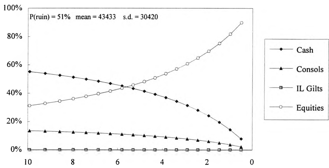
Figure 8.8 Graph of Optimal Asset Proportions vs. Discounted Mean Term of liabilities: sm = 15\% , in real terms, at r = 8 .
