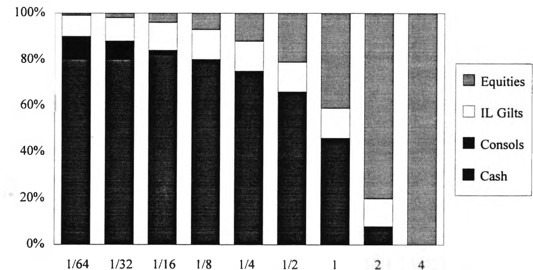
Figure 4.1. Optimal portfolios for the 1 year case in nominal terms at various values of r .
