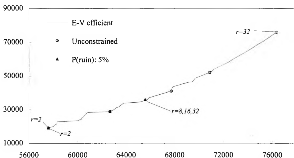
Figure 6.12. Graph of S.D. vs. Mean for E-V efficient and utility maximizing portfolios with and without ruin constraints: sm = 25\% , in real terms.
