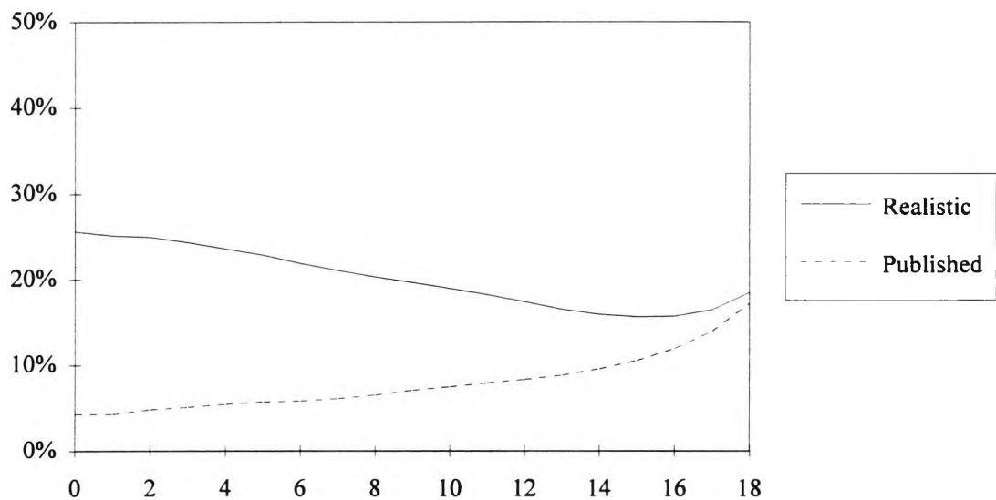
Figure 8.5 Graph of Mean Realistic Free Asset Ratio and Mean Published Free Asset Ratio over time: sm = 15\% , in nominal terms, at r = 32 .
