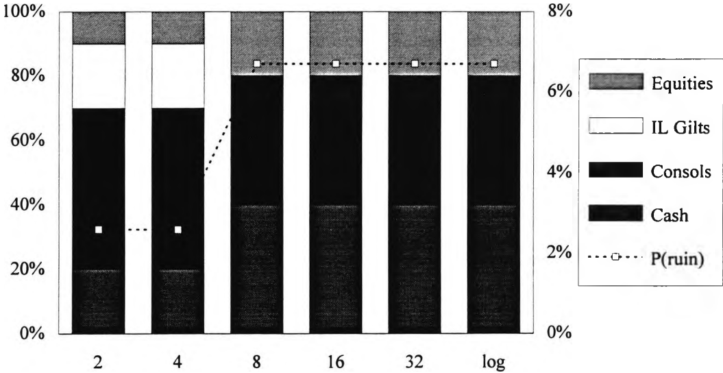
Figure 7.3. Optimal portfolios: sm = 15\% , in real terms.
