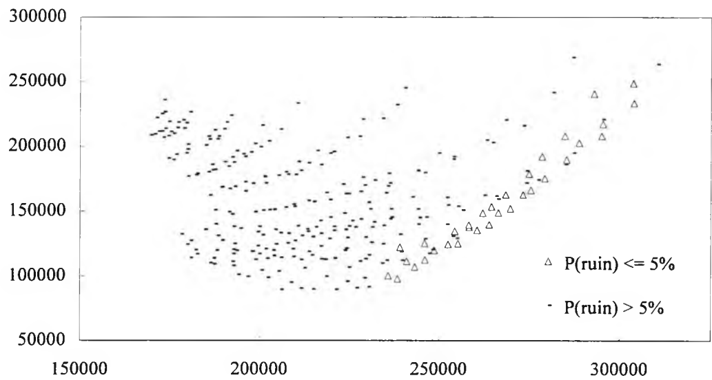
Figure 7.17. Graph of S.D. vs. Mean for all 286 portfolios: a mix of 20 year endowments and 20 year index-linked annuities; sm = 15\% , in nominal terms.
