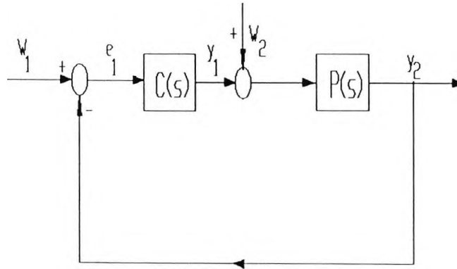
Fig. (2.1): General Control System Configuration
