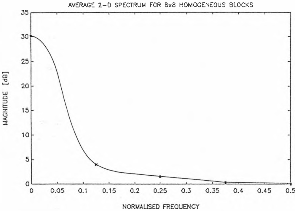
Figure 5.15: Average one-dimensional spectrum for monotone 8 \times 8 blocks.
