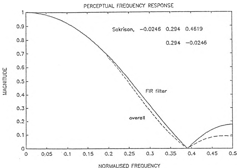
Figure 5.17: Frequency response of the filter h_{st}(x) of order 5 based on the MTF proposed by Mannos and Sakrison.
