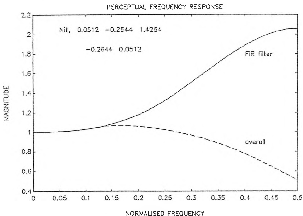
Figure 5.21: Frequency response of the filter h_{en}(x) of order 5 based on the MTF proposed by Nill.
