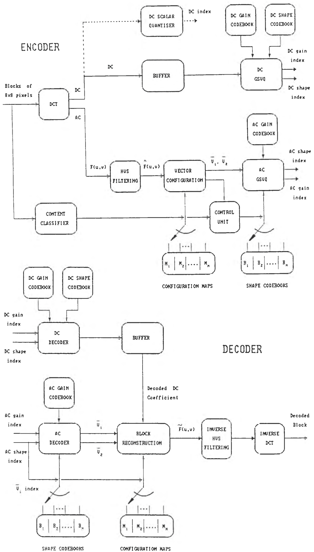
Figure 4.1: DCGSVQ - Block Diagram
