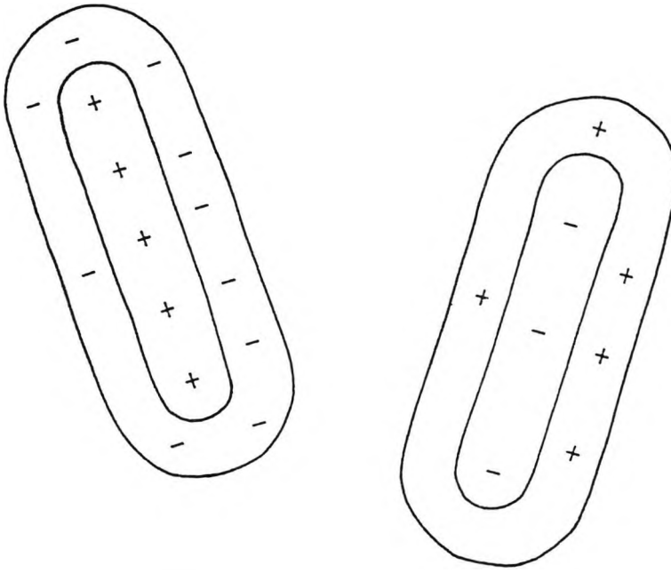
Figure 3.14: Receptive field of a simple cell (after [Kuffler 1976]).
