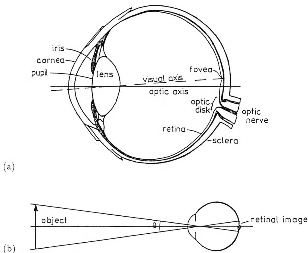
Figure 3.3: (a) Diagram of a cross section of the human eye.
