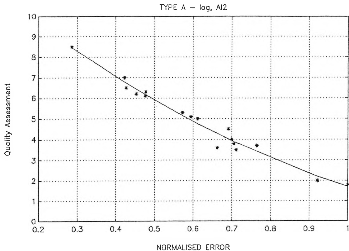
Figure 6.11: Best quadratic fit for Type A procedure. ( logarithmic function and AI2 )
