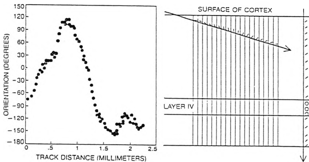
Figure 3.16: Grouping of cortical cells according to orientation preference (after [Huble 1979]).
