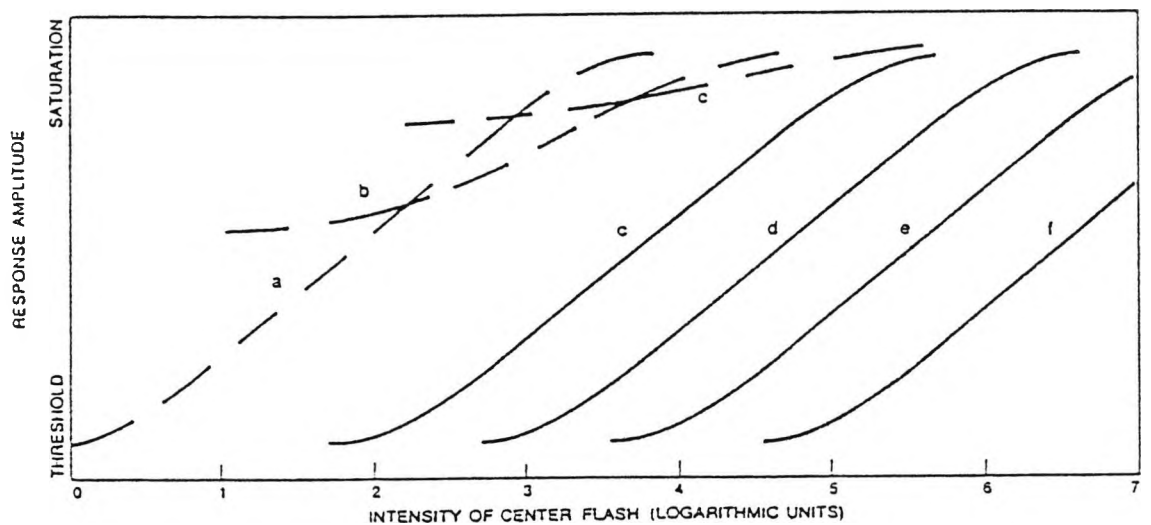
Figure 3.5: Operating characteristics of rods (dashed lines) and cones (solid lines) at six background luminances (a-f) after [Werblin 1973].
