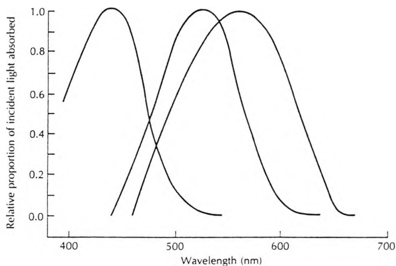
Figure 3.7: Absorption spectra for three classes of cones (after [Wald 1965]).
