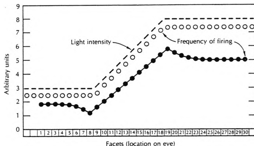
Figure 3.10: Qualitative prediction of the facets activity in the Limulus eye for a given intensity distribution (after [Cornsweet 1970]).
