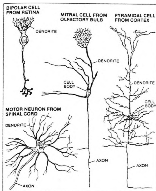
Figure 3.1: Typical neurons (after [Kuffler 1976]).
