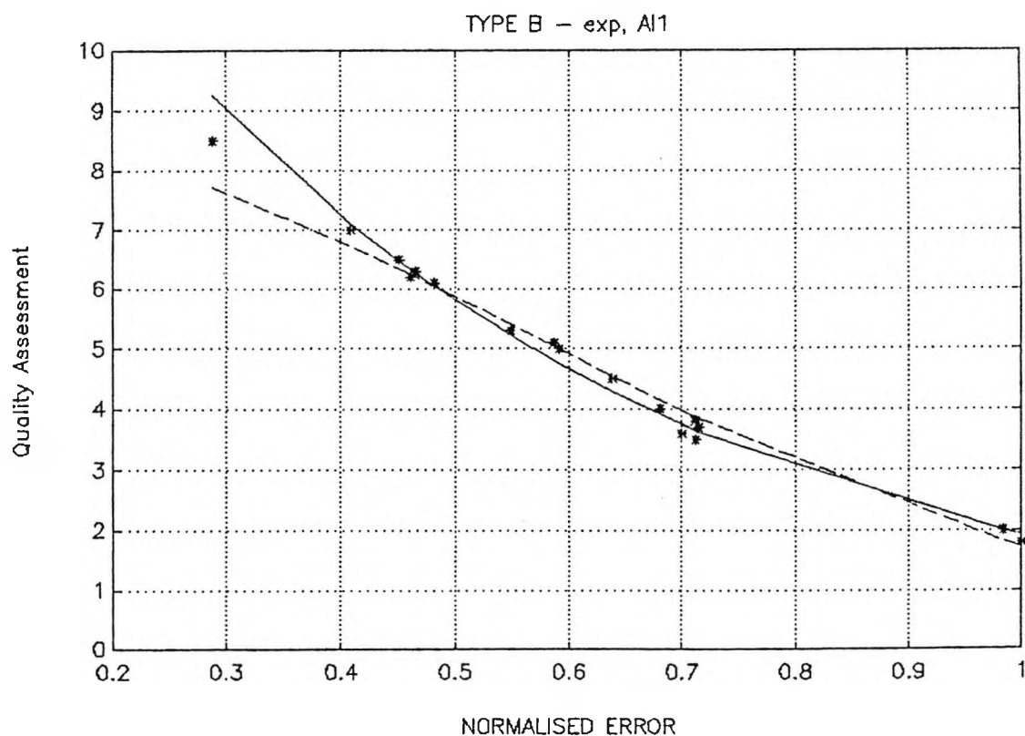
Figure 6.15: Best exponential and gaussian fits for Type B procedure. ( an exponential transform and AI1 )
