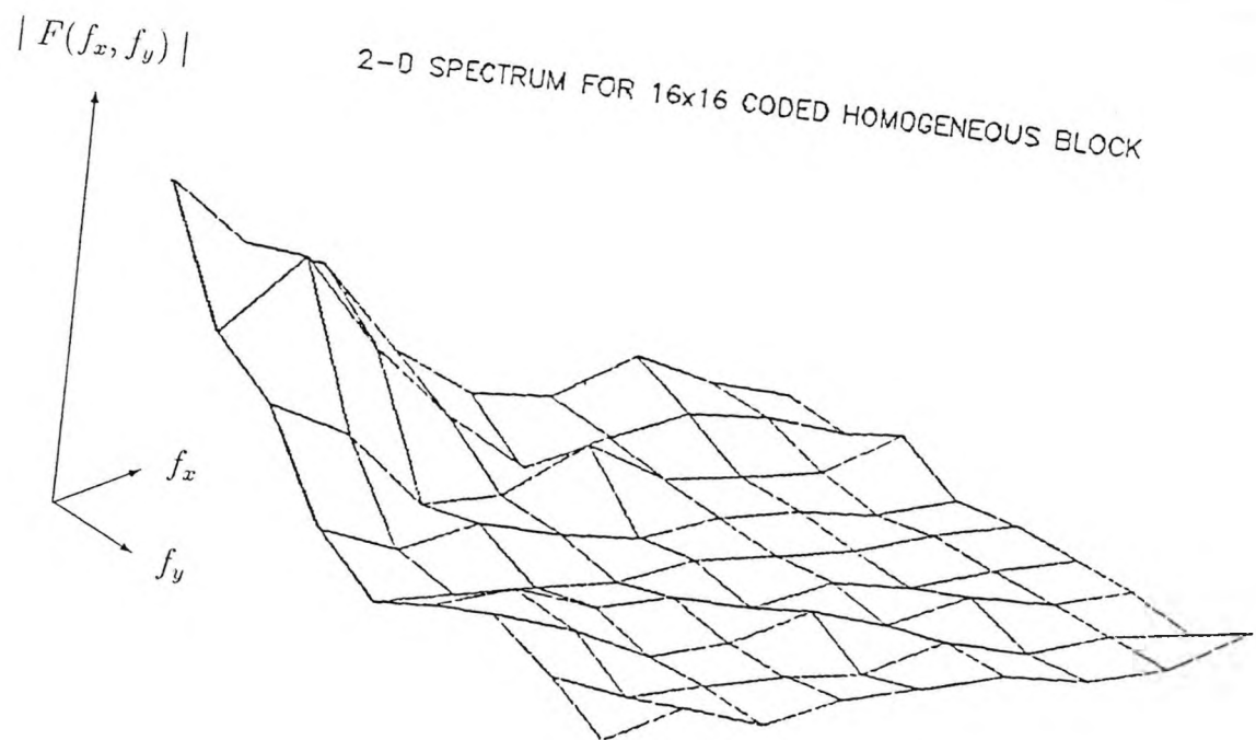
Figure 5.27: Two-dimensional spectrum for a 16 \times 16 monotone subimage from the coded image 'Lena1'.
