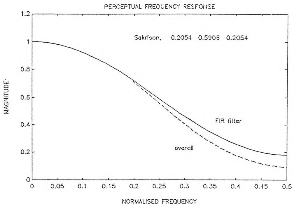
Figure 5.16: Frequency response of the filter h(x) of order 3 based on the MTF proposed by Mannos and Sakrison
