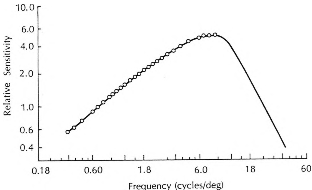
Figure 3.20: Spatial frequency response of the HVS (after [Cornsweet 1970]).
