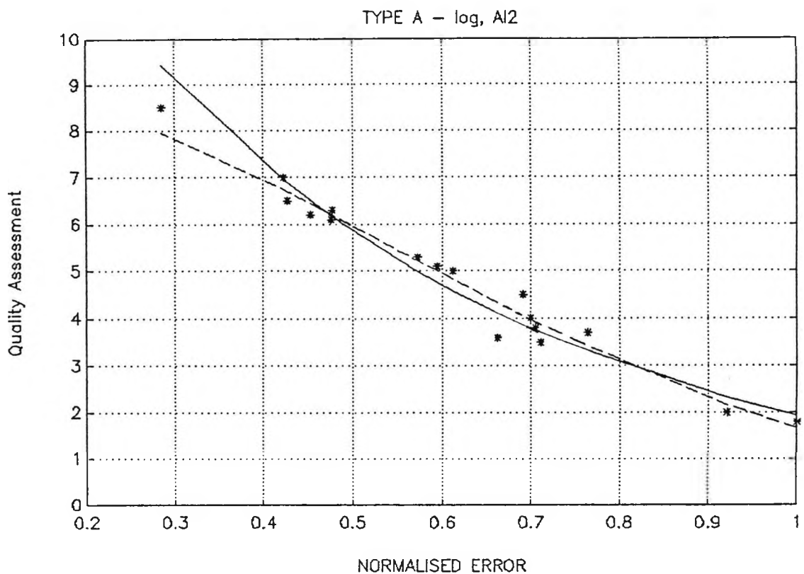
Figure 6.13: Best exponential and gaussian fits for Type A procedure. ( logarithmic function and AI2 )
