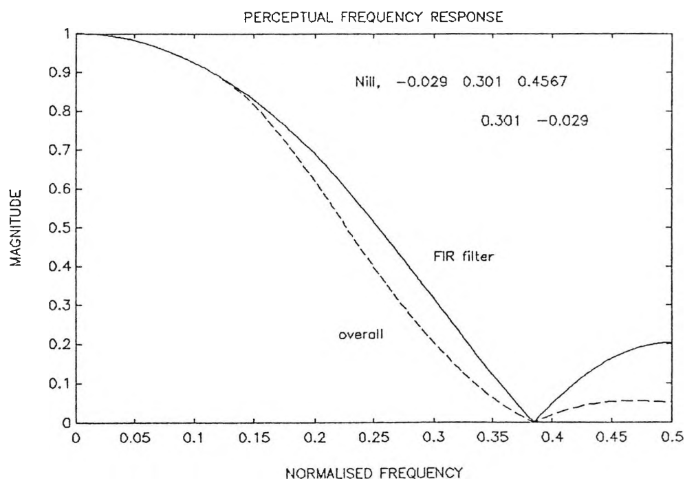
Figure 5.19: Frequency response of the filter h_{st}(x) of order 5 based on the MTF proposed by Nill.
