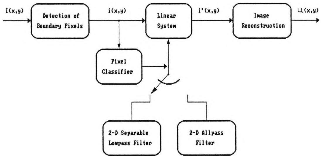
Figure 5.9: First step - grid noise filtering.
