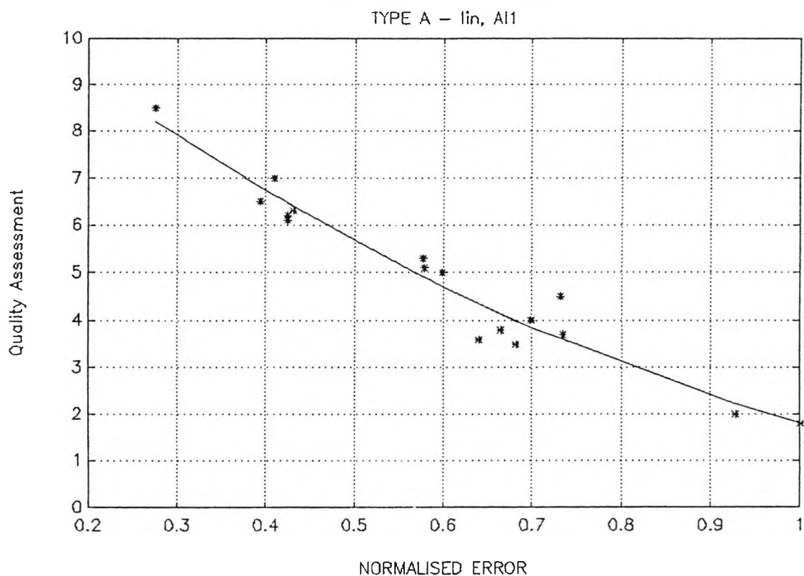
Figure 6.12: Worst quadratic fit for Type A procedure. ( linear function and AI1 )
