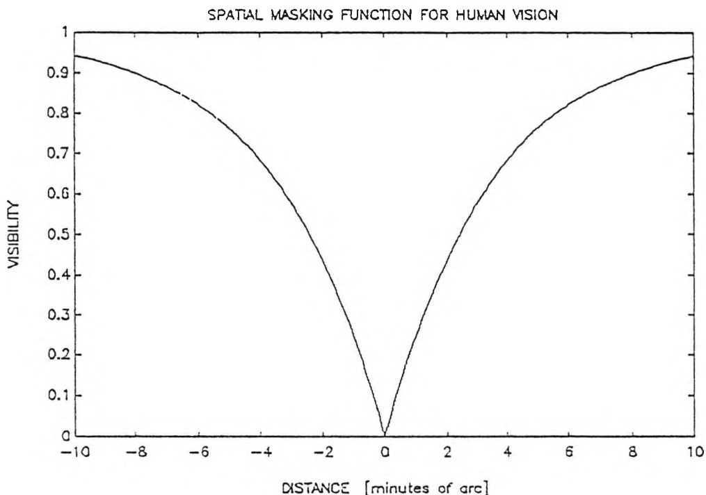
Figure 3.22: Spatial masking function (for a=0.75 ).
