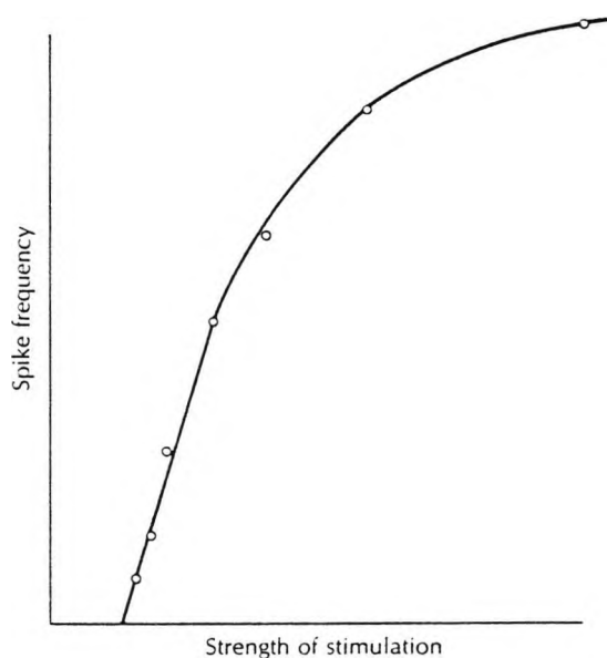
Figure 3.2: The relationship between the intensity of the input stimulus to a neuron and the resulting frequency of its pulses (after [Cornsweet 1970]).
