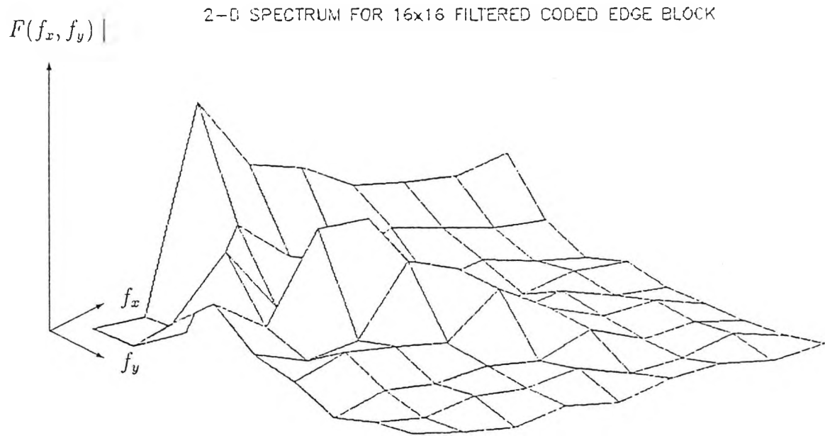
Figure 5.29: Two-dimensional spectrum for a 16 \times 16 edge subimage from the coded image 'Lena1'.
