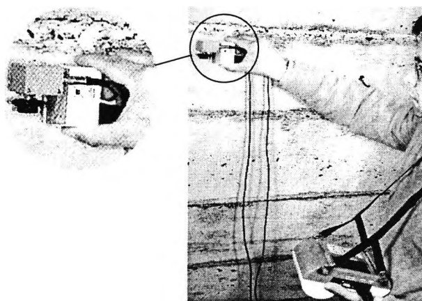
(b) Profometer 4 from Proceq SA (Switzerland) - The operator is using a path-measuring device, an attachment to the search probe that makes re-bars visible on the LCD screen through an integrated CyberScan software
