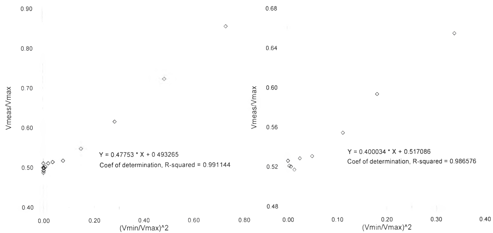
(a) Plot for 12mm re-bars at 36mm cover (b) Plot for 20mm re-bars at 36mm cover Figure F-4.5 Plots of (v_{meas}/v_{max}) versus (v_{min}/v_{max})^2 for 12mm and 20mm re-bars
