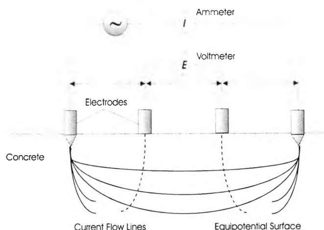
Figure C.6 Four-probe resistivity test layout
