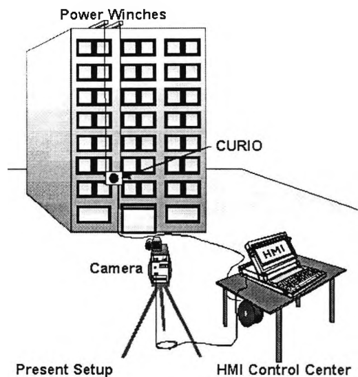
Figure 11.7 Current CURIO Inspection Setup
