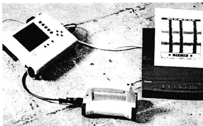
(a) Ferroskan FS 10 from Hilti (Gt. Britain) - Gray scale image of the re-bars is shown on the paper printout
