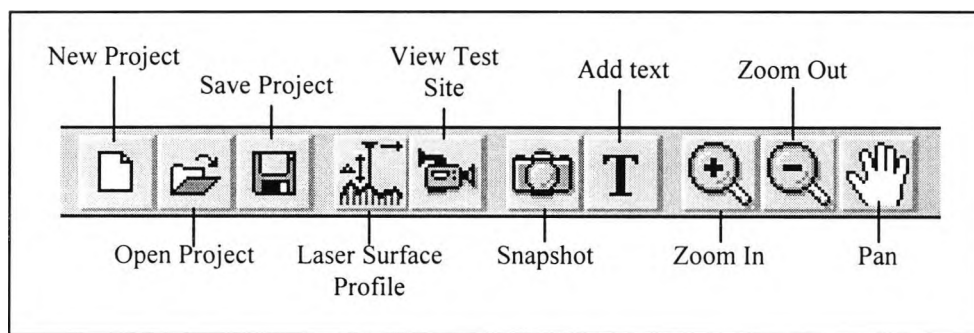
Figure 11.22 The toolbar
