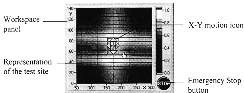
Figure 11.22 Workspace panel
