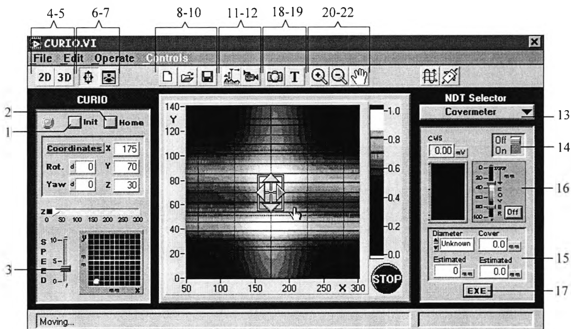
Figure 11.23 CURIO software
