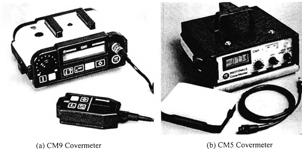
Figure 8.2 Covermeters from Protovalle (Oxford) Ltd
