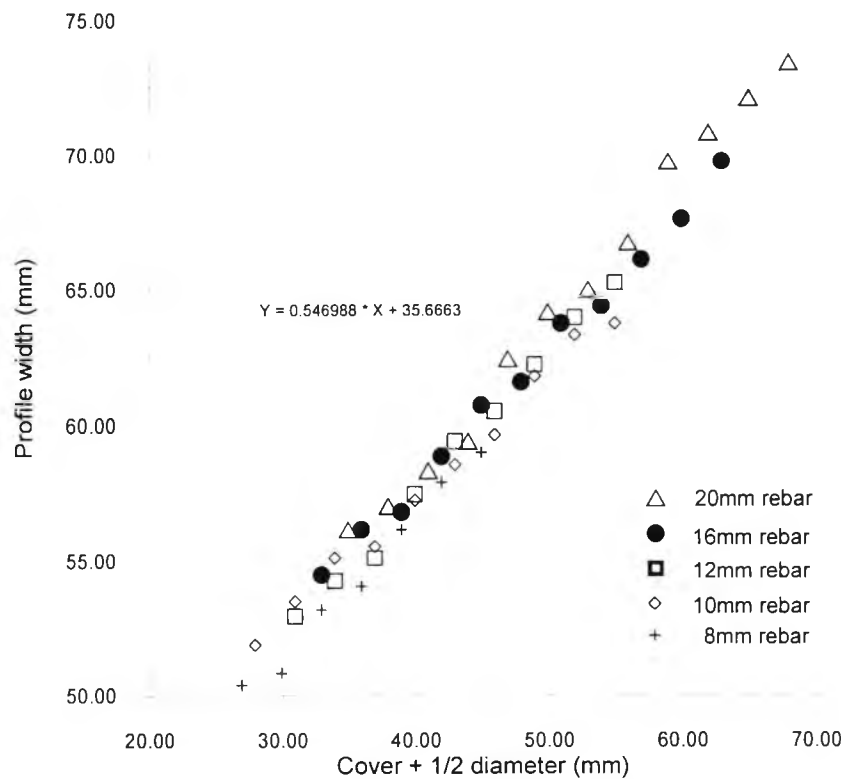
Figure 10.5 A plot of Profile width versus Distance-to-Center using a CM5 covermeter
