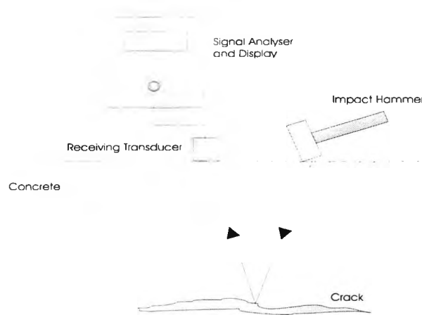
Figure C.3 Pulse Echo Principle
