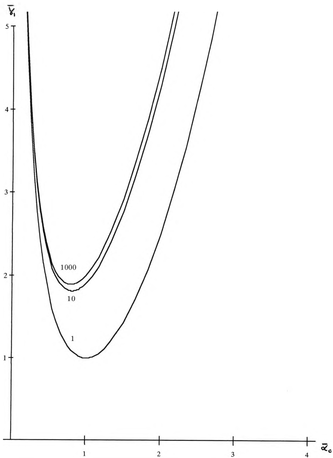
FIGURE 5.3. The neutral stability curve for various values of the scaled Prandtl number \sigma_0 .
