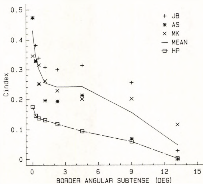
Figure 3.8. Data from Experiment 3 in which a dark border was interposed between the central test object and surround. C_{index} is plotted as a function of the border angular subtense for three normal trichromats (JB, AS and MK) and one protanope HP. The solid line represents the average data for the colour normal subjects.
