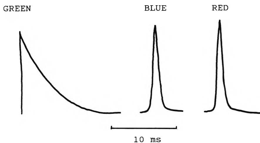
Figure 2.4 (A). Phosphor decay times recorded using the Nicolet oscilloscope and UDT fast response photodiode.
