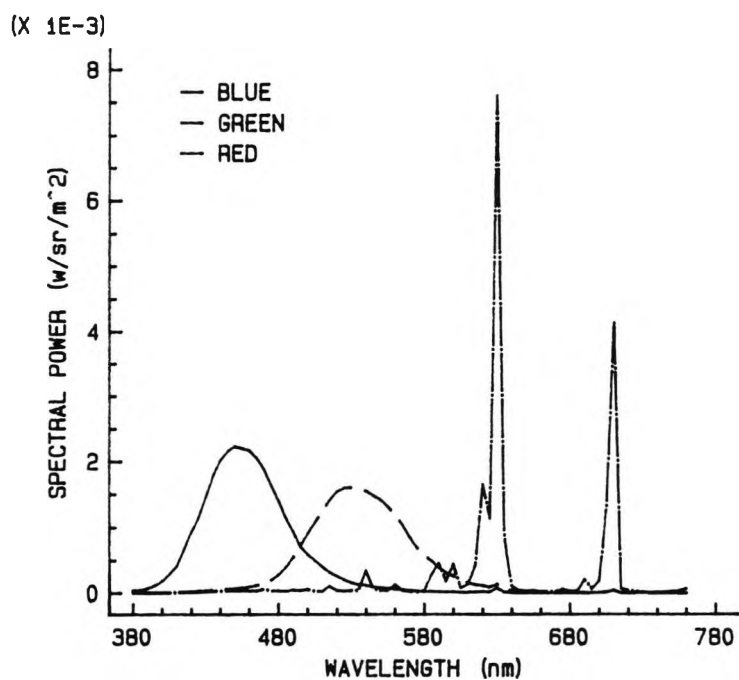
Figure 2.1. Spectral power distributions measured for the three phosphors in the Mitsubishi monitor.
