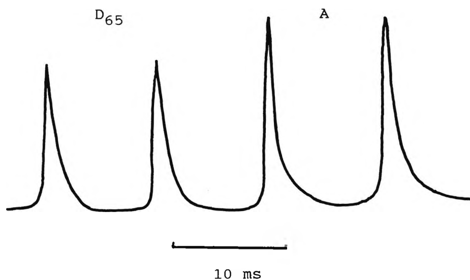
Figure 2.4 (B). Decay times for the combined output of the three phosphors when changing from Standard Illuminant D 65 to Standard Illuminant A.
