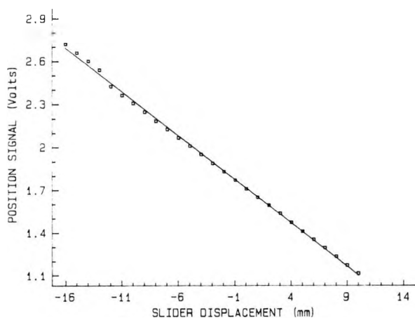
Figure 2.14. Slider calibration showing analogue position signal as a function of displacement in the object plane.
