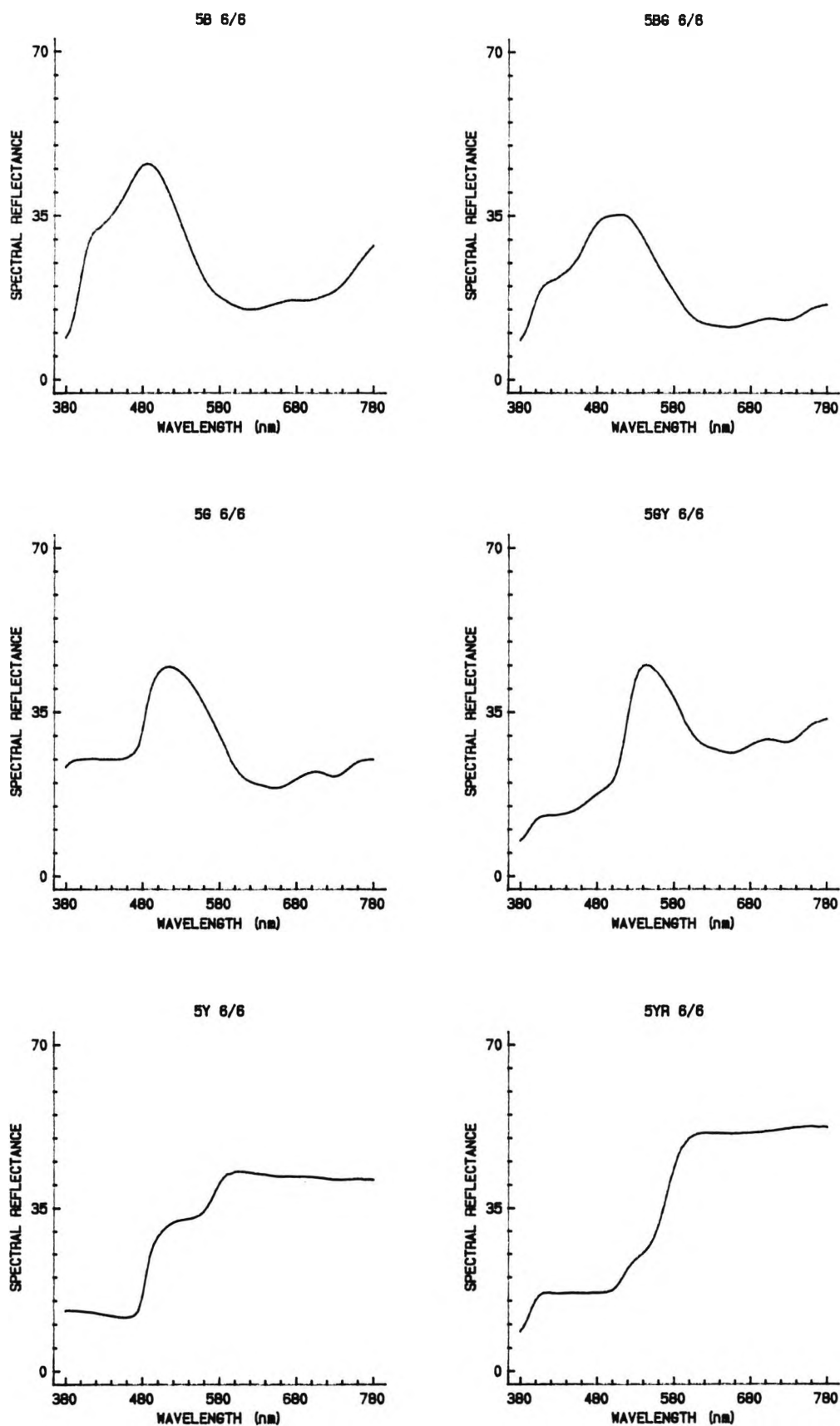
Figure 2.5. The spectral reflectance functions of the Munsell chips used as the basis for the colour samples reproduced in the colour constancy experiment. Measurements were made with the Perkin Elmer spectrophotometer. Contd....
