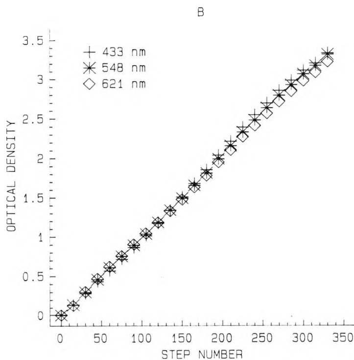
Figure 2.12. (A) Calibration of the neutral density filter wedge for unfiltered white light. (B) Calibration of the same wedge for three wavelengths using narrow band interference filters. In both diagrams, wedge optical density is plotted as a function of the step number.
