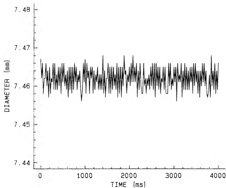
Figure 2.8. Averaged diameter trace for 15 separate recordings of a 7.46 mm artificial pupil over a time period of 4 seconds.
