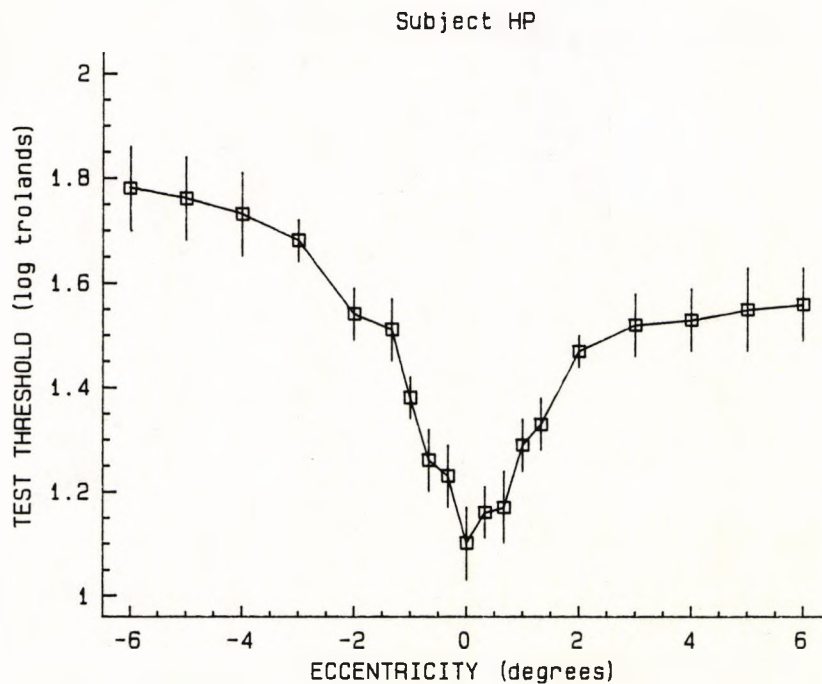
Figure 6.5. The increment threshold retinal illuminance for detection of a test stimulus plotted as a function of eccentricity. The 0.5°, 10 ms test stimulus was presented against a large uniform background field of diameter 44° and retinal illuminance 2.0 log trolands. Negative eccentricities indicate that the test was presented in the nasal visual field. Error bars represent \pm 1 standard deviation.
