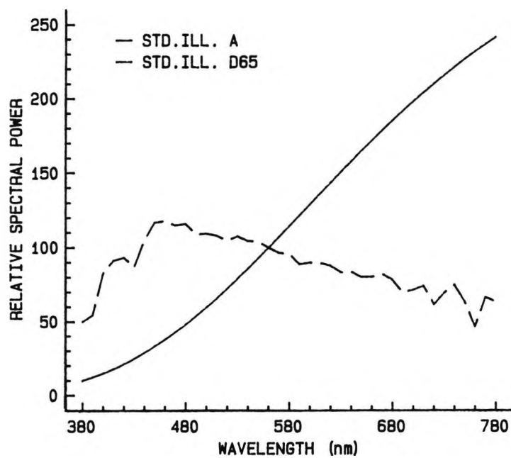
Figure 2.2. Relative spectral power distributions of CIE Standard Illuminants D 65 and A.
