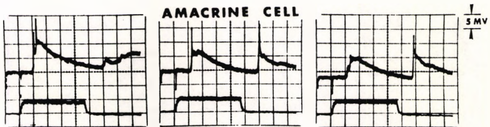
Figure 6.14. Amacrine cell responses for a spot stimulus in the mudpuppy retina (from Werbling and Dowling, 1969).
