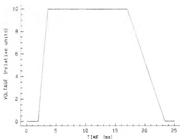
Figure 2.13. The photocurrent versus time trace showing the rise and fall time of the Uniblitz electromagnetic shutter.
