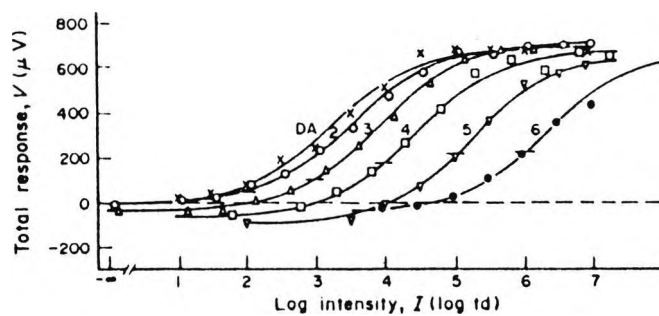
Figure 1.6. Cone flash response versus intensity curves in the presence of adapting background illumination. The background light intensity is indicated by the numbers next to the curves; DA is dark adapted. The small horizontal line in each curve represents the background response level. (After Valetton and van Norren, 1983).
