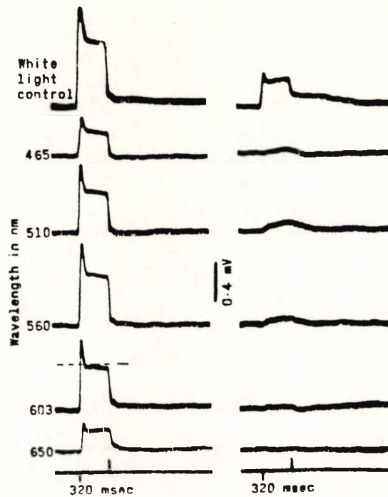
Figure 6.13. Late receptor potentials elicited from the parafovea of the monkey (from Whitten and Brown, 1973).
