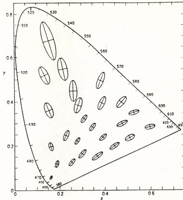
Figure 5.5. Statistical variation of chromaticity matches in different parts of the CIE x,y -chromaticity diagram. The elliptical loci correspond to chromaticities separated from the central point by the standard deviation of settings for chromaticity match. For clarity the axes of each ellipse have been enlarged 10 times. (After MacAdam, 1942).
