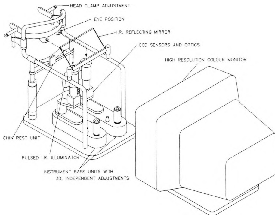
Figure 2.6. Schematic drawing of the P_SCAN 100 system which allows the simultaneous binocular measurement of pupil size and eye movements. See text for detailed description of apparatus. (From Barbur, Hess and Pinney, in preparation).
