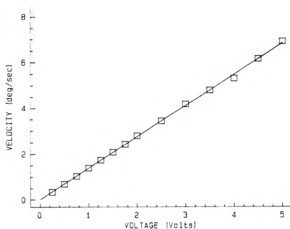
Figure 2.15. Slider velocity is plotted as a function of the analogue output voltage from the computer.
