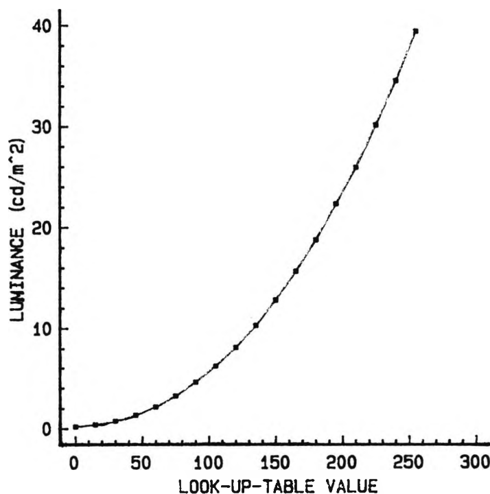
Figure 2.7. Screen luminance level plotted as a function of grey level look-up-table value for the Ayadin monitor used in the pupillometry experiments.
