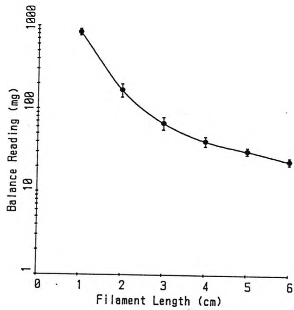
Figure 72. Calibration curve for the Cochet-Bonnet aesthesiometer
