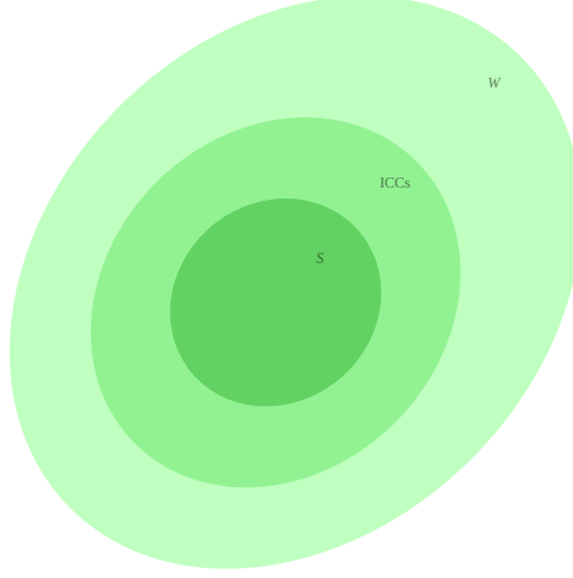
FIGURE 2. The restricted domains according to \mathcal{W}, \mathcal{S}, \text{ICCs} in the menu parameter space.
