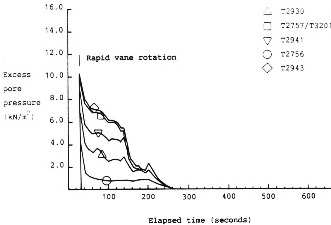
Figure 6.4 Excess pore pressure response recorded in test 180
