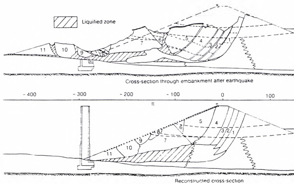
Figure 3.15 Lower San Fernando Dam after collapse (after Seed, 1979b)
