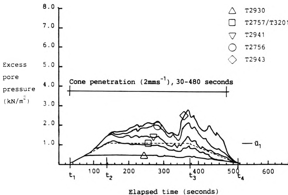
Figure 6.27 An example of a Class II (cone) excess pore pressure response, test 67
