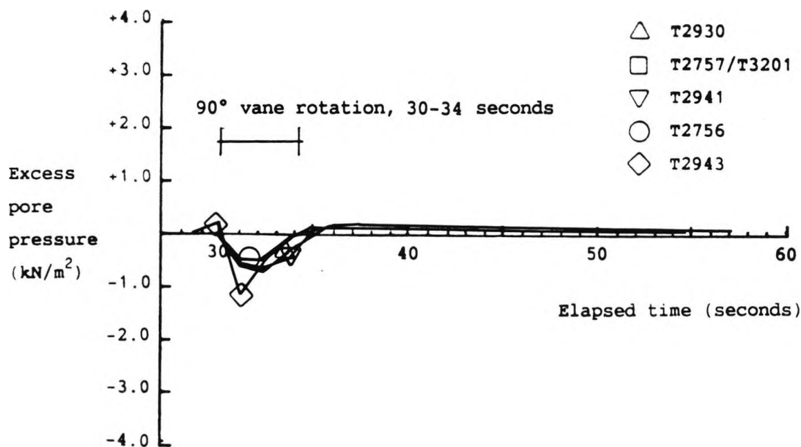
Figure 6.20 A Class III (vane) excess pore pressure response recorded in test 115 (The results of this test are summarised in Table 6.10)
