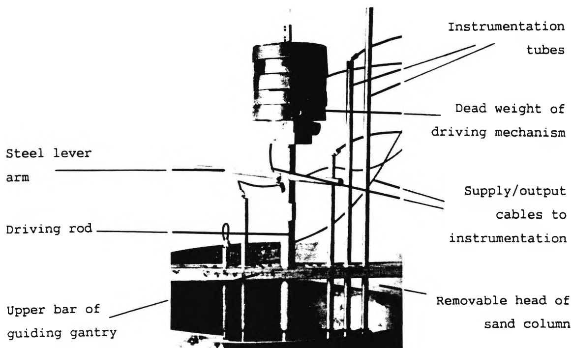
Figure 4.11 Vane rotating mechanism
