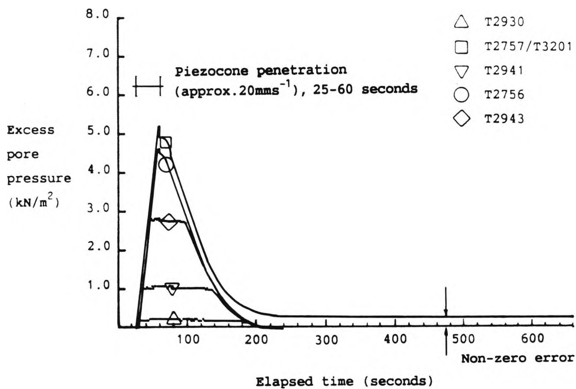
Figure 6.34 Excess pore pressure response recorded in piezocone test 161 (The results of this test are summarised in Table 6.27)
