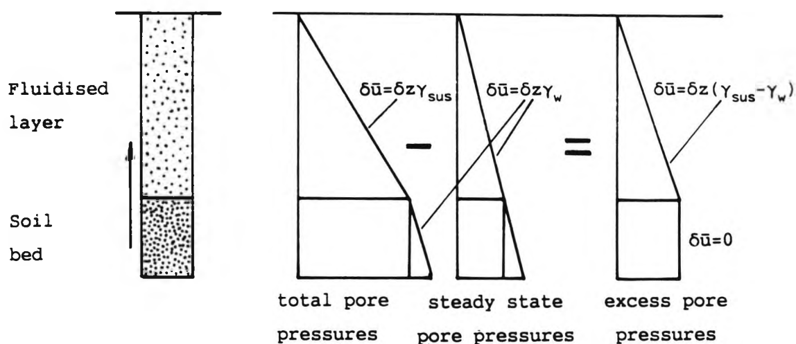
b) Pore pressures in a resedimenting soil bed
