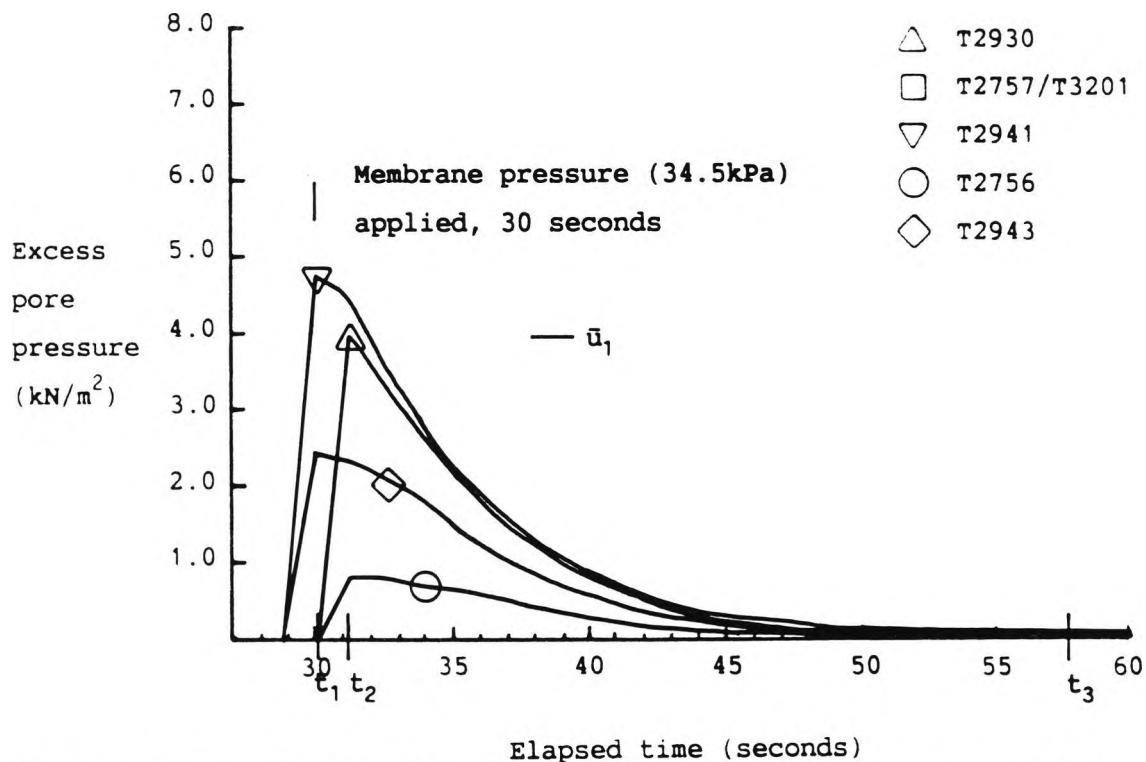
Figure 6.23 An example of a Class II (expanding membrane probe) excess pore pressure response, test 136 (The results of this test are summarised in Table 6.16)
