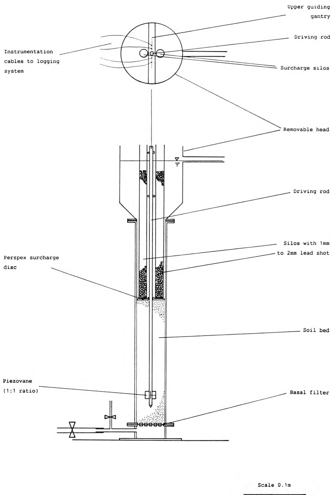
Figure 5.2 Surcharge apparatus assembled inside the sand column (cross- section)
