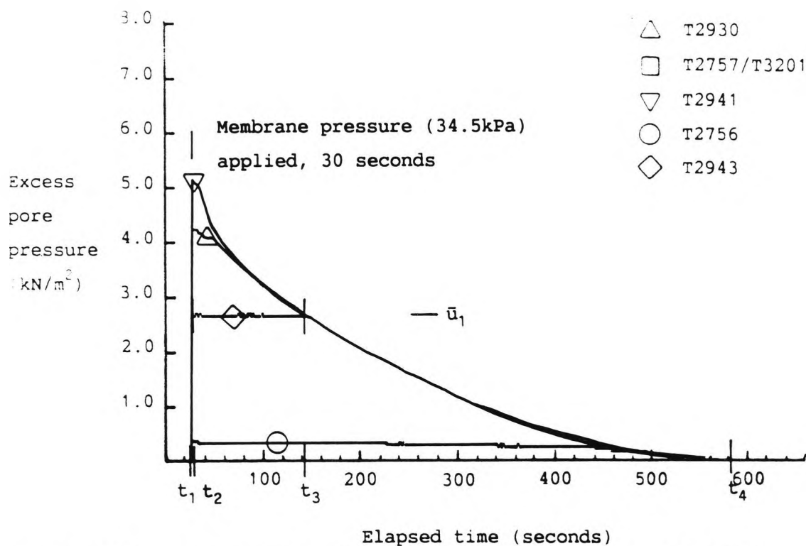
Figure 6.22 An example of a Class I (expanding membrane probe) excess pore pressure response, test 132 (The results of this test are summarised in Table 6.16)
