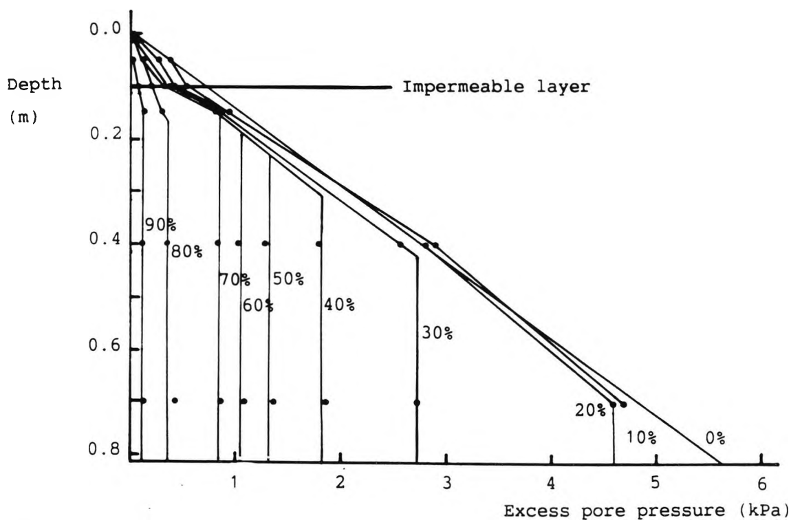
Figure 7.16 Excess pore pressure dissipation recorded in test 182-185, 1540 sec to 2000 sec
