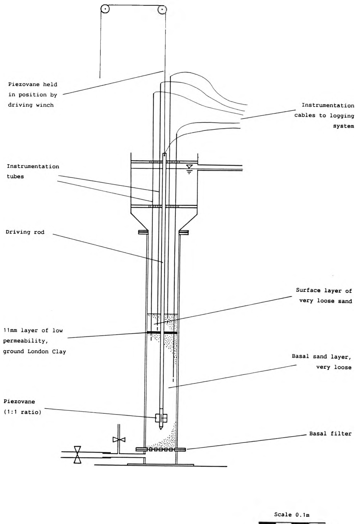
Figure 5.3 Configuration of sand column test 182 - 185 (cross- section)
