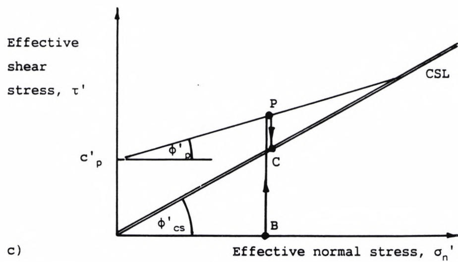
Figure 2.2 State paths for drained shear tests
