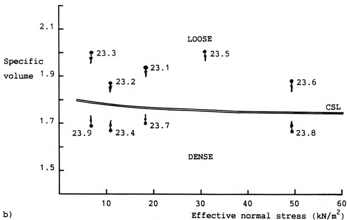
Figure 7.1 Wet and dry soil states, drained behaviour
