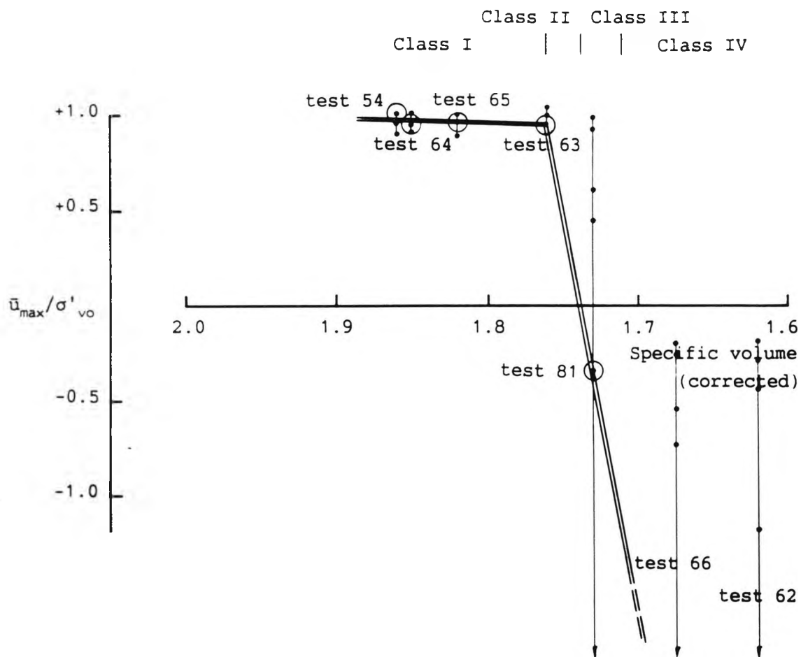
Figure 7.23 Excess pore pressure - specific volume for 60° cone
