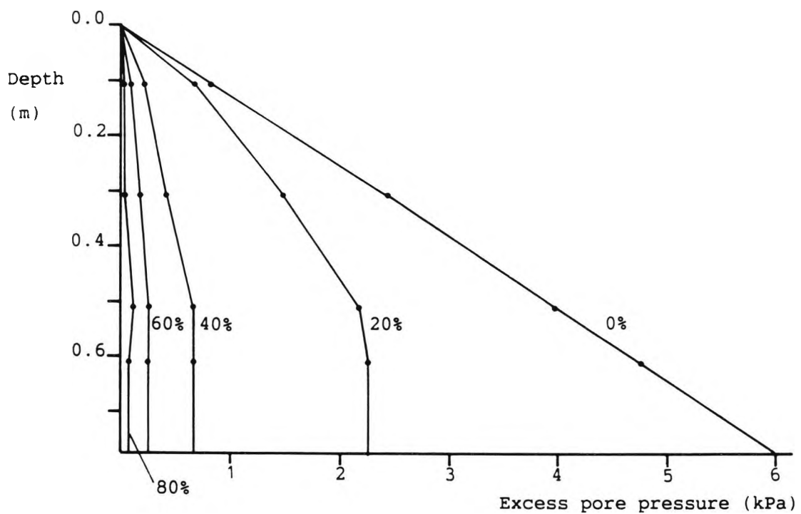
Figure 7.8 Excess pore pressure dissipation recorded in test 136
