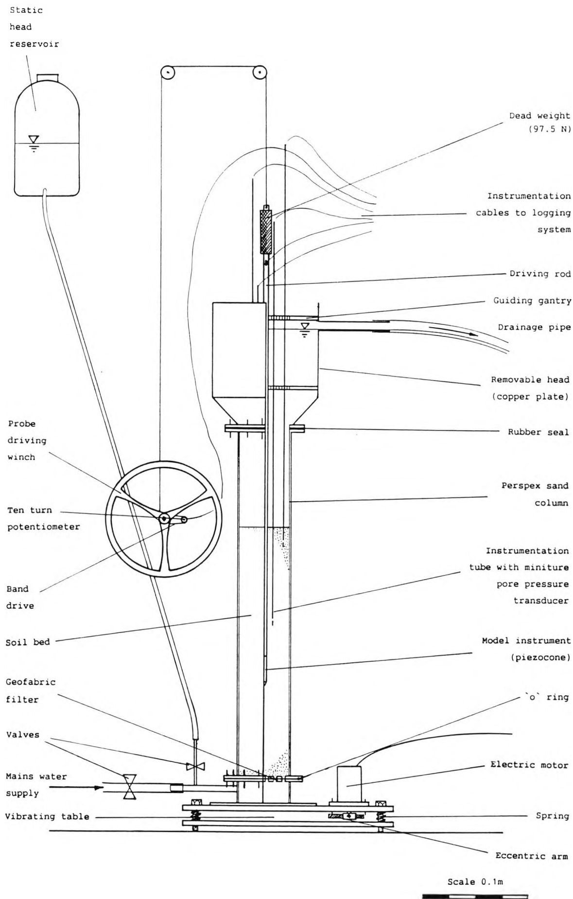
Figure 4.1 Sand column apparatus (half-section)
