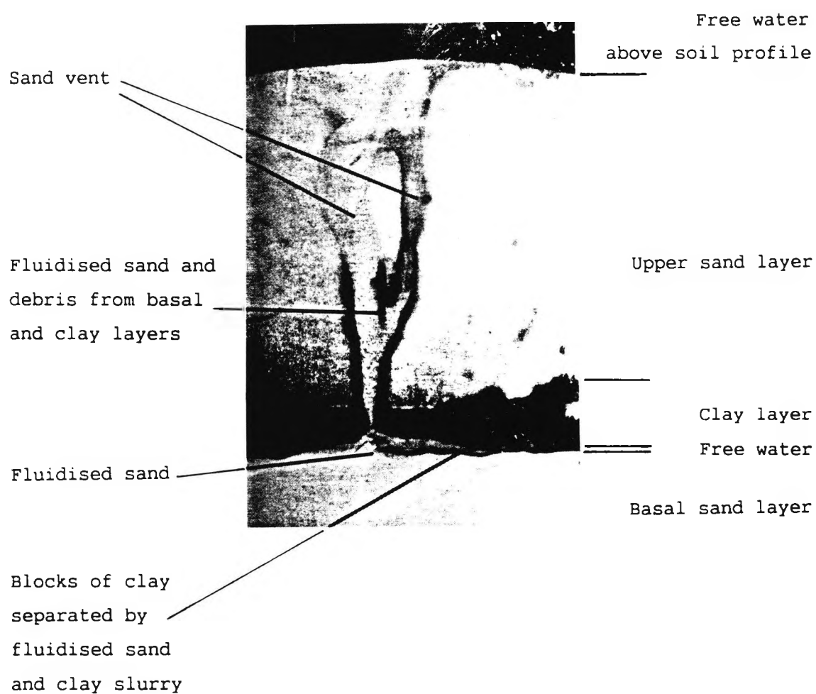
Figure 6.11 Soil profile at the end of test 182 - 185
