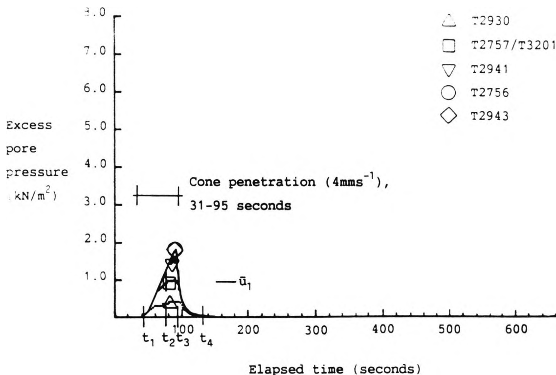
Figure 6.28 An example of a Class II (cone) excess pore pressure response, test 88
