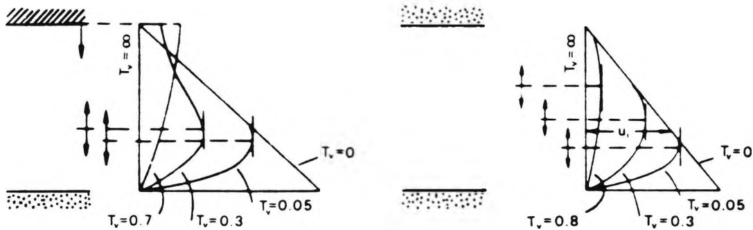
c) Isochrones of excess pore pressure for one-way drainage towards base
