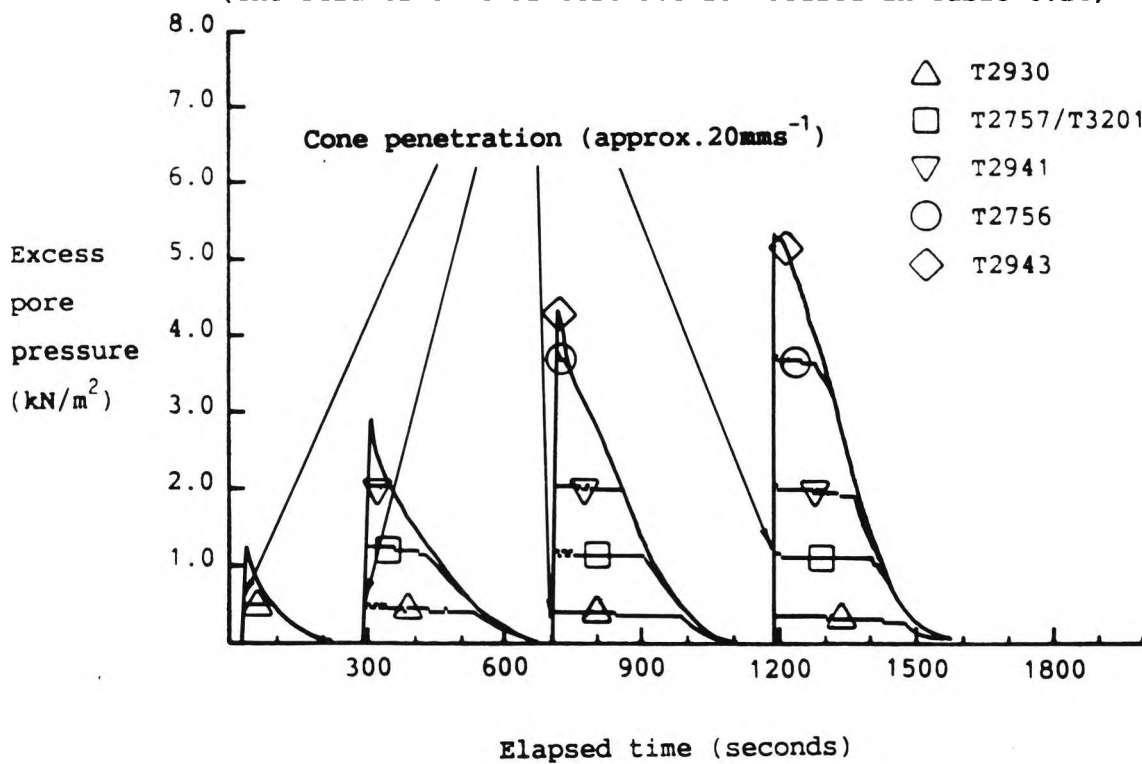
Figure 6.30 An example of a Class IV (cone) excess pore pressure response, test 75
