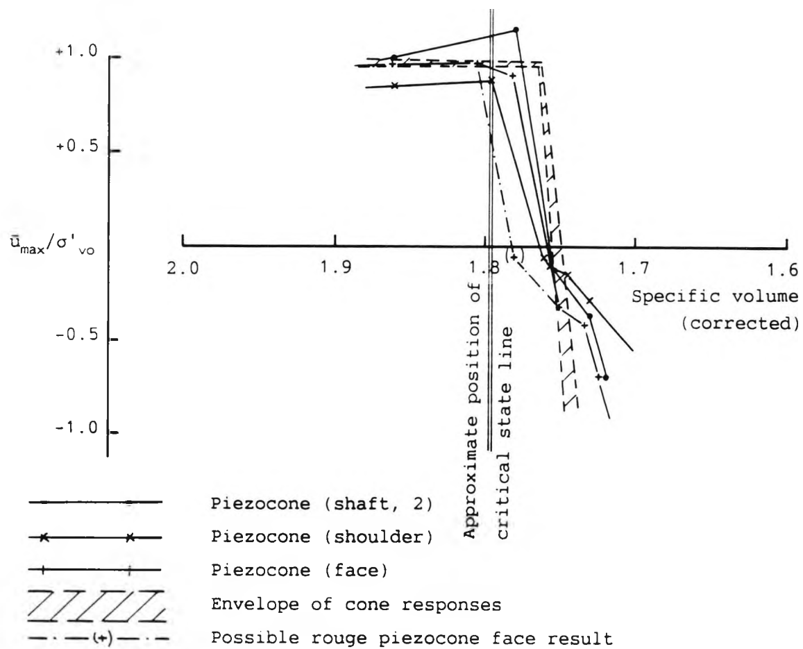
Figure 7.38 Excess pore pressure - specific volume for 60° piezocone
