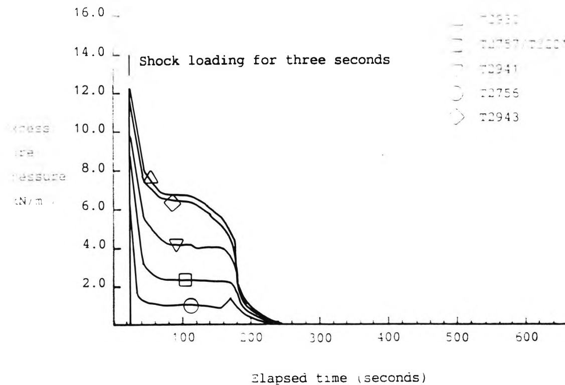
Figure 6.6 Excess pore pressure response recorded in test 186
