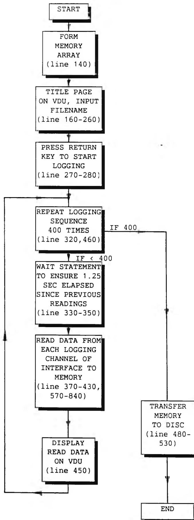
Figure B.3 Flow chart of test logging programs UDISLO5 and PEN2
