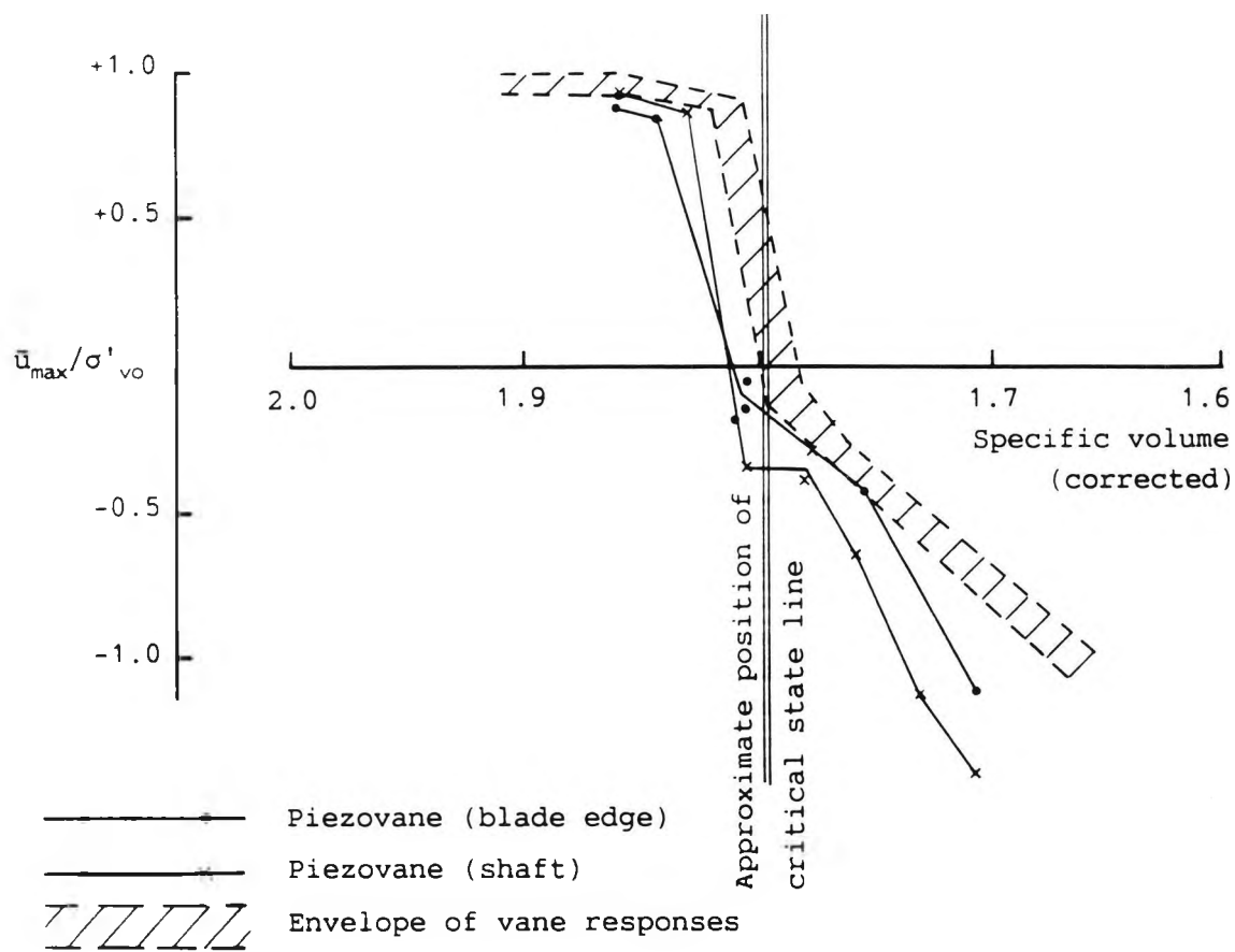
Figure 7.37 Excess pore pressure - specific volume for 1:1 ratio piezovane
