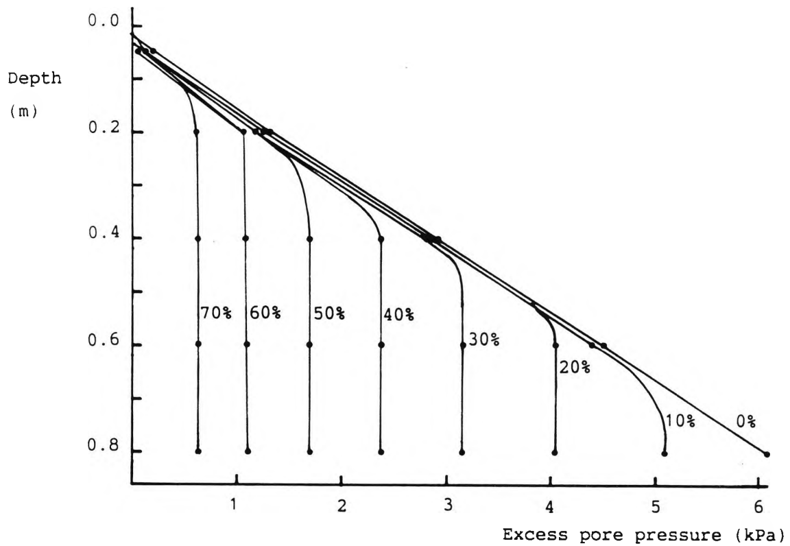
Figure 7.12 Excess pore pressure dissipation recorded in test 42
