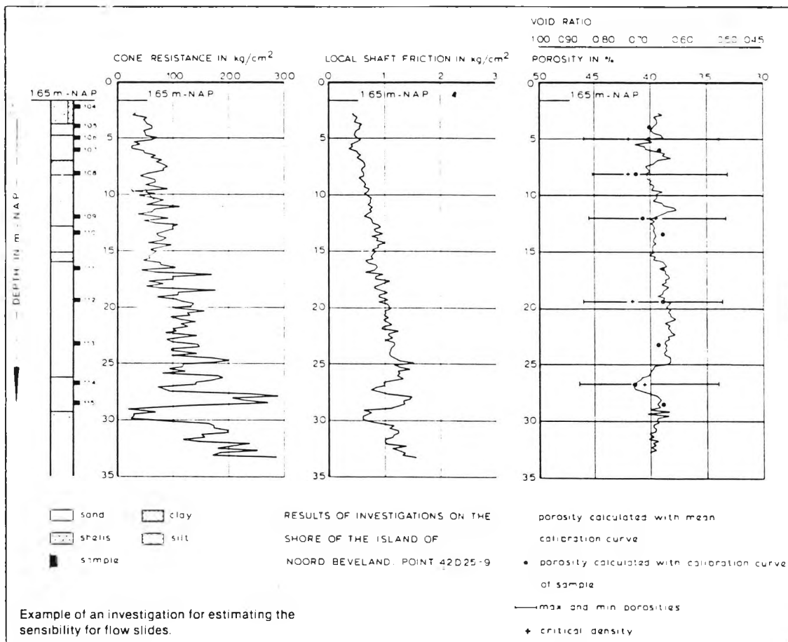
Figure 3.2 Example of results of an investigation to assess the sensitivity of Dutch coastal deposits to flow slide failure (after Delft, 1984)
