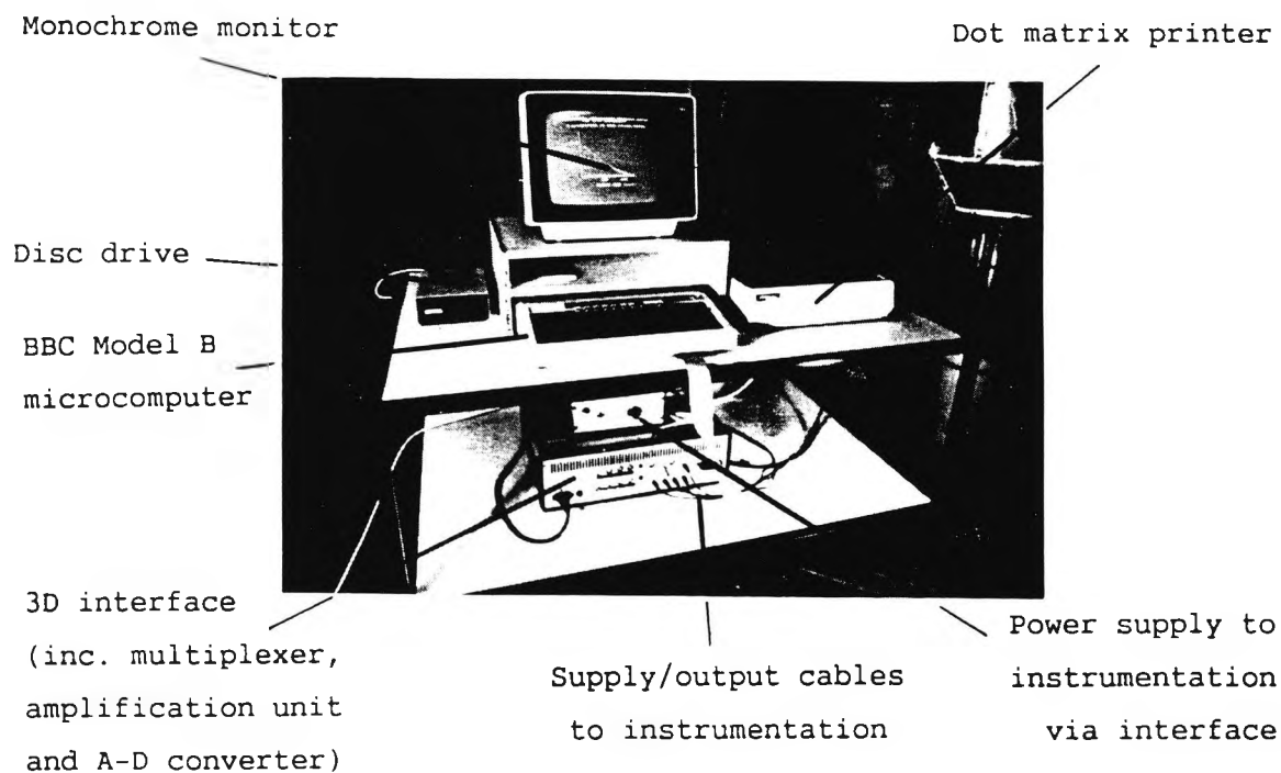
Figure 4.7 Computer controlled data logging system
