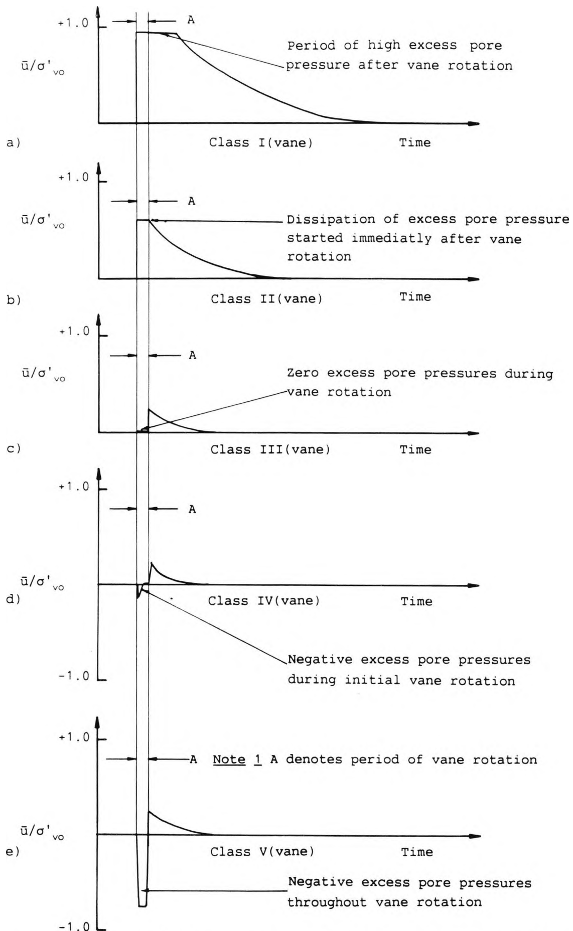
Figure 7.18 Schematic sketches of excess pore pressures recorded during vane tests
