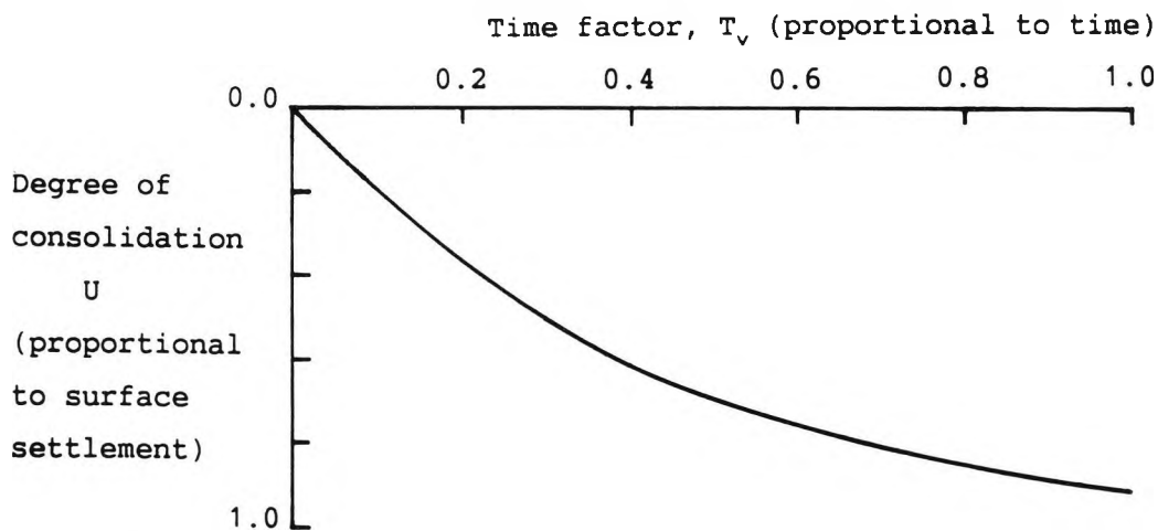
b) Surface settlement with time
