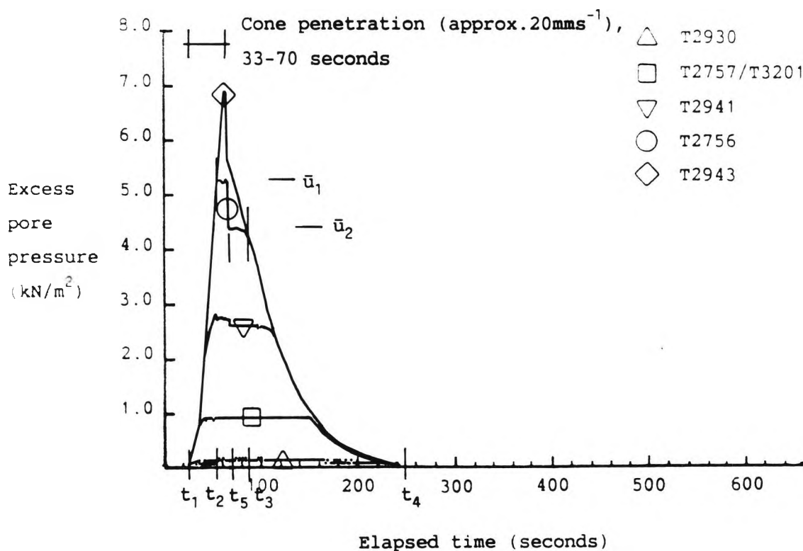
Figure 6.26 An example of a Class Ia (cone) excess pore pressure response, test 63
