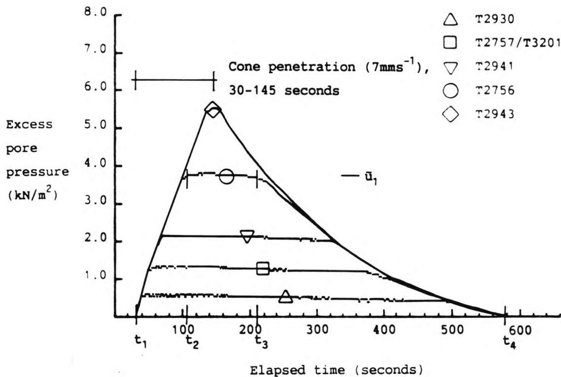
Figure 6.25 An example of a Class I (cone) excess pore pressure response, test 57
