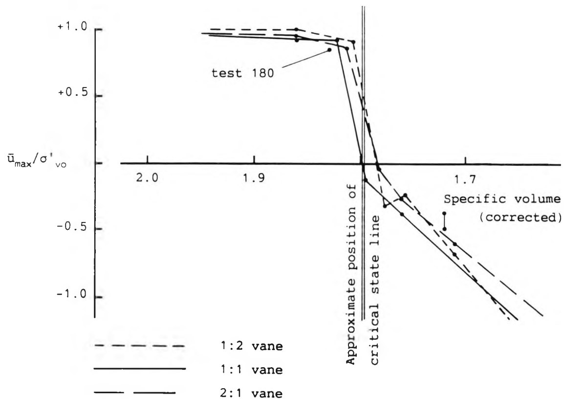
Figure 7.34 Excess pore pressure - specific volume for various vane geometries
