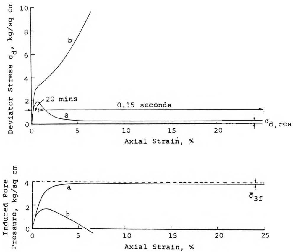
Figure 3.17 Critical void ratio approach, typical test date (after Castro, 1969)
