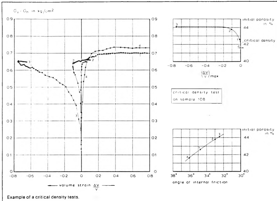
Figure 3.18 An example of test data to define a soil's critical density (after Delft, 1984)
