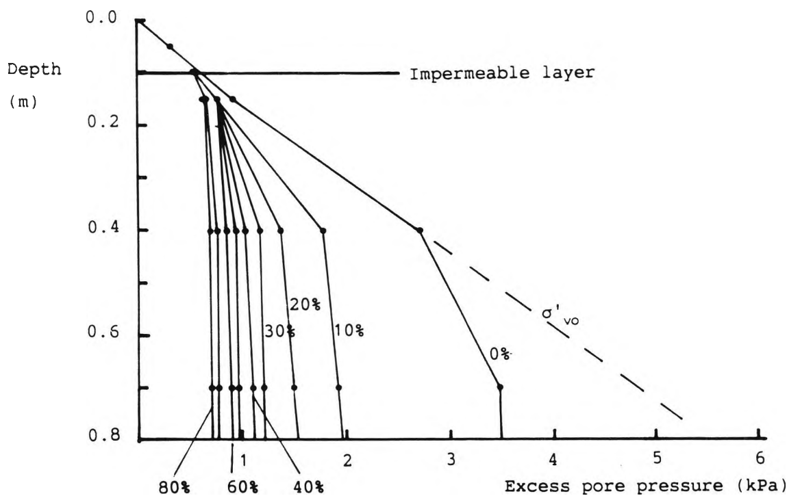
Figure 7.17 Excess pore pressure dissipation recorded in test 182-185, 1480 sec to 1530 sec
