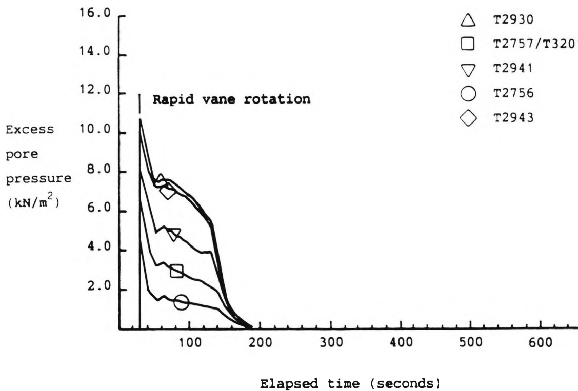
Figure 6.5 Excess pore pressure response recorded in test 181
