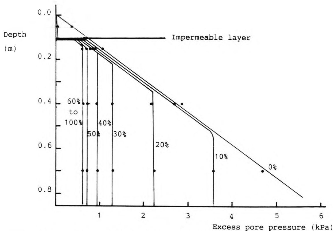
Figure 7.15 Excess pore pressure dissipation recorded in test 182-185, 20 sec to 400 sec
