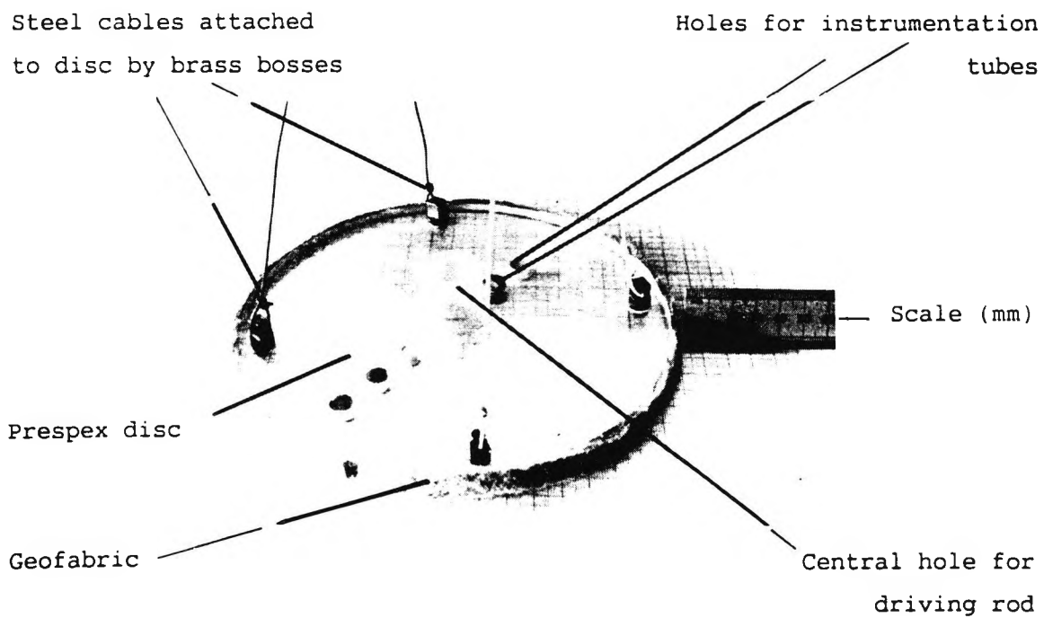
Figure 4.5 Surchage disc
