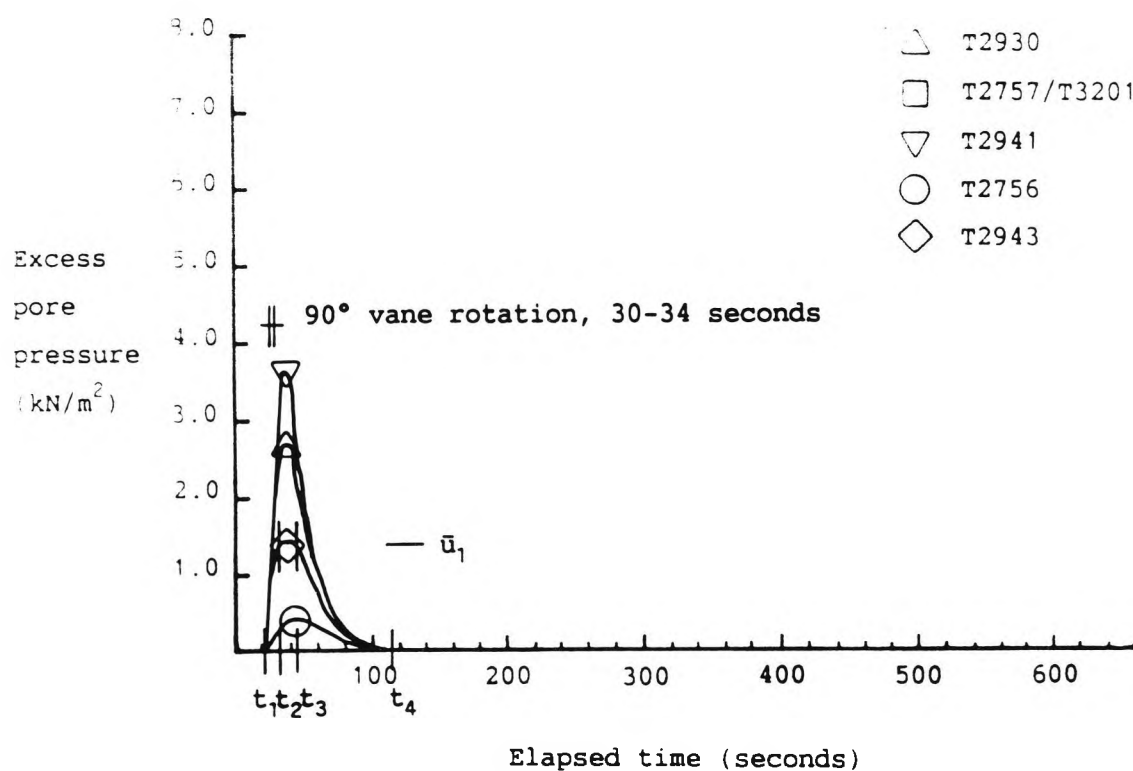
Figure 6.14 An example of a Class II (vane) excess pore pressure response, test 117
