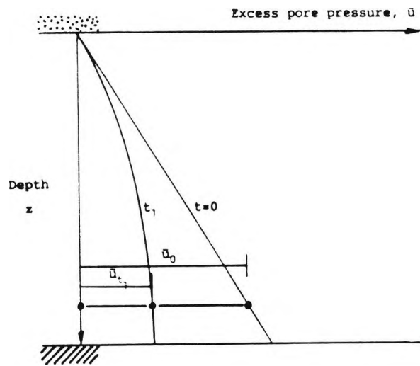
a) Isochrones of excess pore pressure for one-way drainage towards surface (after Dwyer, 1986)
