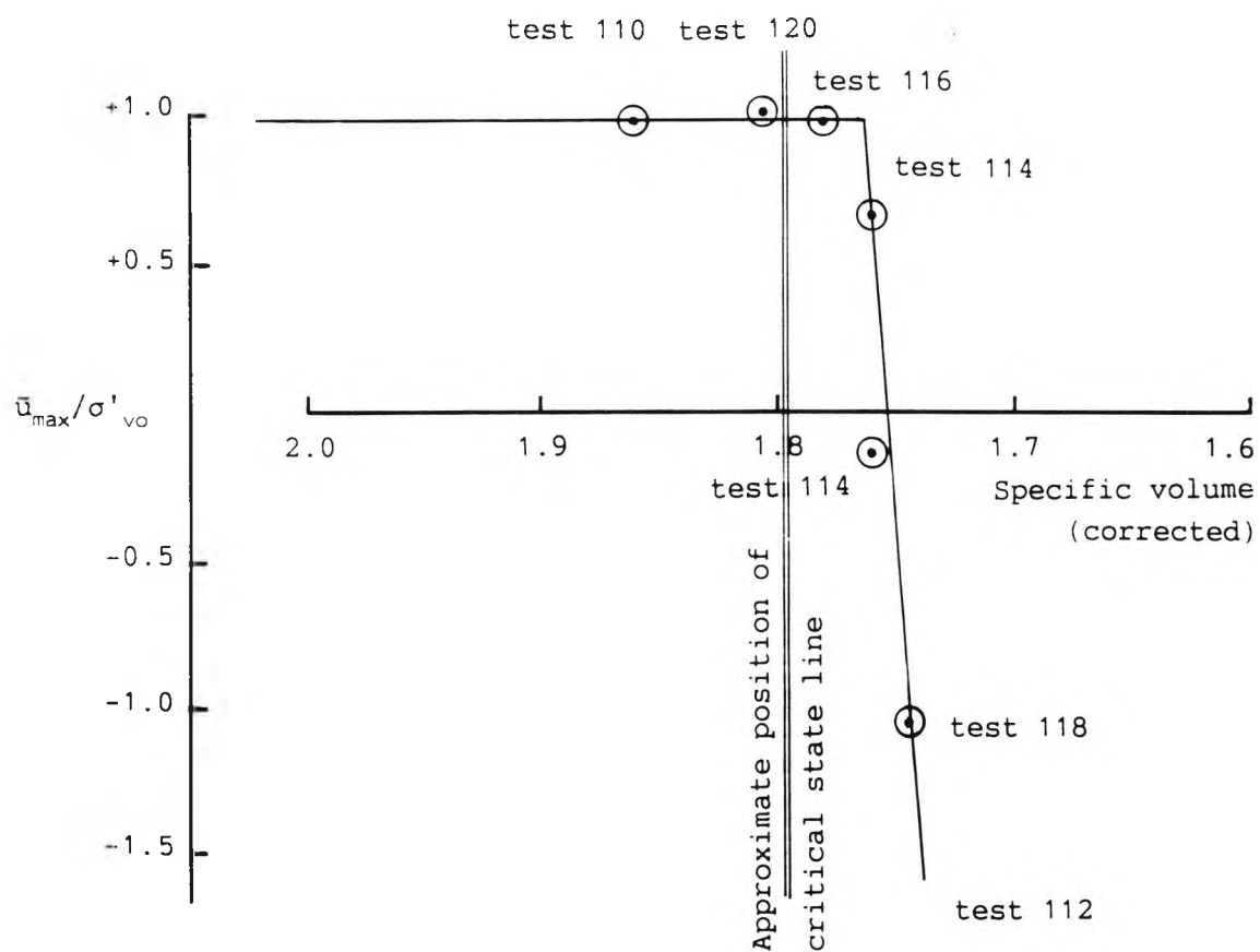
Figure 7.39 Excess pore pressure - specific volume for 1:1 ratio vane driven into soil beds at approximately 20\text{mm s}^{-1}
