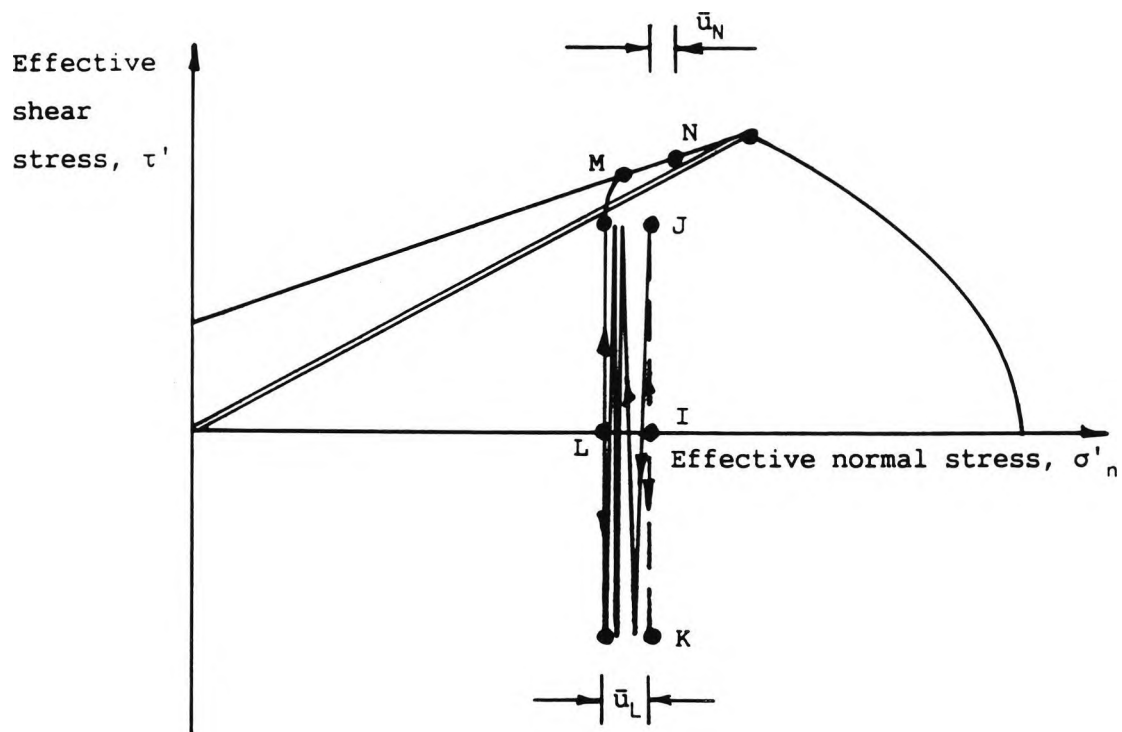
b) Cyclic loading of a dry of critical soil state
