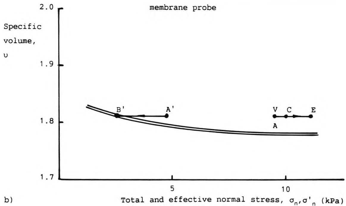
Figure 7.24 Assumed undrained stress paths for model instruments loading soil initially wet of critical
