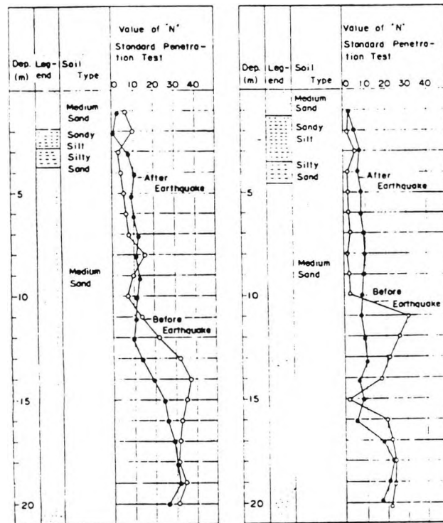
Figure 3.9 Soil profiles and results of standard penetration test performed near structures showing signs of liquefaction failure, Niigata (after the Japanese Society of Soil Mechanics and Foundation Engineering, 1966)
