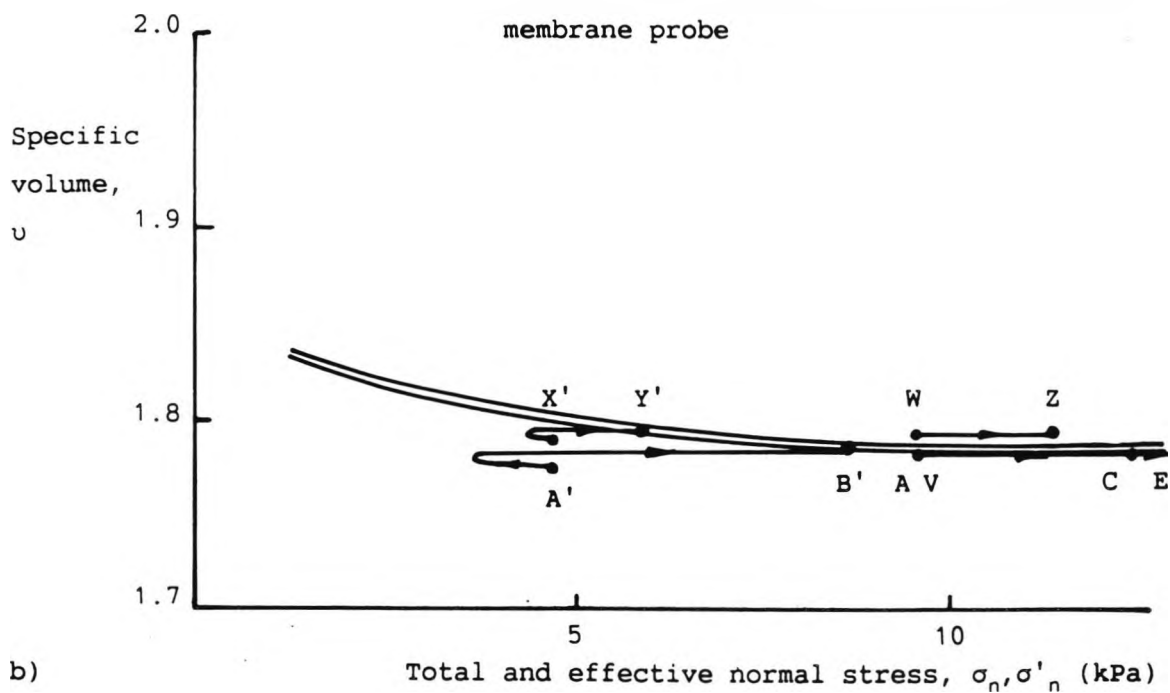
Figure 7.26 Assumed undrained stress paths for model instruments loading soil initially dry of critical
