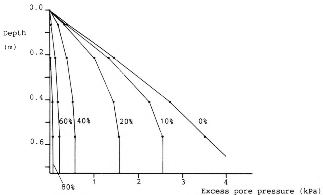
Figure 7.7 Excess pore pressure dissipation recorded in test 117
