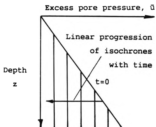
c) Isochrones of excess pore pressure within a resedimenting soil bed
