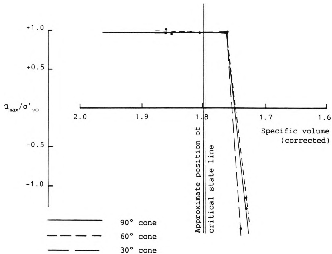
Figure 7.36 Excess pore pressure - specific volume for various cone geometries
