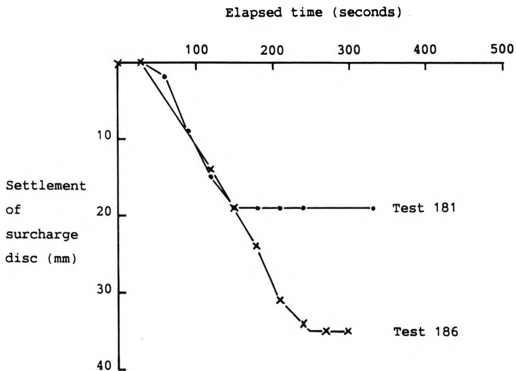
Figure 6.7 Settlement of surcharge disc recorded in tests 181 and 186
