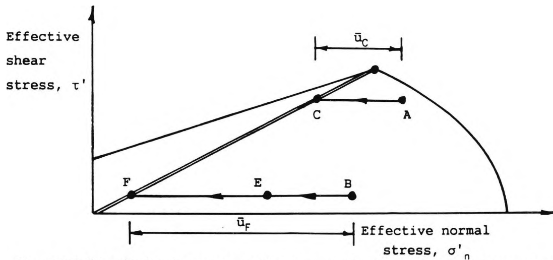
Figure 2.6 Liquefaction at large effective stresses
