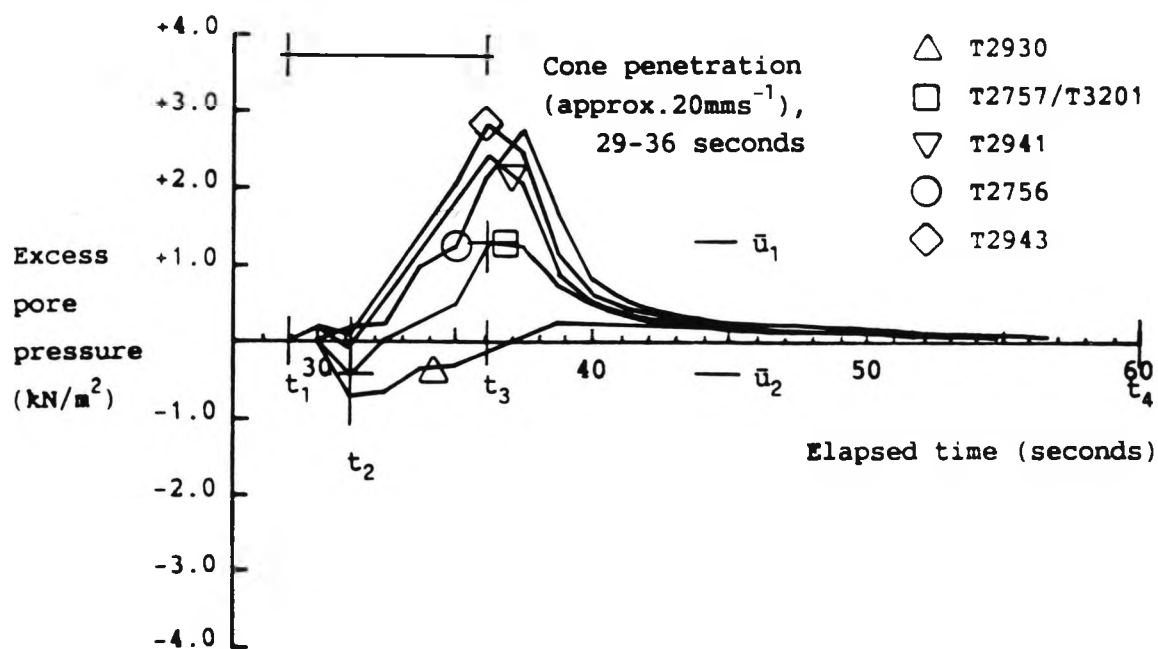
Figure 6.28 An example of a Class II (cone) excess pore pressure response, test 88
