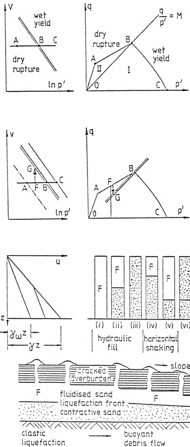
Figure 3.19 A model of soil profile liquefaction (after Schofield, 1981)
