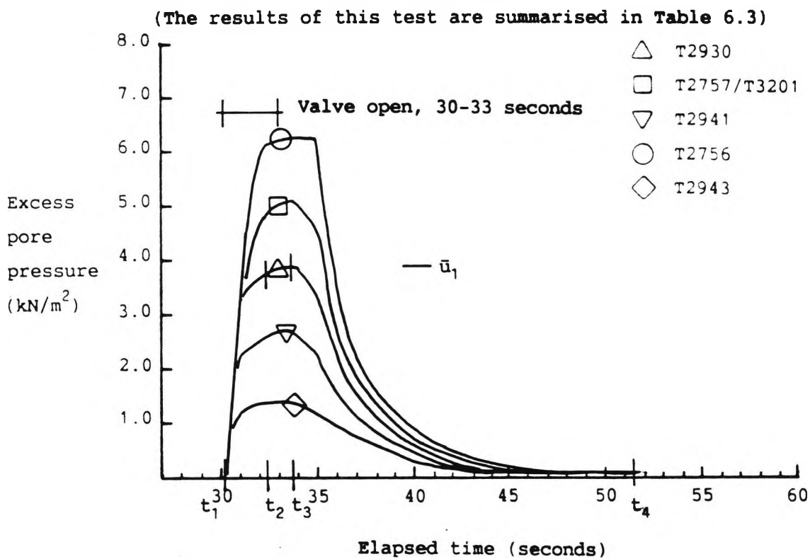
Figure 6.1 An example of a Class I excess pore pressure response, test 42
