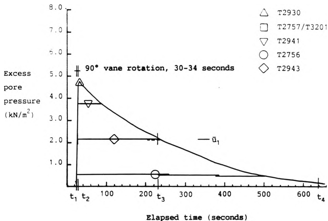
Figure 6.12 An example of a Class I (vane) excess pore pressure response, test 100 (The results of this test are summarised in Table 6.7)
