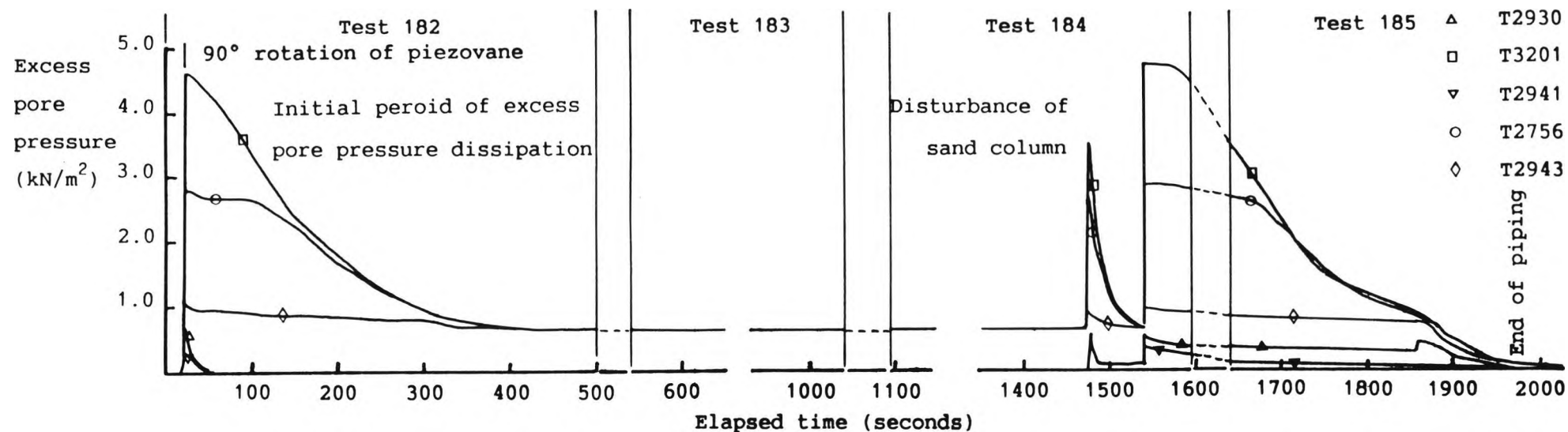
Figure 6.8 Excess pore pressures recorded in test 182 - 185
