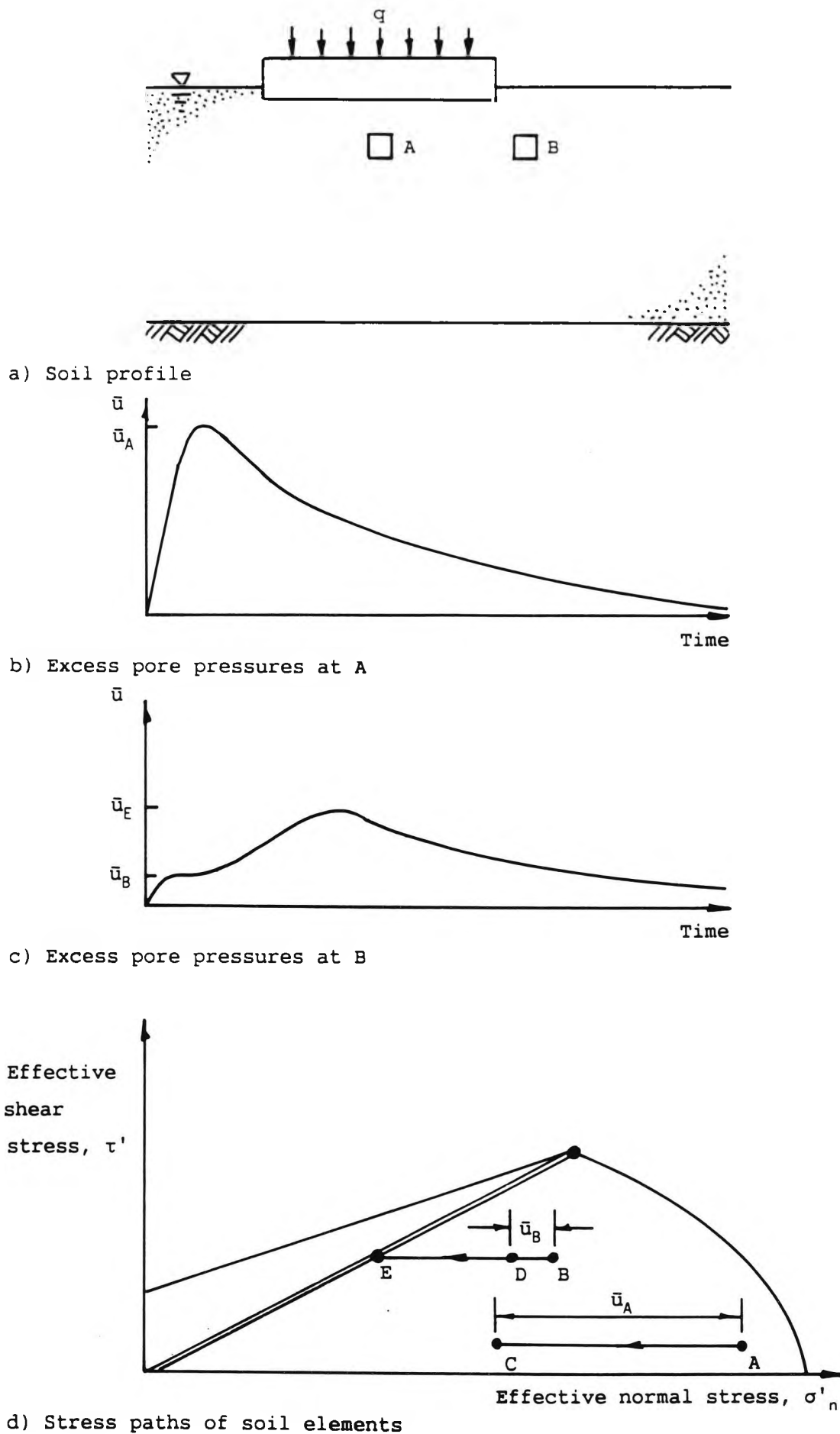
Figure 2.8 Liquefaction beneath a structure
