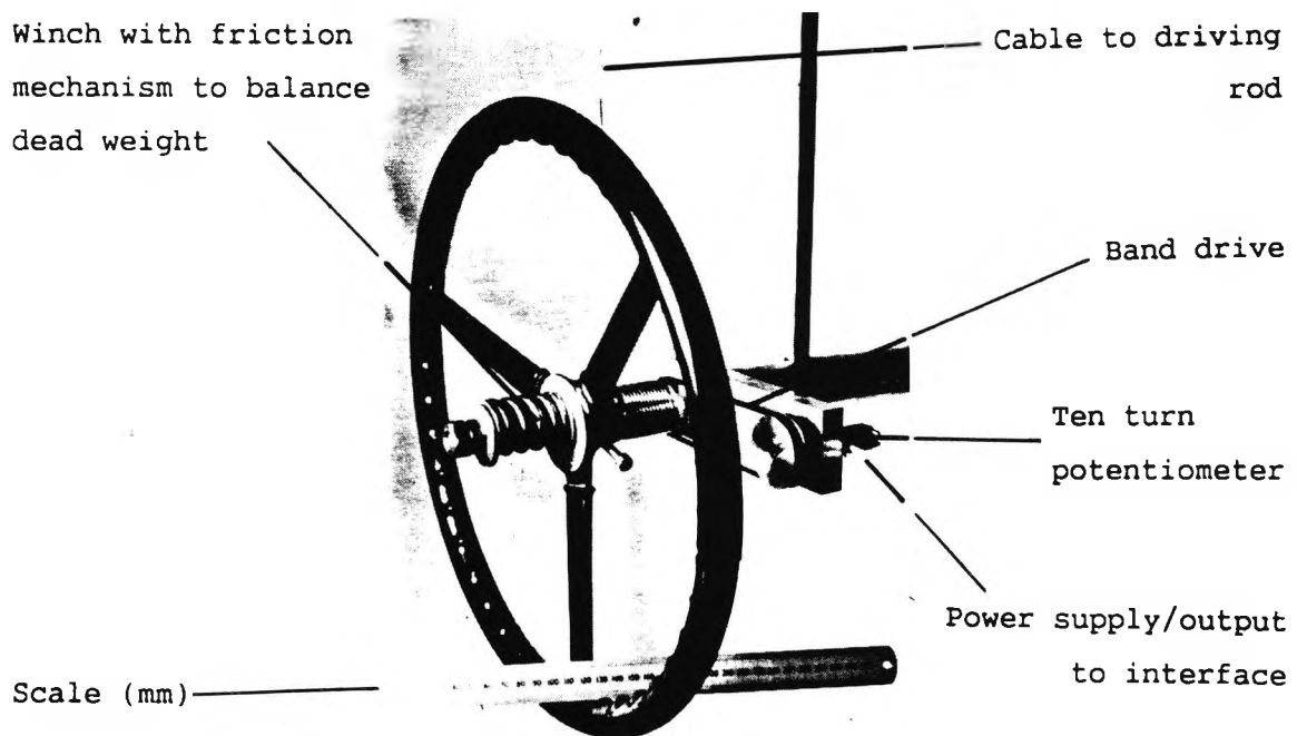
Figure 4.9 Cone driving mechanism
