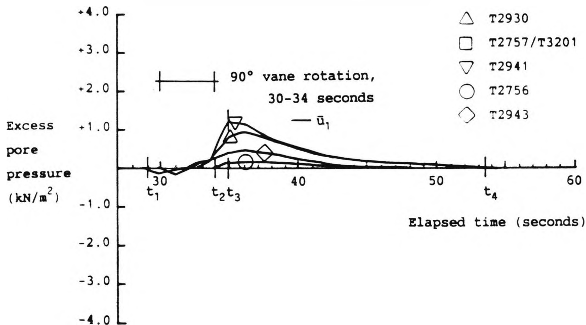
Figure 6.14 An example of a Class II (vane) excess pore pressure response, test 117
