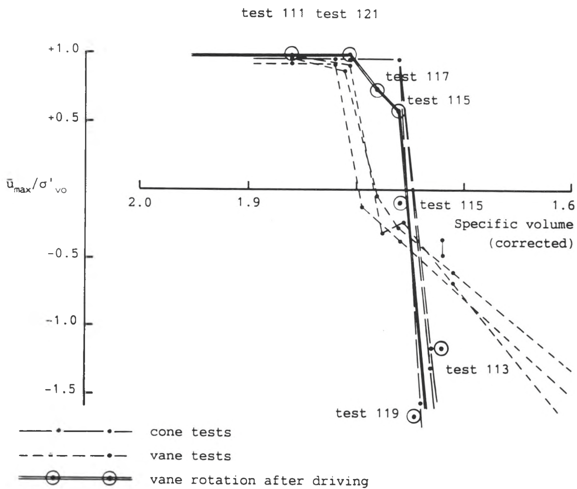
Figure 7.40 Excess pore pressure - specific volume for 1:1 ratio vane rotated in a soil bed after installation by driving
