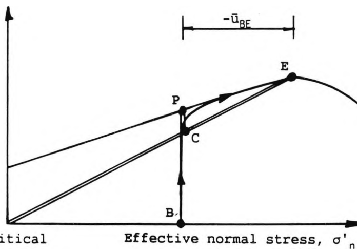
Figure 2.4 Wet and dry of critical soil behaviours
