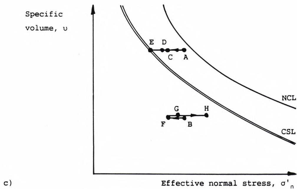
Figure 2.5 Types of soil failure due to increased pore pressures
