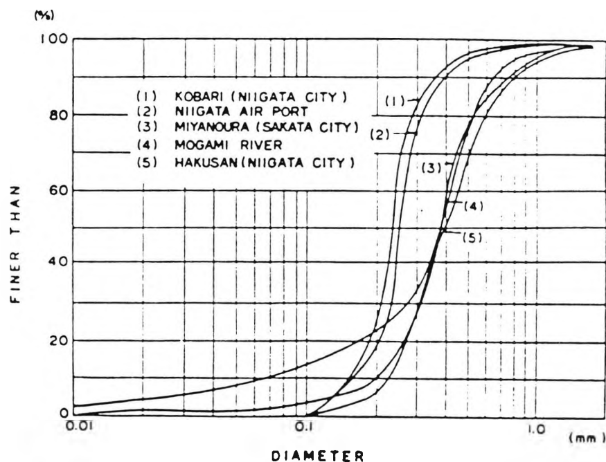
Figure 3.7 Range of particle size distribution curves for soils associated with liquefaction failures at Niigata, 1964 (after the Japanese Society of Soil Mechanics and Foundation Engineering, 1966)
