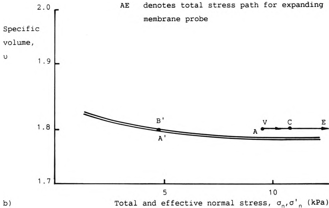
Figure 7.25 Assumed undrained stress paths for model instruments loading soil initially beneath the critical state line
