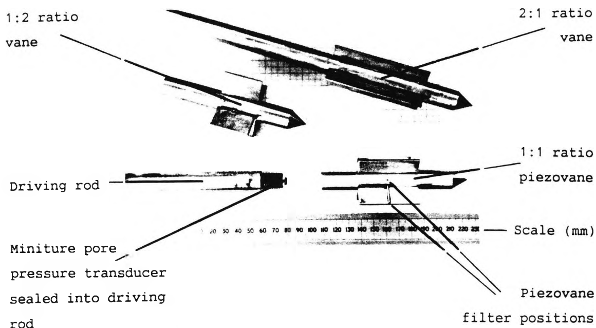
Figure 4.10 Vanes and piezovanes
