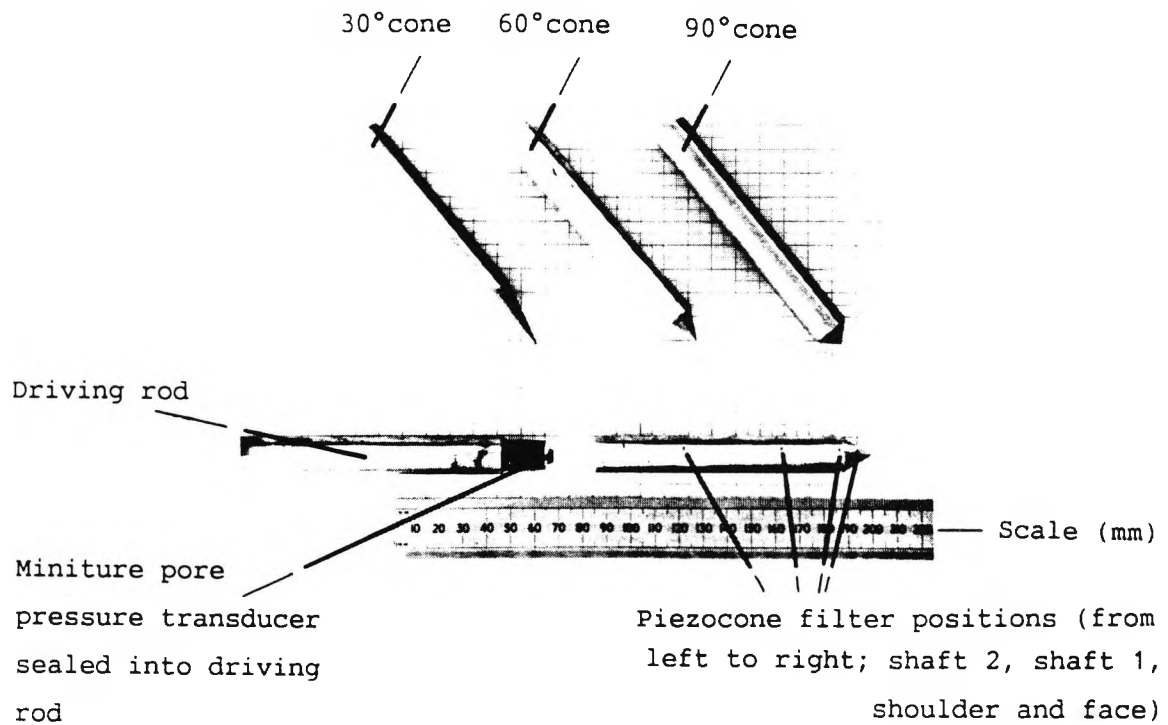
Figure 4.8 Cones and piezocones
