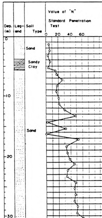
Figure 3.10 Soil profile at Hakusan transformer substation, Niigata (after the Japanese Society of Soil Mechanics and Foundation Engineering, 1966)
