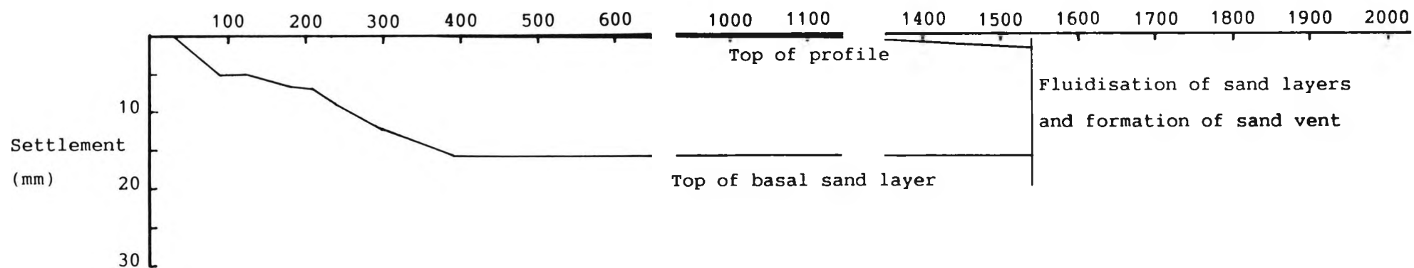
Figure 6.9 Observations of settlement recorded in test 182 - 185
