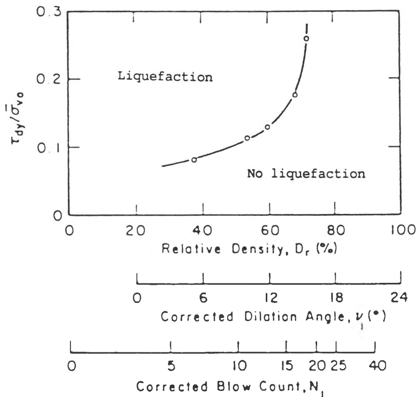
Figure 3.27 Proposed correlation between liquefaction potential and dilation angle (after Vaid et al, 1981)
