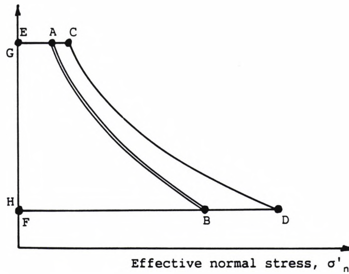
Figure 2.3 The state boundary surface
