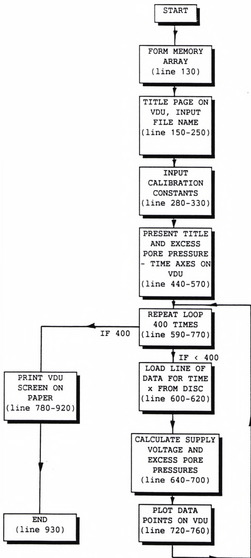
Figure B.9 Flow chart of preliminary data plotting program UDISPR5
