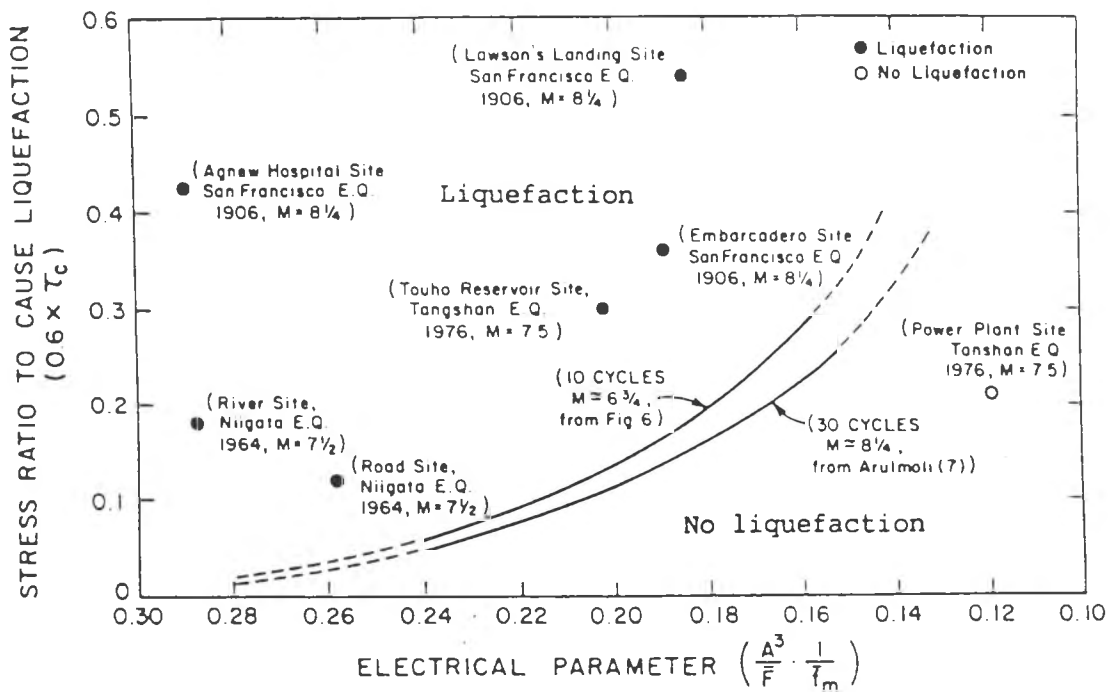
Figure 3.26 Summary of field test results for the electrical resistivity method (after Arulmoli et al, 1981)
