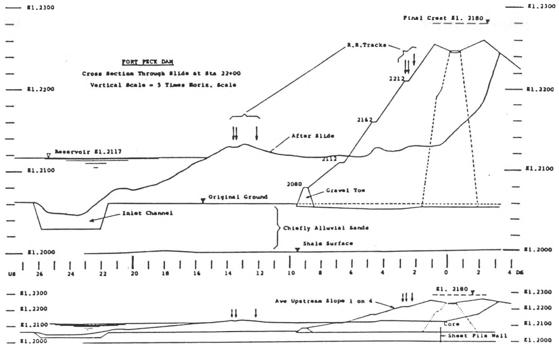
Figure 3.11 Section through Fort Peck Dam before and after partial collapse, 1938 (after Casagrande, 1975)
