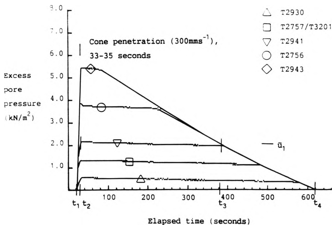
Figure 6.24 An example of a Class I (cone) excess pore pressure response, test 56
