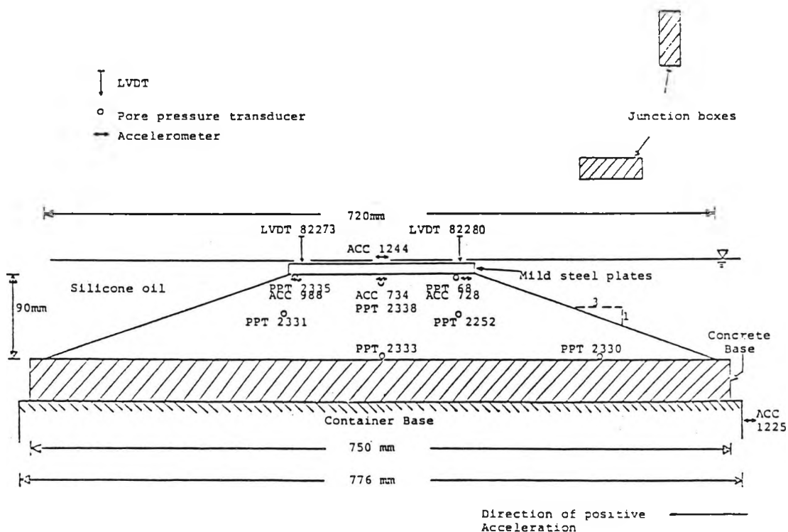
Figure 3.22 Configuration of a centrifuge test on a model island subjected to a simulated earthquake (Test FHL02C) (after Lee and Schofield, 1984)
