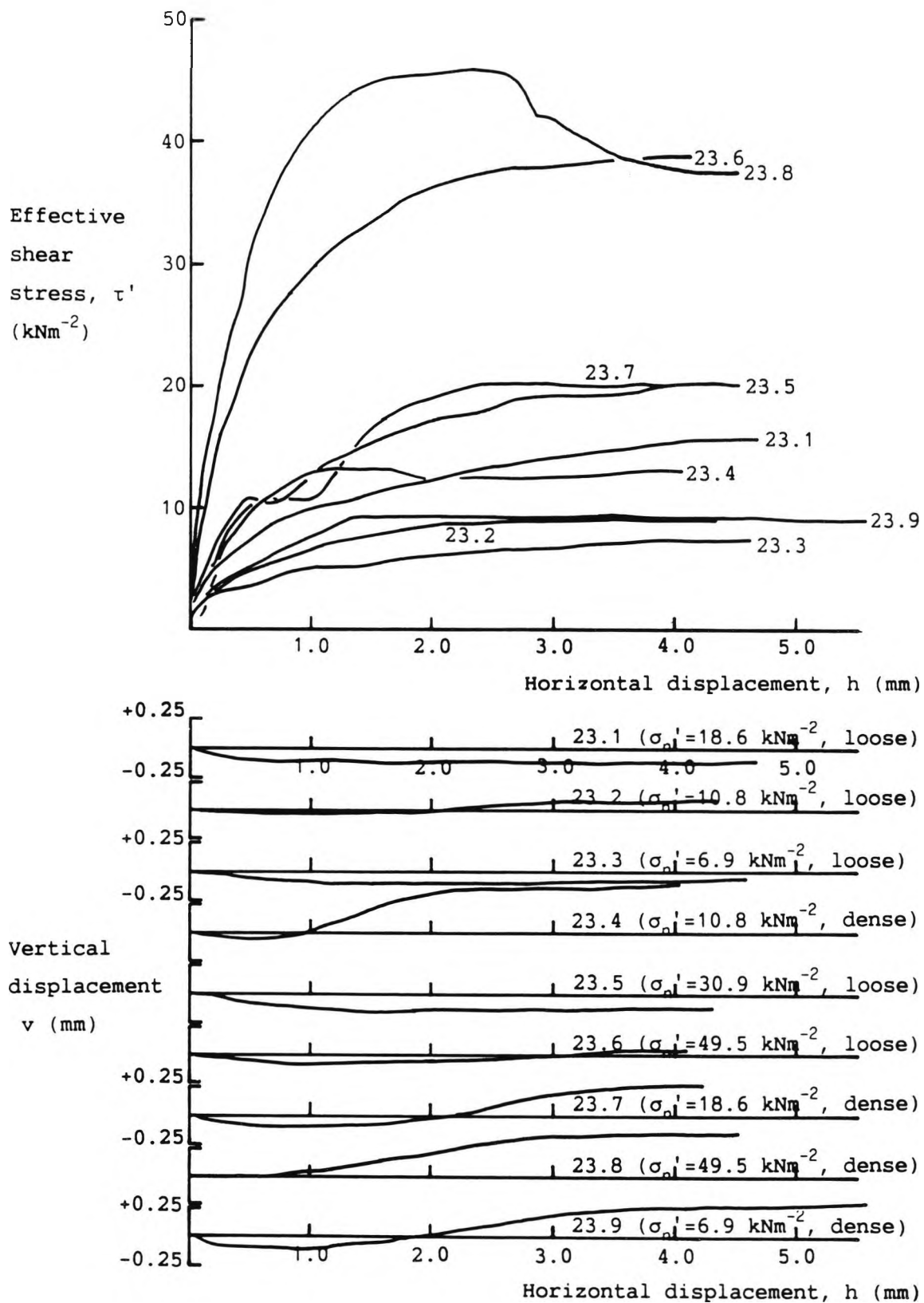
Figure A.2 Direct shear tests with soil 23
