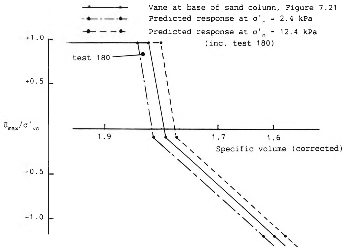
Figure 7.35 Predicted effect of stress level upon excess pore pressures recorded in vane tests
