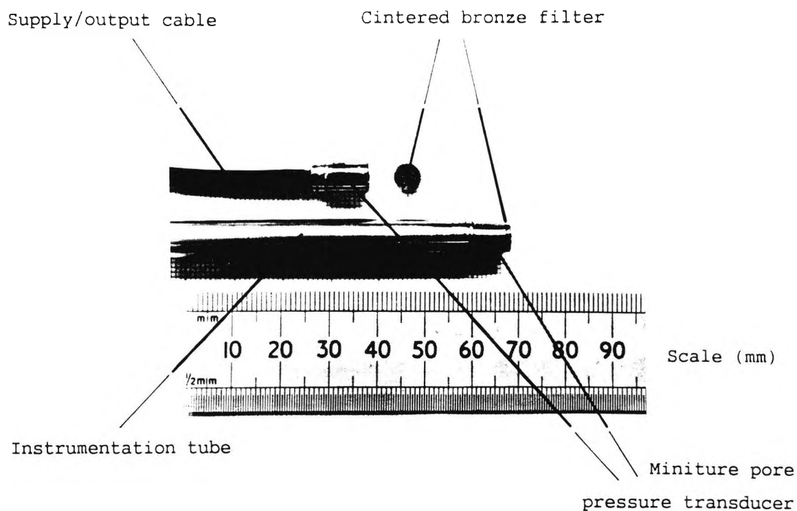
Figure 4.6 Instrumentation tube and miniature pore pressure transducer
