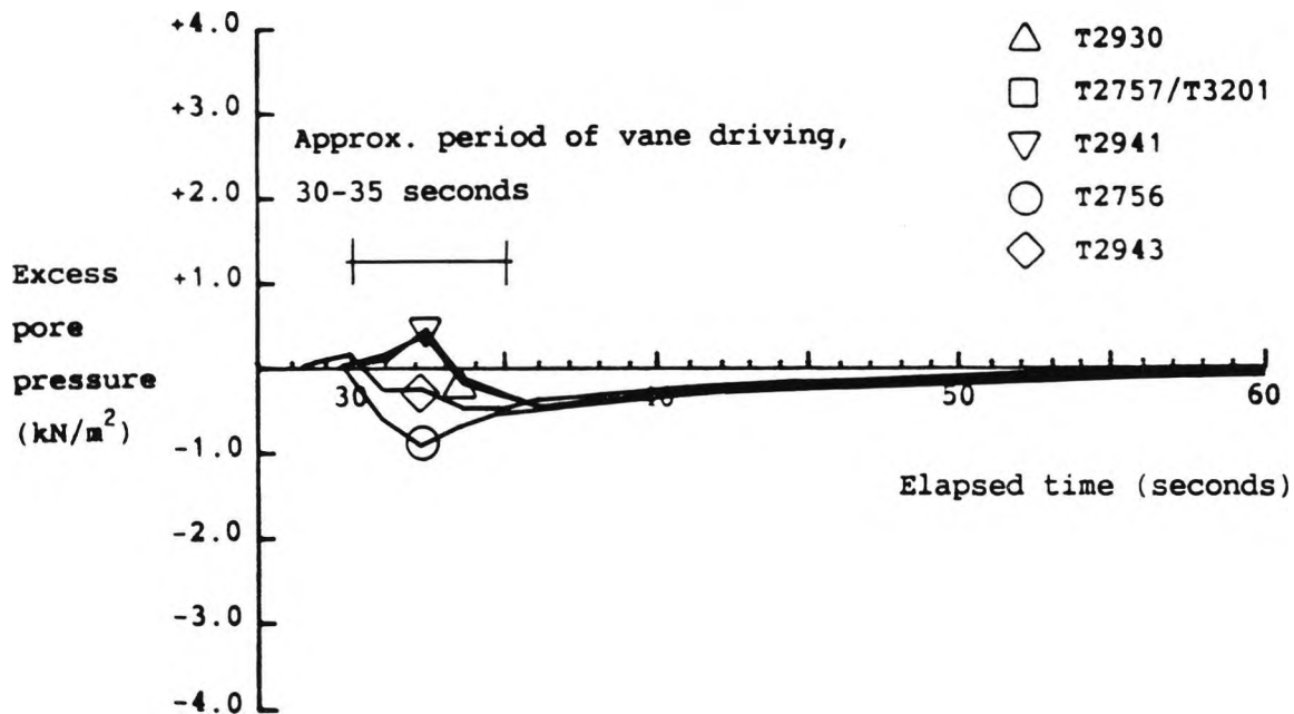
Figure 6.18 A Class III (cone) excess pore pressure response recorded in vane test 114
