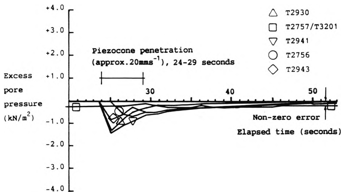
Figure 6.32 Excess pore pressure response recorded in test 70 (The results of this test are summarised in Table 6.18)
