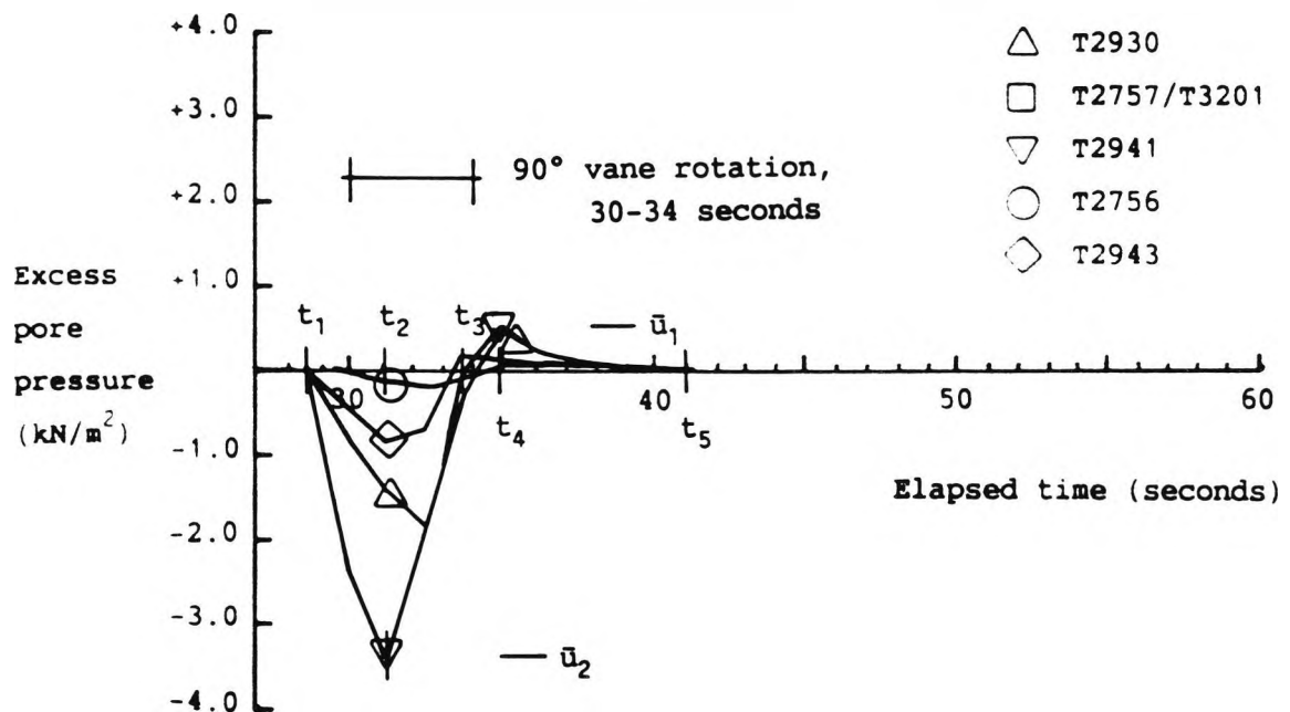
Figure 6.16 An example of a Class IV (vane) excess pore pressure response, test 95
