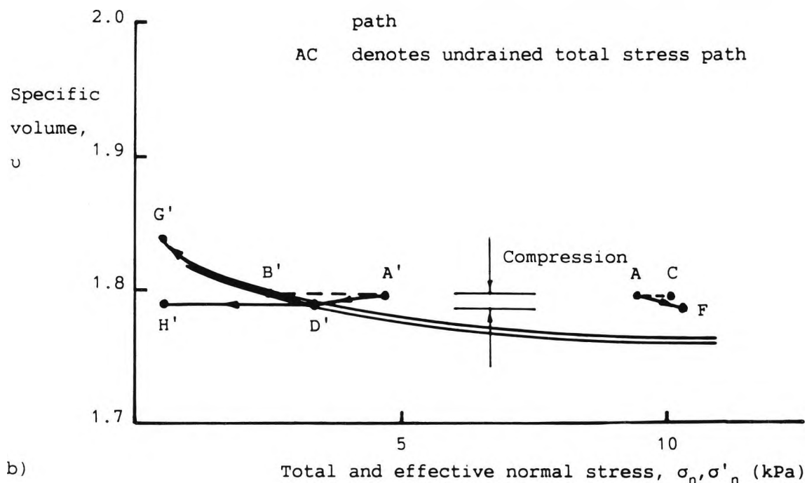
Figure 7.33 Assumed locally drained stress paths for a cone loading soil initially wet of critical
