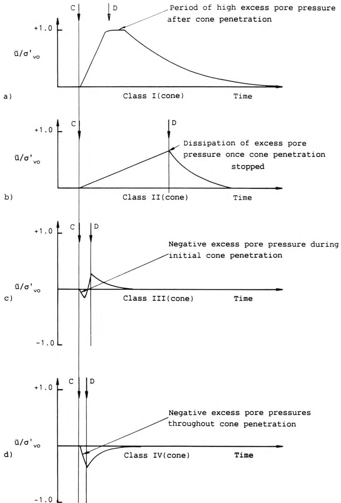
Figure 7.20 Schematic sketches of excess pore pressures recorded during cone tests
