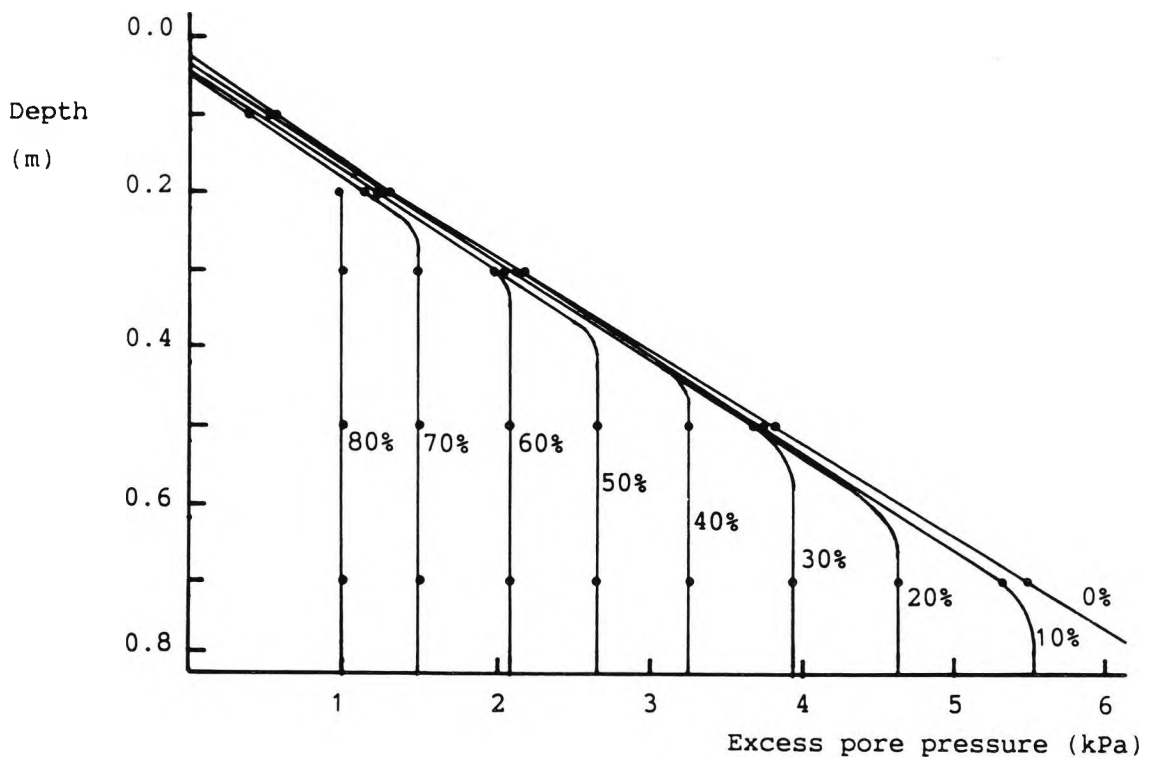
Figure 7.13 Excess pore pressure dissipation recorded in test 56 Note 1 In Figures 7.12 and 7.13 isochrones are for percentage time to full excess pore pressure dissipation, and not average degree of consolidation.
