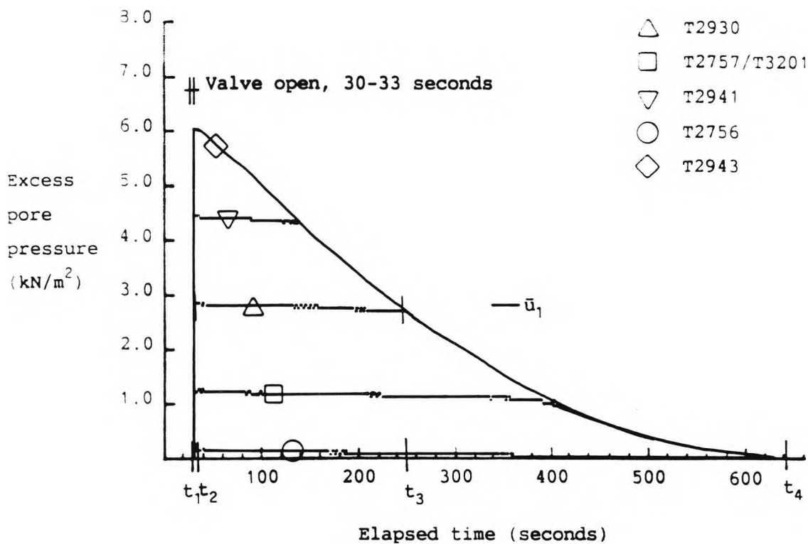
Figure 6.1 An example of a Class I excess pore pressure response, test 42
