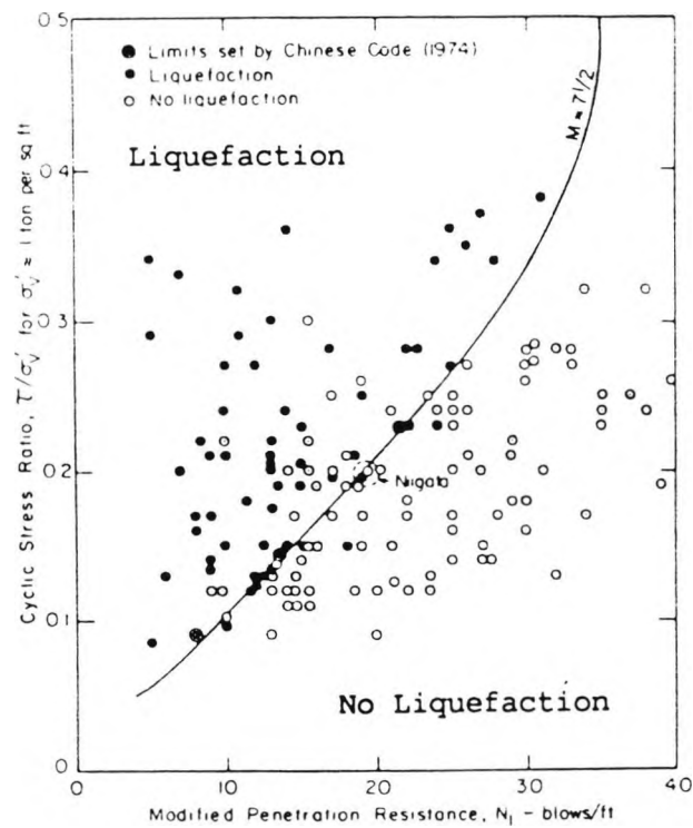
Figure 3.24 Data adopted to define the design curve for sands ( D_{50} > 0.25 \text{ mm} ) subjected to magnitude 7.5 earthquakes, SPT method (after Seed et al, 1983)
