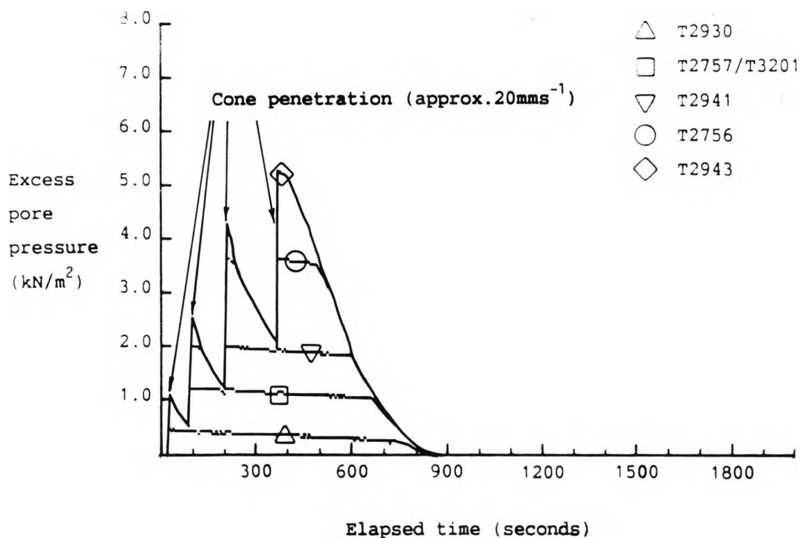
Figure 6.32 Excess pore pressure response recorded in test 70 (The results of this test are summarised in Table 6.18)
