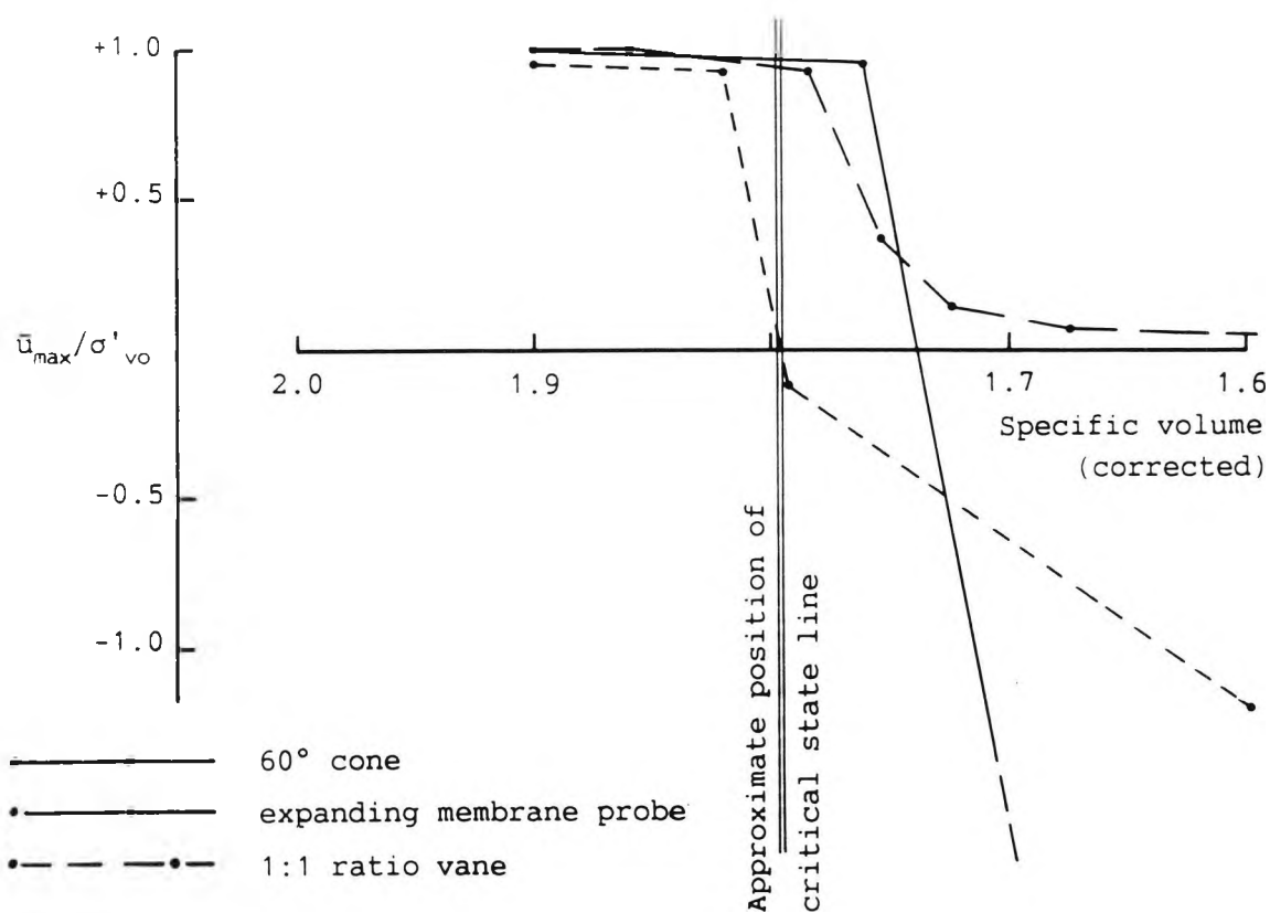
Figure 7.27 Summary plot of excess pore pressure - specific volume for various types of model in situ instruments
