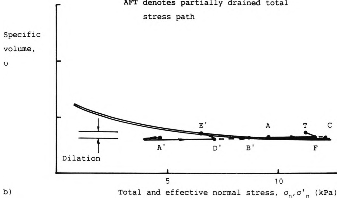
Figure 7.32 Assumed locally drained stress paths for a cone loading soil initially dry of critical
