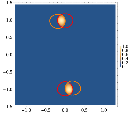
FIG. 2. Intensity plot of the transmission factor (12) in the k_y k_z plane (momenta in units of k_W ) for a zero-energy electron with a potential step V_0 = 0.2 v k_W and tilt angle \theta = 0.2 . The red and orange circles delimit the Fermi surfaces on the two sides of the interface.
