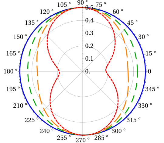
FIG. 9. Polar plot of the splitting angle \cos \chi_s as a function of the azimuthal angle \xi_i for E = 0 , \theta = 0.1 and V_0 = 0.2 v k_W , for various incidence angles: starting from the outer curve and proceeding inwards \chi_i = 0.1 , \chi_i = 0.3 , \chi_i = 0.4 and \chi_i = 0.5 .
