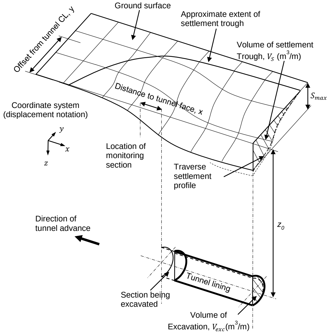
Figure 1. Idealisation of tunnelling induced soil displacement (after Le and Taylor, 2018).
