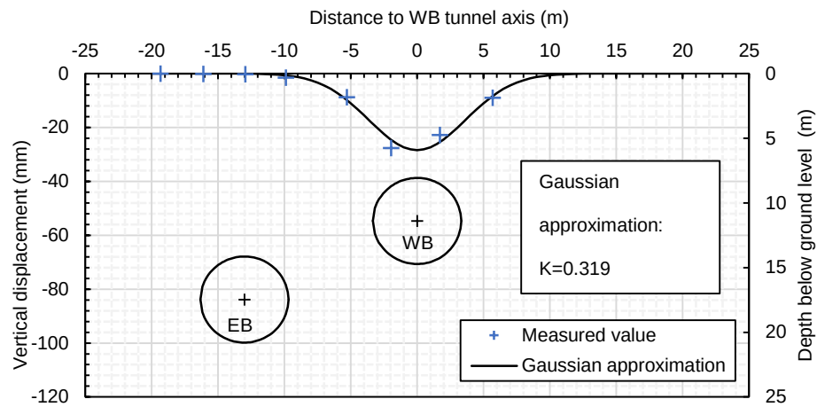
d) Ground surface vertical displacement due to WB tunnel excavation at chainage 1403m
