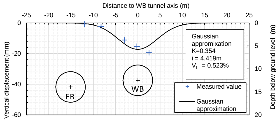
b) Ground surface vertical displacement due to WB tunnel excavation at chainage 1523m
