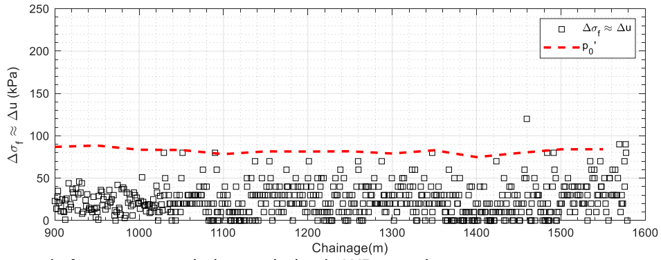
f. Changes in face pressure during each ring in WB tunnel.
