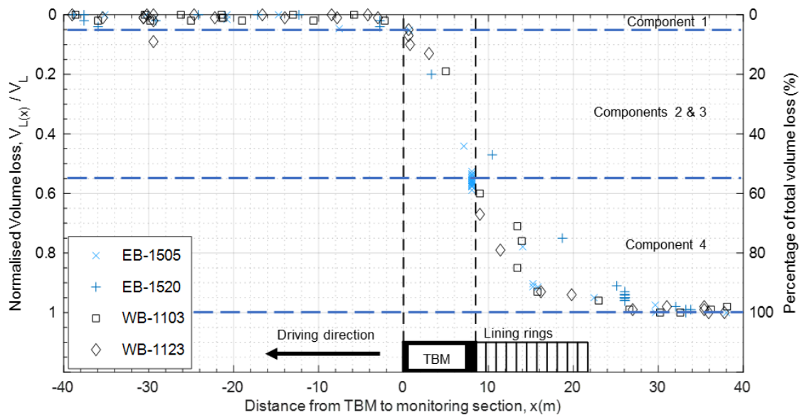
Figure 10. Typical normalised volume losses along the tunnel centre-line
