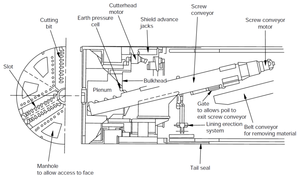
Figure 3. Main components of Earth pressure balance tunnelling machine (Chapman et al., 2018).
