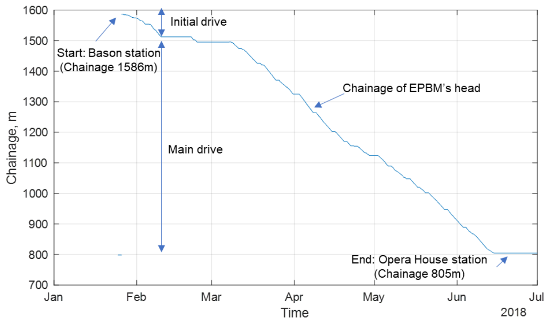
b) TBM advance rate in WB tunnel
