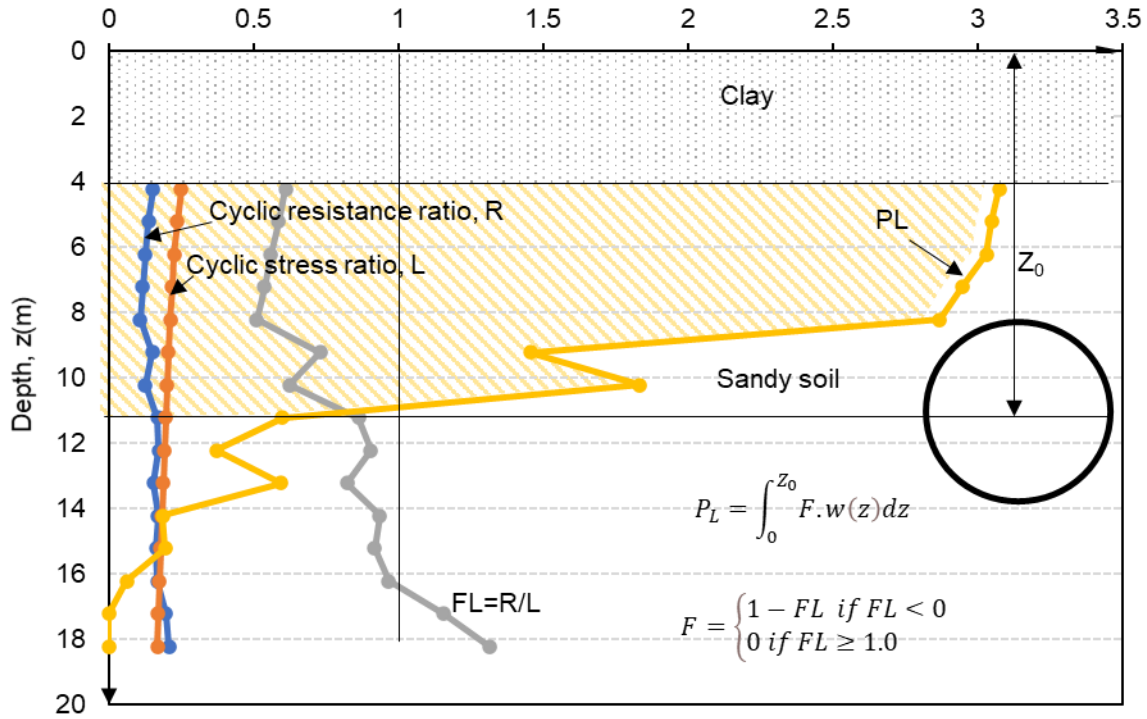
Figure A1. Definition of FL and PL
