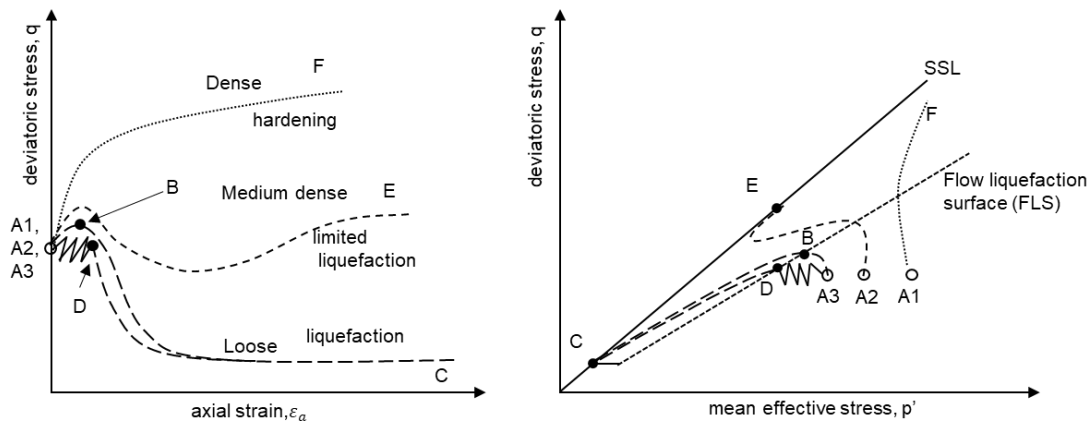
Figure 13. Dilation of dense sand, limited flow liquefaction of medium sand under monotonic loading and flow liquefaction of loose sand initiated by both monotonic and cyclic loading (After Kramer, 1996).
