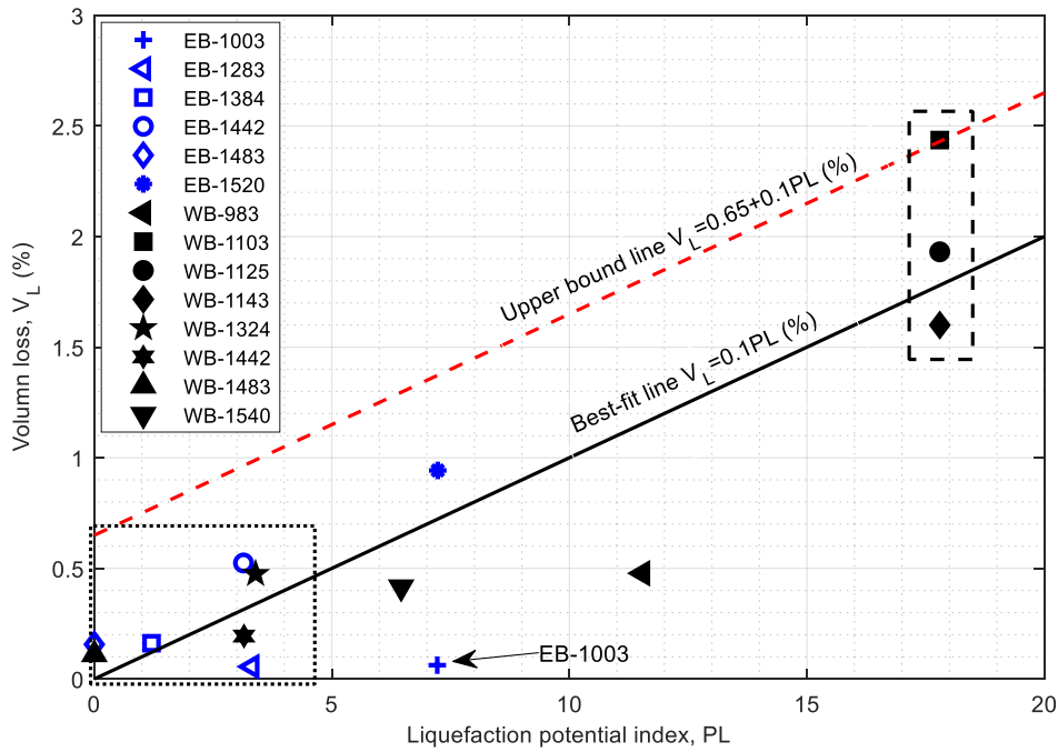
Figure 14. Relationship between the Liquefaction potential index, PL , and volume loss, V_L .
