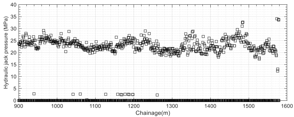
b. Measured hydraulic pressure in a jack during each ring in WB tunnel.
