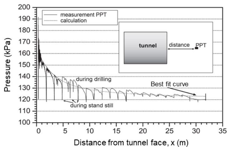
Figure 4. Measured excess pore pressure in front of a TBM in sandy soil (after Bezuijen, 2006).
