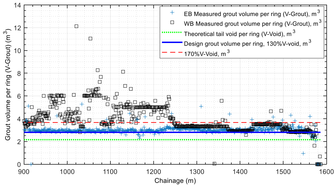
Figure 11. The measured volume of tail void grouting during the tunnel construction.
