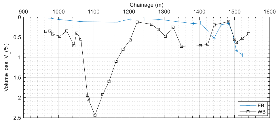
b. Volume loss along the route
