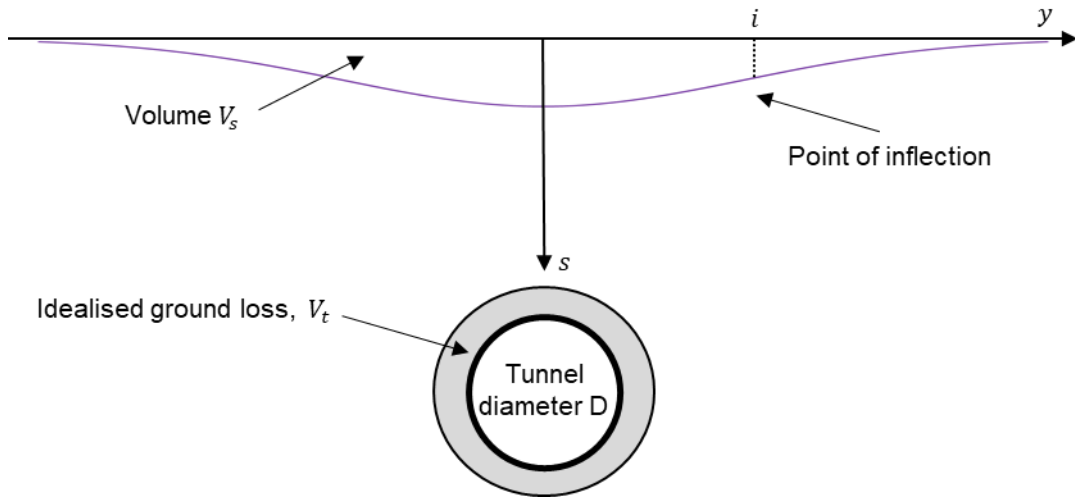
Figure 2. Ground surface settlement trough (Not to scale).
