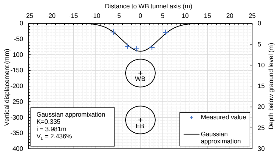
e) Ground surface vertical displacement due to WB tunnel excavation at chainage 1103m
