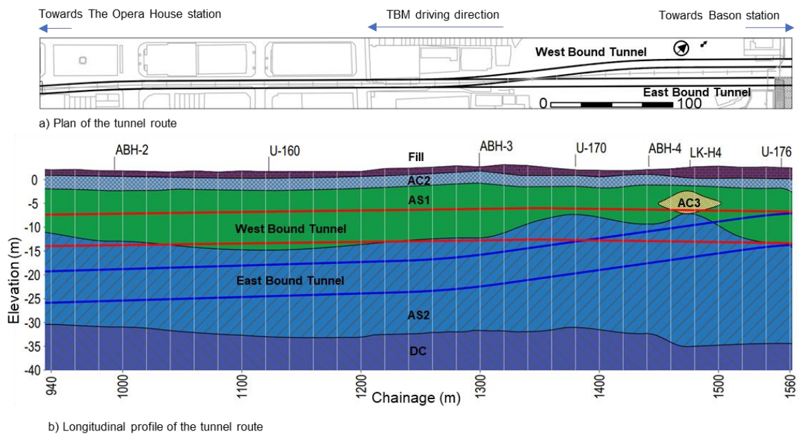
Figure 6. Plan and longitudinal profile of the tunnel route.
