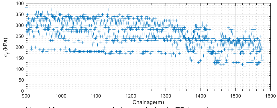
c. Measured tunnel face pressure \sigma_f during each ring in EB tunnel.
