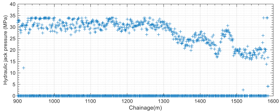
a. Measured hydraulic pressure in a jack during each ring in EB tunnel.
