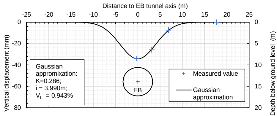
a) Ground surface vertical displacement due to EB tunnel excavation at chainage 1523m
