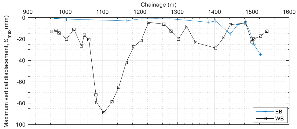
a. Maximum ground surface settlement along the tunnel route
