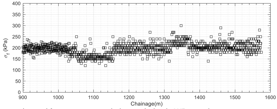
d. Measured tunnel face pressure \sigma_f during each ring in WB tunnel.
