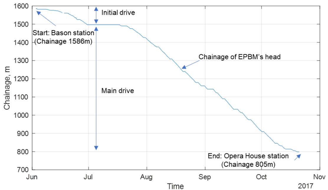
a) TBM advance rate in EB tunnel
