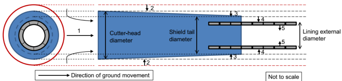
Figure 5. Illustration on components of volume loss (Wan et al., 2017b).
