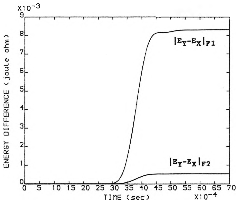
FIG (6.9). ENERGY DIFFERENCE COMPARISON BY (LOC) L1 BETWEEN IN-ZONE AND OUT-OF-ZONE FAULTS WITH f_c = 90.0 (kHz)
