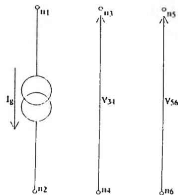
Fig (6) A 2-dimensional voltage controlled current source
