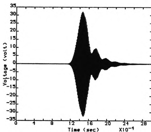
Figure 7 Filtered voltage across resistor R_{p2} of locator (Loc)_n
