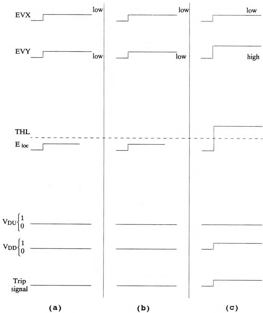
FIG(3.7), THE BEHAVIOUR OF LOCATORS IN FIG(3.1) DUE TO A FAULT AT F2.
