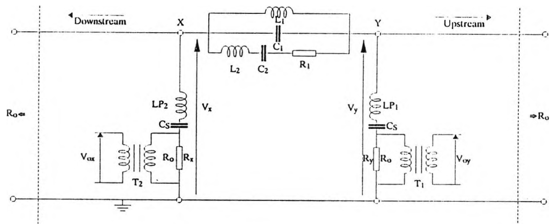
Fig (1), The arrangement of the locator
