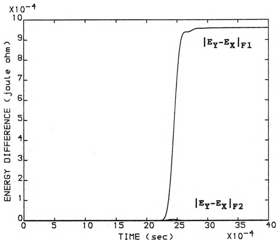
FIG (6.24). ENERGY DIFFERENCE COMPARISON BY (LOC) L1 BETWEEN IN-ZONE AND OUT-OF-ZONE FAULTS WITH f_c = 270.0 (kHz)
