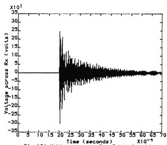
Fig (6) Voltage across Rx of locator L1.
