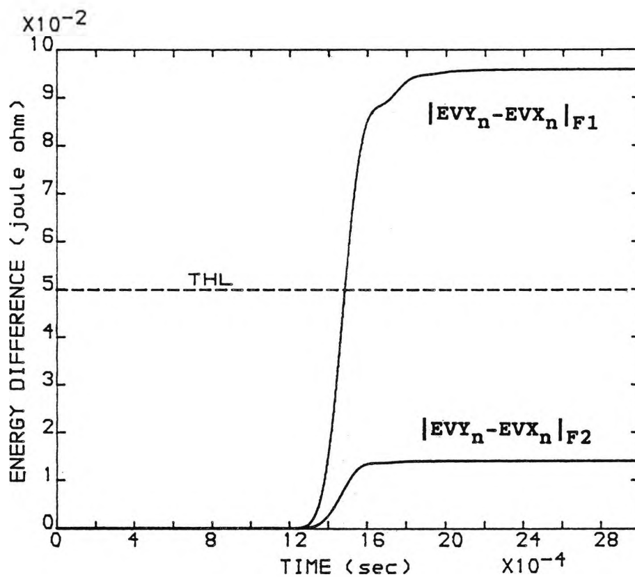
FIG (7.11), DISCRIMINATION BETWEEN FAULTS AT POINTS F1 AND F2 WITH f_c = 90.0 (kHz)
