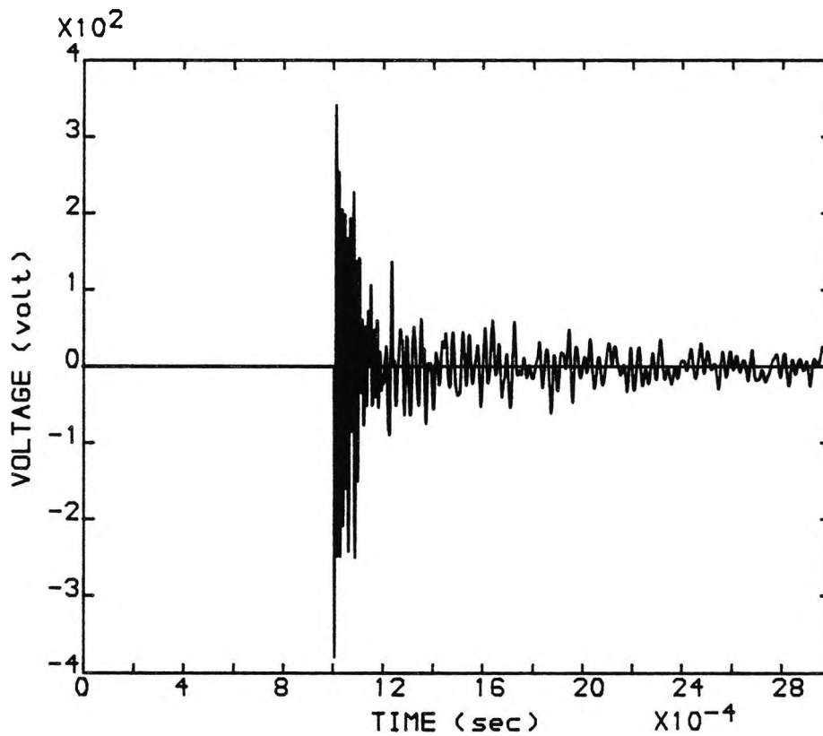
FIG (7.3). VOLTAGE SIGNAL (VYn) F1 DUE TO A FAULT AT POINT F1, WITH f_c = 90.0 (kHz) SHORT-CIRCUIT LEVEL = 250 MVA FAULT RESISTANCE = 0.0 (ohms) TYPE OF FAULT : [a-e] FAULT INCEPTION ANGLE = 90.0 (degrees)
