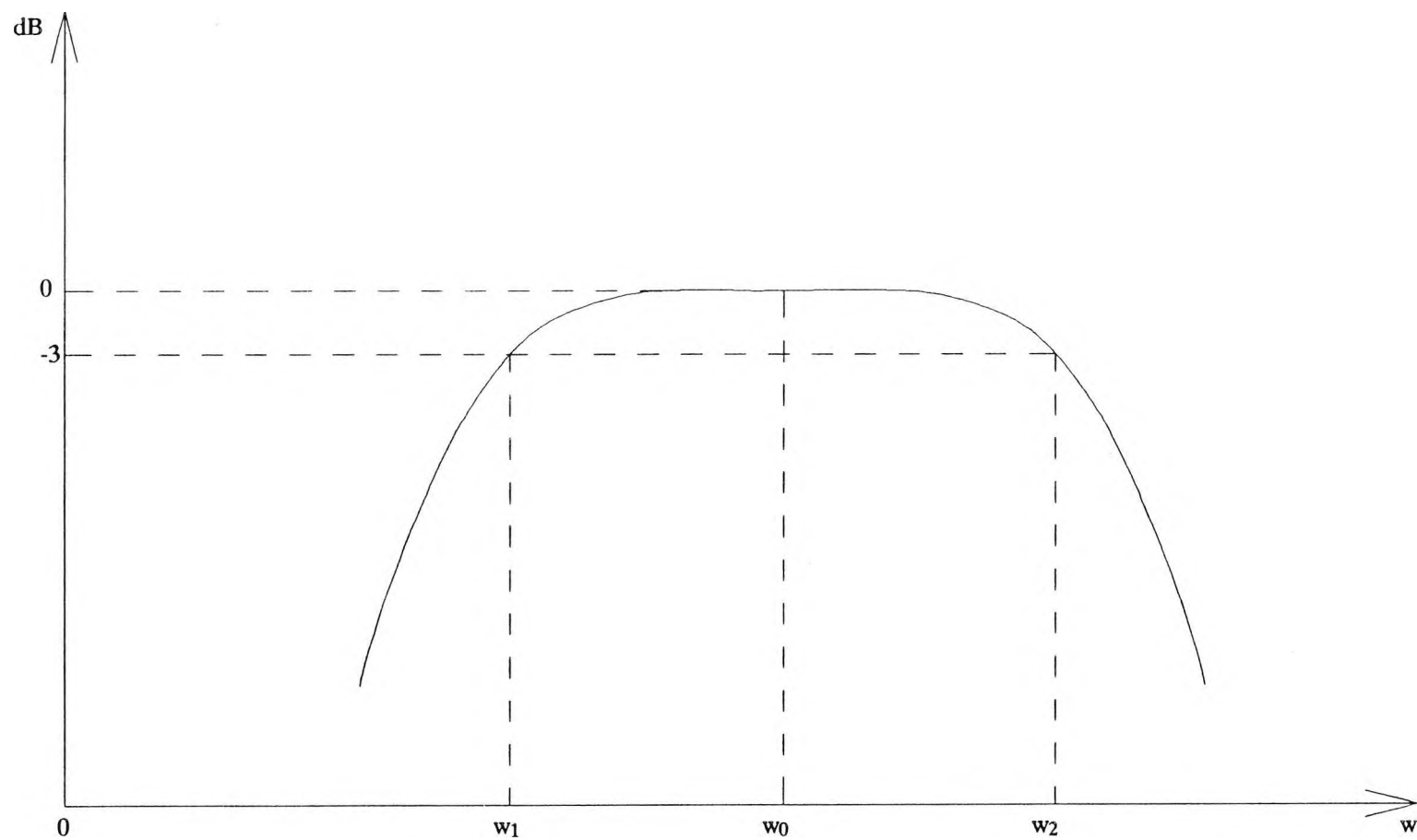
FIG(3.8), MAGNITUDE FREQUENCY RESPONSE OF A BAND-PASS FILTER.
