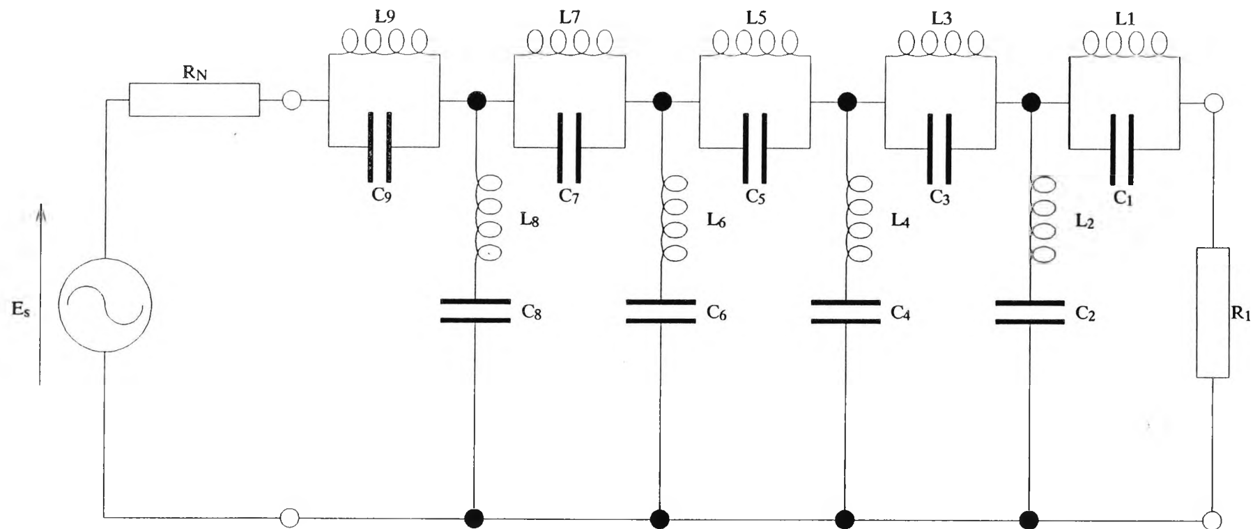
FIG(3.10), THE REQUIRED BAND-PASS FILTER.
