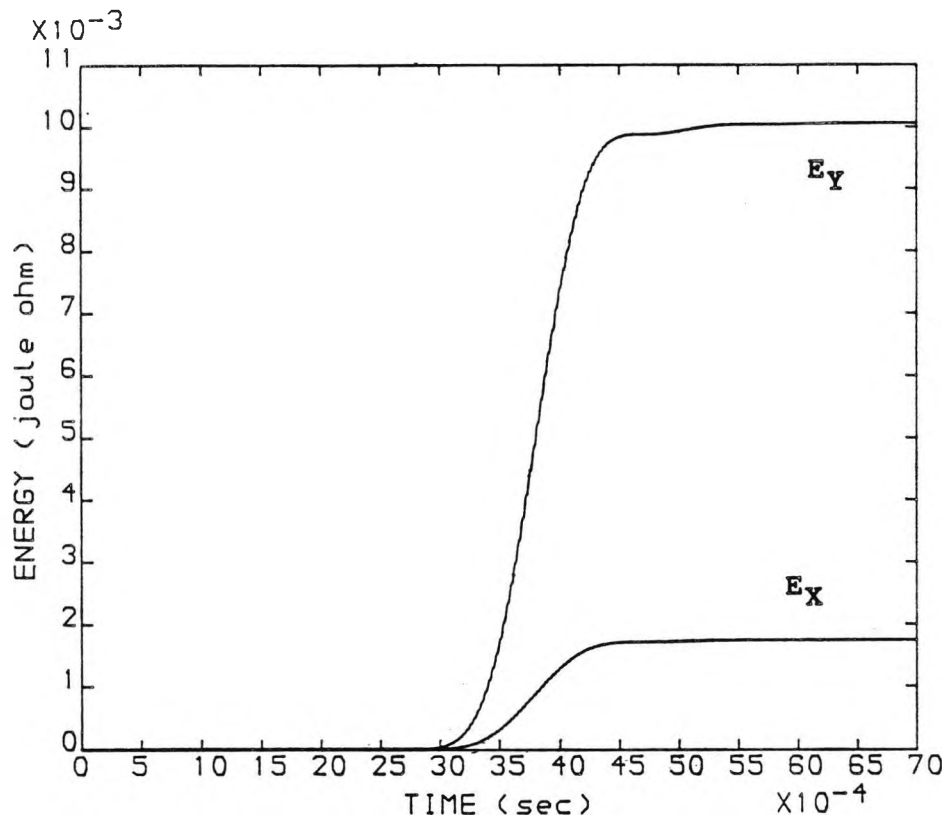
FIG 5.9 (a). ENERGY COMPARISON BY (LOC) L1 DUE TO A FAULT AT POINT F1, WITH f_c = 90.0 (kHz)
