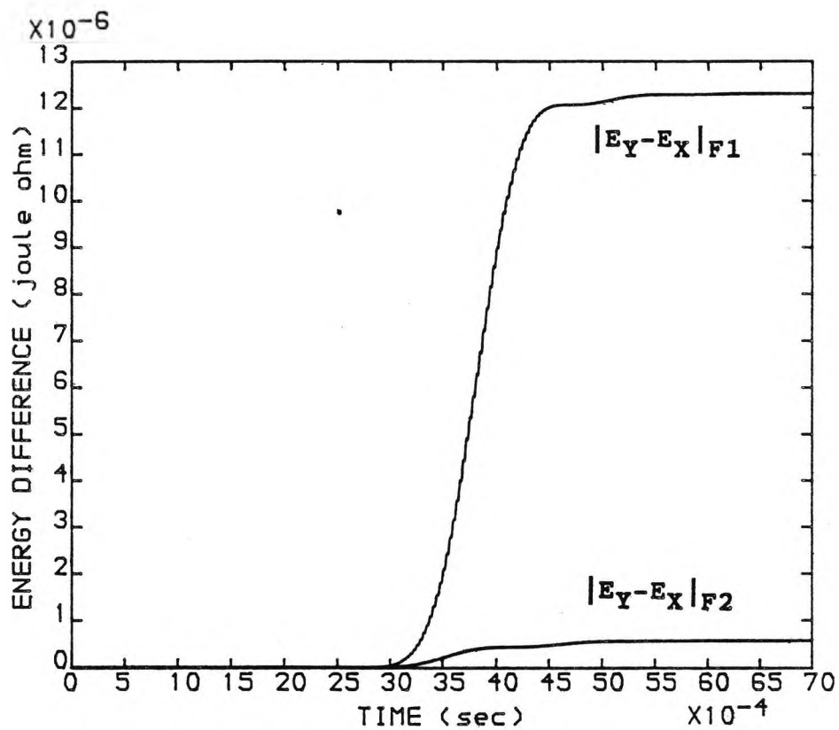
FIG (6.16). ENERGY DIFFERENCE COMPARISON BY (LOC) L1 BETWEEN IN-ZONE AND OUT-OF-ZONE FAULTS WITH f_c = 90.0 (kHz)
