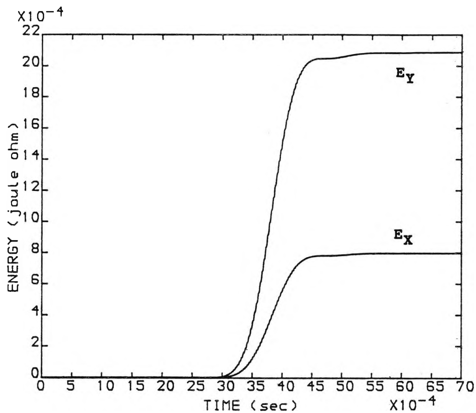
FIG (5.17). ENERGY COMPARISON BY (LOC) L1 DUE TO A FAULT AT POINT F1, WITH f_c = 90.0 (kHz)
