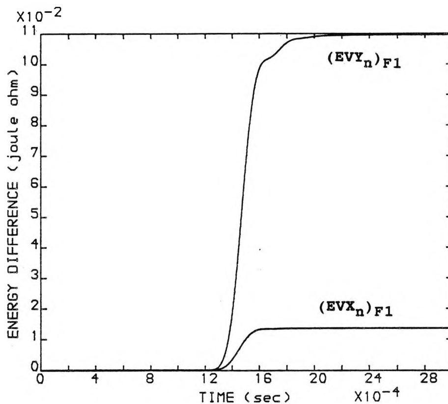
FIG (7.7). ENERGY COMPARISON BY (LOC) n DUE TO A FAULT AT POINT F1 WITH f_c = 90.0 (kHz)
