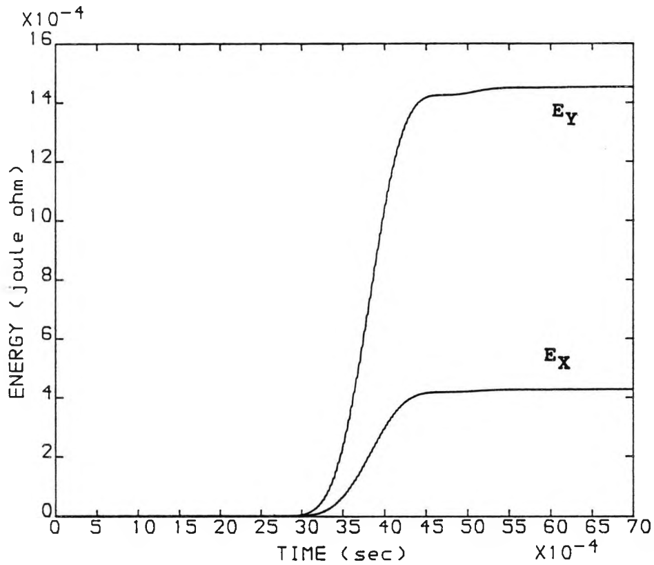
FIG (5.12). ENERGY COMPARISON BY (LOC) L1 DUE TO A FAULT AT POINT F1, WITH f_c = 90.0 (kHz)
