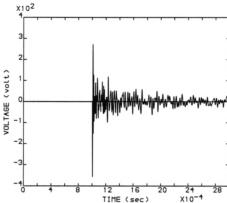
FIG (7.4). VOLTAGE SIGNAL (VXn) F1 DUE TO A FAULT AT POINT F1, WITH f_c = 90.0 (kHz)
