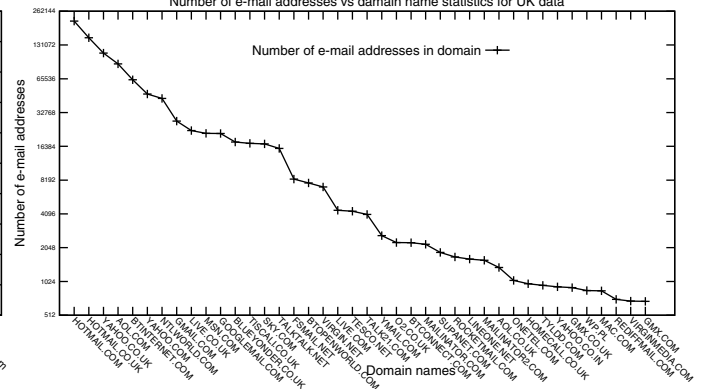
Fig. 4. Frequency of 40 most frequent surnames and 40 most frequent e-mail address domains for United Kingdom data set
