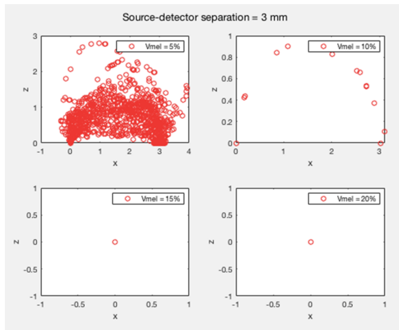
Fig. 4 (a) Photon propagation of red light when d = 1 mm for different skin pigmentations. (b) Photon propagation of red light when d = 3 mm for different skin pigmentations.
