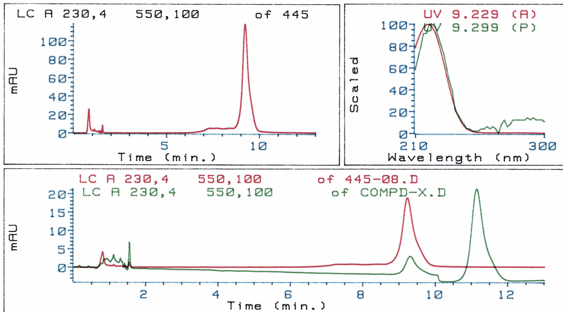
Figure 5-12. Purity assessment of 445-08, run under isocratic conditions with 25 x 0.45 cm Hypersil-ODS 5 \mu m column, eluted with 28:72 MeCN/H 2 O at 2 ml/min, monitored at 230 nm (Top left). (Top right): Superimposed UV spectra of 445-08 and that of the transformation product of "Compound X". (Bottom): Superimposed chromatograms of 445-08 and the partially transformed reference sample of "Compound X". 445-08 corresponds to the transformation product of Compound X.
