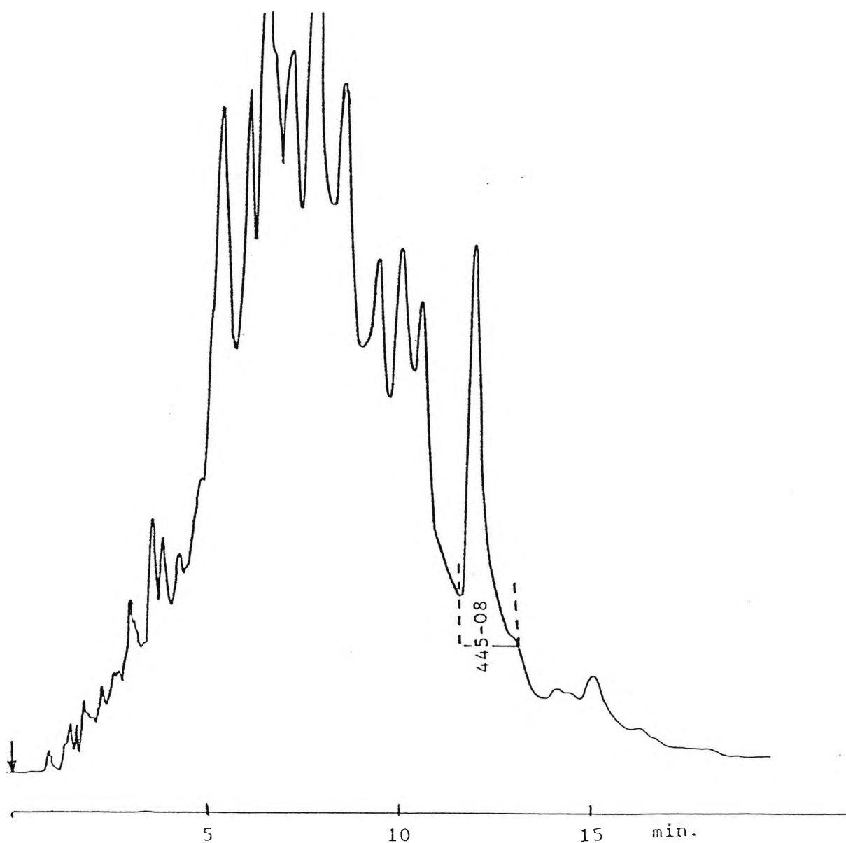
Figure 5-11. Semipreparative isocratic separation of the active fraction 425-08 on a 33 x 0.7 cm ODS-Hypersil 5 \mu m column eluted with 28:72 MeCN/H 2 O at 5 ml/min and monitored at 230 nm at 0.02 AUFS to obtain subfraction 435-08. Loaded sample : 5 mg in MECN on a 100 \mu l injection loop.
