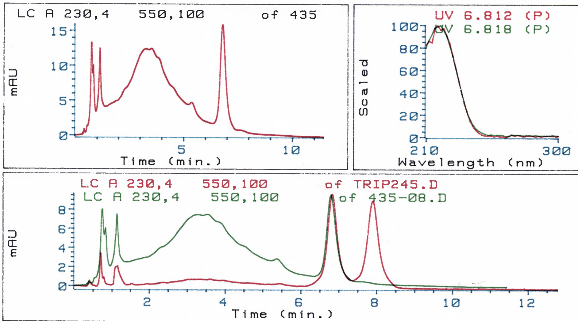
Figure 5-10. Isocratic HPLC separation method for 425-08, on a 25 x 0.45 cm analytical ODS-Hypersil 5 \mu m column, eluted with 28:72 MeCN/H 2 O at 2 ml/min and monitored at 230 nm (Top left). (Top right): Superimposed UV spectra of the main component of 425-08 eluted at 6.8 min and that of the transformation product of "Compound X". (Bottom): Superimposed chromatograms of 425-08 and the partially transformed reference sample of "Compound X". The main component of 425-08 corresponds to the transformation product of "Compound X".
