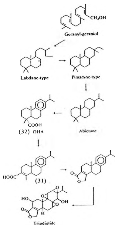
Scheme 4-2 : Biosynthetic pathway to tripdiolide
