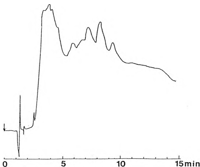
Figure 5-17. Normal phase HPLC separation of subfraction 435-01-3 in a 25 x 0.45 cm Ultrasphere-cyano 5 \mu m column, eluted with 85:5:15 Hexane/ \text{CH}_2\text{Cl}_2 /MeOH at 2 ml/min, monitored at 230 nm.
