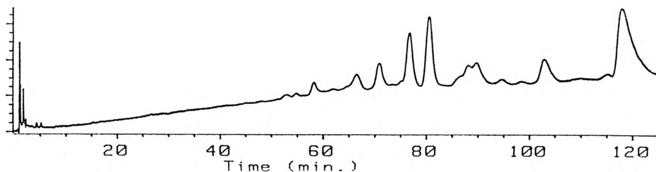
Figure 5-29. Resolution of P5 on a 25 x 0.45 cm Exsil-ODS 5 \mu m column, eluted with a continuous gradient from 4:4:92 to 9:9:82 MeCN/MeOH/H 2 O at 2 ml/min using a 25 ml mixing flask and monitored at 230 nm.
