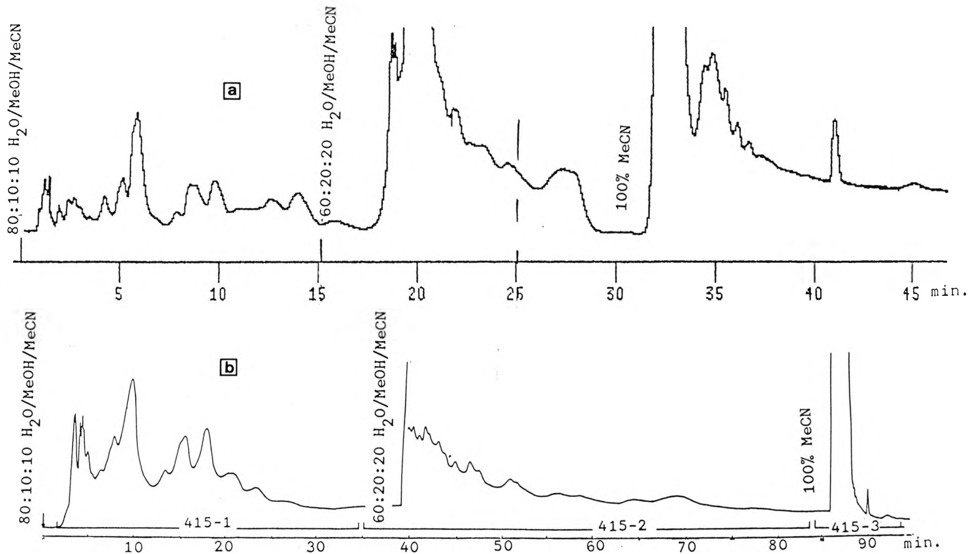
Figure 5-1. Multistep gradient HPLC separation of TW405 on ODS. a) Analytical HPLC on 25 x 0.45 cm ODS-Hypersil 5 \mu m eluted with 10:10:80 MeCN/MeOH/H 2 O from 0-15 min., 20:20:60 MeCN/MeOH/H 2 O from 15-25 min. and 100% MeCN from 25-45 min. at 2 ml/min, monitored at 230 nm. b) Preparative separation on 1" O.D. x 33 cm Hypersil-ODS 5 \mu m, eluted with 10:10:80 MeCN/MeOH/H 2 O from 0-35 min., 20:20:60 MeCN/MeOH/H 2 O from 35-85 min., and 100% MeCN from 85-95 min., at 30 ml/min, monitored at 230 nm, at 0.05 AUFS, loading 200 mg in a 4 ml loop.
