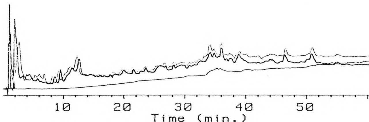
Figure 5-5. Reproducibility of continuous gradient elution profile of TW405 and comparison with a blank run, on a 25 x 0.45 cm Spherisorb-ODS1 5 \mu m, with a continuous gradient elution from 10:10:80 MeCN/MeOH/H 2 O to 50:50 MeCN/MeOH using a 100 ml mixing flask at 2 ml/min and monitored at 230 nm.
