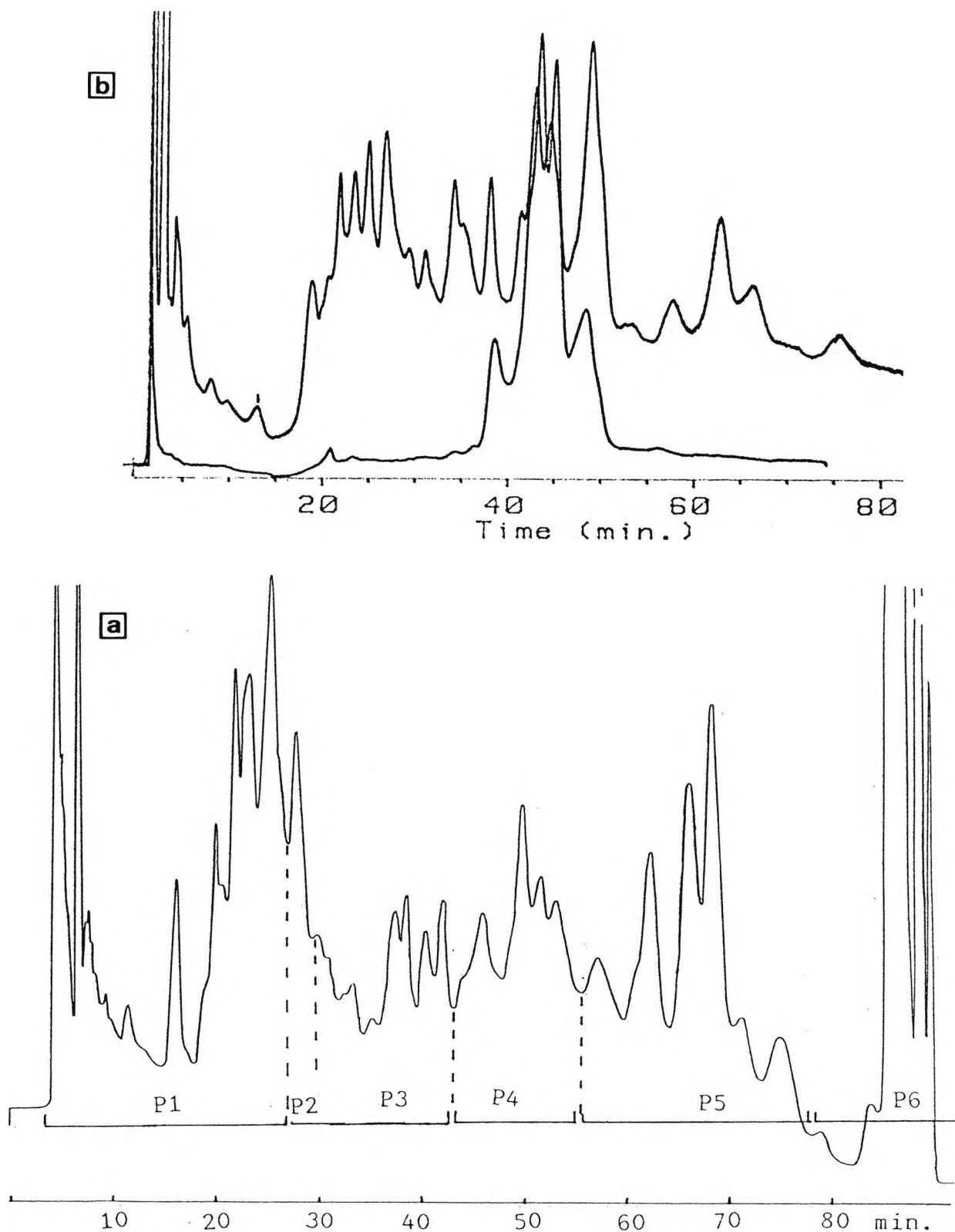
Figure 5-27. a) Separation of 402-S in 6 subfractions, on a 1" O.D. x 50 cm ODS-Vydac 300A 15-20 \mu m preparative column (protected with a 9 cm x 1" ODS-Vydac 300A 15-20 \mu m guard column), eluted for 5 min with 100% H 2 O, then gradient elution to 12:12:76 MeCN/MeOH/H 2 O at 36 ml/min using a 1 l mixing flask, monitored at 230 nm and 1 AUFS using an analytical flowcell. Loaded sample: up to 3 g dissolved in warm water and introduced with a 13 ml sample loop.
