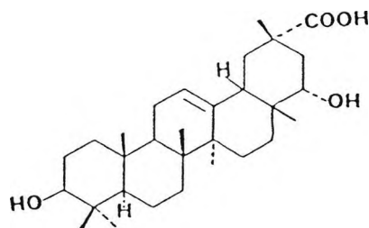
(41) Triptotriterpenic acid A
