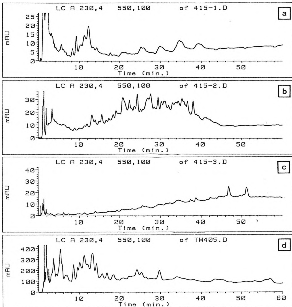
Figure 5-16. Fractions 415-1 (a), 415-2 (b), 415-3 (c) and starting material TW405 (d) run under continuous gradient elution on a 25 x 0.45 cm ODS-Hypersil 5 \mu m column from 10:10:80 to 22:22:56 MeCN/MeOH/H 2 O using a 50 ml mixing flask at 2 ml/min, monitored at 230 nm. 415-2 is the only active fraction.
