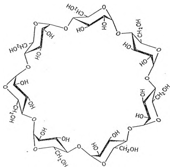
Figure 3-5: Structure of b-cyclodextrin
