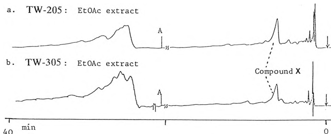
Figure 4-3. HPLC of solvent extraction fractions prepared from tablets of Tripterygium wilfordii according to Extraction Schemes 4-3 and 4-4. Column 25 x 0.45 cm Hypersil-APS 5 \mu m, eluted initially with 8:2:10:80 MeCN-iPrOH-Hexane-CH 2 Cl 2 , switching to 15:5:80 MeCN-iPrOH-CH 2 Cl 2 at point A; monitored at 230 nm.
