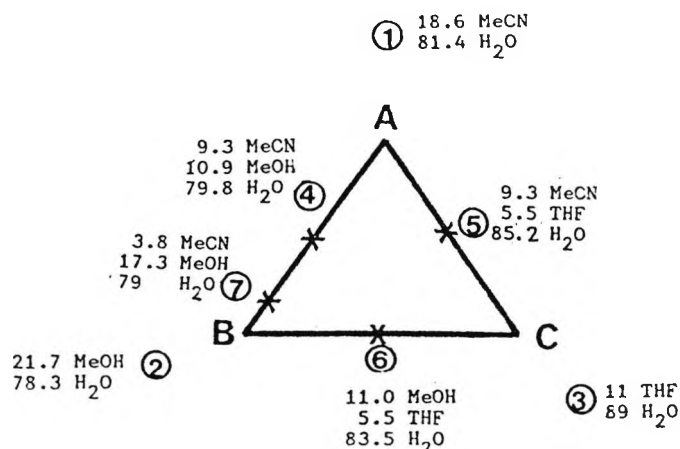
Figure 5-19. Selectivity triangle for reverse phase chromatography, using solvent mixtures containing MeOH, MeCN and THF, all with an eluent strength ( P' ) of 8.48.
