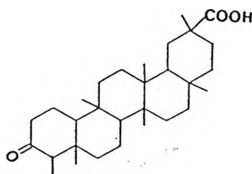
(36) Populnonic acid
