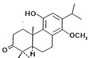
(54) Triptonorterpene methyl ether
