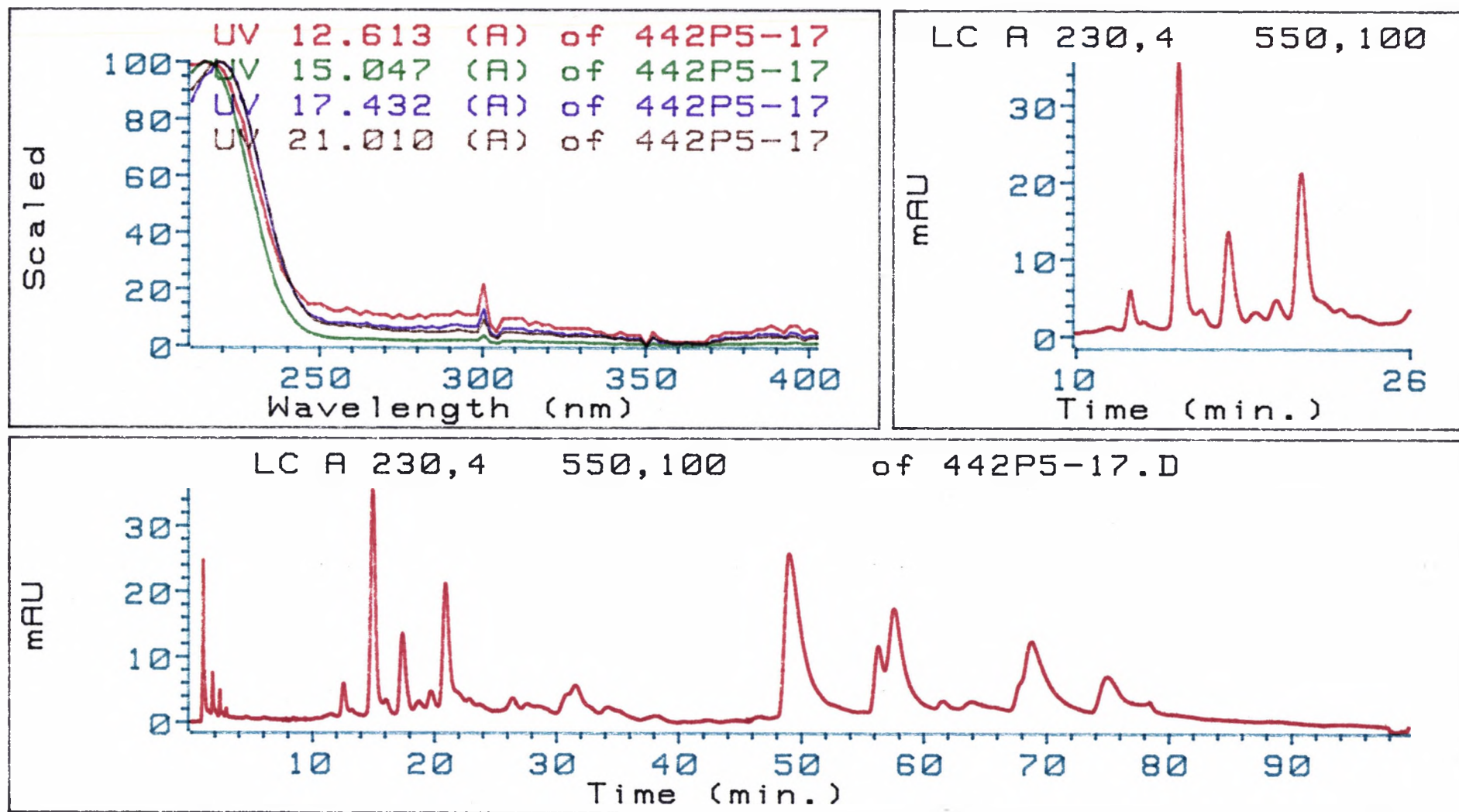
Figure 5-30. HPLC separation of the active preparative subfraction P5 (bottom) and close up section of the chromatogram containing the 4 early eluting peaks (top right), all with UV spectra superimposable to that of triptolide (top left), eluted on a 25 x 0.45 cm Exsil-ODS 5 \mu m column, with 96/4 H 2 O:THF for 20 min and gradient elution to 90/10 H 2 O:THF at 2 ml/min, using a 25 ml mixing flask, and monitored at 230 nm with a HP 1040 photodiode array detector, using a 20 \mu l sample loop.
