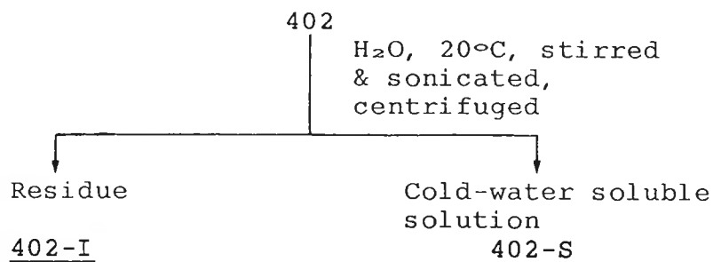
Scheme 5-2 Extraction sequence to remove the cold water insoluble solid from 402.
