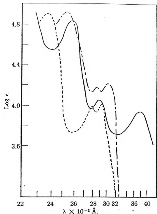
(1) —, Gossypol; (2) —, \beta,\beta -binaphthyl; (3) —, \alpha,\alpha -binaphthyl.
