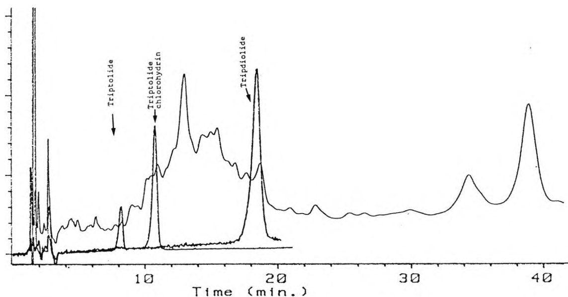
Figure 5-42. Normal phase HPLC separation of the crude fraction TW600 on 25 x 0.45 cm Nucleosil-nitro bonded 5 \mu m column, eluted with 80:5:5:10 Hexane/ \text{CH}_2\text{Cl}_2 /THF/MeOH at 2 ml/min, monitored at 230 nm. Comparison with the active reference samples of triptolide, triptolide chlorohydrin and triptidiolide.
