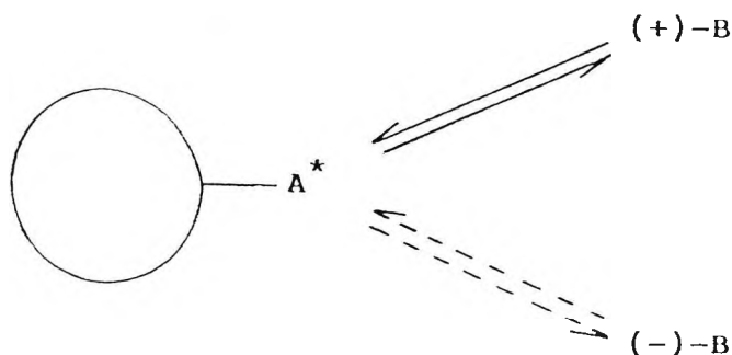
In situ formation of diastereoisomeric complexes
