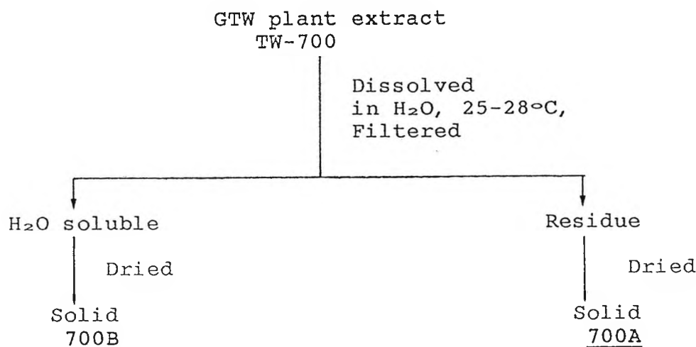
Scheme 5-4: Extraction sequence of TW-700 series
