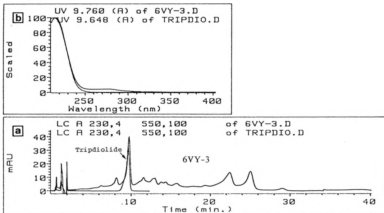
Figure 5-43. a) Superimposed analytical chromatograms of the preparative subfraction 6VY-3 and a reference sample of tripdiolide; run on a 25 x 0.45 cm Exsil-ODS 5 \mu m column with 96:4 H 2 O/THF at 2 ml/min and monitored at 230 nm with a HP 1040 photodiode array detector. b) Superimposed UV spectra of the main peak of 6VY-3 and the reference sample of tripdiolide. The main component in 6VY-3 is tripdiolide.
