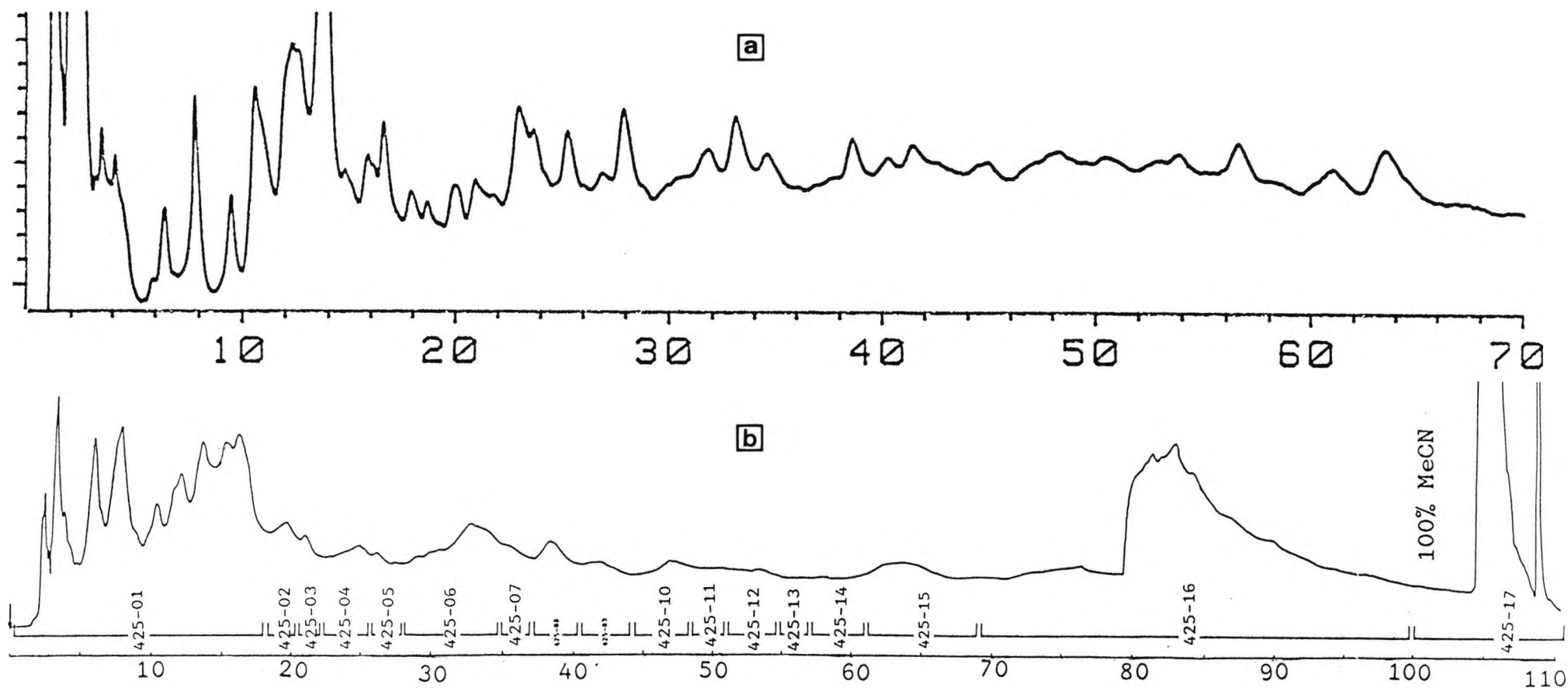
Figure 5-6. HPLC separation of 405 by continuous gradient elution on reverse phase (monitored at 230 nm). a) Analytical HPLC on 25 x 0.45 cm ODS-Hypersil 5 \mu m column, eluted by continuous gradient from 10:10:80 to 22:22:56 MeCN/MeOH/H 2 O using a 25 ml mixing flask at 2 ml/min. b) Preparative HPLC separation into 17 fractions on a 1" O.D. x 33 cm ODS chemically bonded to silica-Hypersil 5 \mu m column, eluted by continuous gradient from 10:10:80 to 22:22:56 MeCN/MeOH/H 2 O using a 2 l mixing flask at 30 ml/min, monitored at 0.02 AUFS using an analytical flowcell.
