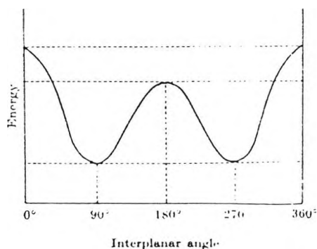
Fig 2-5: Energy diagram for racemization of biphenyls
