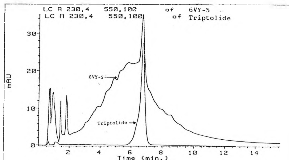
Figure 5-41. Superimposed chromatograms of the preparative subfraction 6VY-5 and a reference sample of triptolide, run under isocratic conditions on a 25 x 0.45 cm Hypersil-ODS 5 \mu m column, eluted with 28:72 MeCN/H 2 O at 2 ml/min, monitored at 230 nm.
