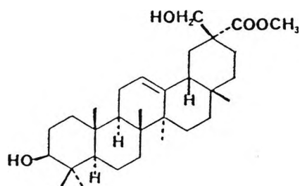
(45) Triptodihydroxy acid methyl ether
