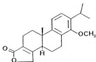
(50) Hypolide methyl ether
