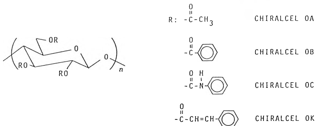
Fig. 3-3: Chiral sugar sorbents
