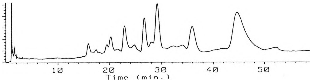
Figure 5-28. Resolution of P5 on a 25 x 0.45 cm Exsil-ODS 5 \mu m column, eluted with 8:8:84 MeCN/MeOH/H 2 O at 2 ml/min and monitored at 230 nm.
