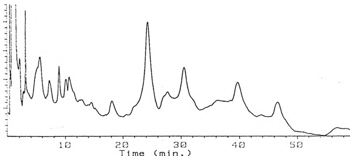
Figure 5-22. HPLC chromatogram corresponding to point 5 of the selectivity triangle in Figure 5-21, to achieve the optimum separation for 435-01-3 on a 25 x 0.45 cm ODS2-Spherisorb 5 \mu m column, monitored at 230 nm. Mobile phase 2.5:2.1:1.4:94 MeOH/MeCN/THF/H 2 O, with a P' of 8.88.
