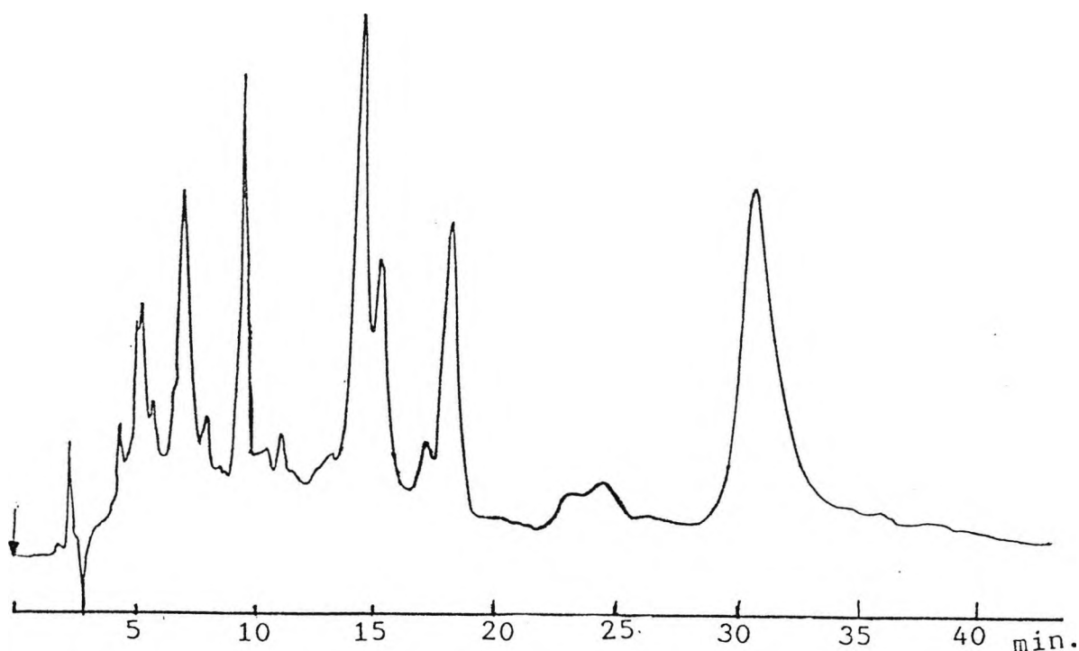
Figure 5-18. Normal phase HPLC separation of subfraction 435-01-3 in 25 x 0.45 cm Nucleosil-nitro bonded 5 \mu m column, eluted with 80:5:5:10 Hexane/ \text{CH}_2\text{Cl}_2 /THF/MeOH at 2 ml/min, monitored at 230 nm.
