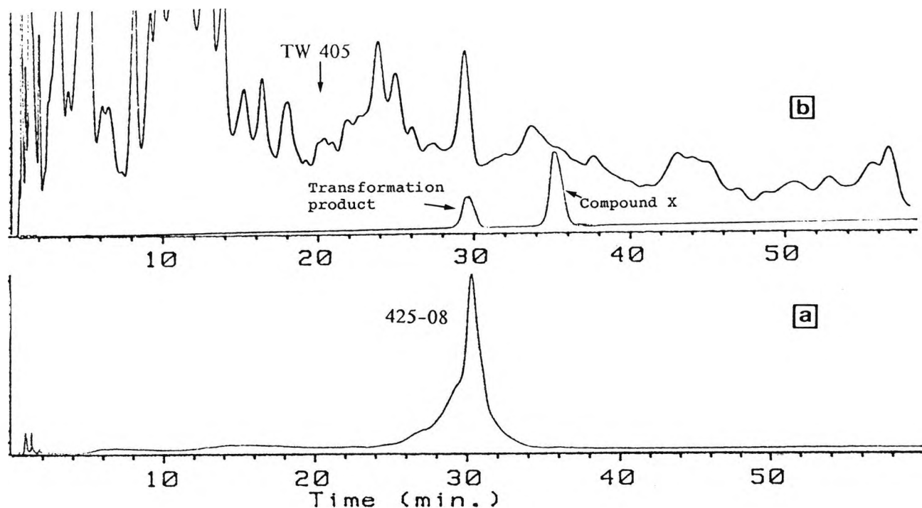
Figure 5-8. Purity assessment of the active fraction 425-08 (a) and comparison with the starting material 405, and the active reference standard, "Compound X" (b), on a 25 x 0.45 cm Spherisorb-ODS1 5 \mu m column, eluted under continuous gradient from 10:10:80 to 22:22:56 MeOH/MeCN/H 2 O using a 50 ml mixing flask at 2 ml/min, monitored at 230 nm.
