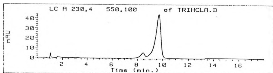
Figure 5-15. Transformation of triptolide to triptolide chlorohydrin by reaction with dry HCl gas in MeCN at 30 seconds, 3, 6, 15 and 30 minutes. Comparison with "Compound X" identified as triptolide chlorohydrin which has been partially transformed to triptolide on standing on MeOH. Chromatographed on a 25 x 0.45 cm Hypersil-ODS 5 \mu m column, eluted with 28:72 MeCN:H 2 O at 2 ml/min, monitored at 230 nm.
