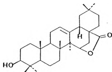
(40) Triptotriterpenoidal lactone A
