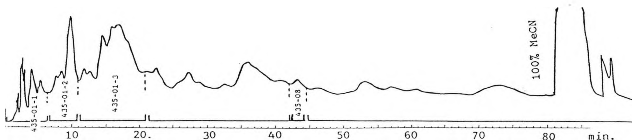
Figure 5-7. Collection of the active fractions 435-01 and 435-08 by selective fractionation of the active groups. 200mg sample was injected using a 4 ml loop on a 1" O.D. x 33 cm preparative ODS bonded on silica-Hypersil 5 \mu m column and eluted with continuous gradient elution from 10:10:80 to 22:22:56 MeCN/MeOH/H 2 O at 30 ml/min using a 2 l mixing flask, monitored at 230 nm and 0.02 AUFS using an analytical flowcell. 435-01 is subfractionated in 435-01-1, 435-01-2 and 435-01-3.
