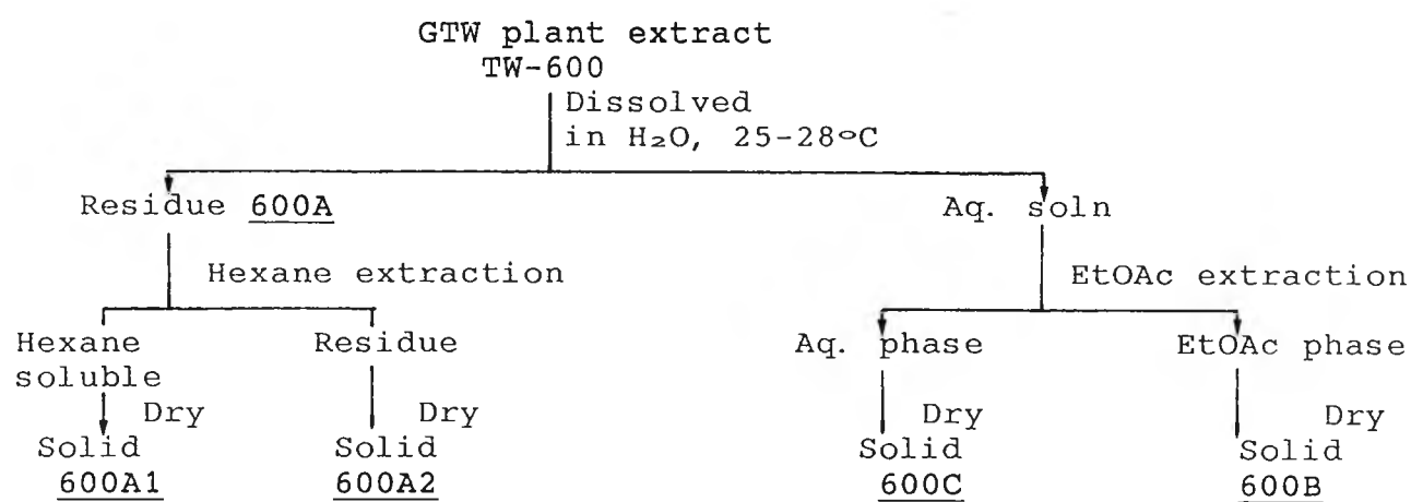
Scheme 5-3: Extraction sequence for TW-600 series
