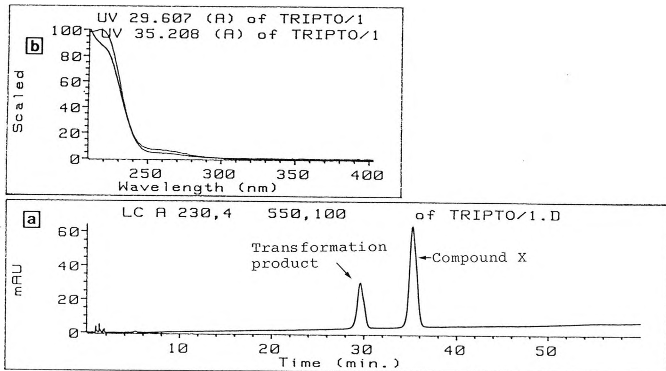
Figure 5-9. a) "Compound X", partially transformed on standing in methanol, chromatographed on a 25 x 0.45 cm Hypersil-ODS 5 \mu m HPLC column, eluted with a continuous gradient from 10:10:80 to 22:22:56 MeOH/MeCN/H 2 O using a 50 ml mixing flask at 2 ml/min, monitored at 230 nm. b) UV spectra with the photodiode array detector of both, "Compound X" and its transformation product.
