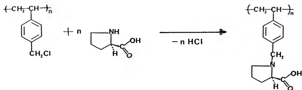
Scheme 3-3
