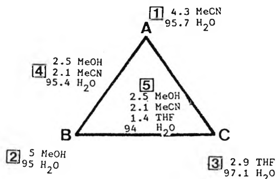
Figure 5-21. Selectivity triangle for reverse phase chromatography, using solvent mixtures containing MeOH, MeCN, and THF, all with an eluent strength ( P' ) of 8.88.
