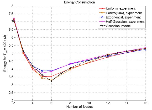
Figure 6: Energy consumption per node with different data production PDFs, d = 4 and r = 4.8 kbps; each node aggregates the received data with its own data within each transmission opportunity.
