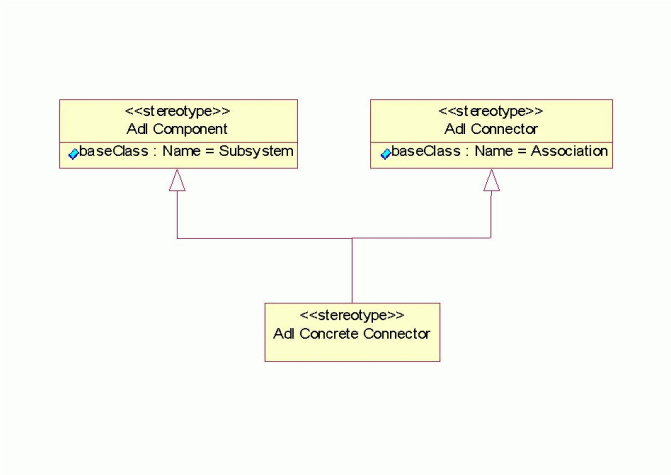
Figure 1: The ADLConcreteConnector stereotype
