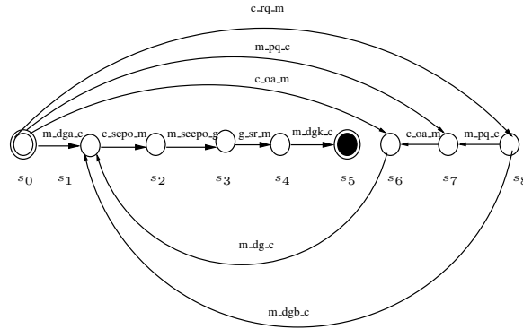
Fig. 2: A variant of the NetBill protocol
