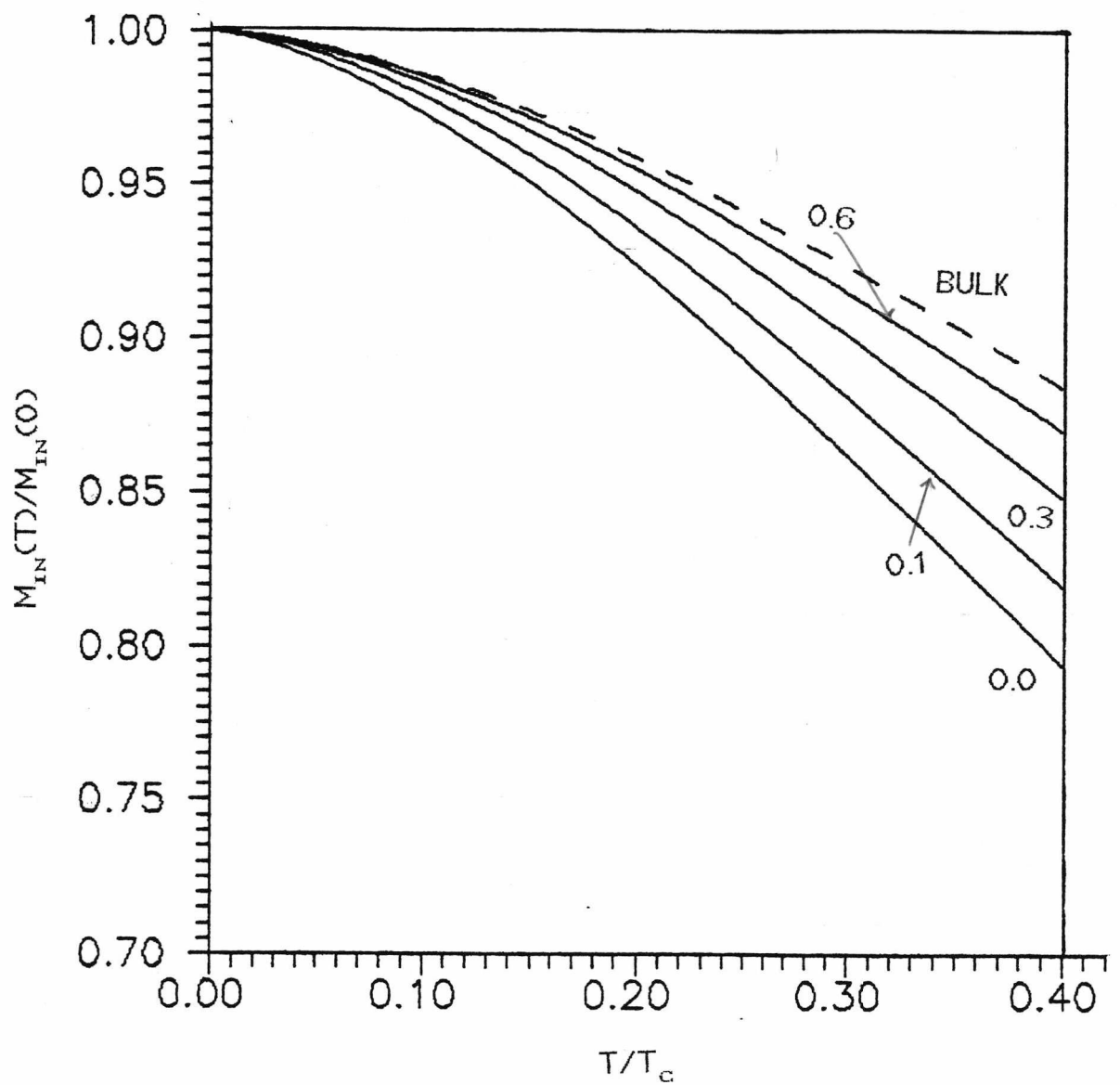
Fig.3.6 Calculated temperature dependence of the interface magnetization M_{IN}(T)/M_{IN}(0) for an interface separating two identical semi-infinite Heisenberg ferromagnets with a softened perpendicular exchange J_{10}/J . The values of J_{10}/J are 0.0, 0.1, 0.3 and 0.6.
