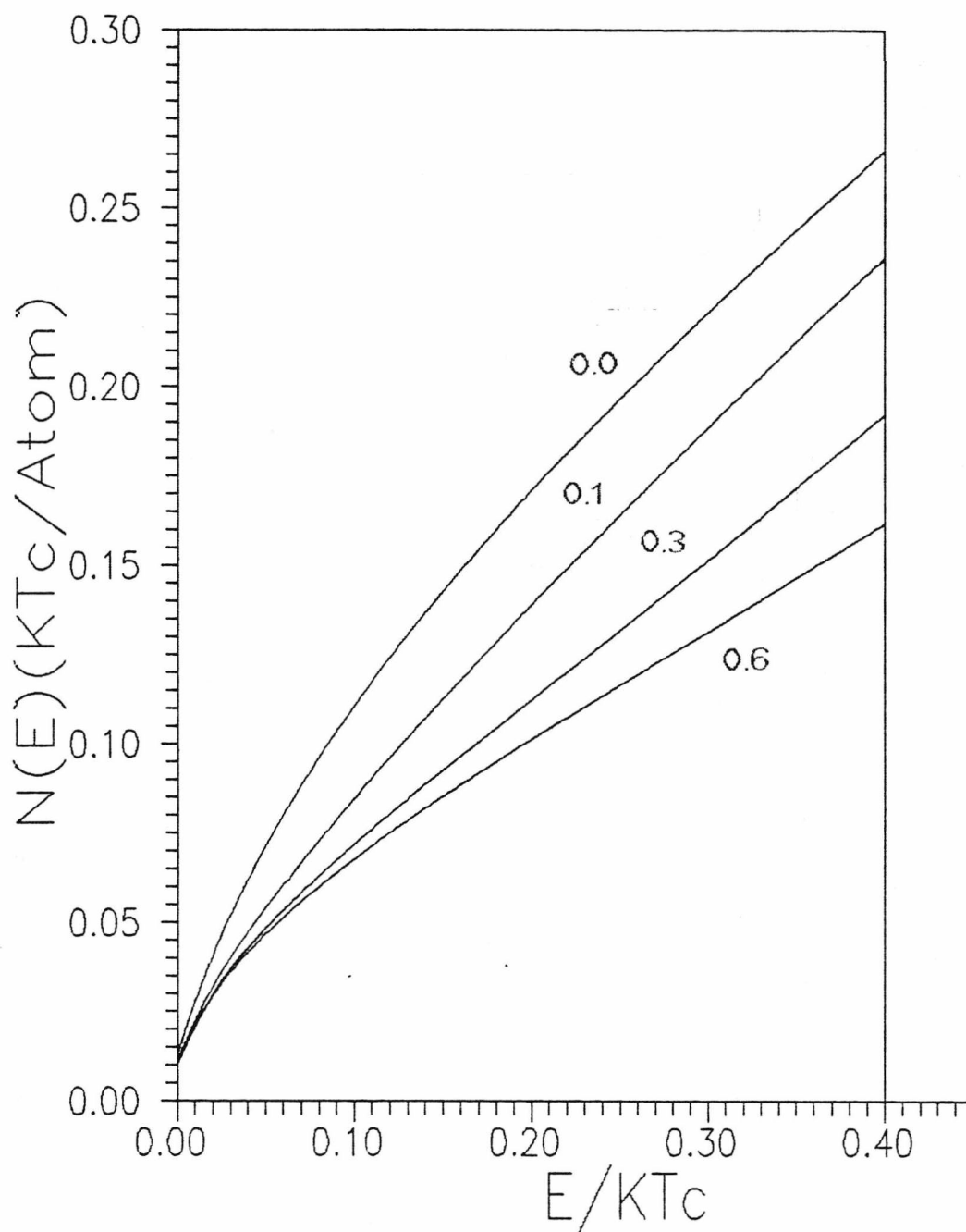
Fig.3.2 Calculated density of spin wave states N(E) in the (100) interface separating two identical semi-infinite Heisenberg ferromagnets. Only the exchange integral J_{10} perpendicular to the interfaces is softened. The values of J_{10}/J are 0.0, 0.1, 0.3 and 0.6.
