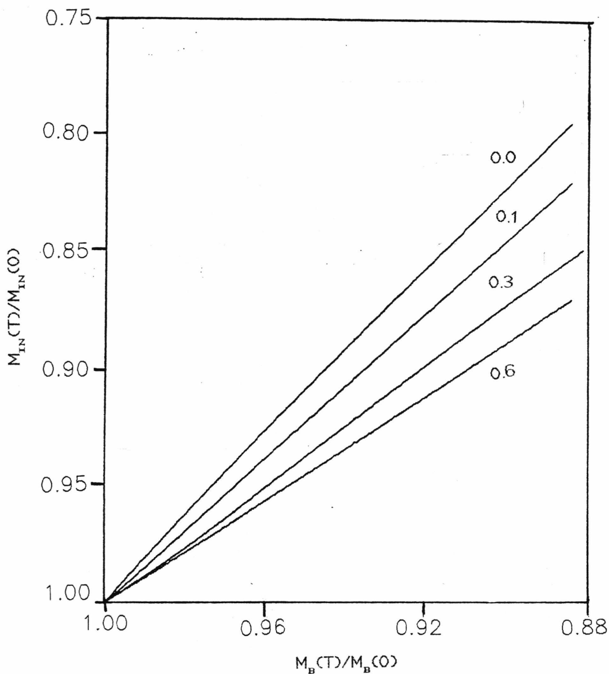
Fig.3.7 Plot of the temperature dependence of interface magnetization M_{IN}(T)/M_{IN}(0) against the bulk dependence M_B(T)/M_B(0) for an interface separating two identical semi-infinite Heisenberg ferromagnets. The values of J_{10}/J are 0.0, 0.1, 0.3 and 0.6.
