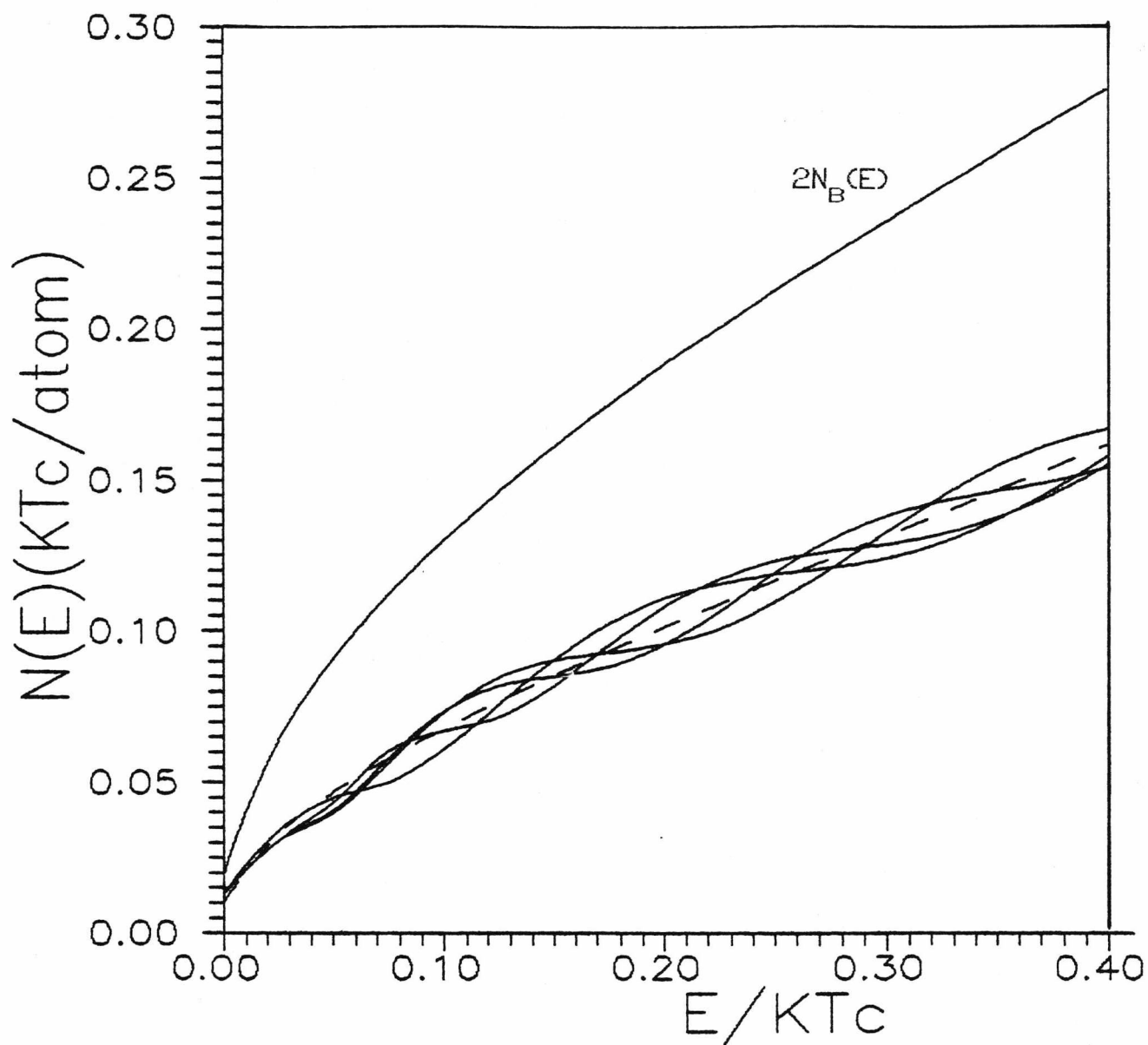
Fig.2.21 The density of spin wave states in the subsurface layer n=5 for an overlayer with softened surface-bulk exchange J_{10}/J=0.1, 0.3, 0.6 and 1.0 . The broken curve denotes the DOS of the bulk N_B(E) and the curve 2N_B(E) denotes the DOS of a geometric surface.
