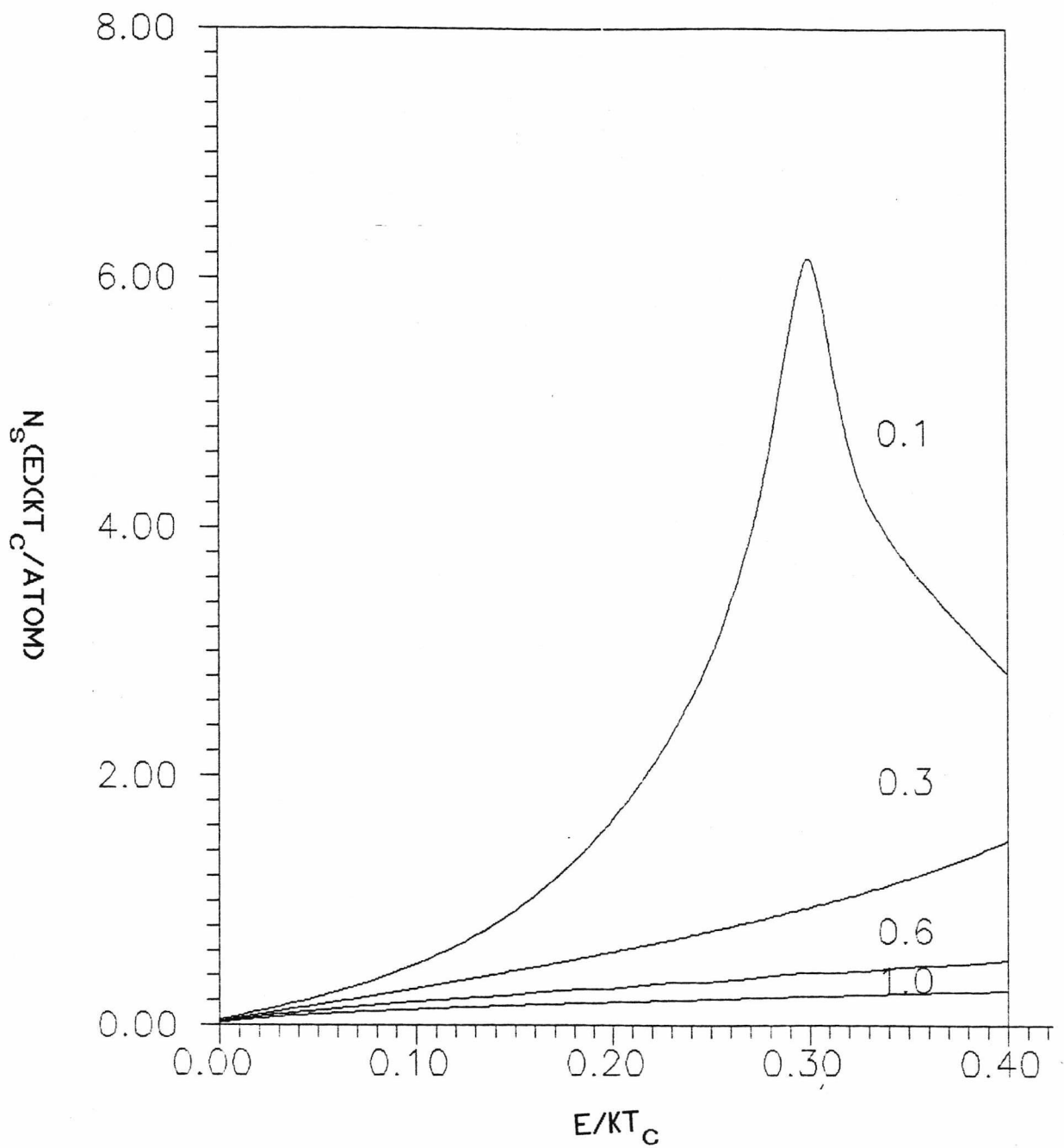
Fig.2.9 The total densities of spin waves states N_s(E) for an atomic overlayer above (100) surface of sc ferromagnet with a softened parallel exchange J_{11} . The result is obtained by using Cunningham points integral in BZ: nc = 128 and eps = 0.01 .
