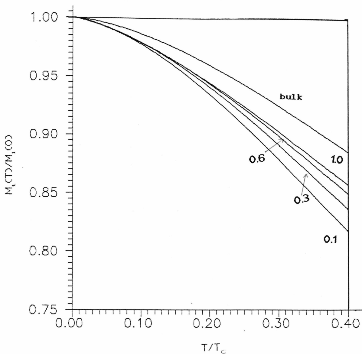
Fig.2.24 Calculated temperature dependence of the subsurface magnetization M_1(T)/M_1(0) for the subsurface layer n=1 with softened exchange J_{10} . The values of J_{10}/J are 0.1, 0.3, 0.6 and 1.0.
