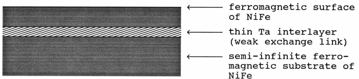
Fig.2.12 The NiFe-Ta-NiFe sandwich with thin Ta interlayer (different thicknesses) as a controller for weak exchange link.
