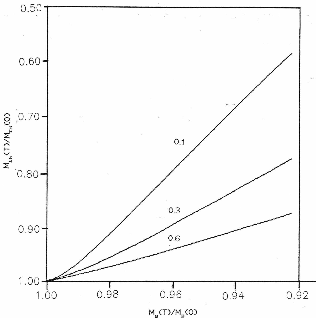
Fig.3.9 Plot of the interface M_{IN}(T)/M_{IN}(0) against the bulk dependence M_B(T)/M_B(0) for an interface consisting of two at. layers with parallel exchange J_{||}/J=0.1, 0.3 and 0.6
