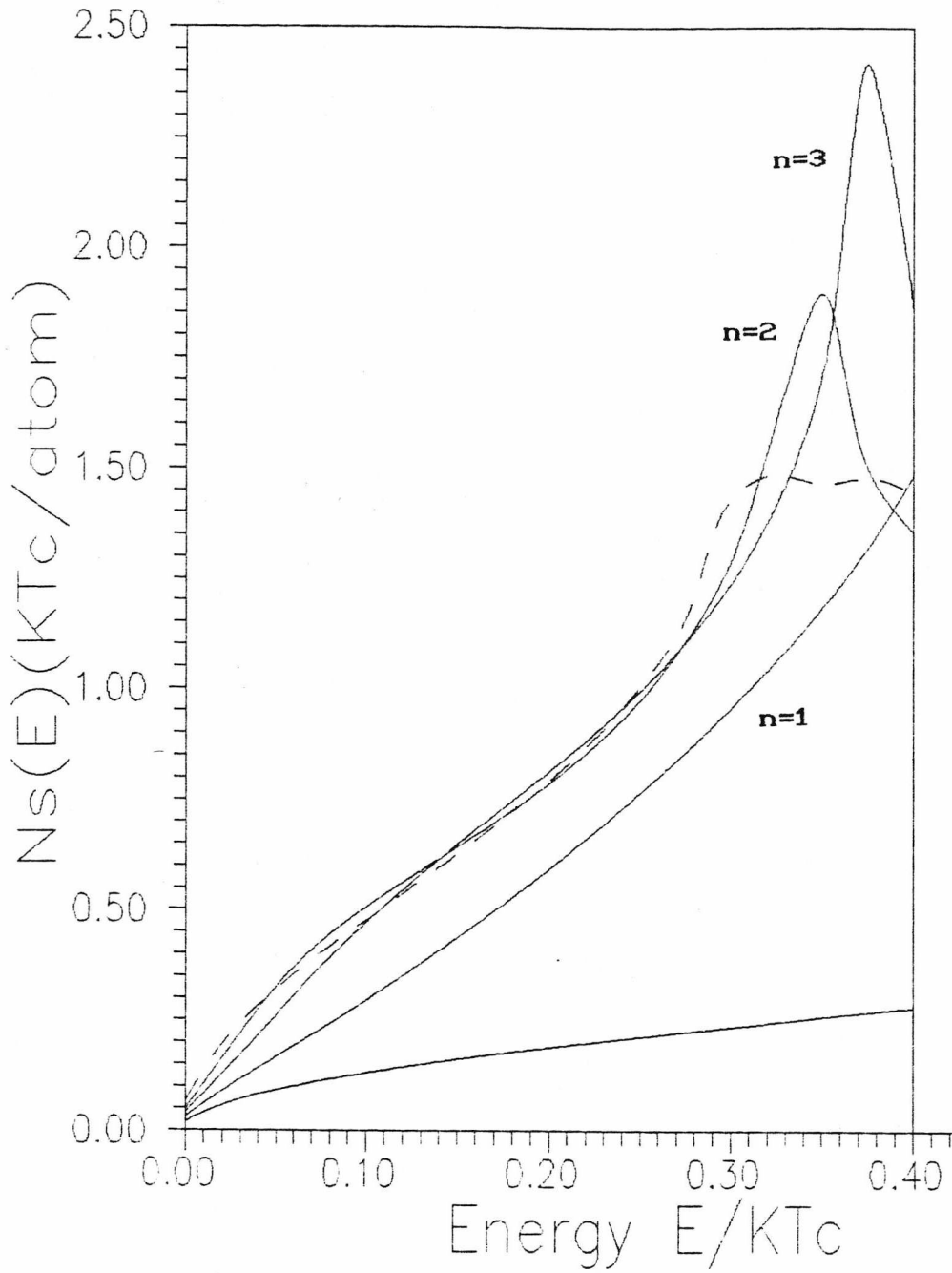
Fig.2.17 Density of spin wave states in the surface of an overlayer of n atomic layers with a softened parallel exchange J_{\parallel}/J=0.3 in overlayer. The broken curve denotes the asymptotic behaviour for n \gg 20 .
