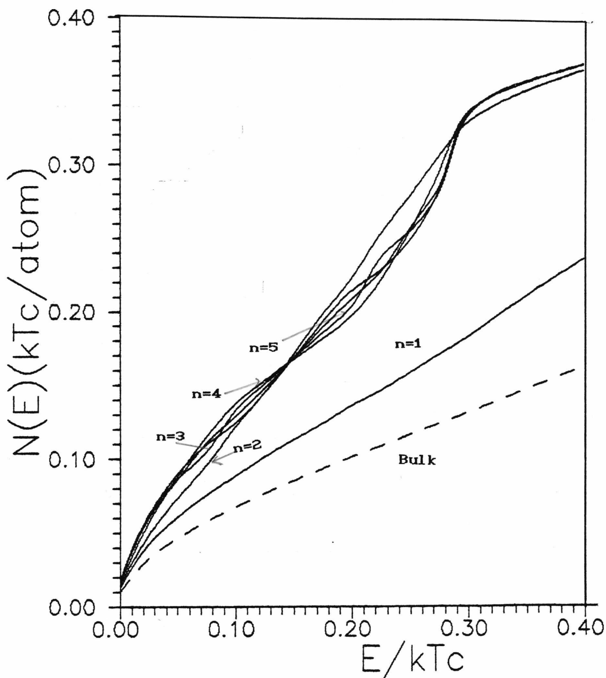
Fig.3.4 Calculated density of spin wave states N(E) in interface layers n=1, 2, 3, 4 and 5 for an interface consisting of 10 at. layers with the perpendicular exchange integral J_{\perp}/J=0.3 .
