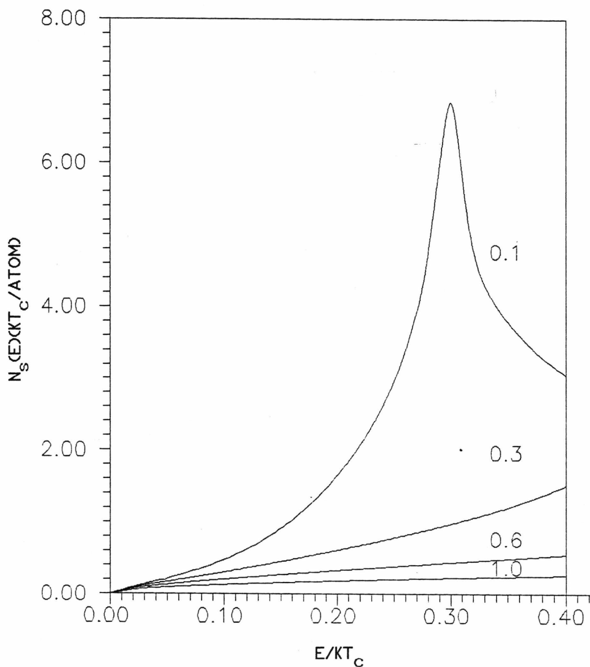
Fig.2.7 The total densities of spin waves states N_s(E) in the (100) surface of a sc ferromagnet with a softened parallel exchange J_{11} within the surface of overlayer. The values of J_{11} are 0.1, 0.3, 0.6 and 1.0.
