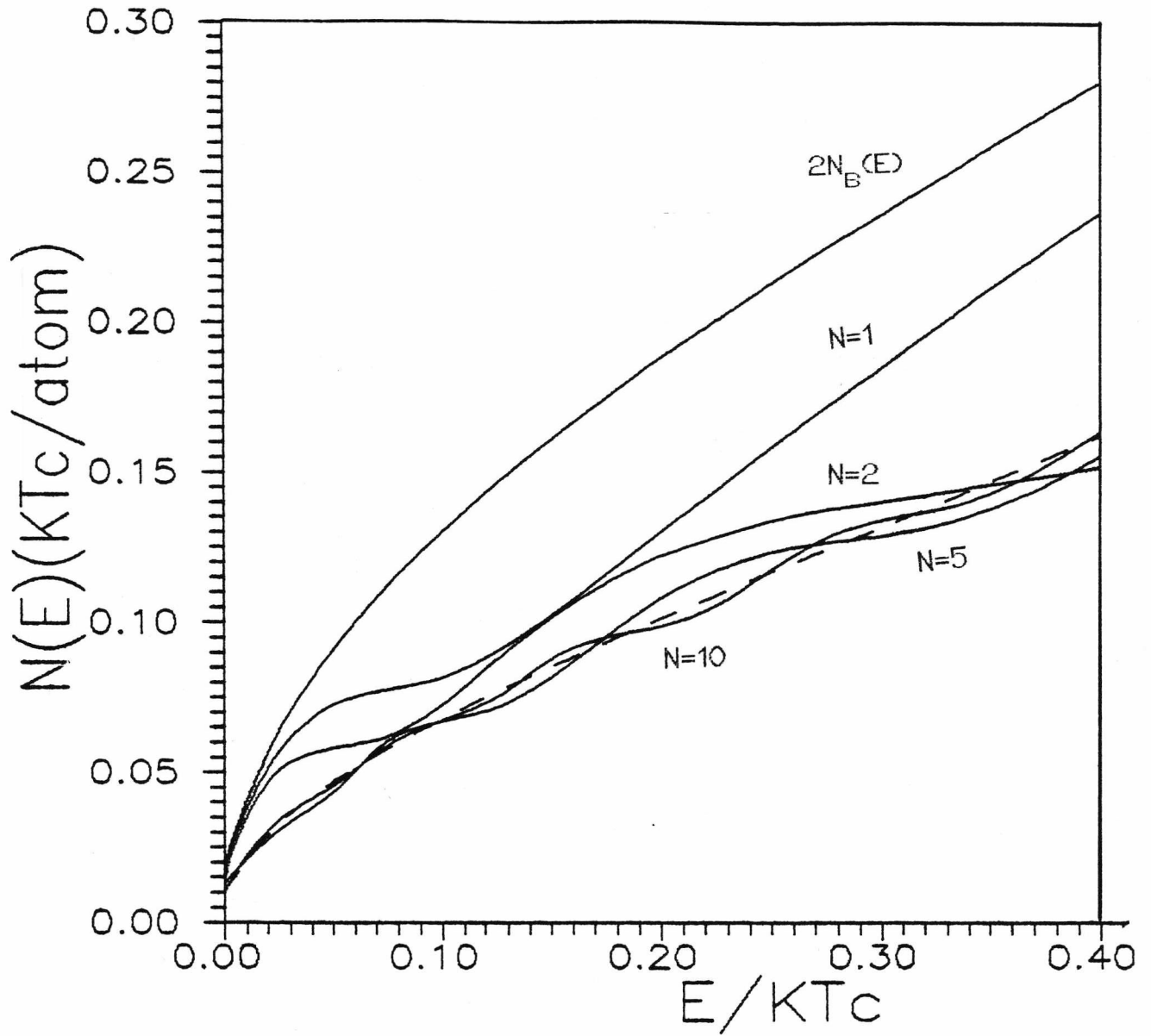
Fig.2.23 The density of spin wave states in the subsurface layer n=1, 2, 5 and 10 for an overlayer with softened surface-bulk exchange J_{10}/J=0.3 . The broken curve denotes the DOS of the bulk N_B(E) and the curve 2N_B(E) denotes the DOS of a geometric surface.
