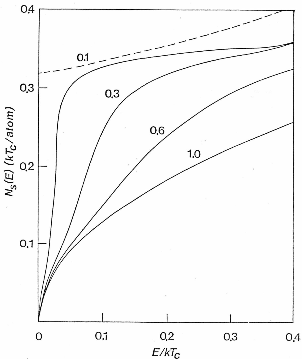
Fig.2.3 Calculated density of spin wave states N_s(E) in the (100) surface of sc ferromagnet with a softened exchange integral J_{10} perpendicular to the surface. The values of J_{10}/J are 0.1, 0.3, 0.6 and 1.0. The DOS of a two-dimensional ferromagnet is denoted by broken curve.
