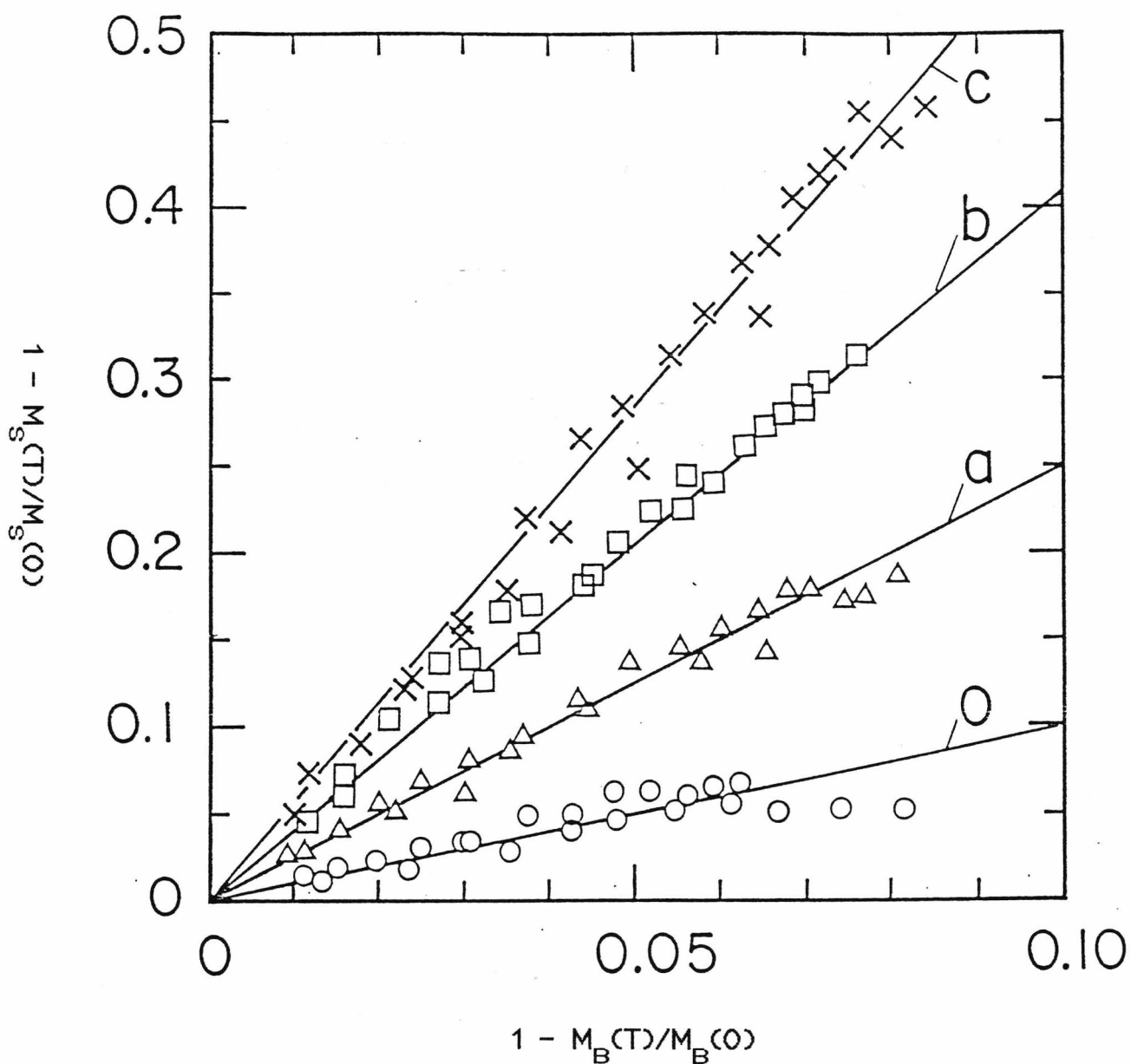
Fig.2.13 Experimental results of Mauri et al. (1989) for M_s(T) in FeNi-Ta-FeNi sandwich. The surface M_s(T) is plotted against the bulk M_b(T) for three thicknesses of Ta interlayer: 0.5, 1.0, 1.5 at. layer (curves a, b, c; 0 is for clean permalloy surface).
