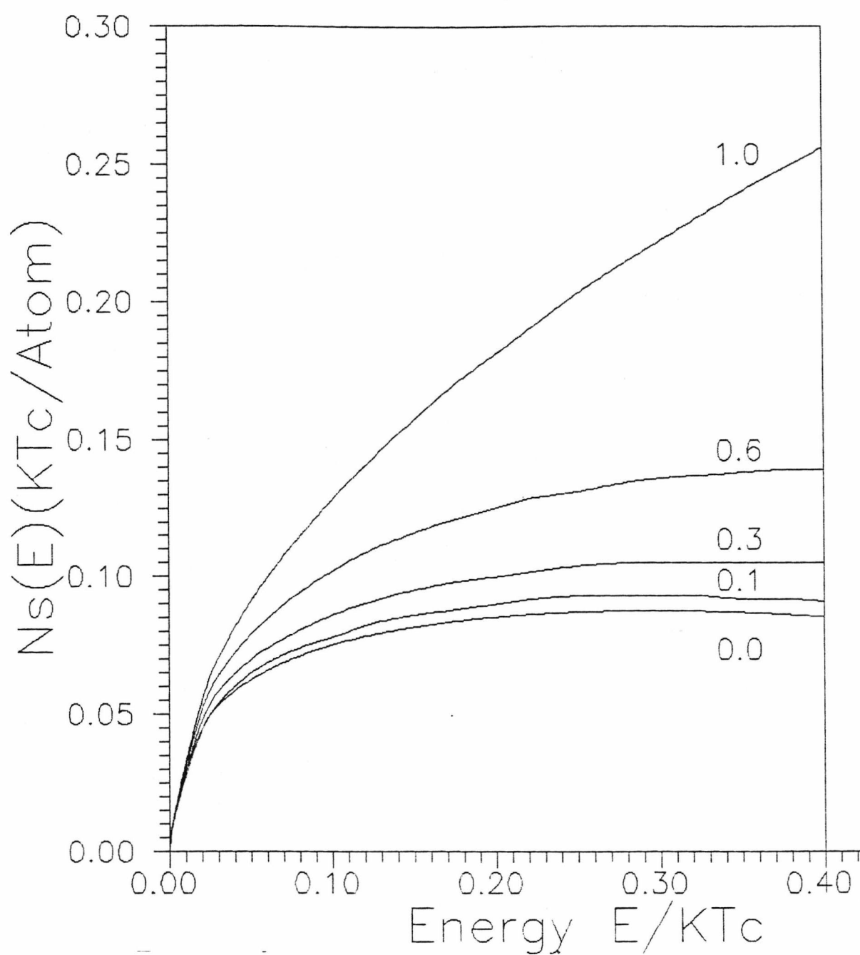
Fig.2.4 The surface density of spin wave states N_s(E) for an atomic overlayer above (100) surface of sc ferromagnet with a softened parallel exchange J_{11} . The values J_{11}/J are 0.0, 0.1, 0.3, 0.6 and 1.0.
