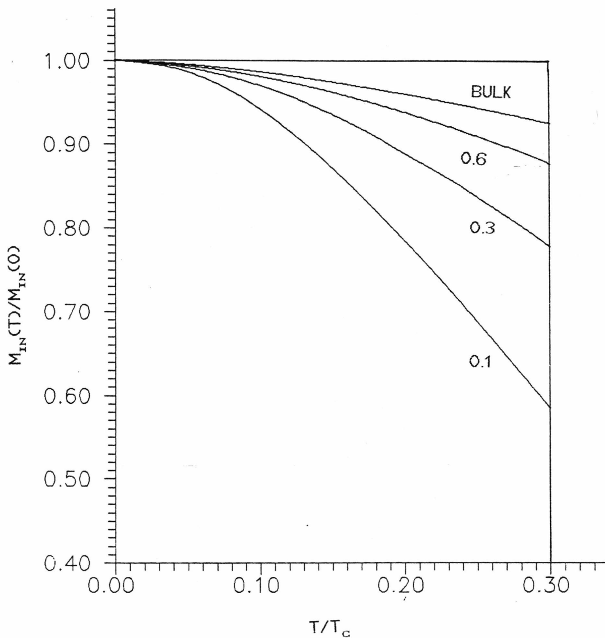
Fig.3.8 Calculated temperature dependence of interface magnetization M_{IN}(T)/M_{IN}(0) in the middle of an interface consisting of two at. atomic layers with a softened parallel exchange J_{||} . The values of J_{||}/J are 0.1, 0.3 and 0.6.
