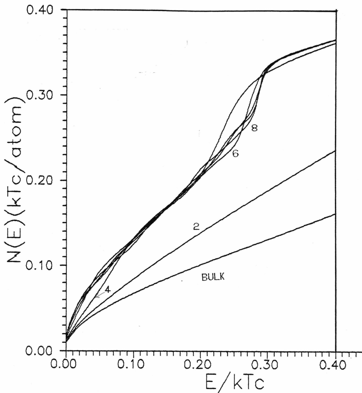
Fig.3.5 Calculated density of spin wave states N(E) in the middle of an interface for various thicknesses of interface N : 2, 4, 6, 8 and 10. The perpendicular exchange integral is J_{\perp}/J=0.3 . Asymptotic behaviour is attained for N \geq 10 .
