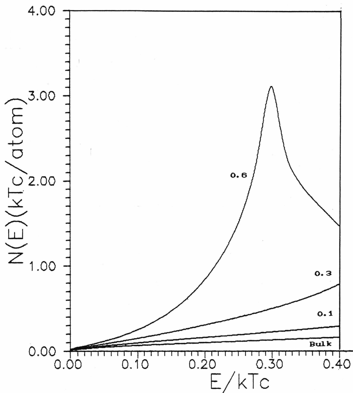
Fig.3.3 Calculated density of spin wave states N(E) in the (100) interface separating two identical semi-infinite Heisenberg ferromagnets. Only the parallel exchange J_{\parallel} within the interface layer is softened. The values of J_{\parallel}/J are 0.1, 0.3 and 0.6.
