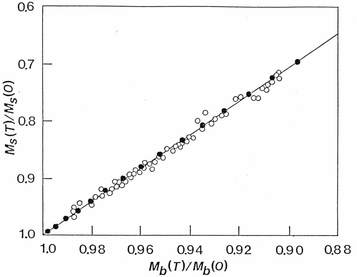
Fig.2.11 Plot of the temperature dependence of the surface magnetization M_s(T)/M_s(0) against the bulk dependence M_b(T)/M_b(0) . Full circles are the calculated results and open circles are the SPLEED results of Pierce et al.. The first calculated point is for T=0.02T_c and the last for T=0.3T_c .
