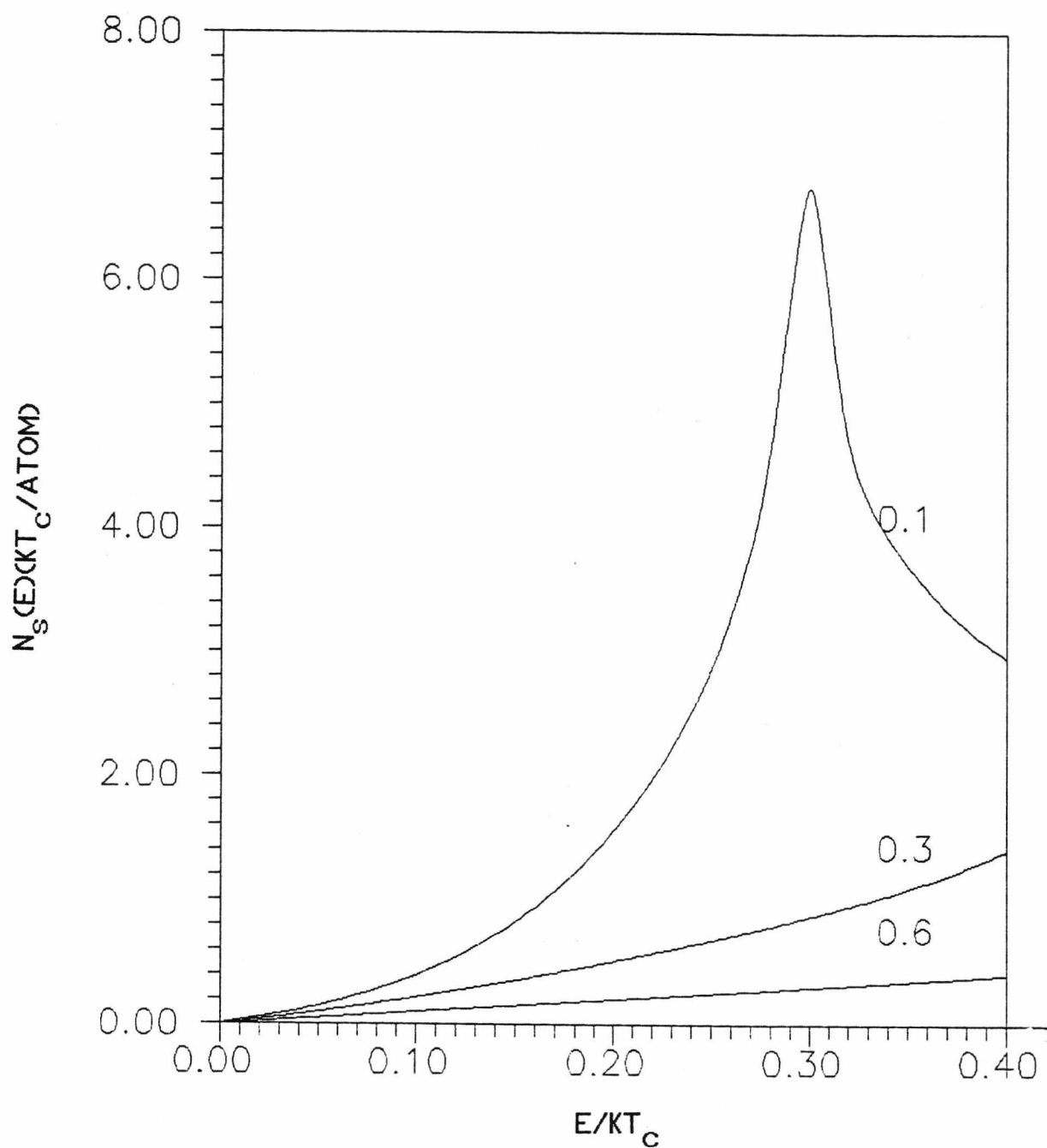
Fig.2.6 The density of states of surface spin waves N_s(E) in the (100) surface of a sc ferromagnet with a softened parallel exchange J_{11} within the surface of overlayer. The values of J_{11}/J are 0.1, 0.3 and 0.6.
