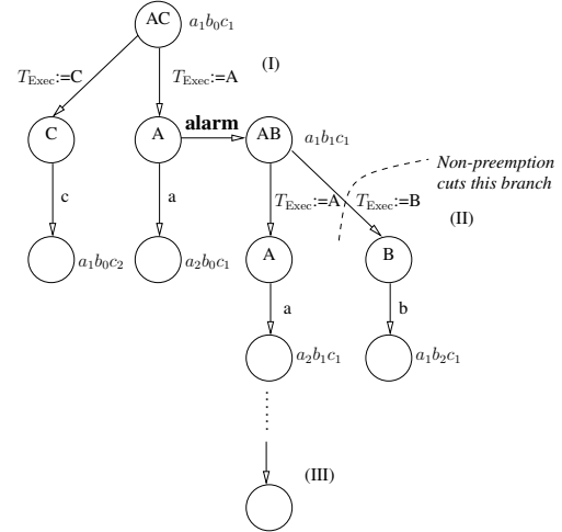
Letters inside states denote tasks able to execute; vectors beside the states show possible values of the task PCs.
