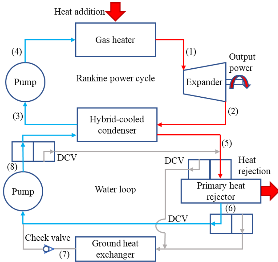
Figure 5.8: Schematic diagram representing mode 2; only primary heat rejector is operating
