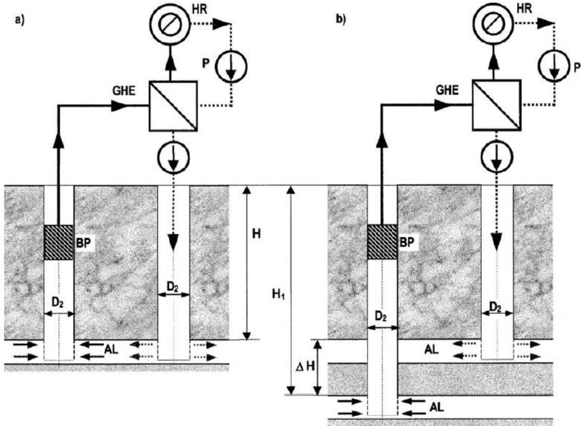
Figure 2.8: Closed two-hole system for extracting geothermal water: (a) one layer, (b) two layer; aquifer layer (AL), geothermal heat exchanger (GHE), pump (P), borehole pump (BP), and heat reservoir (HR) [34]
