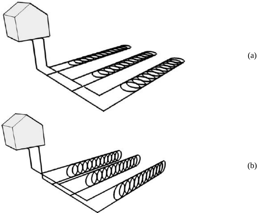
Figure 2.24: Schematics of (a) horizontal and (b) vertical slinky ground heat exchangers [100]
