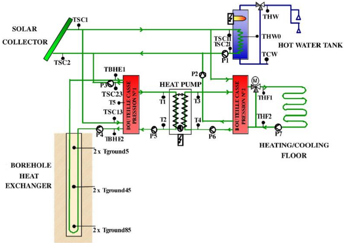
Figure 2.33: Diagram of GEOSOL process proposed by Trillat-Berdal et al. [123]
