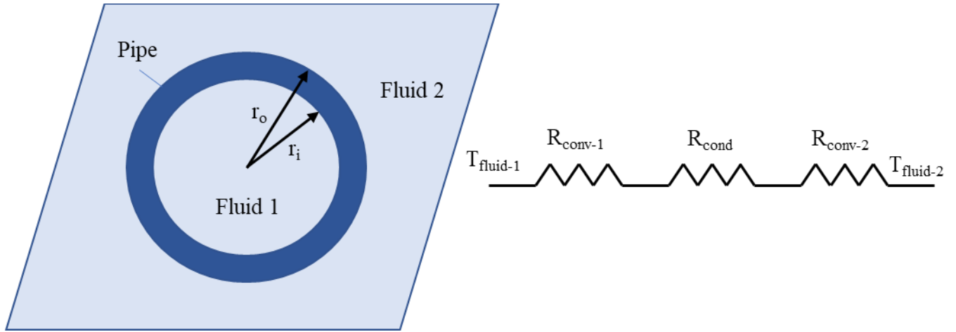
Figure 3.3: Schematic representation for the thermal resistances inside the heat exchanger
