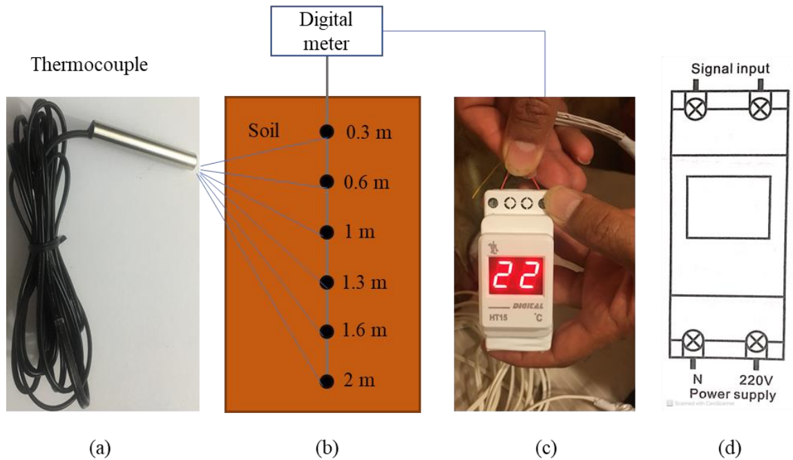
Figure 4.1: Temperature measuring setup; (a) thermocouple, (b) depths of measurement, (c) digital meter and (d) schematic of digital meter
