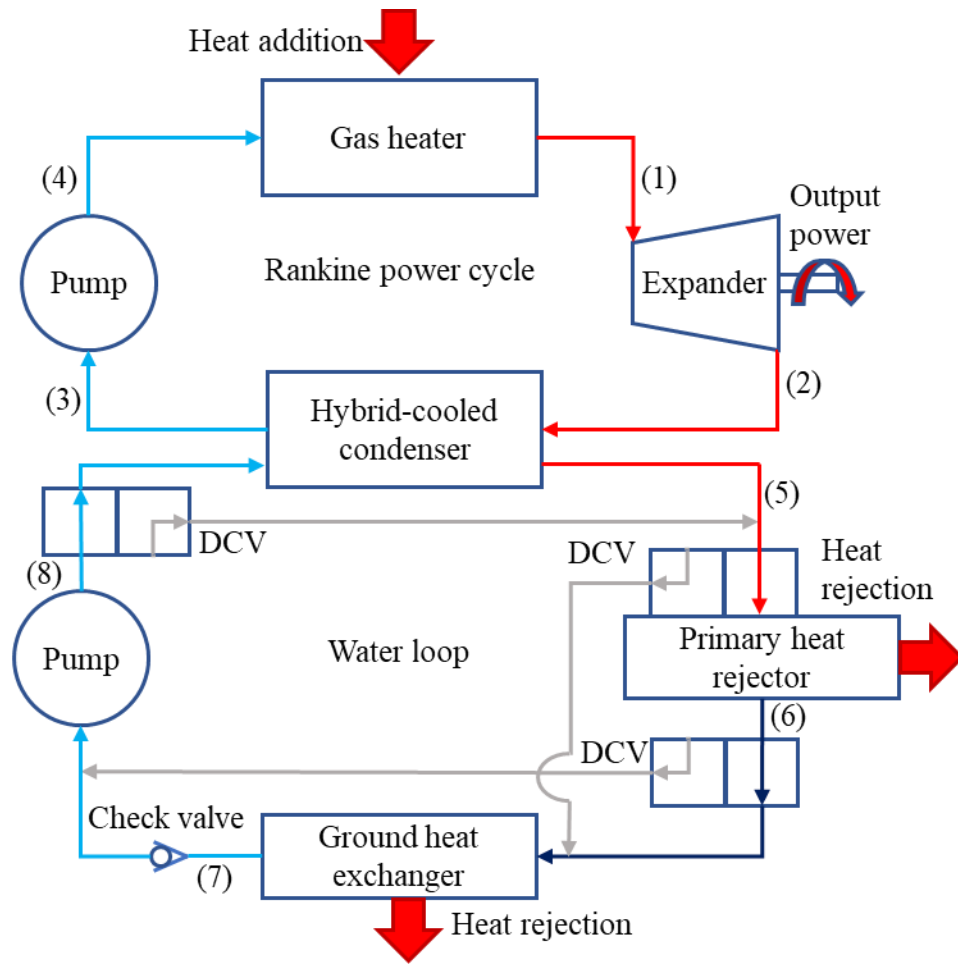
Figure 5.7: Schematic diagram of the normal mode operation
