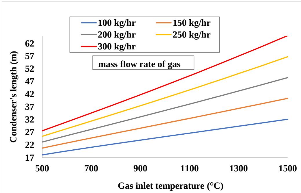
Figure 3.13: The effect of gas conditions (flow rate and temperature) on the condenser's length
