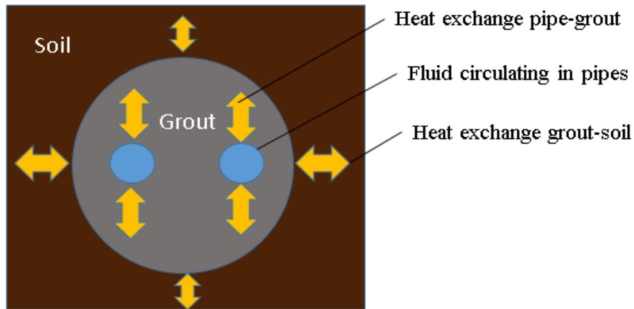
Figure 2.14: Heat transfer inside the ground heat exchanger
