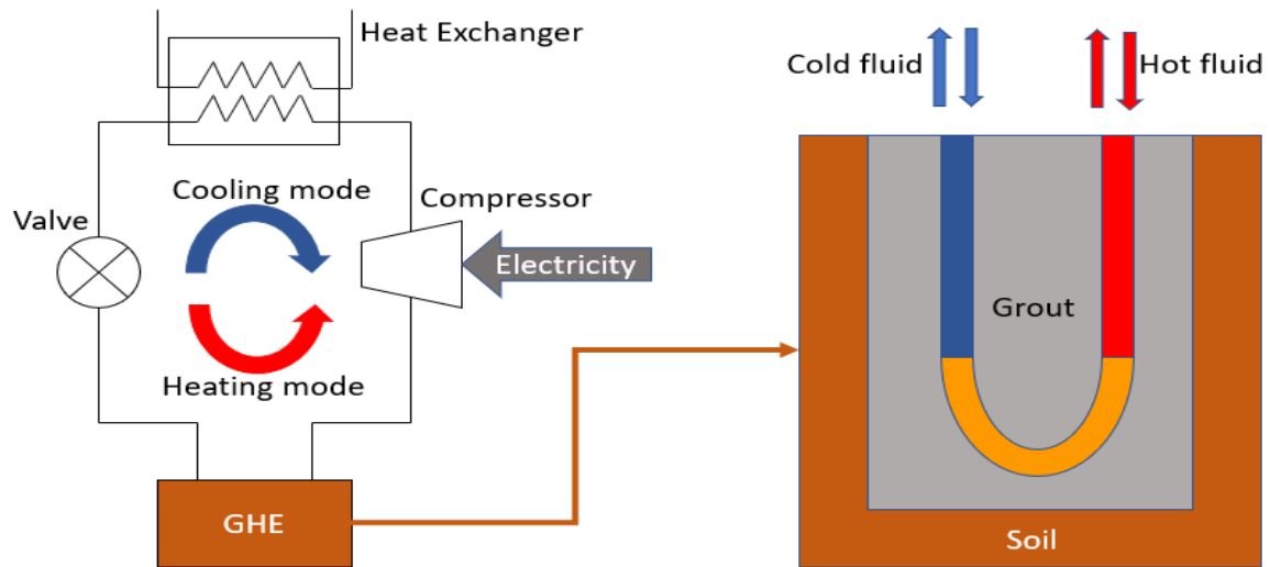
Figure 2.2: The ground source heat pump (GSHP) in heating and cooling modes
