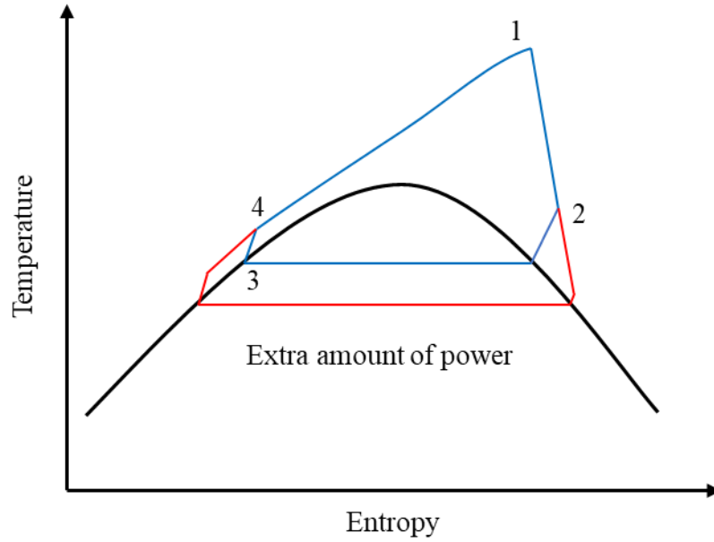
Figure 3.1: Adjusted temperature-entropy diagram of a transcritical Rankine cycle enhanced with a ground cooling system
