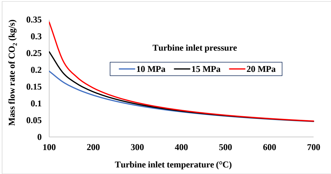
Figure 3.6: The effect of turbine inlet temperature ( T_1 ) on the mass flow rate of CO 2 at different Pressures ( p_1 )
