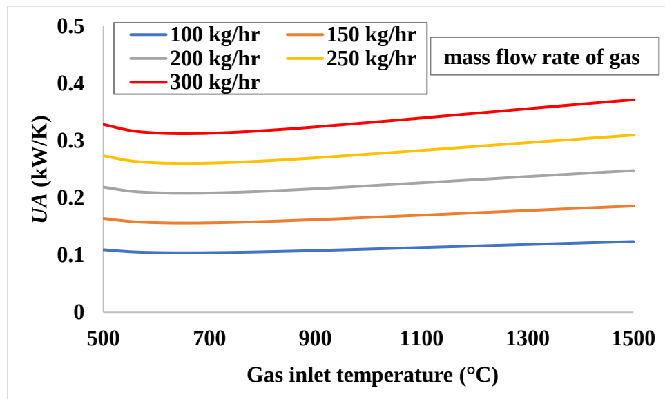
Figure 3.12: The effect of gas conditions (flow rate and temperature) on the UA value of the gas heater
