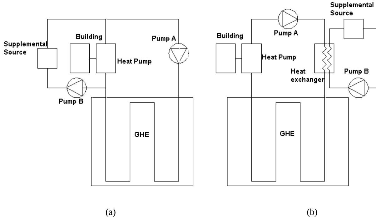
Figure 2.35: Parallel (a) vs. serial (b) hybrid ground source heat pump configurations
