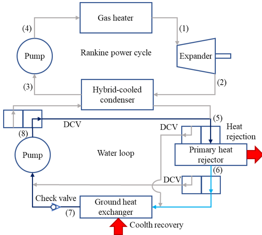
Figure 5.10: Schematic diagram of the recovery operating mode
