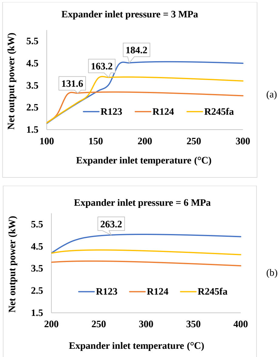
Figure 5.12: Effect of expander inlet pressure on the best point temperature
