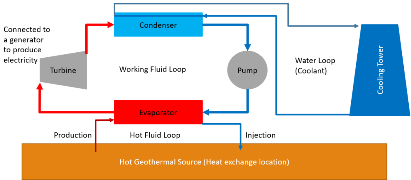
Figure 2.6: Binary geothermal power plant
