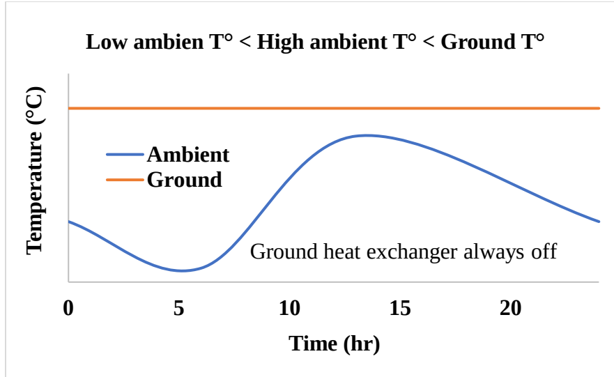
Figure 4.5: Ground cooling system not operating (case 2)
