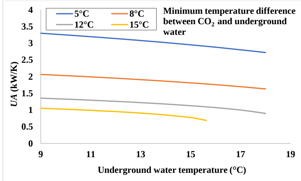
Figure 3.17: The effect of underground water temperature under different minimum temperature differences on the condenser's UA value
