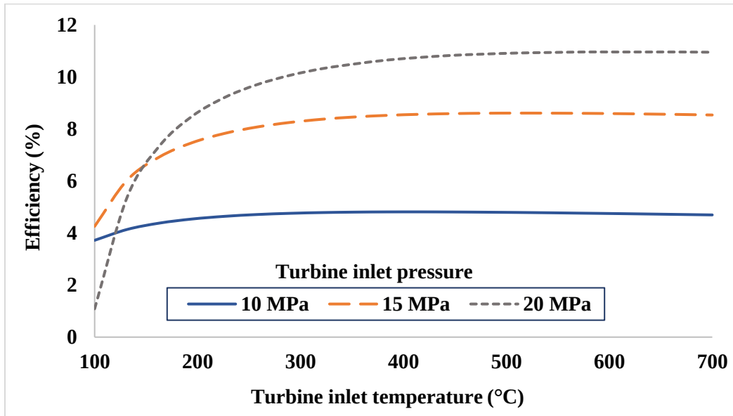
Figure 3.7: The effect of turbine inlet temperature ( T_1 ) on the cycle's efficiency at different pressures ( p_1 )
