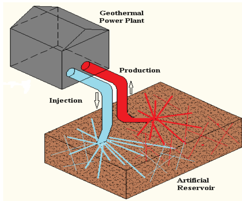
Figure 2.5: Conceptual diagram showing the enhanced geothermal system
