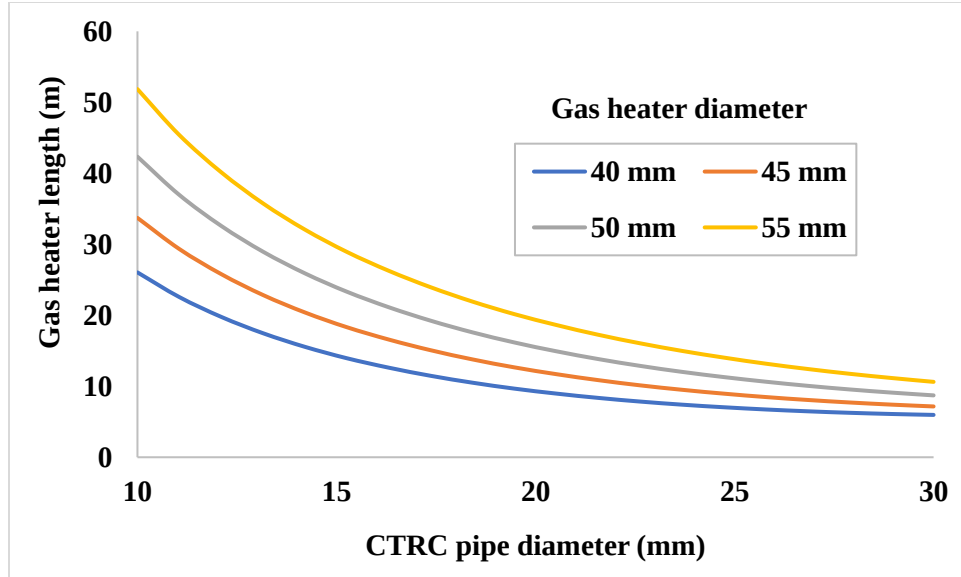
Figure 3.10: The relation between gas heater's length and the diameter of both pipes; gas heater and CTRC
