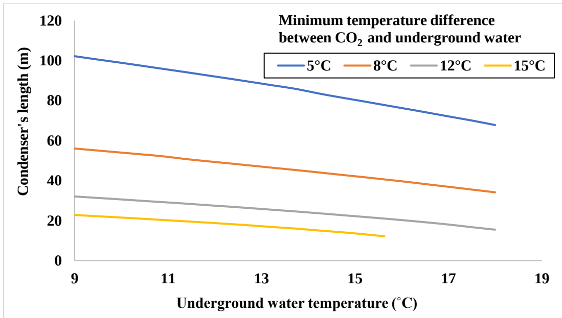
Figure 3.16: The effect of underground water temperature under different minimum temperature differences on the condenser's length
