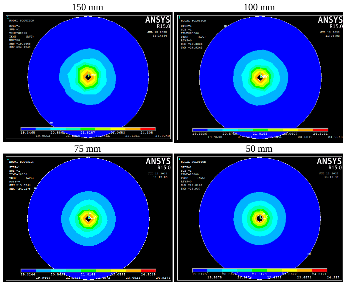
Figure 6.2: Sensitivity analysis based on the element edge size
