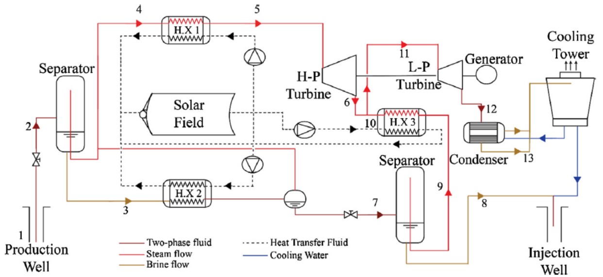
Figure 2.31: Double-flash hybrid power plant [115]
