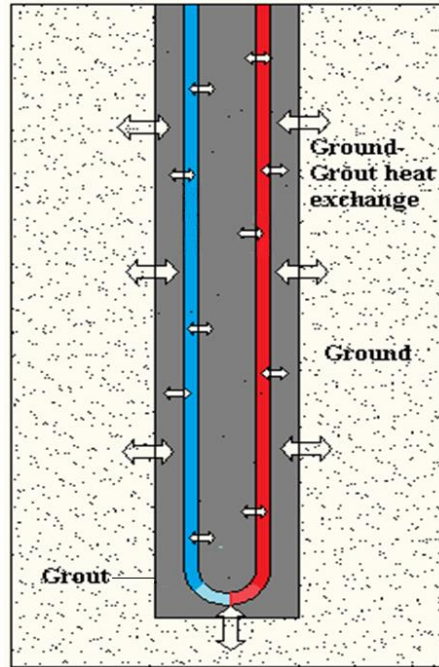
Figure 2.13: Geothermal borehole heat exchanger
