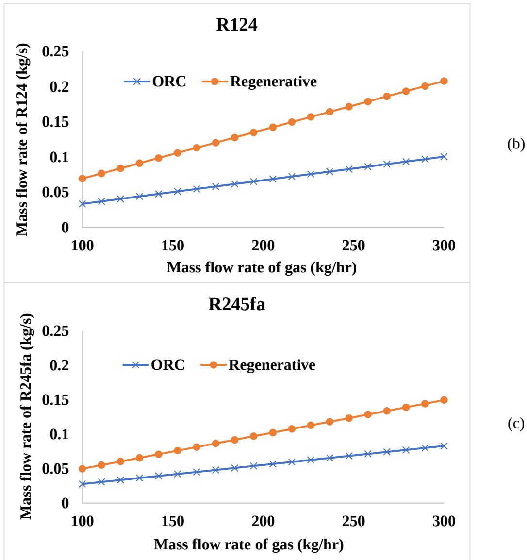
Figure 5.19: The relation between mass flow rate of heat source and working fluids in basic and regenerative organic Rankine cycles for (a) R123, (b) R124 and (c) R245fa
