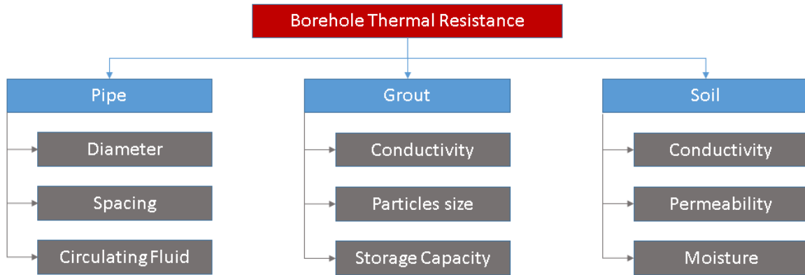
Figure 2.15: Factors that affect the borehole thermal resistance
