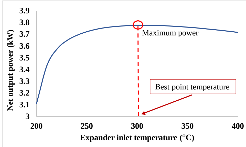
Figure 7.1: The variation of net output power as function of expander inlet temperature for R123 at 5 MPa
