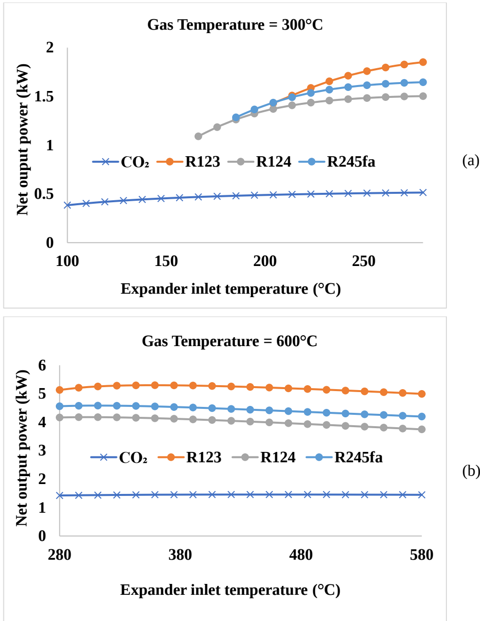
Figure 5.11: Effect of gas and expander inlet temperatures on the performance of working fluids
