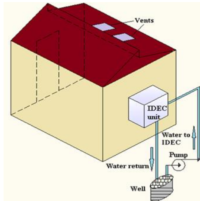
Figure 2.4: Using well water to activate the indirect-direct evaporative cooling (IDEC) system, reproduced from [22]
