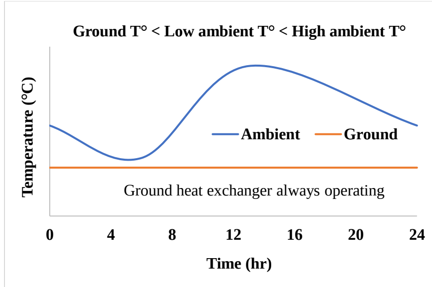
Figure 4.4: Ground cooling system operating the entire day (case 1)
