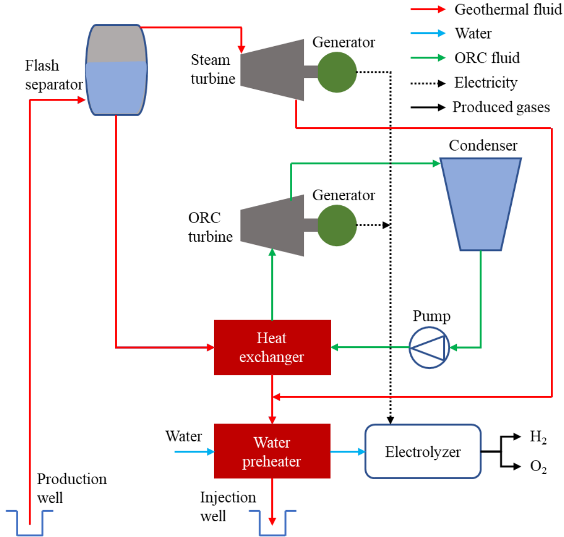
Figure 2.10: Hydrogen production using flash-binary geothermal power plant
