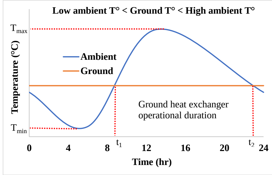
Figure 4.6: Ground cooling system partially operating (case 3)
