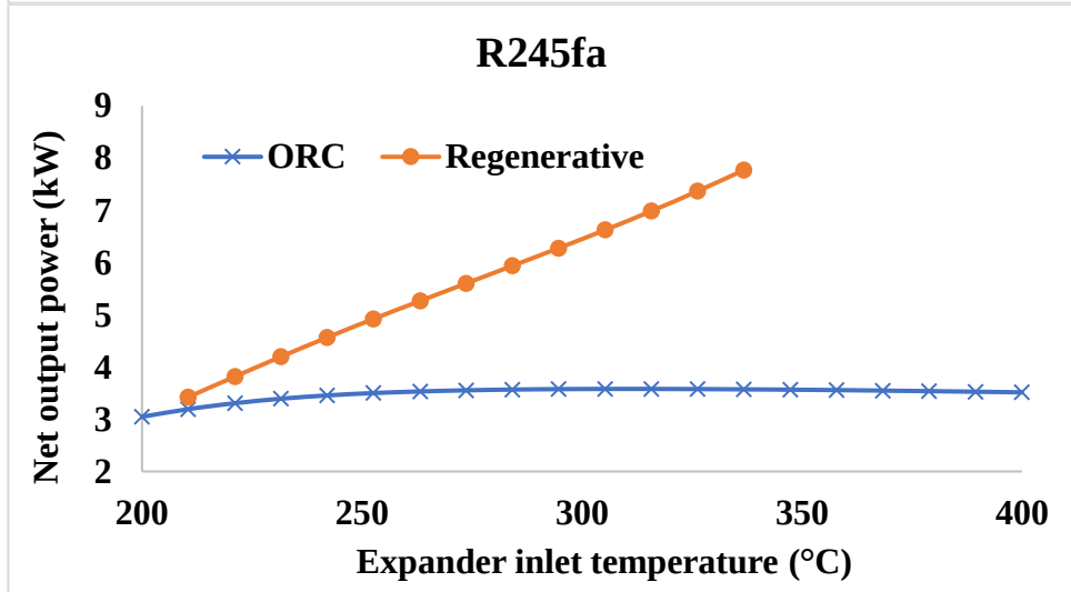
Figure 5.16: Effect of expander inlet temperature on the net output power of basic and regenerative organic Rankine cycles for (a) R123, (b) R124 and (c) R245fa
