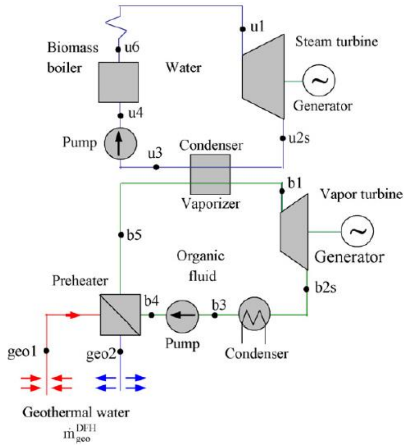
Figure 2.37: Dual fluid hybrid geothermal-biomass power plant [135]
