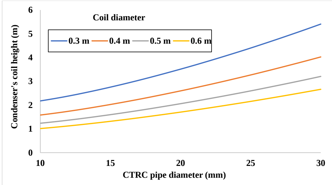
Figure 3.18: The variation of condenser's coil height with respect to the pipe and coil diameters
