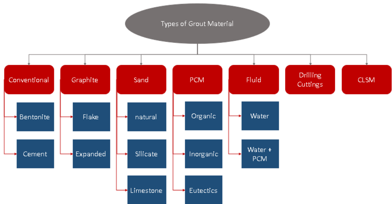
Figure 2.17: The types of grout materials that could be used in a borehole heat exchanger
