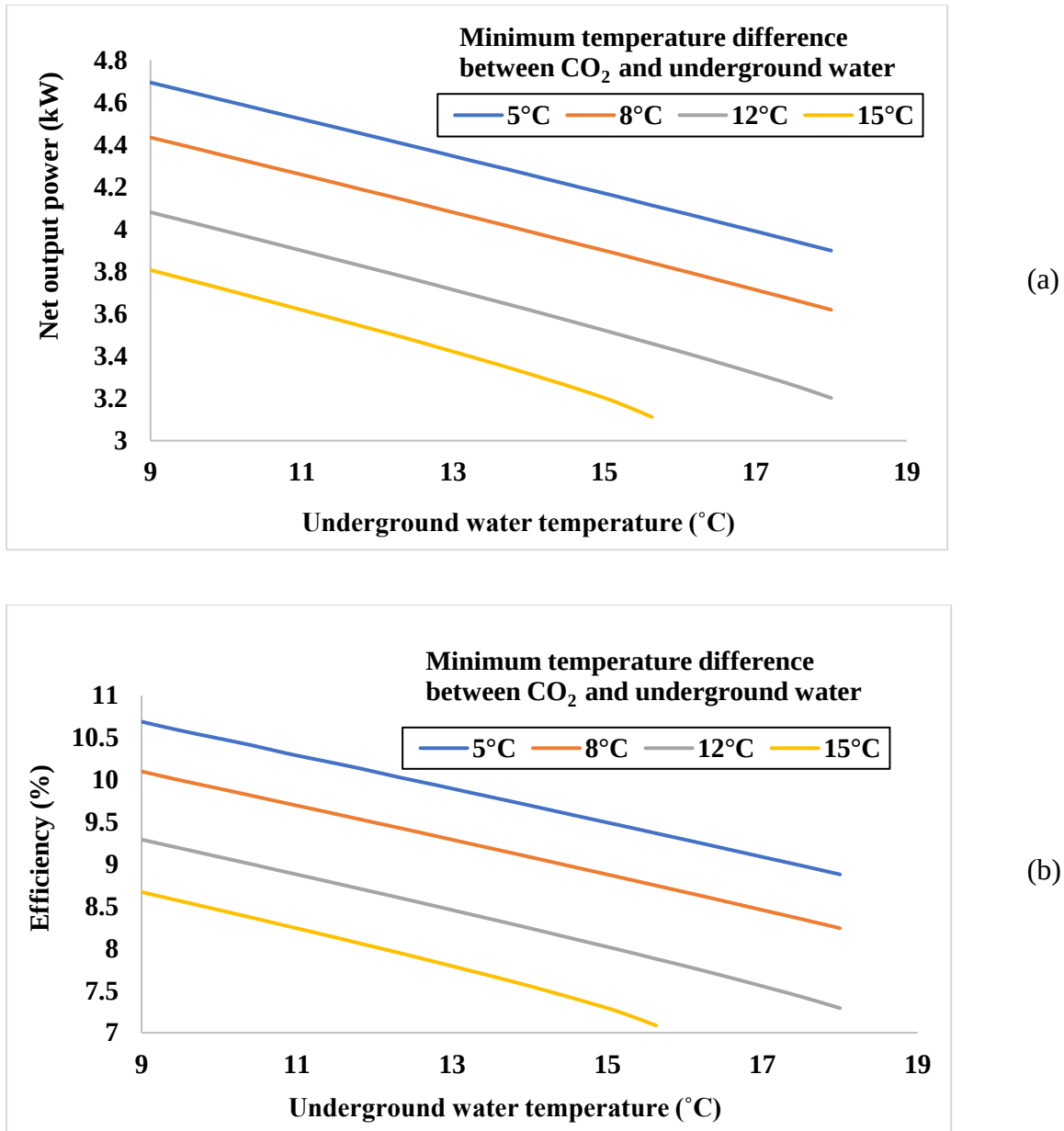
Figure 3.9: The effect of underground water temperature on the cycle's performance with respect to the minimum temperature difference in the condenser
