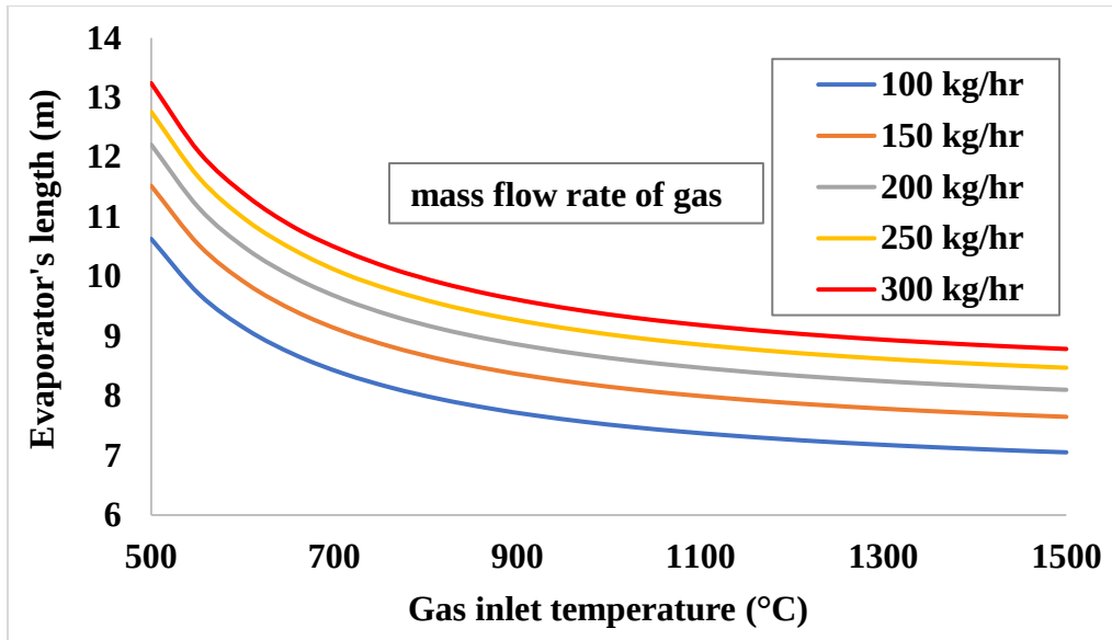
Figure 3.11: The effect of gas conditions (flow rate and temperature) on the gas heater's length
