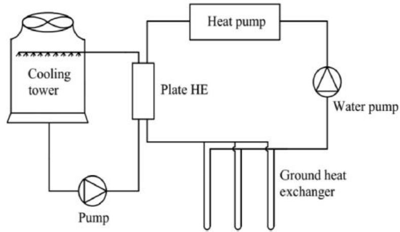
Figure 2.34: Ground source heat pump coupled with a cooling tower [126]
