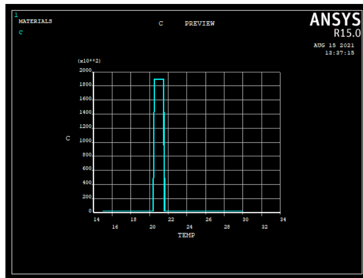
Figure C.1: The variation of RT 21HC specific heat with respect to the temperature and change of phase
