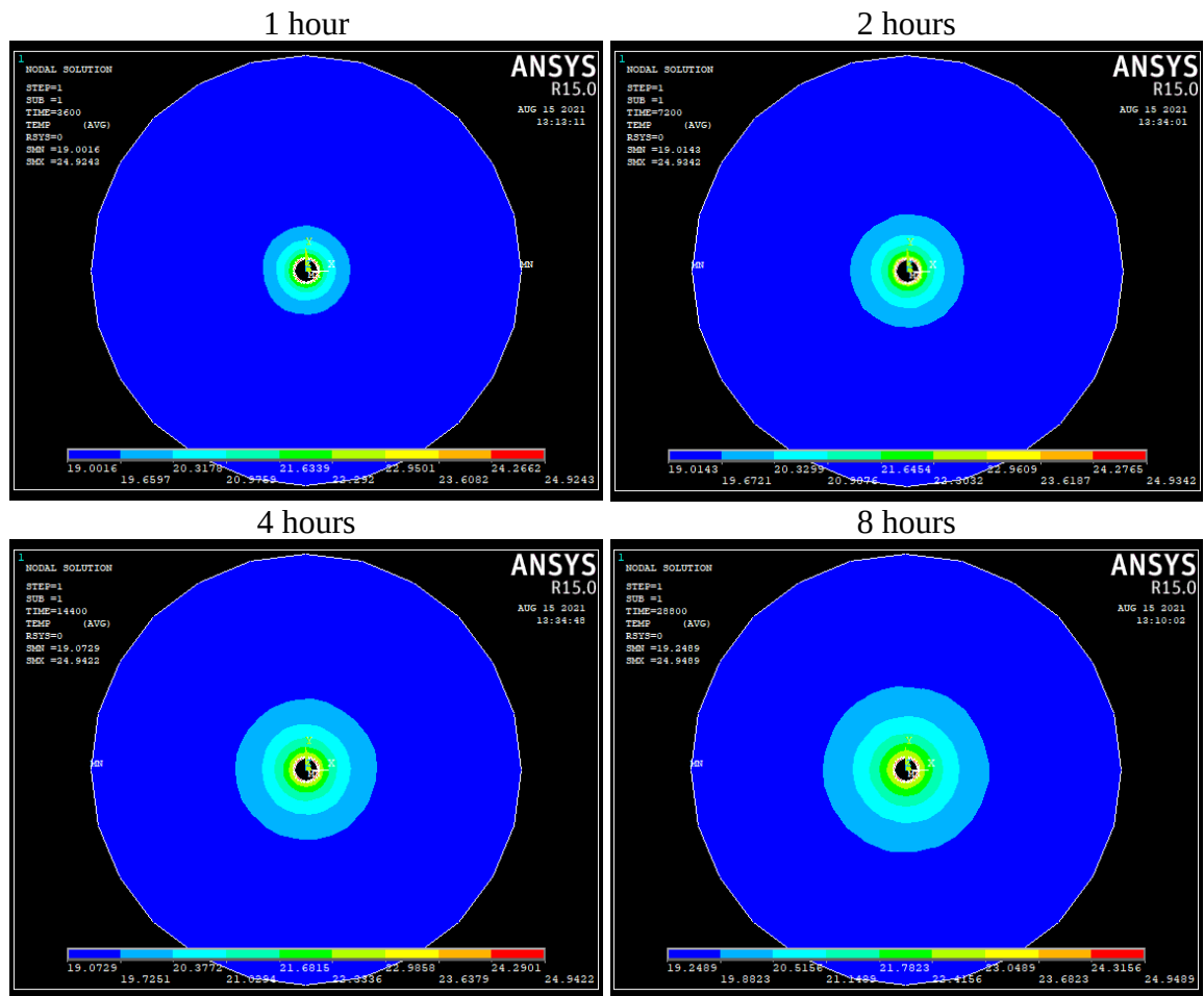
Figure 6.4: The nodal thermal distribution in soil using RT 21HC as a phase change material
