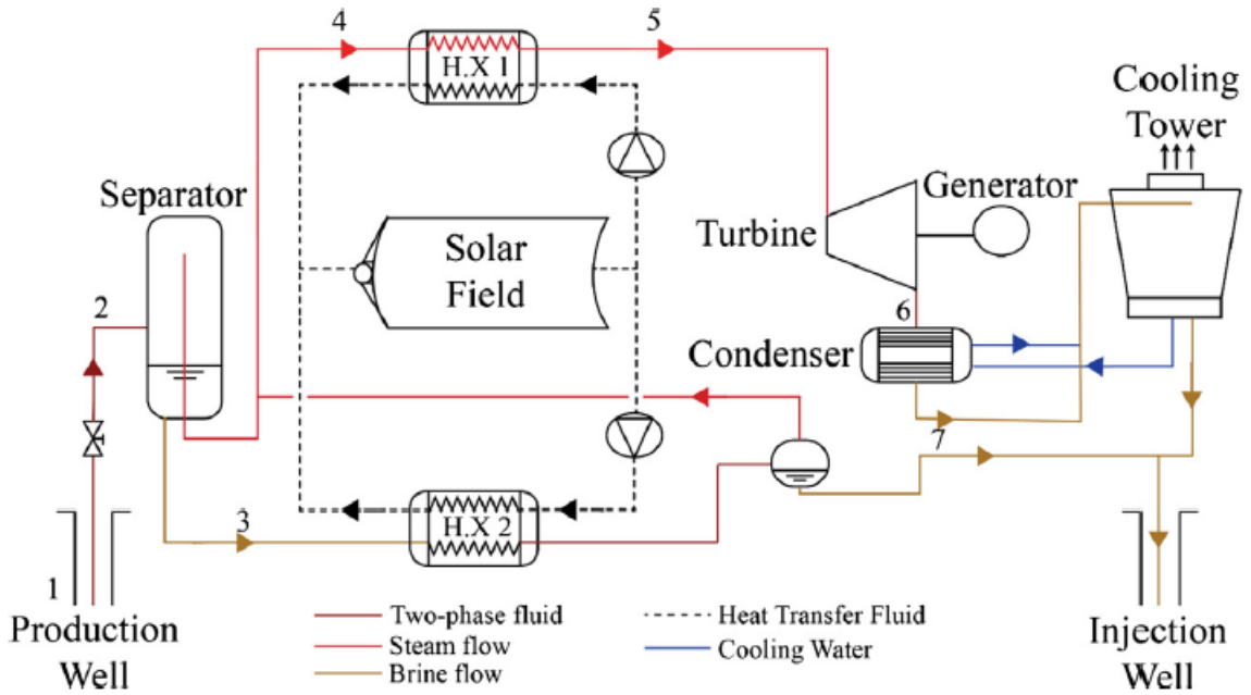
Figure 2.30: Single-flash hybrid power plant [115]
