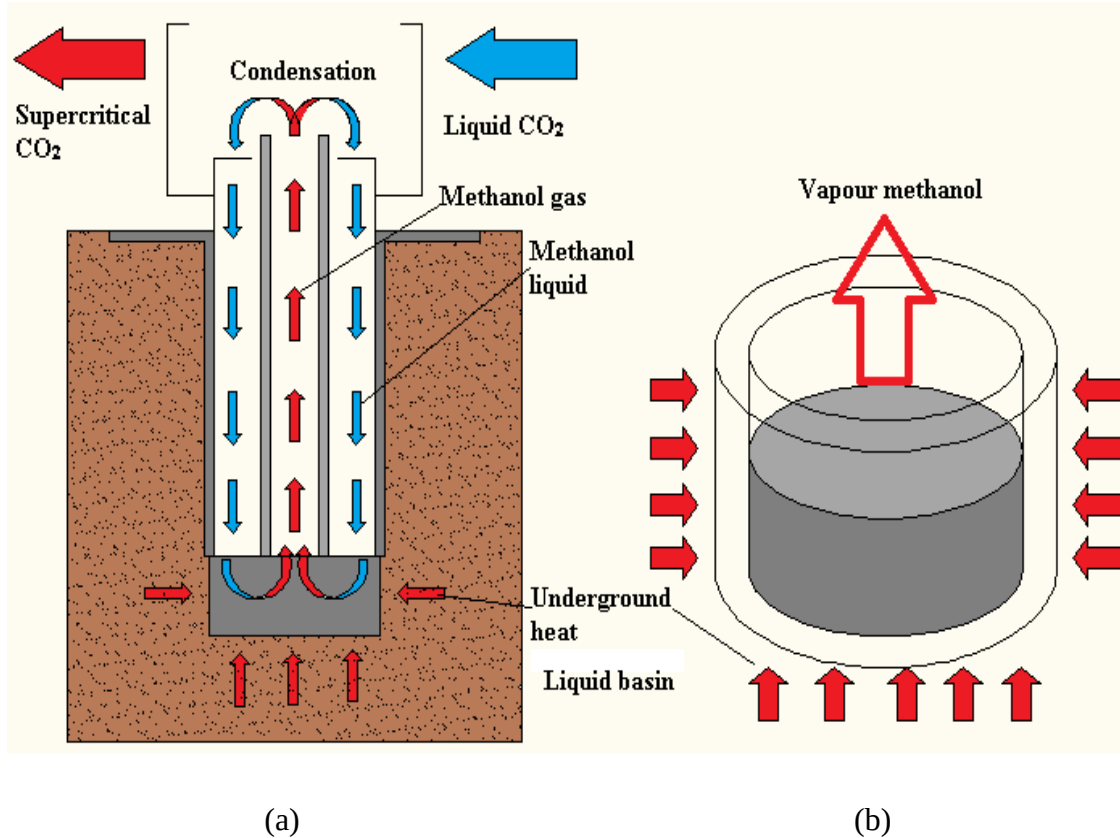
Figure 2.7: (a) Low-temperature geothermal heat pipe and (b) detail view of a bottom basin, reproduced from [33]
