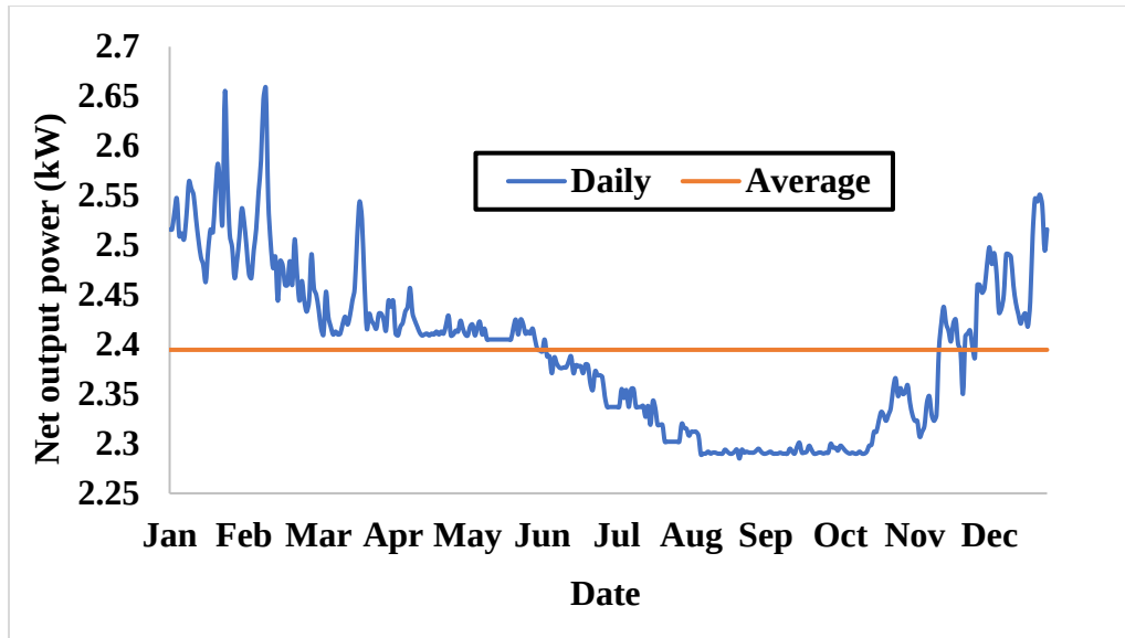
Figure 7.2: The annual energy generated by the organic Rankine cycle
