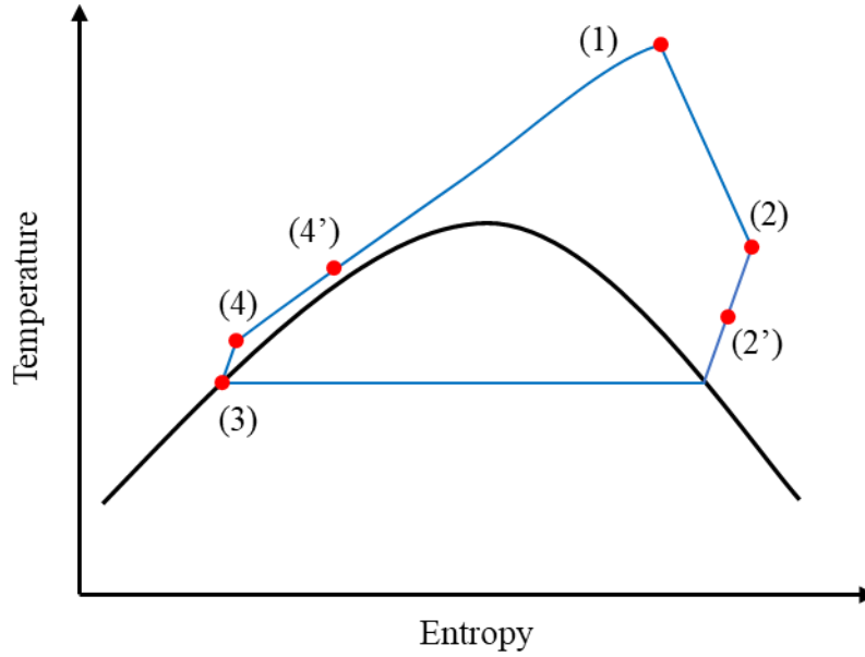
Figure 5.15: Temperature-entropy diagram of the regenerative transcritical organic Rankine cycle
