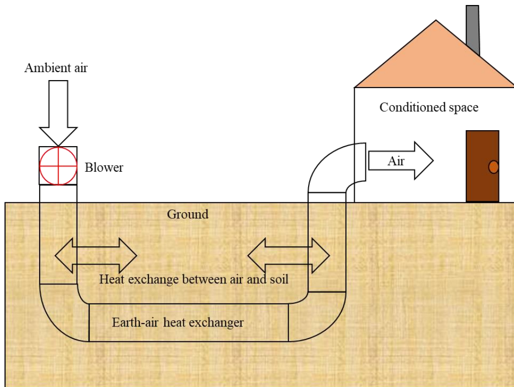
Figure 2.3: Earth-air heat exchanger (EAHE) system
