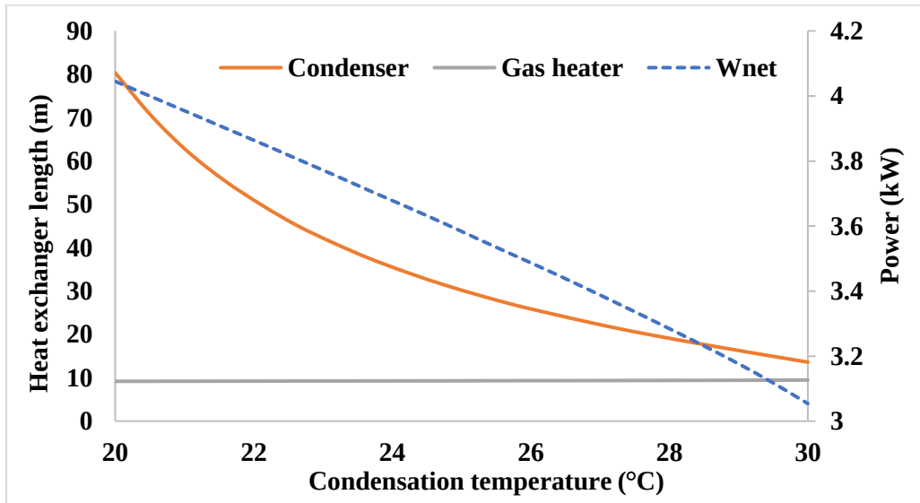
Figure 3.21: The variation of heat exchangers' lengths (gas heater and condenser) and net output power as a function of condensation temperature ( T_3 )
