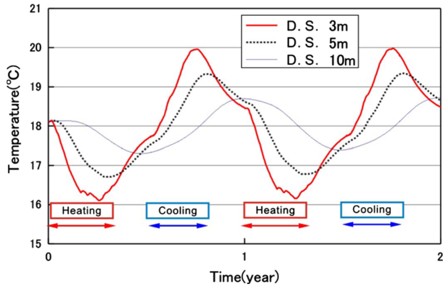
Figure 2.38: Subsurface temperature changes during 2 years at the downstream side (D.S.) of the heat exchanging well at a depth of 35 m [148]
