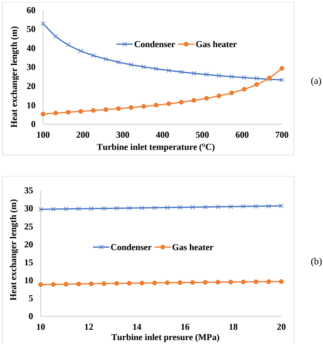
Figure 3.19: The difference between heat exchangers' lengths (gas heater and condenser) with respect to the (a) turbine inlet temperature ( T_1 ) and (b) pressure ( p_1 )
