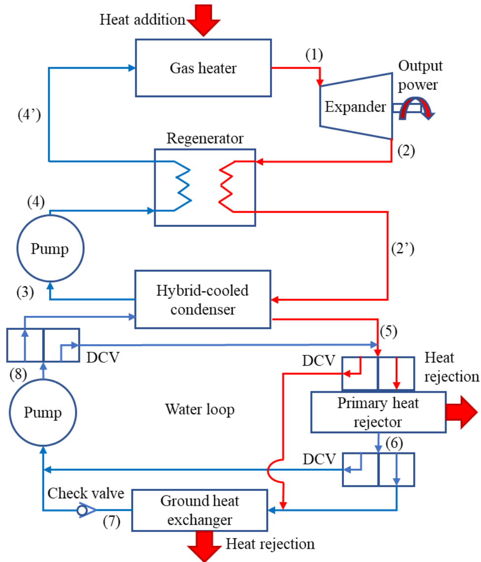
Figure 5.14: Schematic diagram of the regenerative cycle
