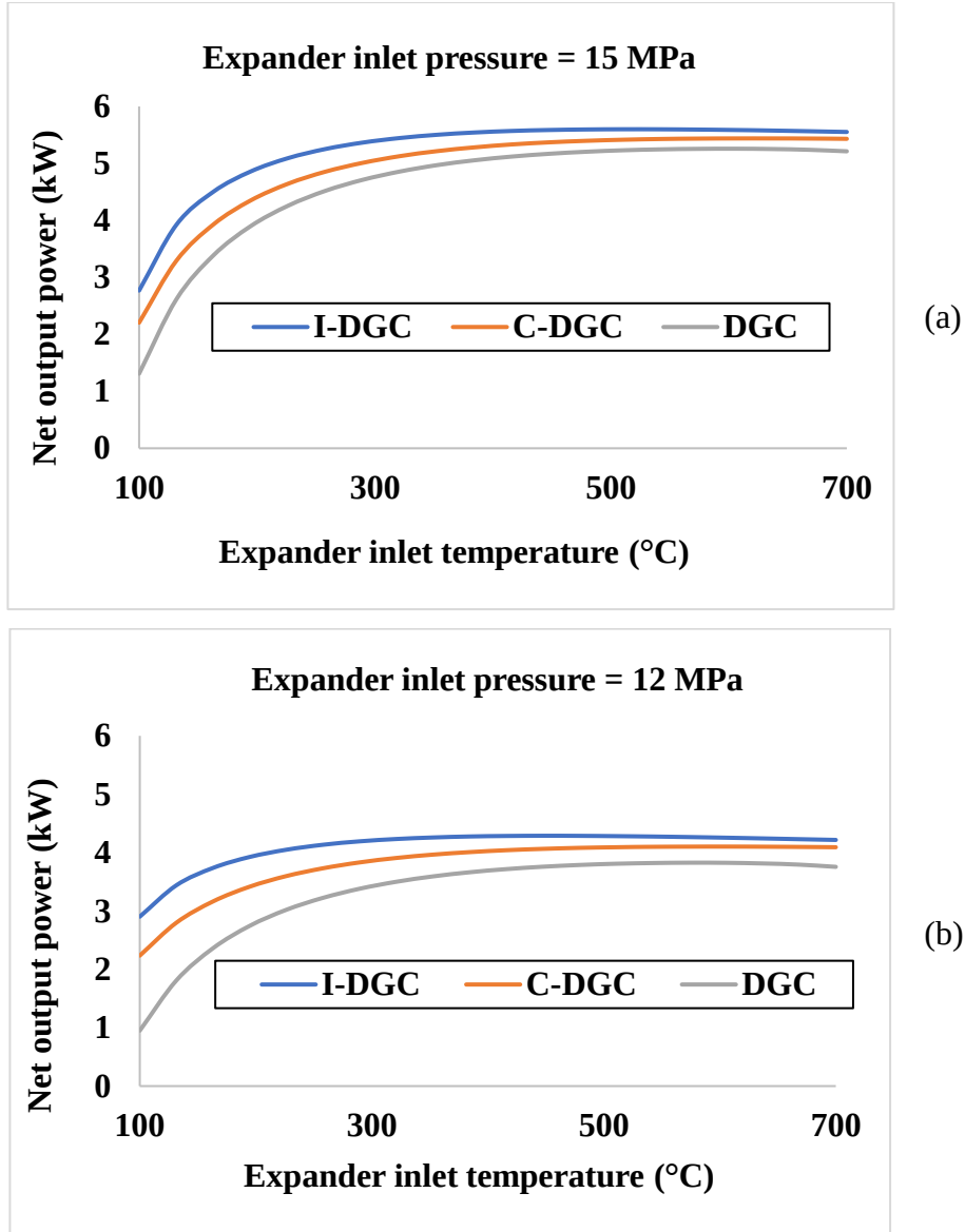
Figure 5.5: The influence of expander inlet conditions on the effect of pressure drops at (a) 15 MPa and (b) 12 MPa
