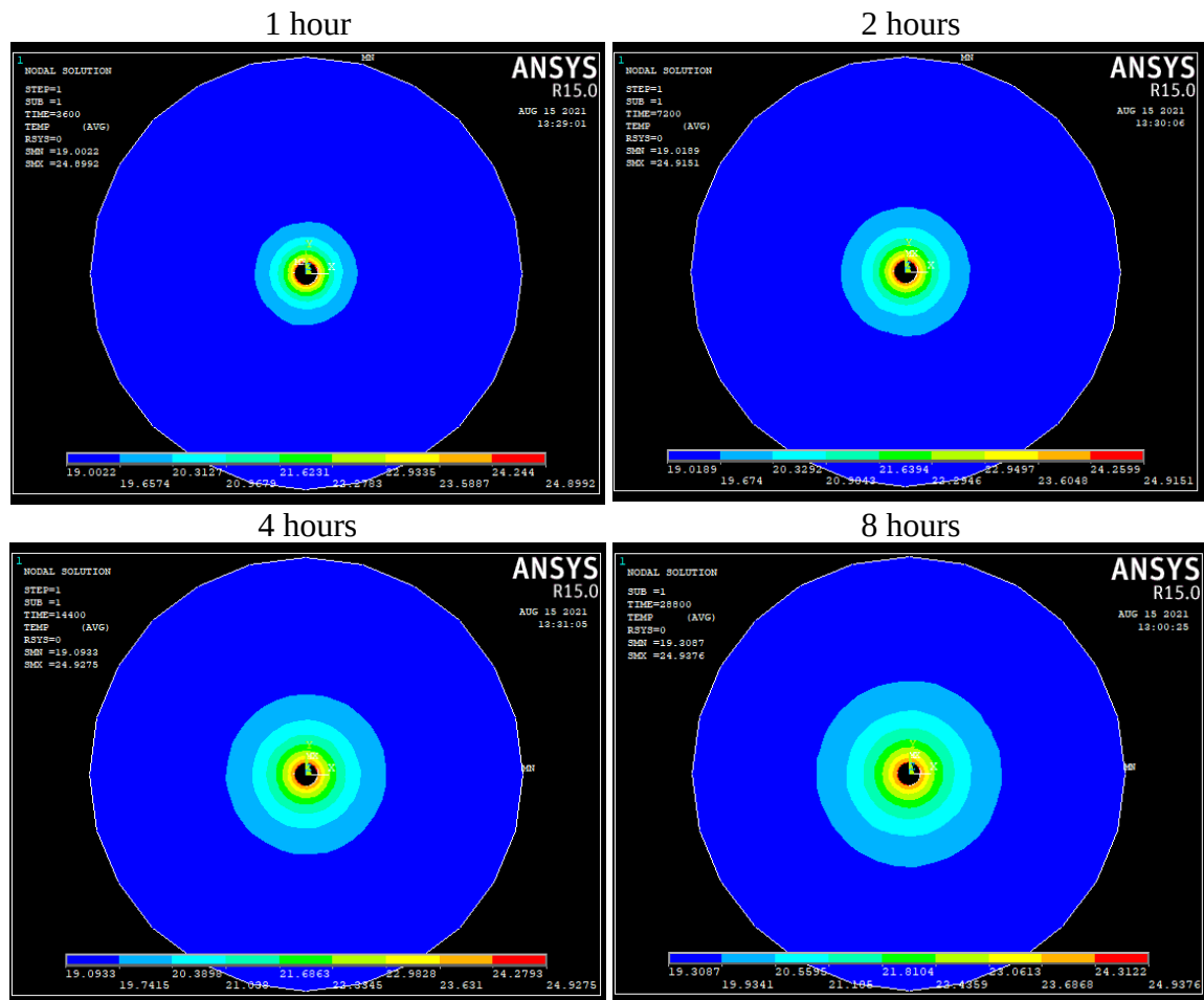
Figure 6.3: The nodal thermal distribution in soil without using phase change materials during 8 hours of operation
