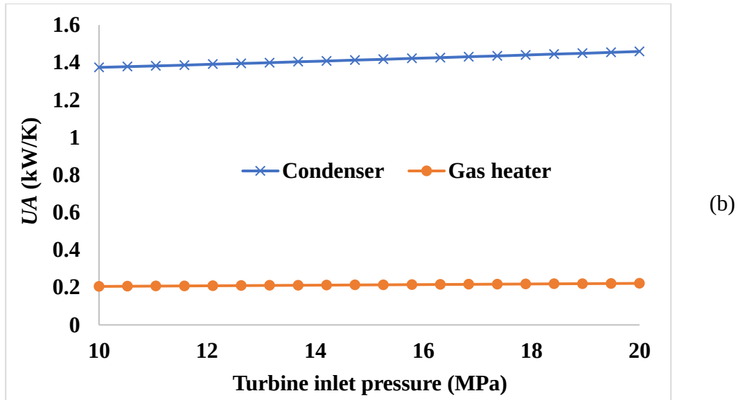
Figure 3.20: The difference between heat exchangers' UA values (gas heater and condenser) with respect to the (a) turbine inlet temperature ( T_1 ) and (b) pressure ( p_1 )
