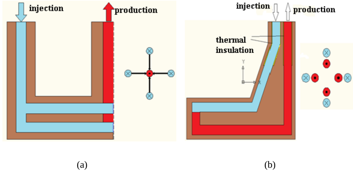
Figure 2.9: (a) Multi-horizontal-well system and (b) annular-well system, reproduced from [35]
