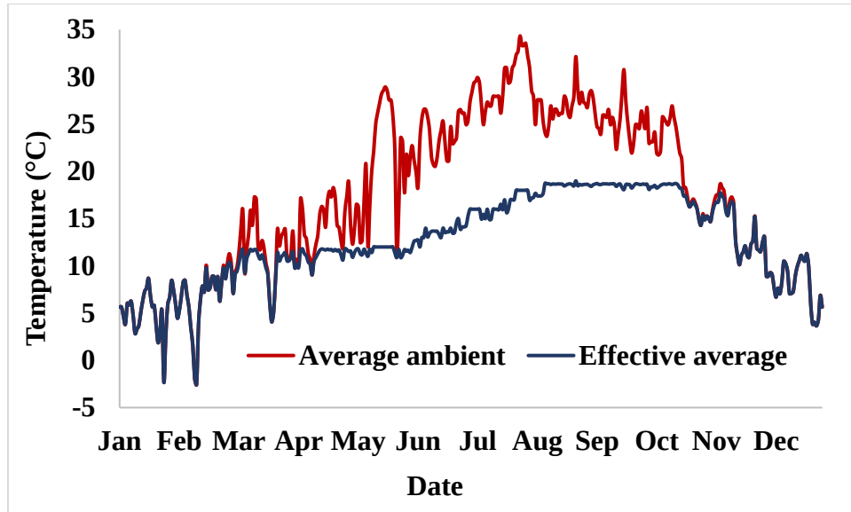
Figure 4.8: The variation of average ambient and effective cooling source temperatures in Bekaa-Lebanon during 2020
