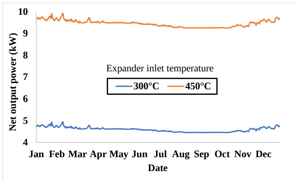
Figure 7.3: The annual energy generated by the regenerative organic Rankine cycle
