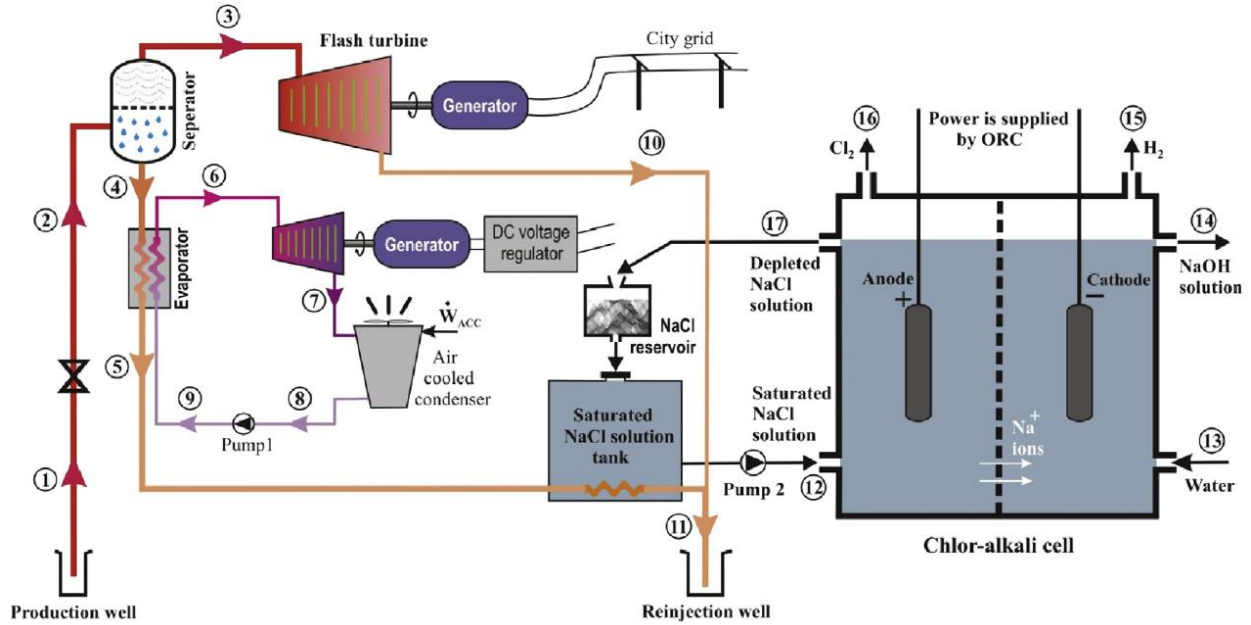
Figure 2.12: Chlor-alkali cell integrated into a geothermal power plant [46]
