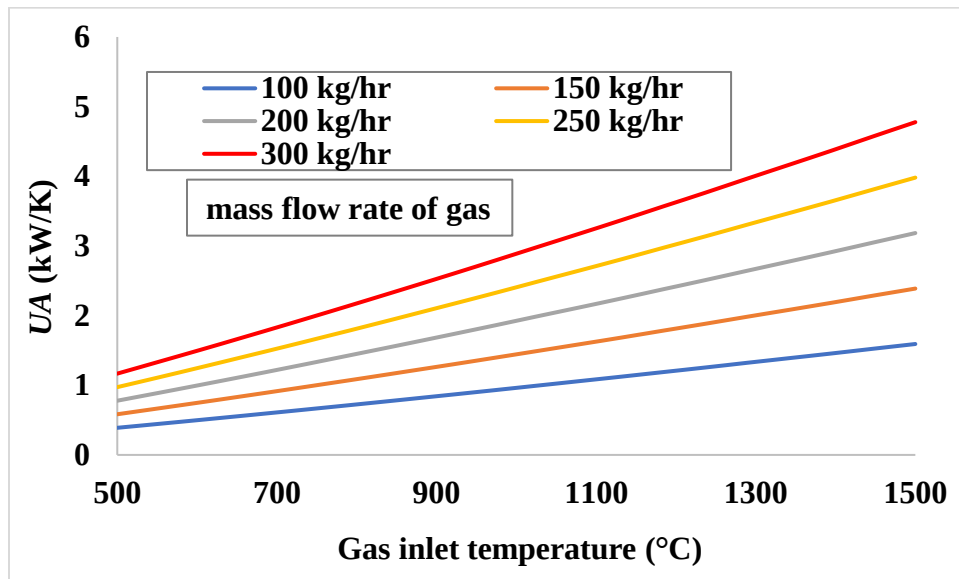
Figure 3.14: The effect of gas conditions (flow rate and temperature) on the UA value of the condenser
