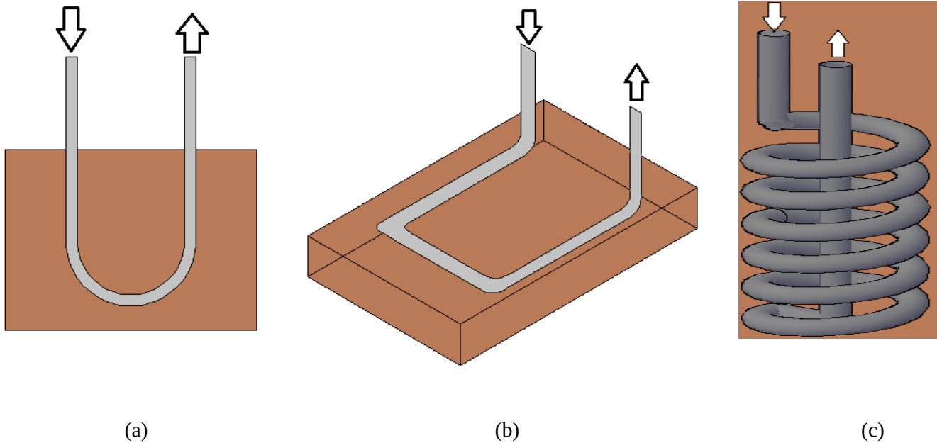
Figure 2.21: Ground heat exchanger configurations; (a) vertical, (b) horizontal and (c) spiral
