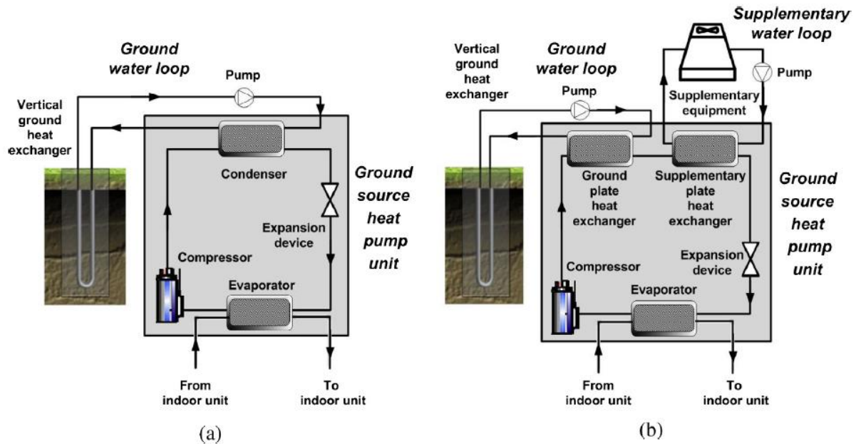
Figure 2.25: Difference between (a) ground source heat pump and (b) hybrid ground source heat pump [103]
