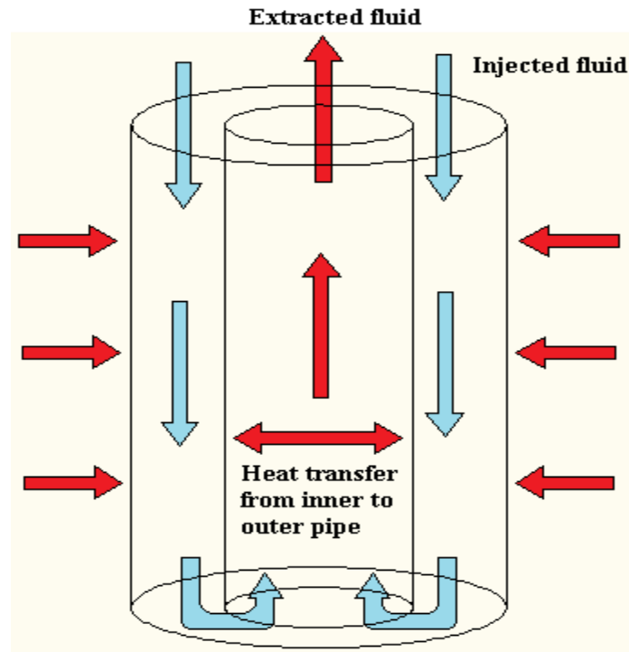
Figure 2.22: Heat transfer through a closed loop double pipe heat exchanger, reproduced from [99]
