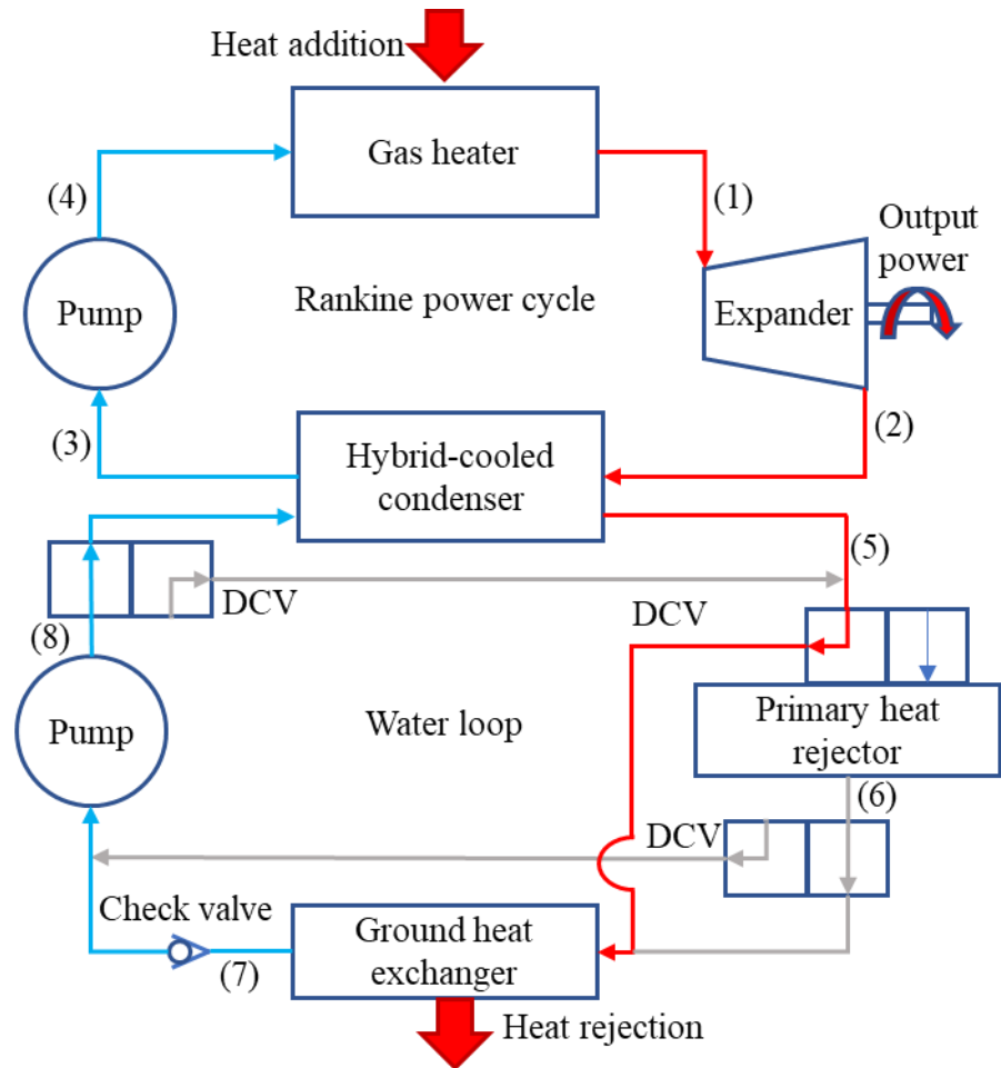
Figure 5.9: Schematic diagram representing mode 3; primary heat rejector is turned off
