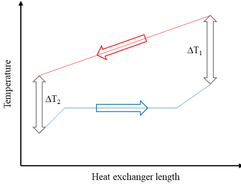
Figure 3.4: The variation of hot and cold fluid temperatures inside a counter flow heat exchanger
