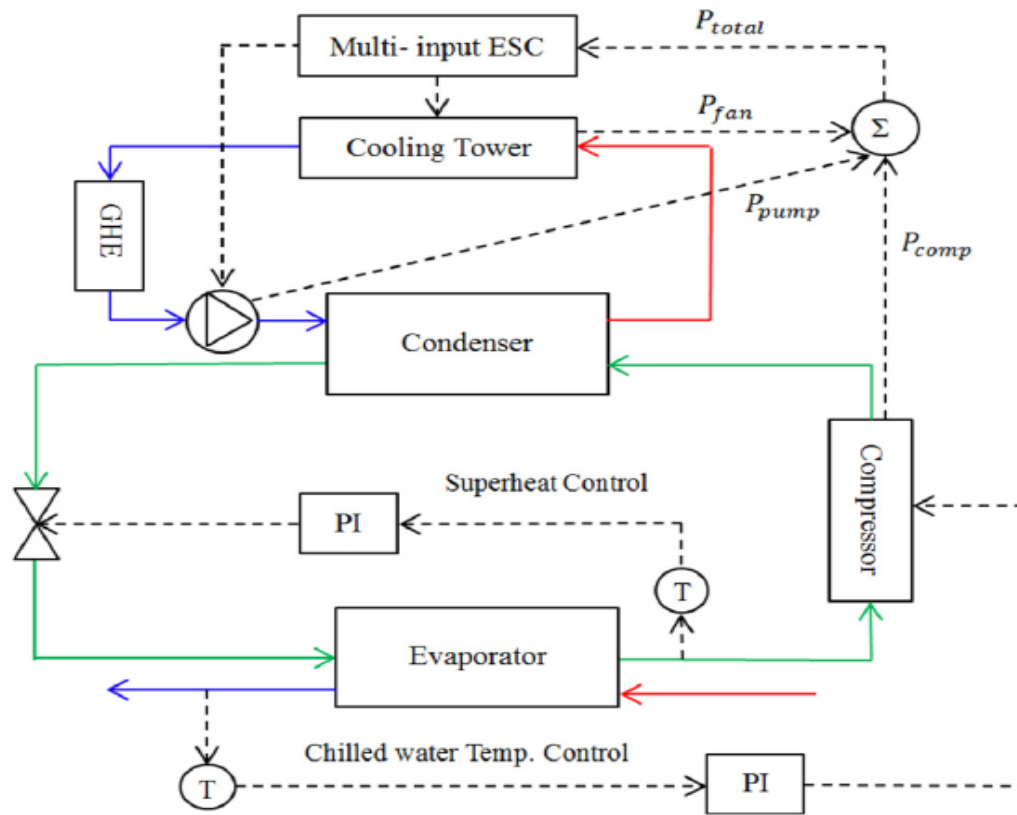
Figure 2.36: Extremum seeking control for optimizing efficiency of hybrid ground source heat pump [126]
