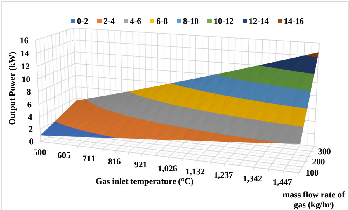
Figure 3.8: The variation of net output power as function of the gas temperature ( T_{gi} ) and its mass flow rate ( \dot{m}_g )
