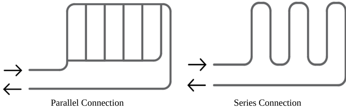
Figure 2.23: Horizontal ground heat exchanger configurations
