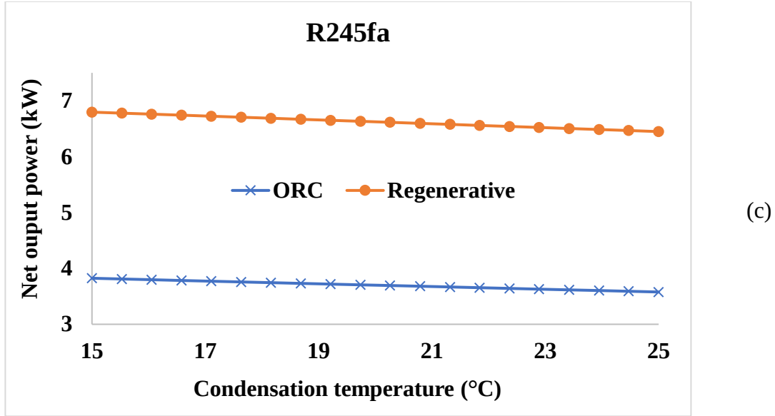
Figure 5.18: Effect of condensation temperature on the net output power of basic and regenerative organic Rankine cycles for (a) R123, (b) R124 and (c) R245fa
