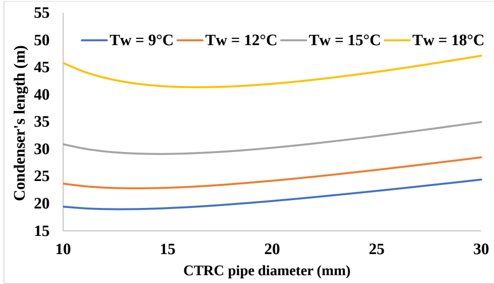
Figure 3.15: The variation of condenser's length as a function of cycle's pipe diameter at several underground water temperatures ( T_w )
