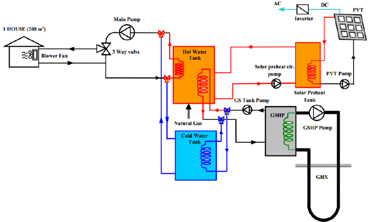
Figure 2.32: Photovoltaic thermal integrated with ground source heat pump [121]
