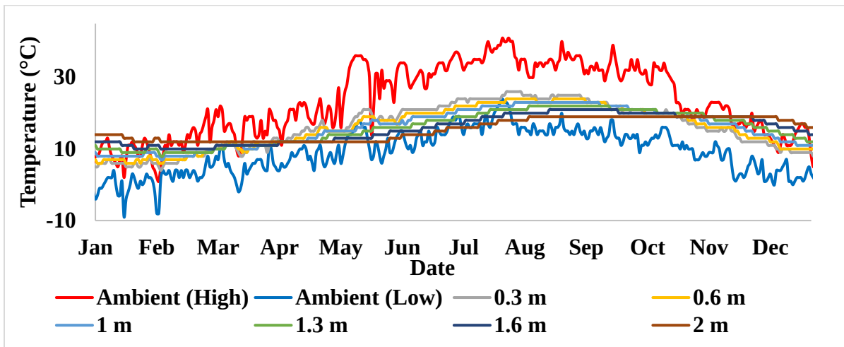
Figure 4.2: Ambient and ground temperature measurement in Bekaa-Lebanon during 2020
