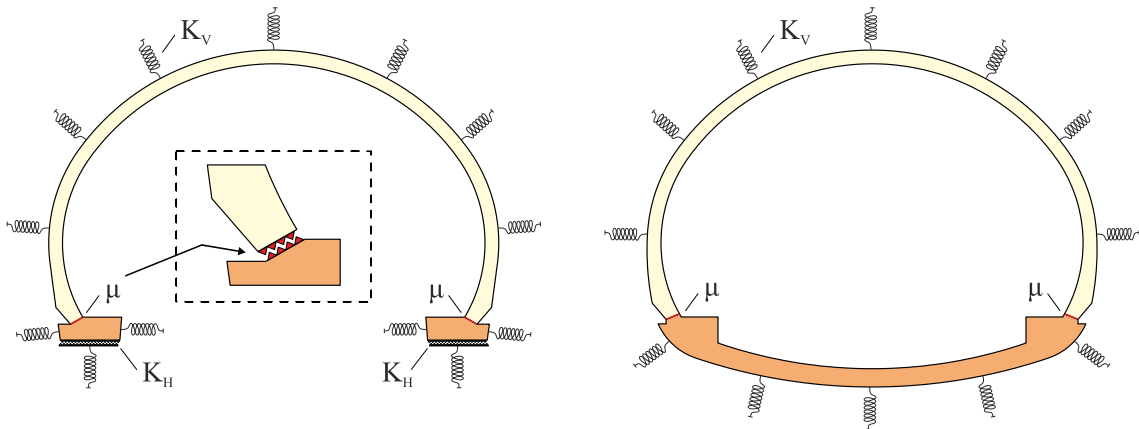
Fig. 3 Boundary conditions between tunnel lining and surrounding rock mass.
