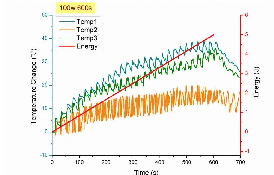
Figure 7. Temperature change measurements (micro-strain) by FBG sensors (left), and energy absorbed (right) versus time (s) under 100W.
