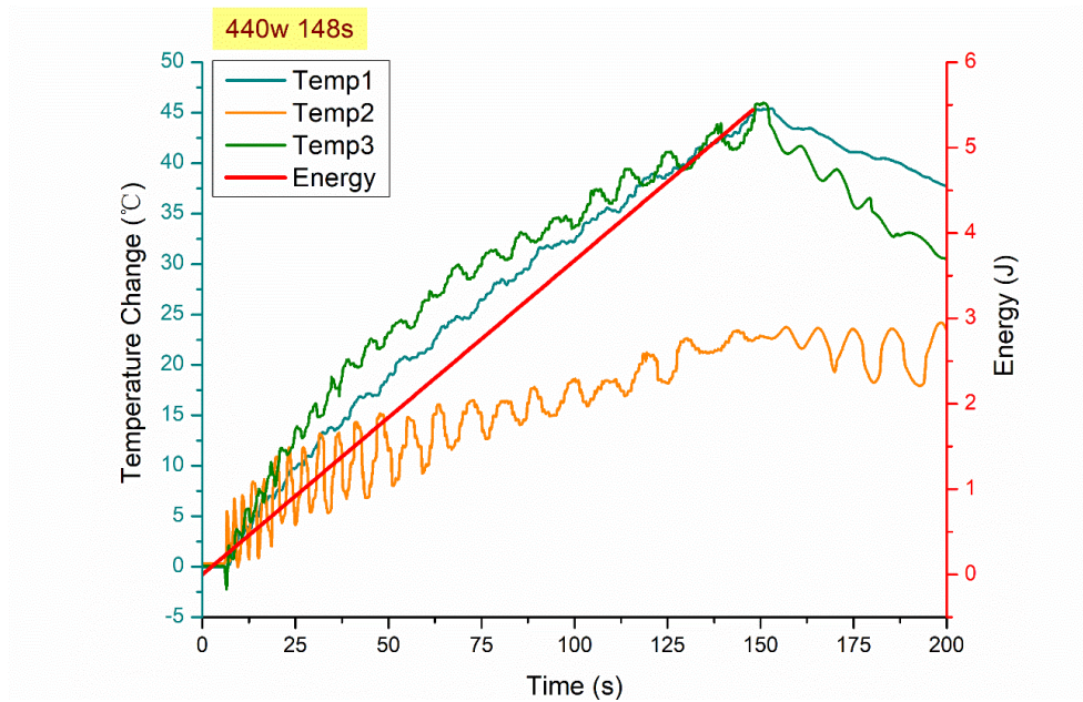
Figure 8. Temperature change measurements (micro-strain) by FBG sensors (left), and energy absorbed (right) versus time (s) under 440W.
