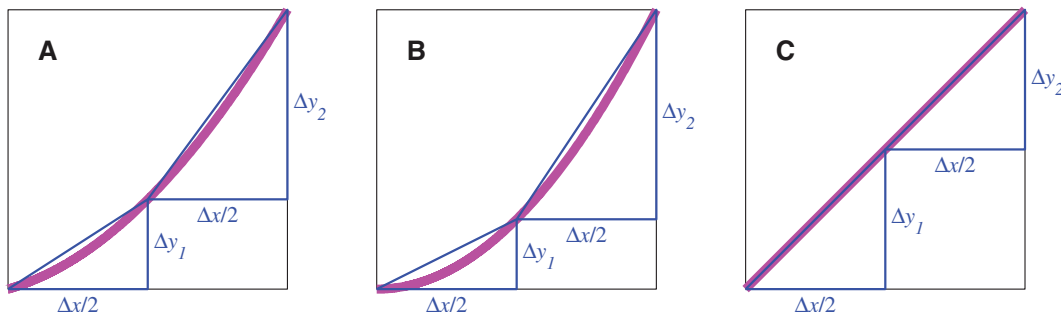
Figure 19. Index of acceleration, \eta . (A) The wide, magenta curve shows an expansive power function sampled over a range of inputs from a to (a+\Delta x) , where a > 0 . The horizontal blue lines both have length \Delta x/2 , and the vertical blue lines have length \Delta y_1 and \Delta y_2 as indicated. The slope, S_1 , of the secant (the oblique line) across the left half of the curve is given by \Delta y_1/(\Delta x/2) , and the slope, S_2 , of the secant across the right half of the curve is given by \Delta y_2/(\Delta x/2) . Our index of acceleration, \eta , is given by S_2/S_1 . For the power function, when a \neq 0 , \eta \rightarrow 1 as \Delta x \rightarrow 0 , so the curve is “strongly locally linear” at x=a . (B) The same as A, but with the bottom of the range of inputs, a , equal to zero. In this case, \eta depends only on the exponent of the power function, and so it does not approach 1 as \Delta x approaches zero. The power function is not “strongly locally linear” at x=0 . (C) The same as A, but for a straight line function. Here, \eta = 1 for all a and \Delta x .
