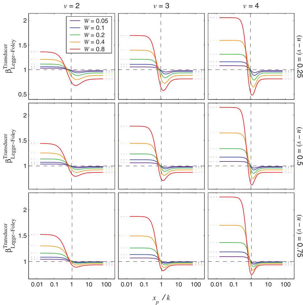
Figure 13. \beta^{\text{Transducer}}_{\text{Legge-Foley}} for the Legge-Foley transducer with nonzero pedestal. The curves were generated using Equation (74). Each column of panels has a particular value for \nu , and each row of panels has a particular value for the difference (u - v) . Within the panels, the Weber fraction, W , is indicated by the colour of the curve (the legend in the top-left panel applies to all panels). The curves approach horizontal asymptotes on the right (indicated by dotted lines), with vertical position given by Equation (67) with b = u - v . This is because, as the input signal increases, the Legge-Foley transducer approaches a power function with exponent (u - v) . This asymptote can also be derived from Equation (74) by setting k/x_p \rightarrow 0 , which gives the limit as x_p \rightarrow \infty . On the left, the curves come close to approaching an asymptote with vertical position given by Equation (67) with b = u because, at low contrasts, the Legge-Foley transducer approximates a power function with exponent u . These near-asymptotes are indicated by dotted lines on the left of each panel. They are not true asymptotes because, even for x_p = 0 , the Legge-Foley transducer is not exactly equal to a power function over a finite range of inputs. The horizontal, dashed lines indicate \beta^{\text{Transducer}}_{\text{Legge-Foley}} = 1 . The vertical dashed lines indicate the value of x_p/k corresponding to the point of inflection of the Legge-Foley transducer. An expression for this quantity is derived in Appendix S2. For typical values of u and \nu , including those in this figure, the point of inflection occurs very close to an input of k , giving x_p/k \approx 1 . For pedestals above this value, both the target and pedestal will lie in the compressive region of the Legge-Foley transducer, so \beta^{\text{Transducer}}_{\text{Legge-Foley}} must be less than 1. For this reason, none of the curves enter the top-right quadrant in any of the panels. doi:10.1371/journal.pone.0074815.g013
