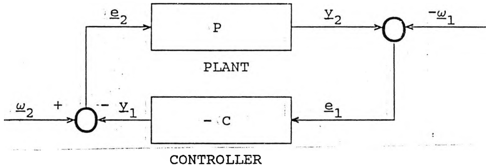
Figure (3.2): Alternative Control System Configuration
