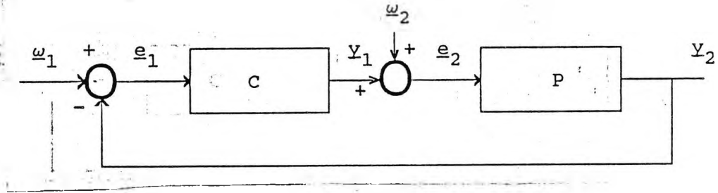
Figure (3.1): General Control System Configuration
