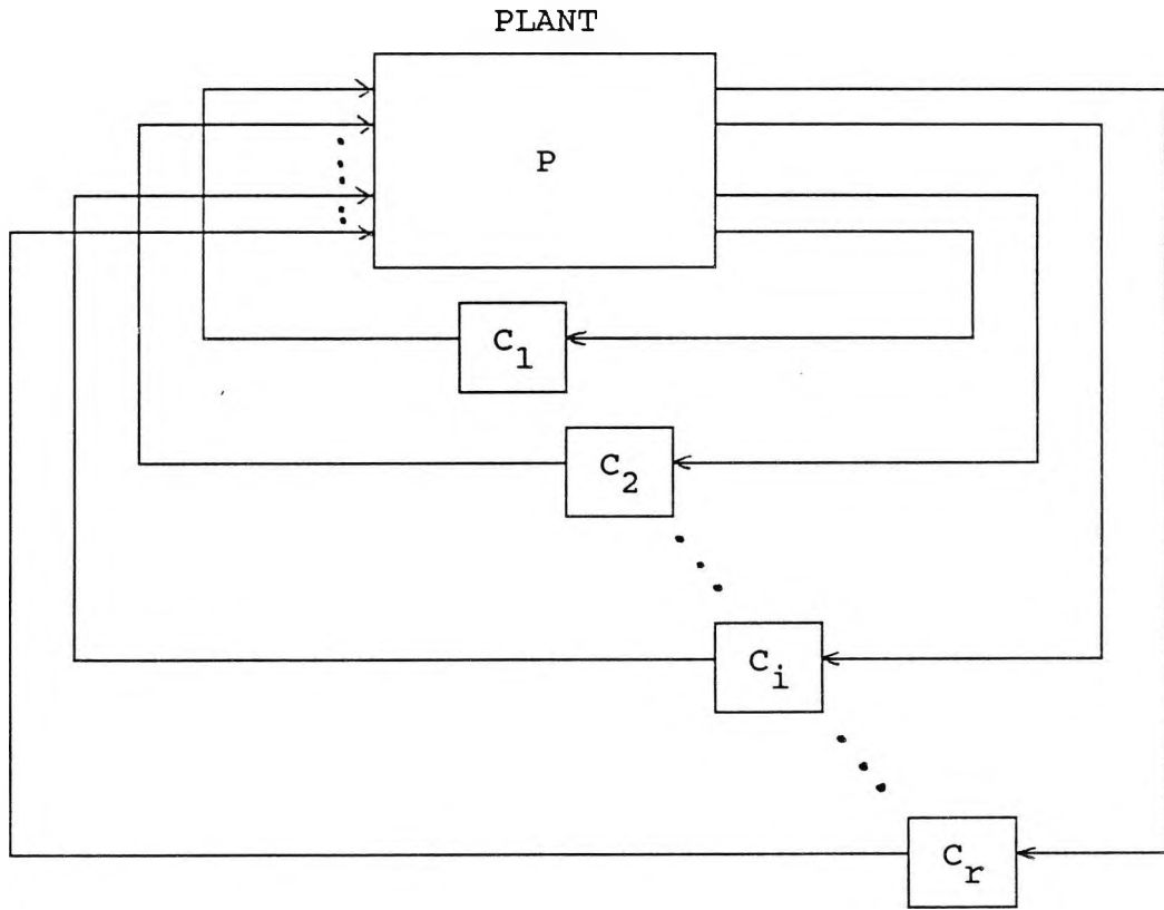
Fig. 6.4 Feedback Control Scheme: Permutation of Diagonal Controllers
