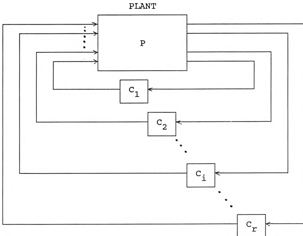
Fig. 6.3 Feedback Control Scheme: Diagonal Controller
