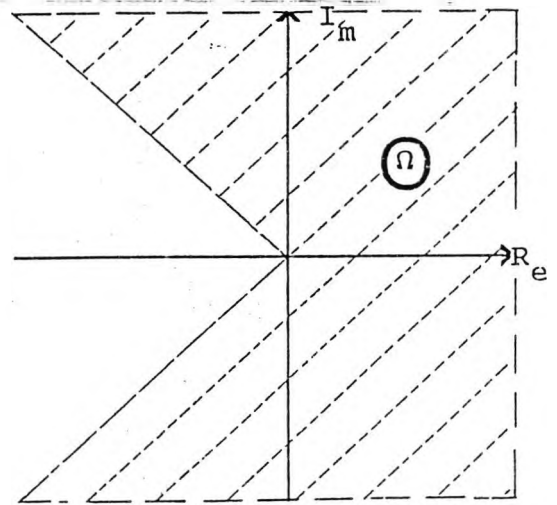
B. \Omega is the undesired part of the complex plane. In the above case \Omega is the right half of the complex plane and a selected part of the left half plane chosen such that a desired maximum damping factor is not exceeded.
