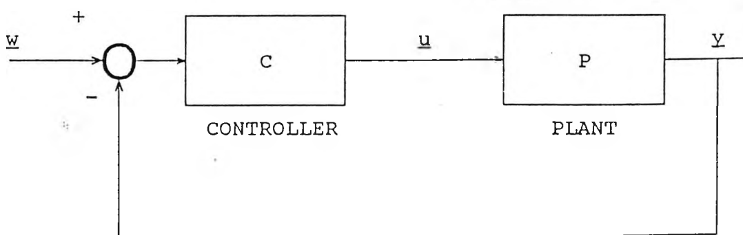
Figure (3.4): Basic feedback control configuration
