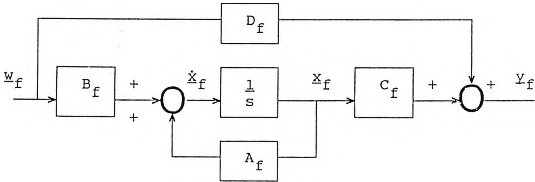
Figure (3.3): State Space representation of general feedback configuration
