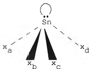
Pyramidal 4 co-ordinate
