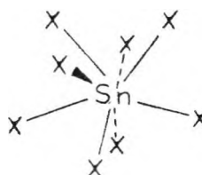
Figure 1-1: The Common Geometries of Inorganic Tin(IV) Compounds
