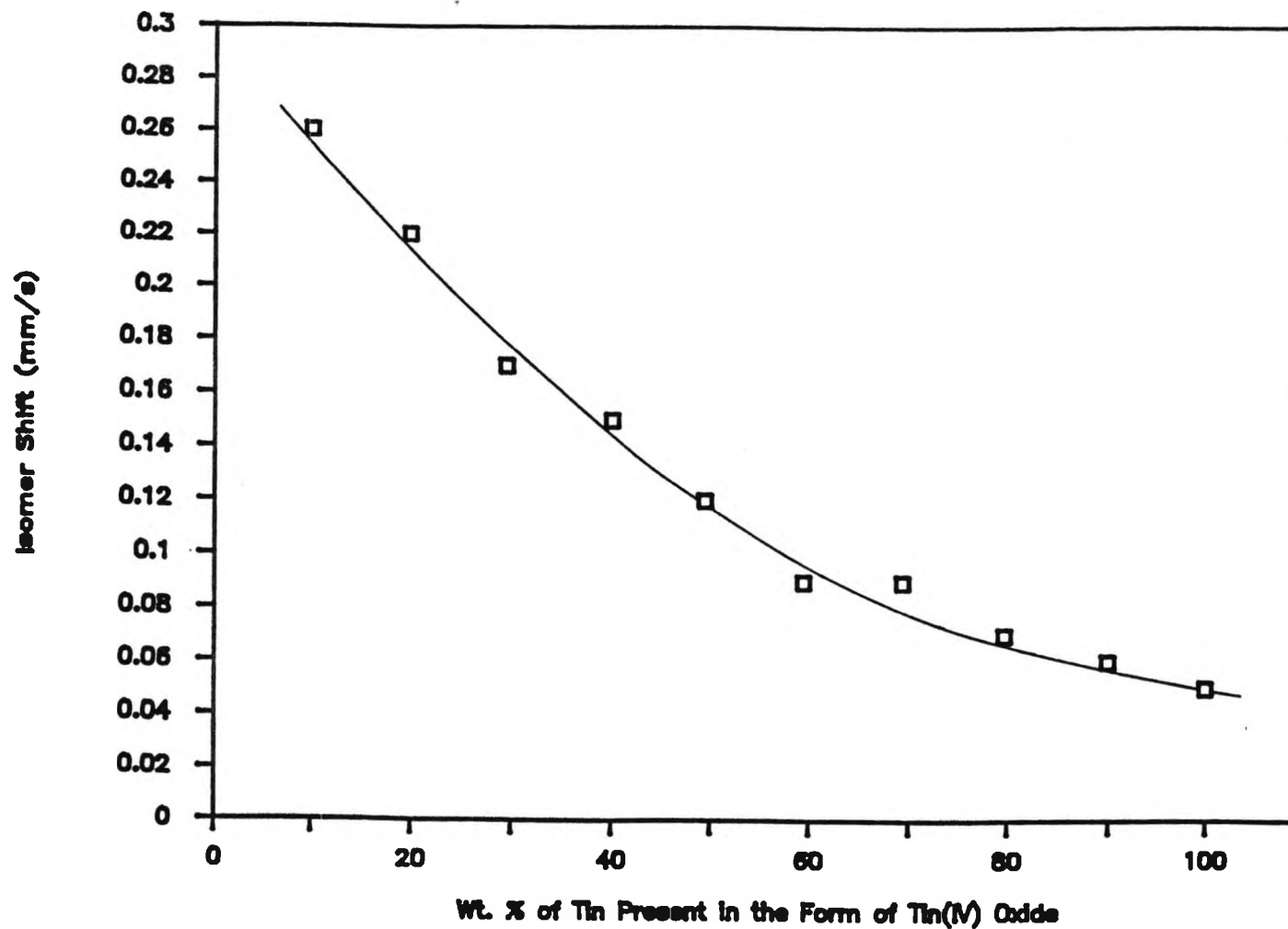
Figure 4-8: Variation of Isomer Shift with Weight Percent of Tin Present in the Form of \text{SnO}_2 in \text{SnO}_2 / \text{SnCl}_4 \cdot 5\text{H}_2\text{O} Mixtures
