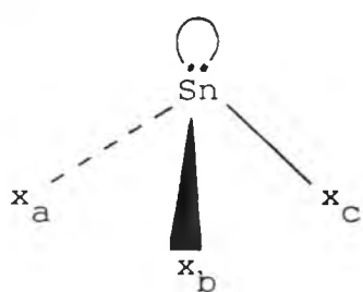
Trigonal Pyramidal
