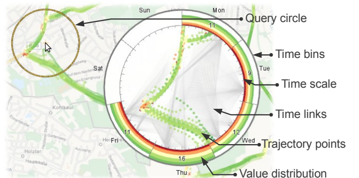
Fig. 5. The time lens visualizes temporally aggregated information.
