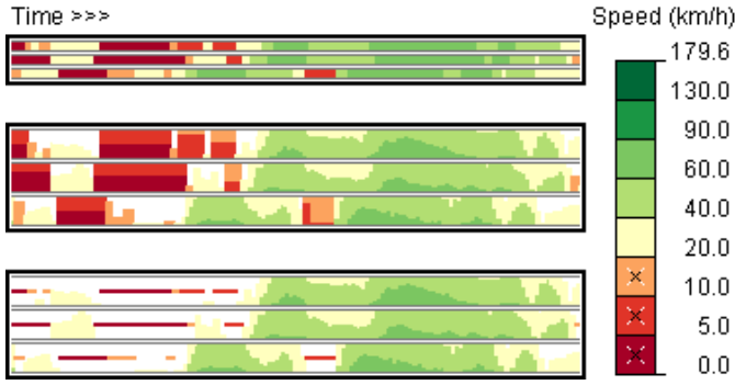
Fig. 2. Alternatives for color-coding attribute values along trajectory bands. Top: plain color-coding requires less space; middle: two-tone pseudo-coloring [30] increases precision; bottom: color filtering reduces visual load.
