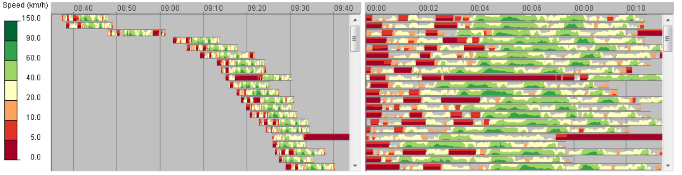
Fig. 6. The time graph shows the dynamics of attribute values within trajectories by two-tone pseudo-coloring. The alignment of the trajectories has a significant impact on what can be seen in the display (left: alignment by time of the day, right: alignment by start time).
