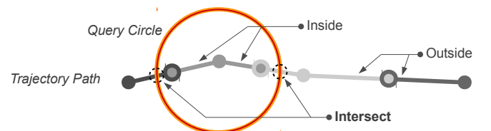
Fig. 10. Cases of path-segment-circle intersections.
