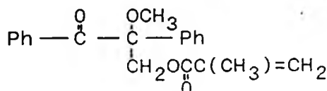
\alpha -Methylolbenzoin Methyl Ether Methacrylate, VI
