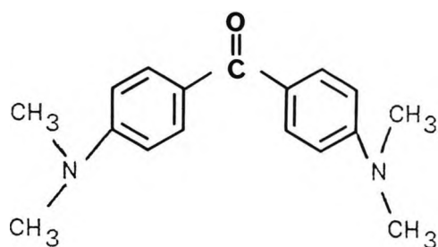
Michler's Ketone
