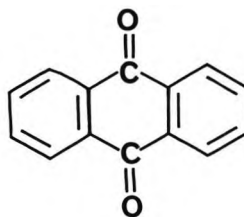
Anthraquinone
