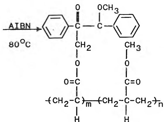
MB Copolymers
