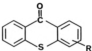
Substituted Thioxanthone
