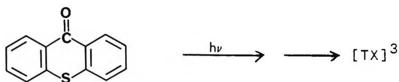
Thioxanthone TX
