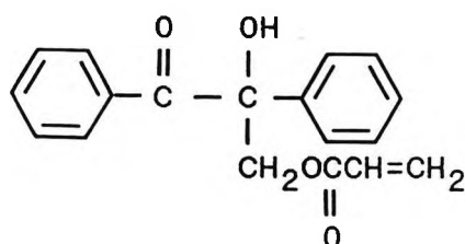
\alpha -Methylolbenzoin Acrylate
