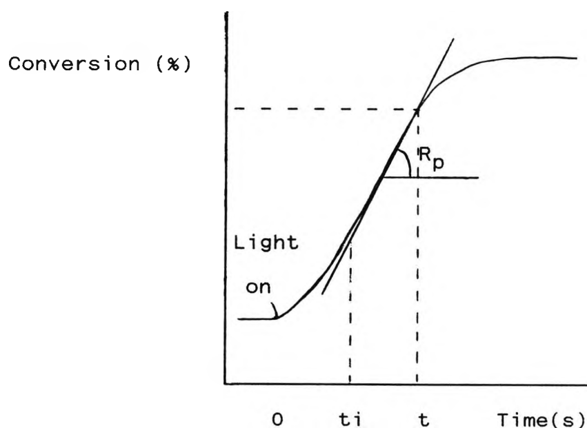
Typical cure profile for an acrylic coating
