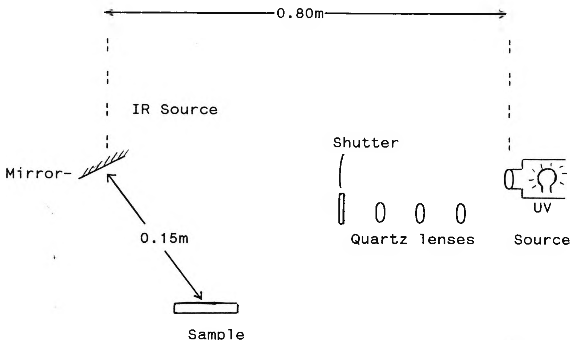
Schematic Representation of Real-Time Infrared Apparatus
