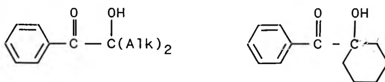
\alpha -Hydroxyalkylphenones
