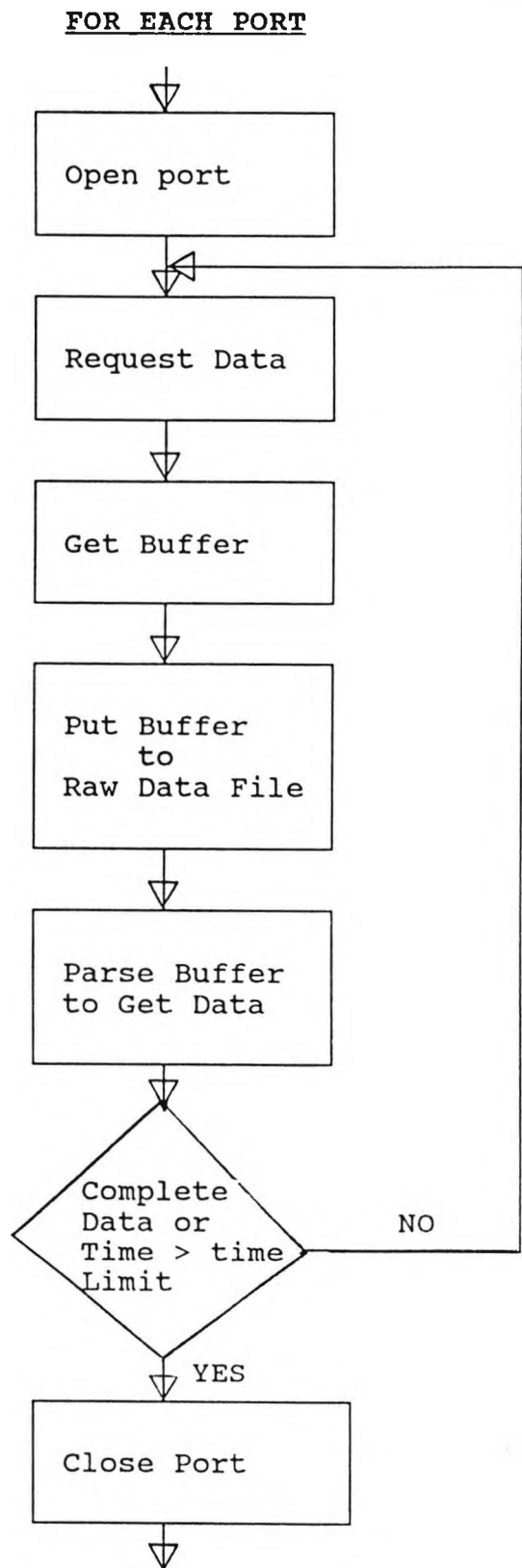
Figure 6.6: Flow Diagram for Each Port.
