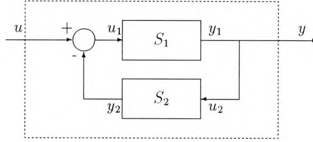
Σ 3: Feedback Connection
