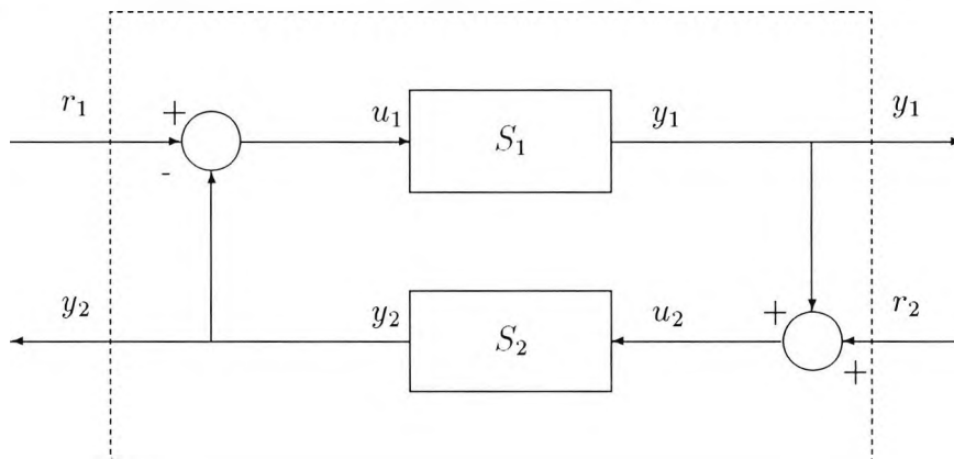
Fig. 6.4: \Sigma_{12} : Complete feedback configuration
