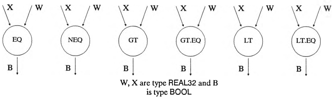
Figure 5.16 Relational nodes
