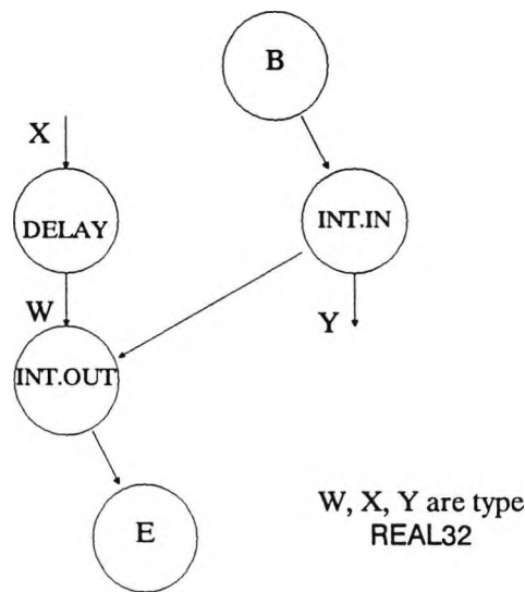
Figure 5.10 Multiple delay
