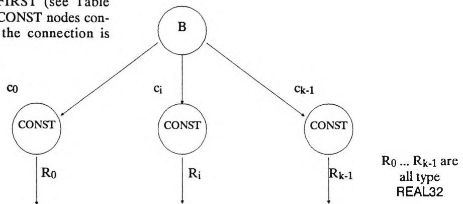
Figure 5.7 Constant nodes
