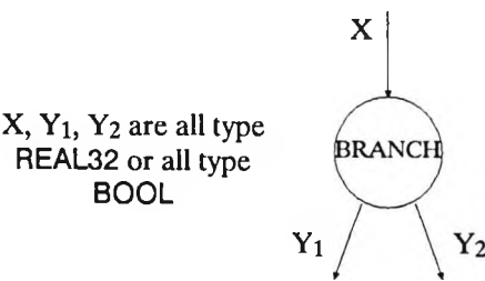
Figure 5.13 Branch node
