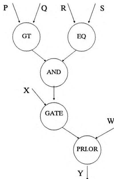
Figure 5.22 Conditional graph structure
