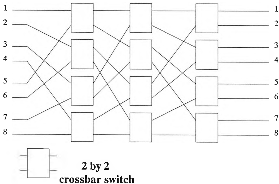
Figure 1.12 Omega network
