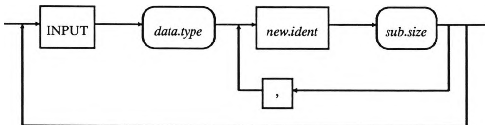
Figure D.3 Input flow
