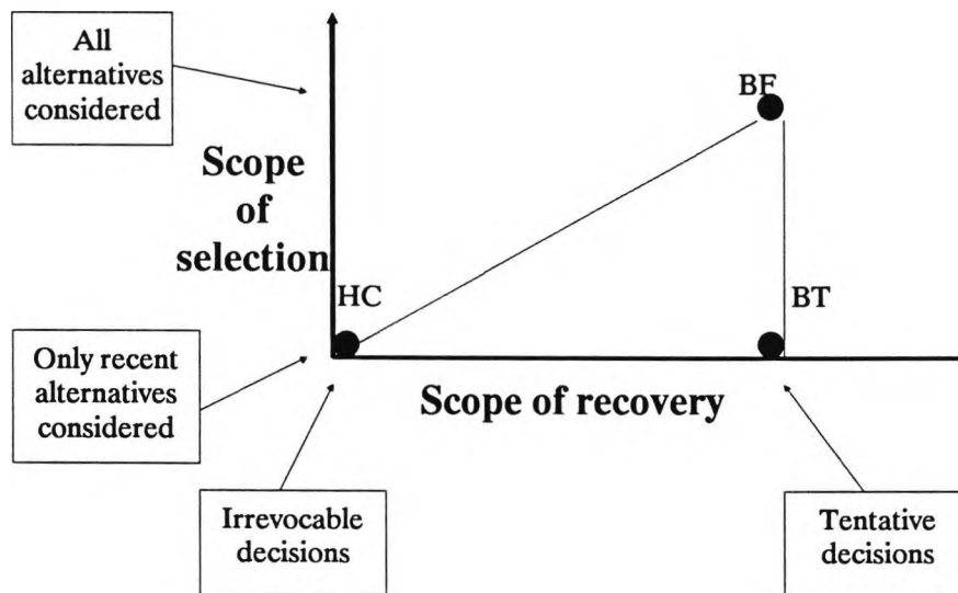
Figure 7.7 2-dimensional space of hybrid strategies
