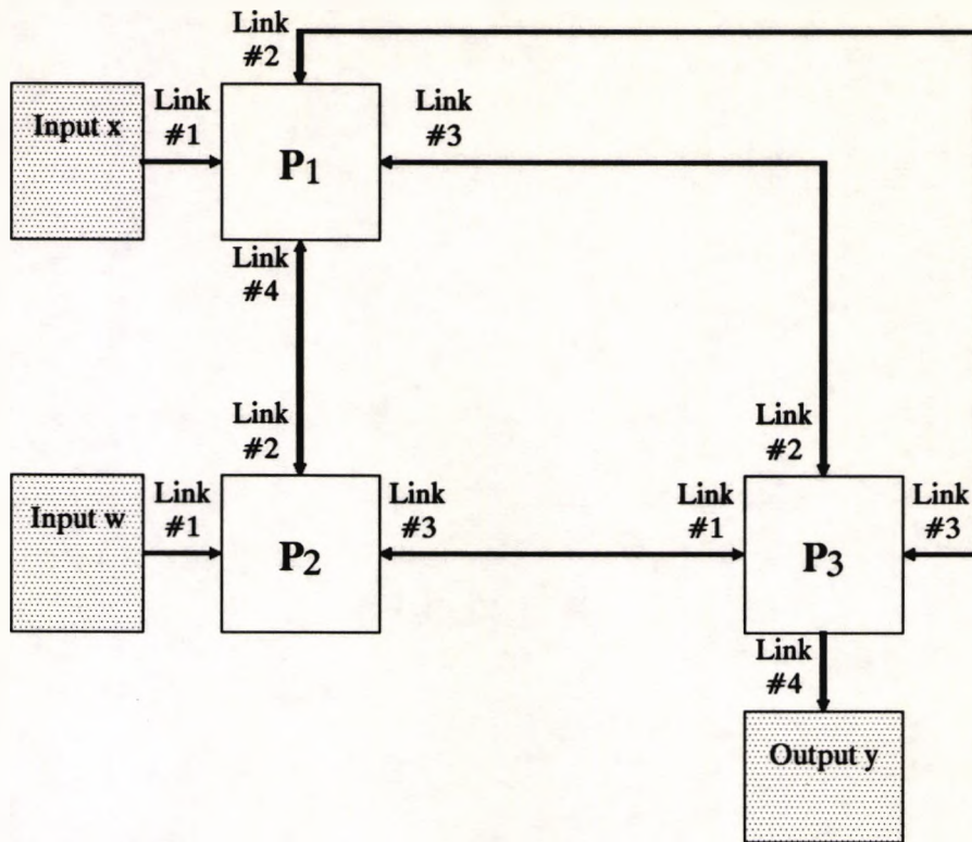
Figure 6.2 Transputer interconnection network
