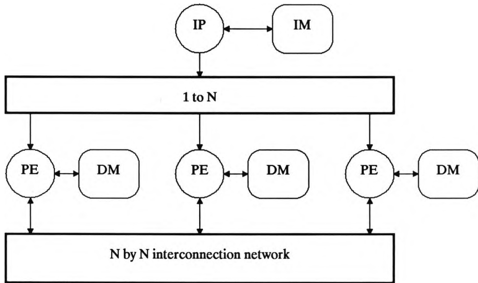
Figure 1.2 Array architecture
