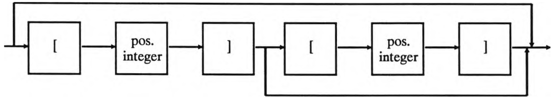
Figure D.7 Subscript size flow
