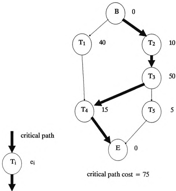
Figure 2.9 DAG, showing the critical path
