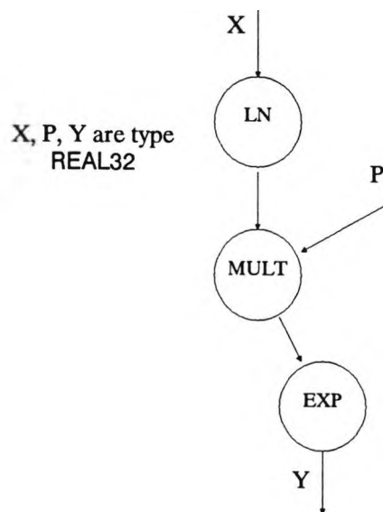
Figure 5.19 Power graph structure
