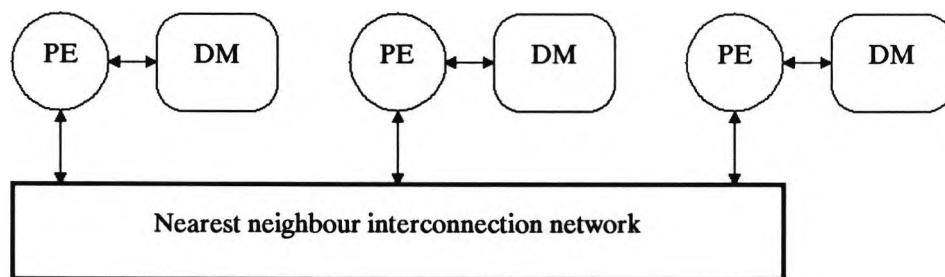
Figure 1.5 Wavefront array architecture
