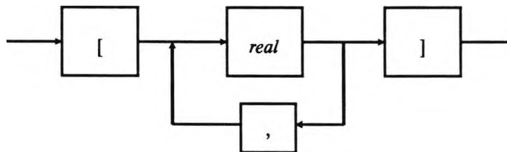
Figure D.9 Real string flow
