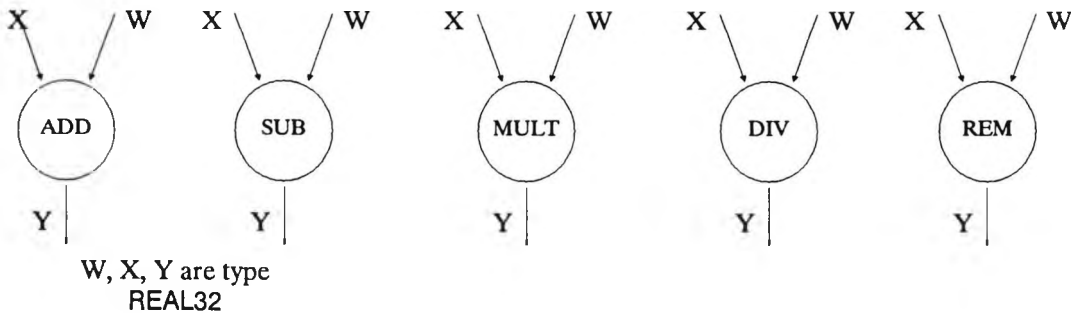
Figure 5.12 Dyadic arithmetic nodes
