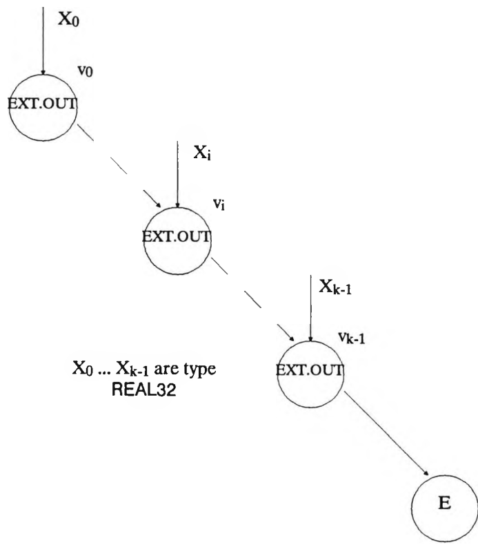
Figure 5.4 External output stream (REAL32)
