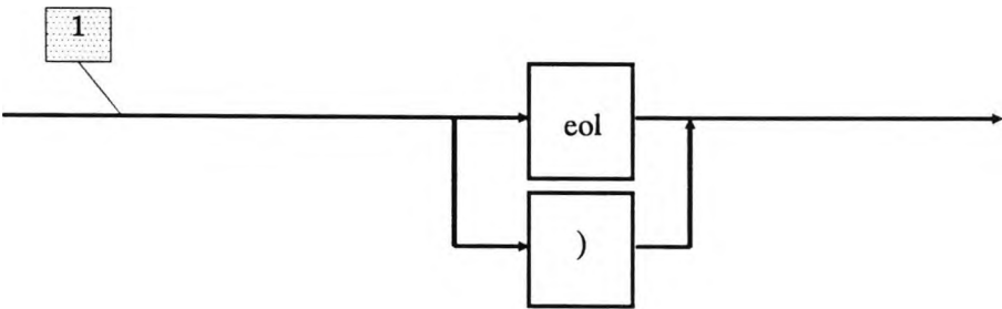
Figure D.17 Parse right real flow
