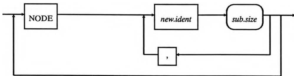
Figure D.4 Node flow
