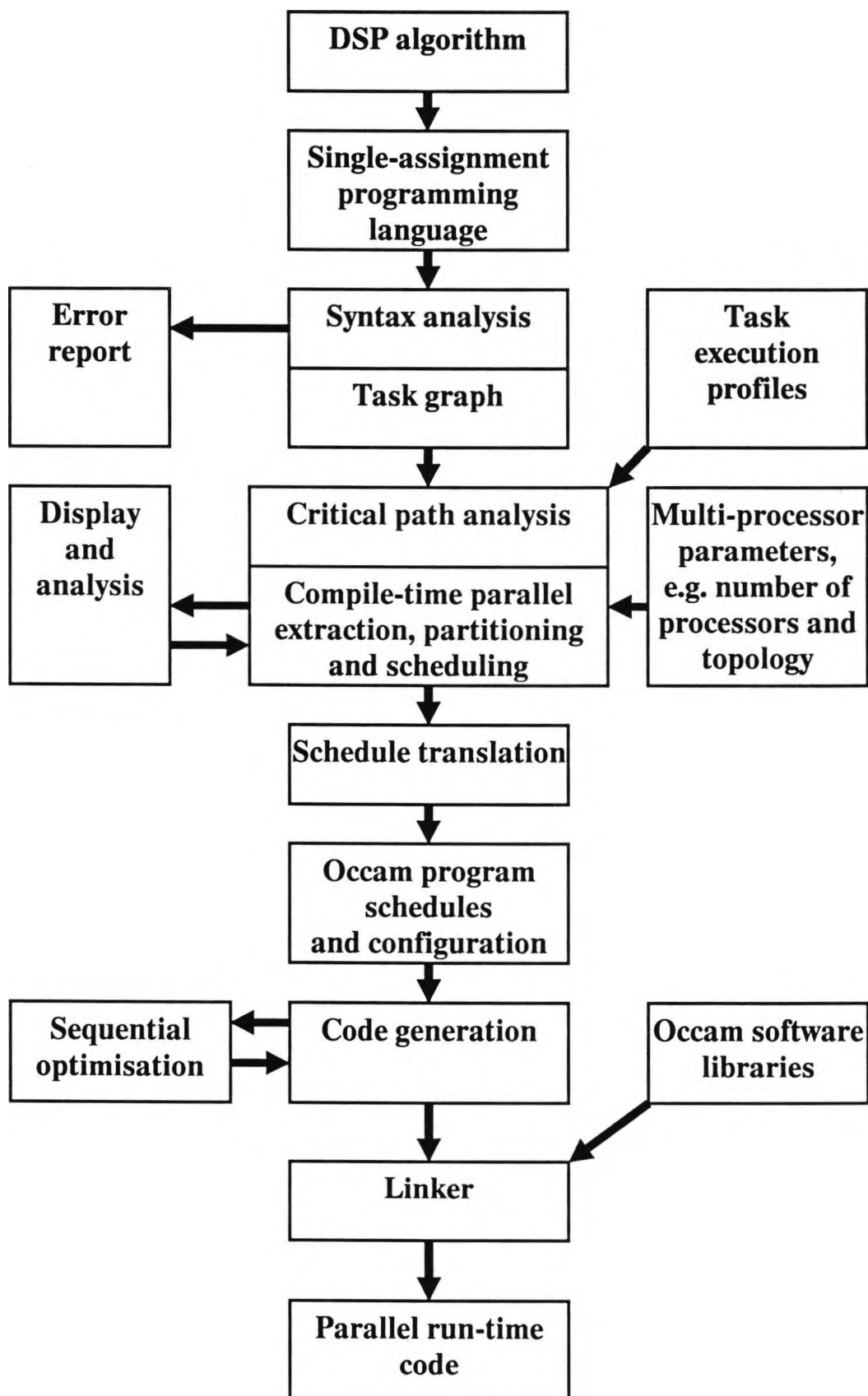
Figure 1.14 Compile-time implementation strategy
