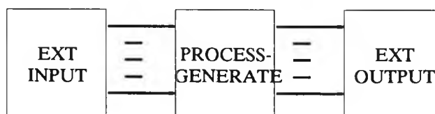
Figure 2.2 Input-process-output synchronisation
