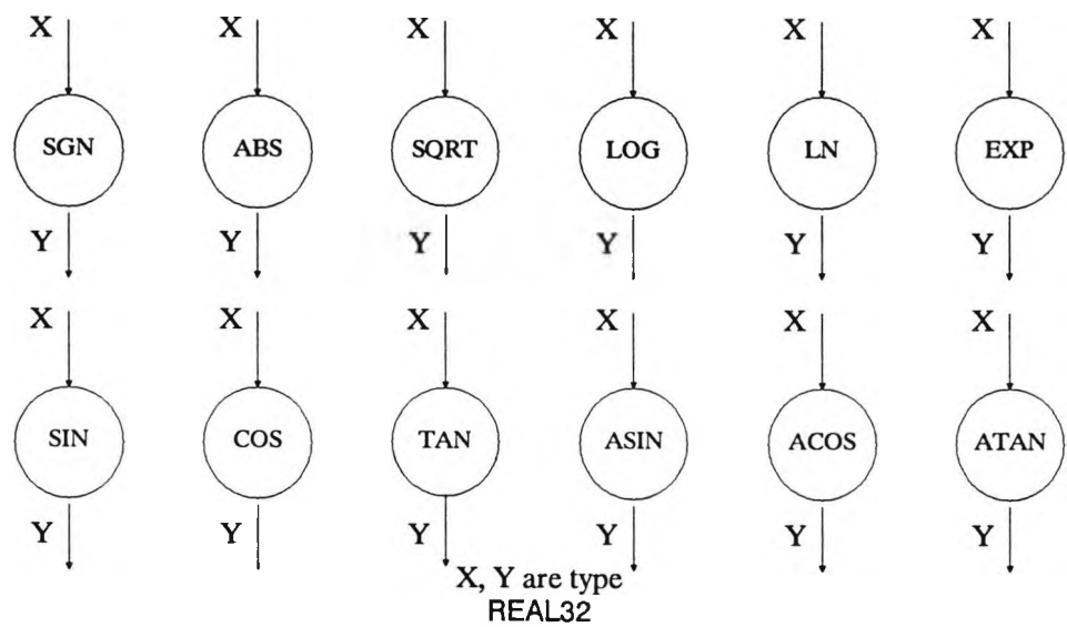
Figure 5.14 Function nodes
