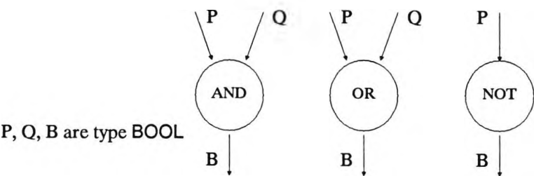
Figure 5.17 Boolean nodes
