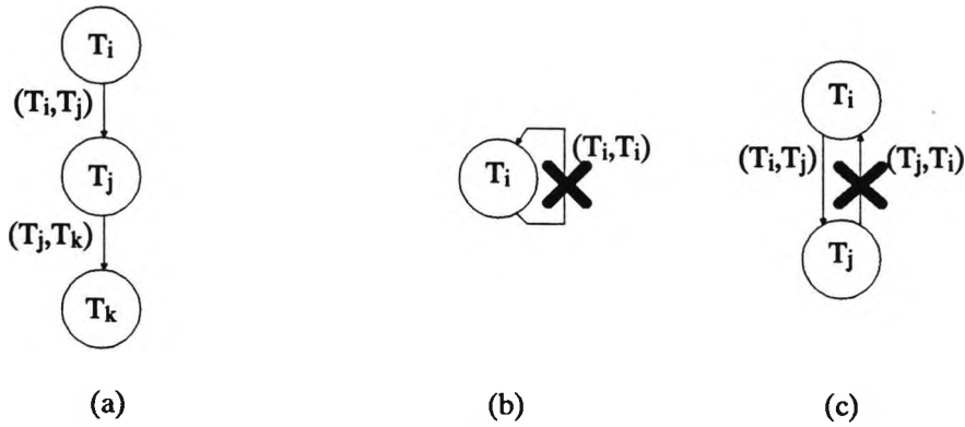
Figure 2.6 Arc relationships
