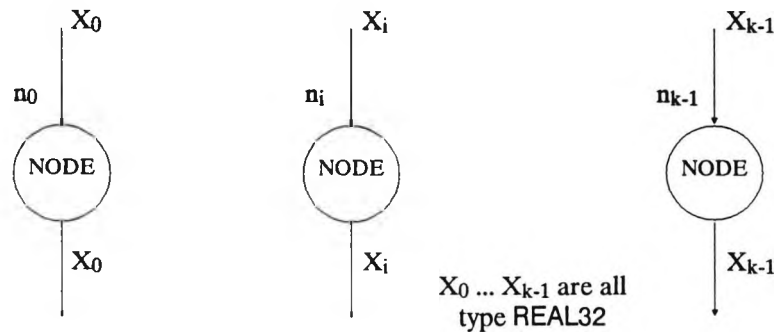
Figure 5.6 Node nodes
