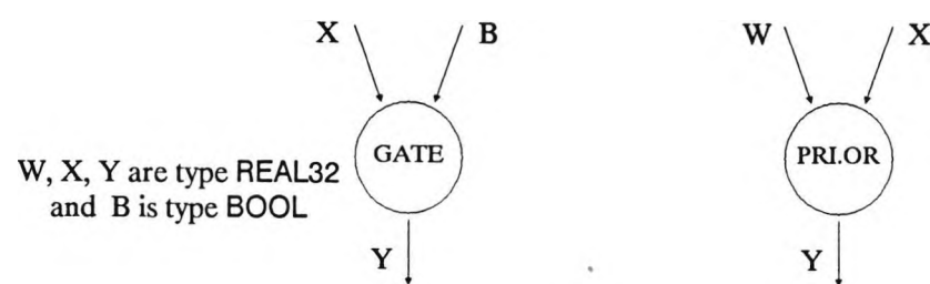
Figure 5.18 Conditional nodes
