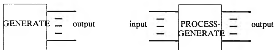
Figure 2.1 Algorithm input-output
