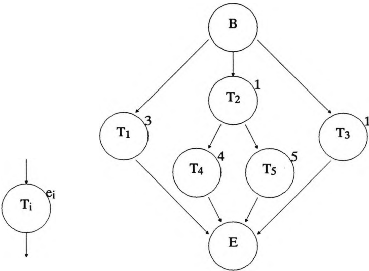
Figure 7.1 Task graph, G
