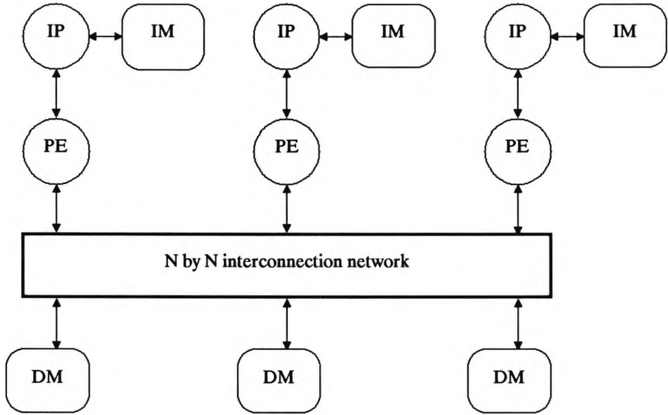
Figure 1.7 Tightly coupled architecture
