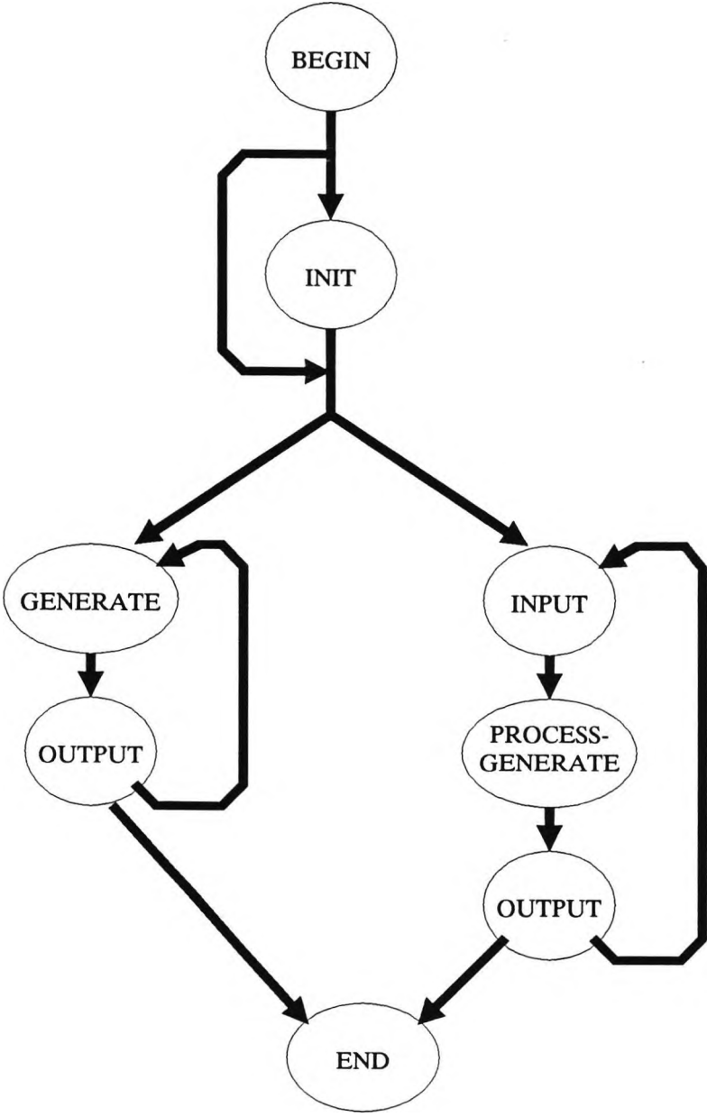
Figure 3.2 DFDL program structure models
