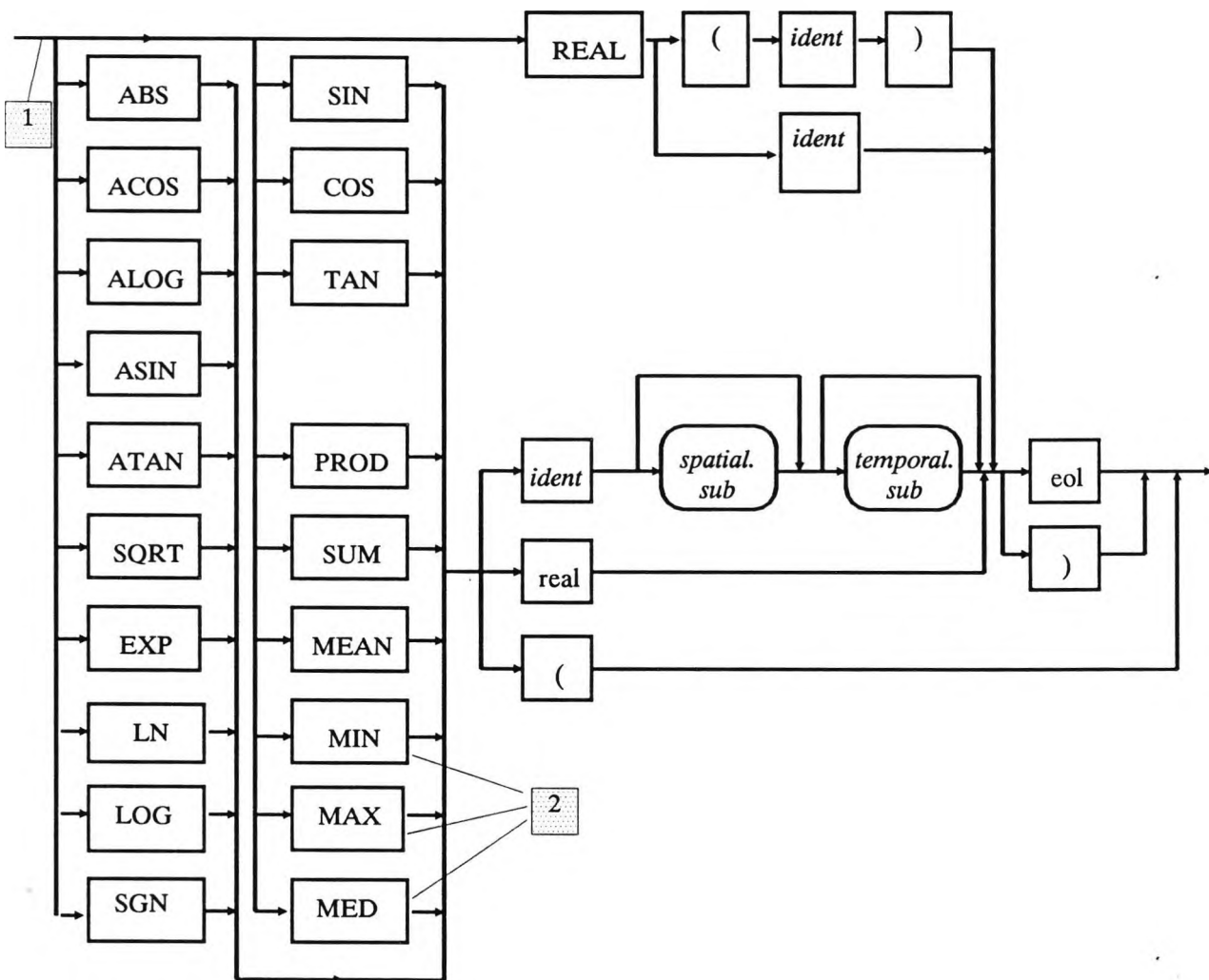
Figure D.18 Function flow
