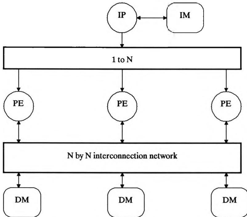
Figure 1.3 Array architecture
