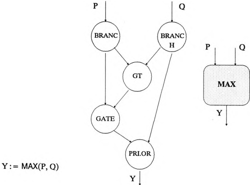
Figure 5.23 Maximum graph structure
