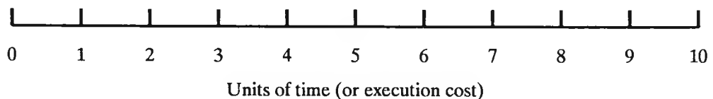
Figure 7.3 Scheduling methods
