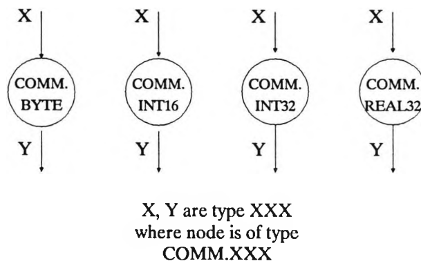
Figure 5.15 Communication nodes
