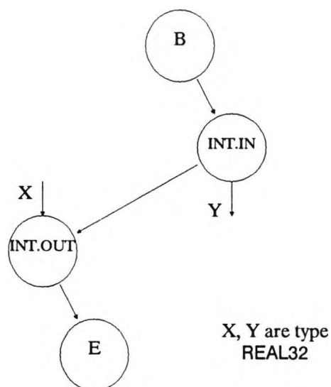
Figure 5.9 Single delay
