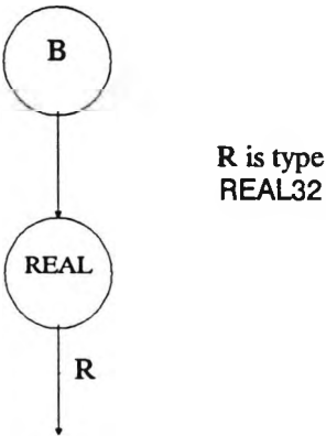
Figure 5.8 Real node
