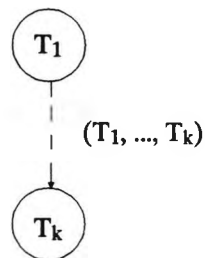
Figure 2.7 Acyclic path
