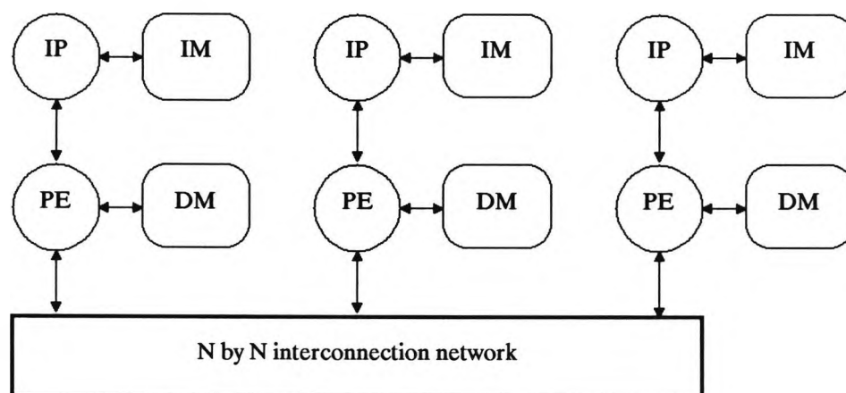
Figure 1.6 Loosely coupled architecture
