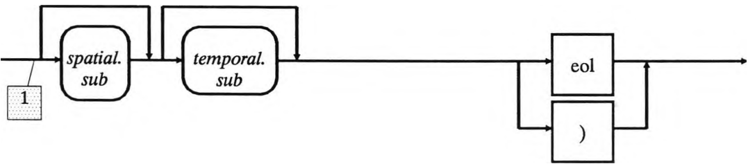
Figure D.16 Parse right identifier flow
