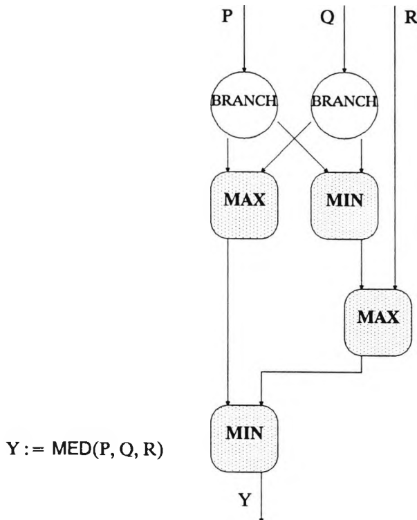
Figure 5.25 Median graph structure
