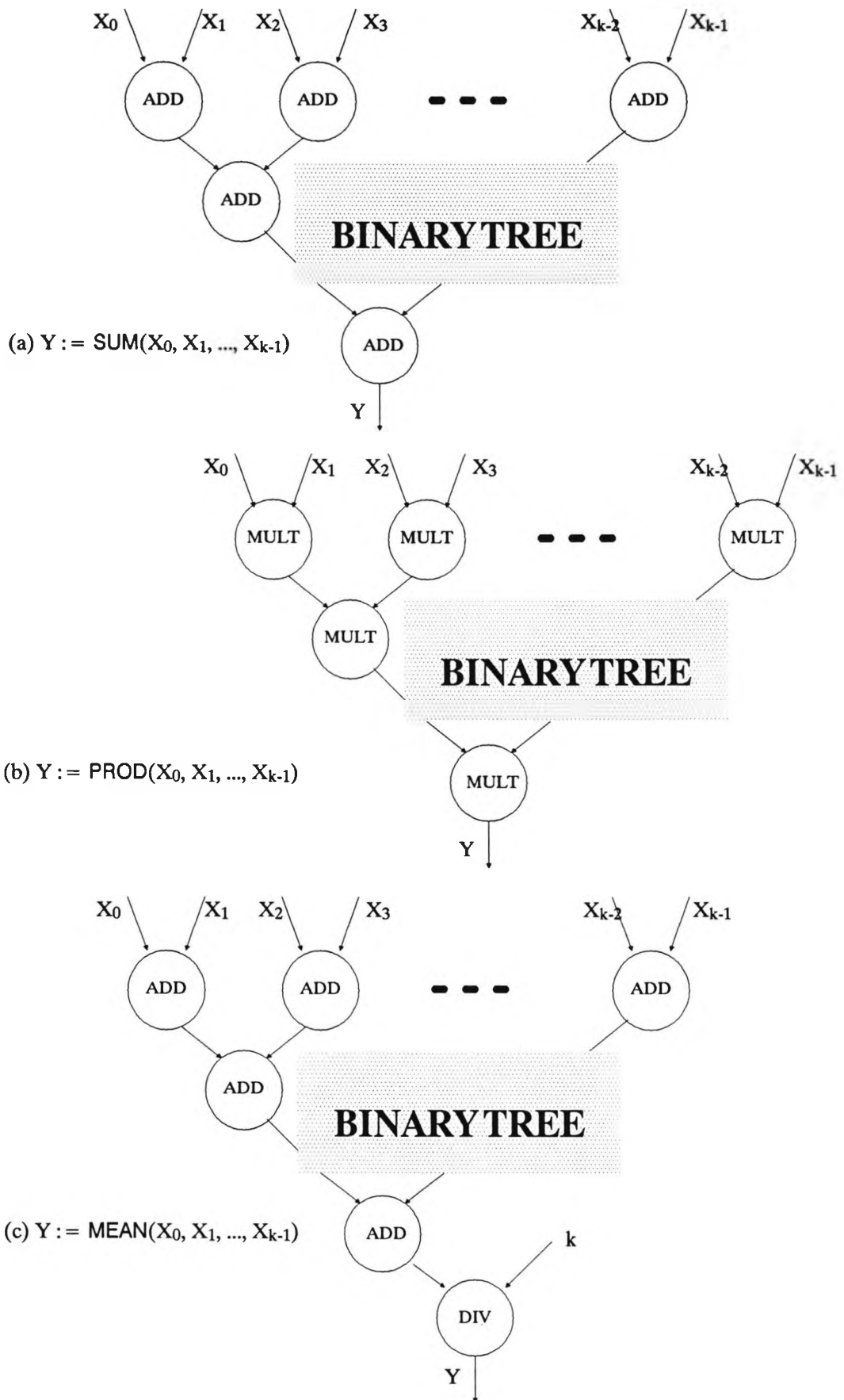
Figure 5.21 (a)SUM (b)PROD (c)MEAN graph structures
