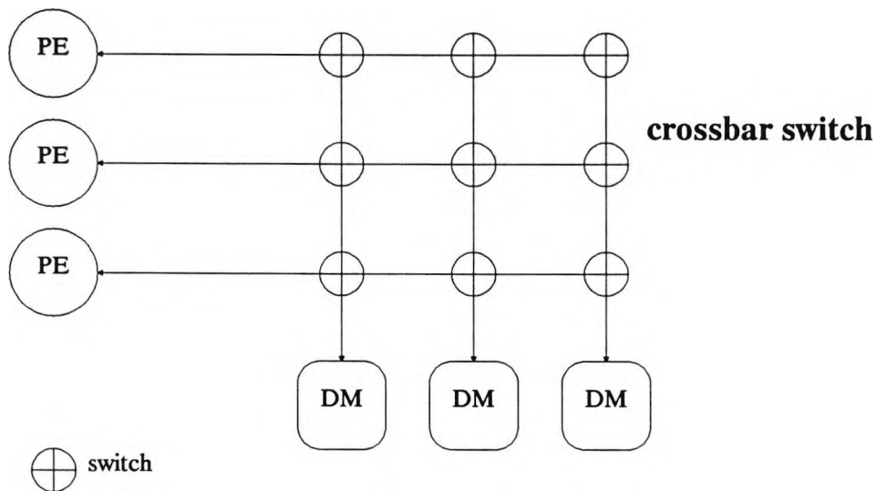
Figure 1.11 Full connectivity
