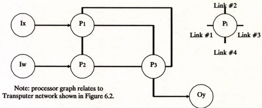
Figure 6.4 Processor graph of Transputer network
