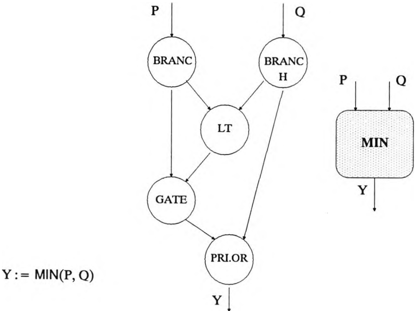
Figure 5.24 Minimum graph structure
