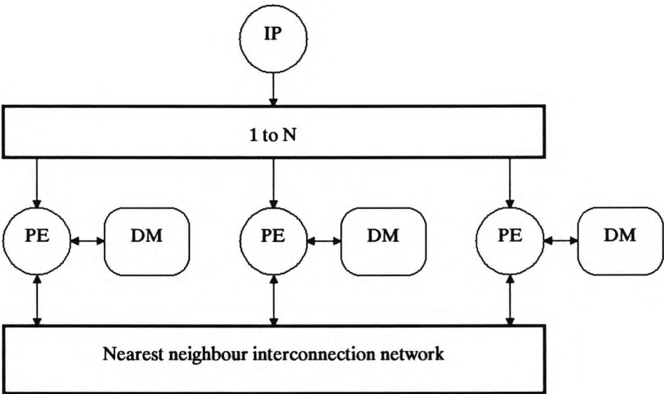
Figure 1.4 Systolic array architecture
