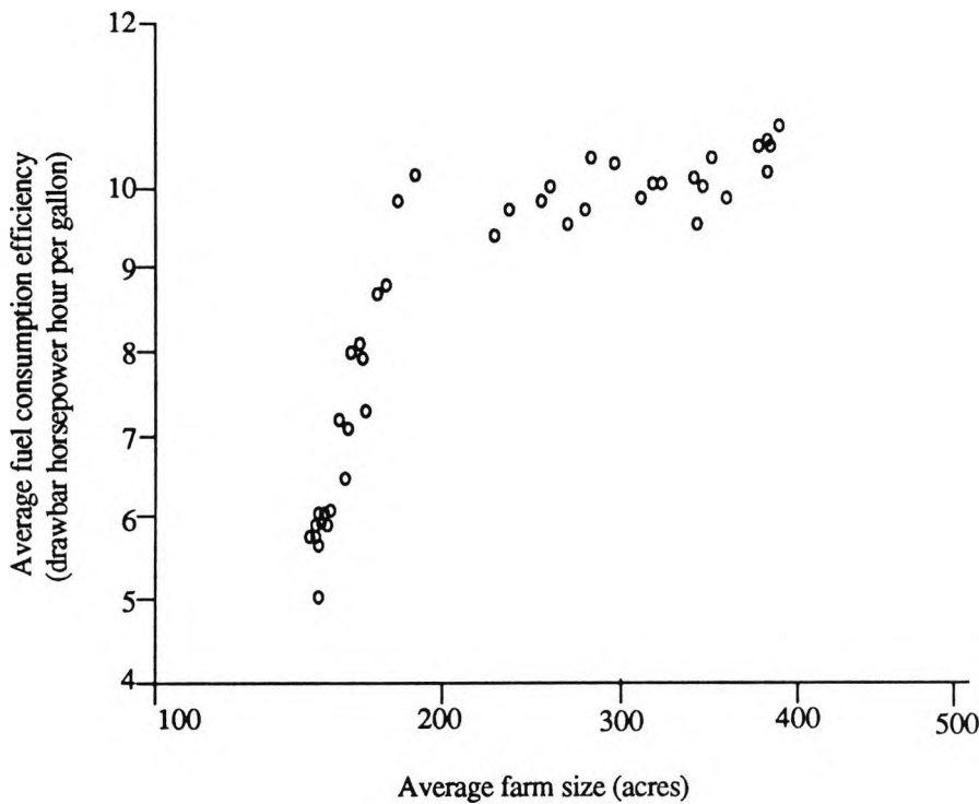
Figure 2.2 Relationship between fuel consumption efficiency of farm tractors and average farm size, 1921-1968 (Sahal, 1979a, p. 270)
