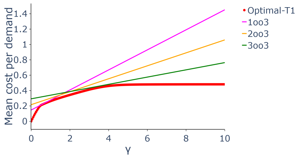
Figure 40: Mean cost per demand for optimal adjudicator T1, 1003, 2003 and 3003 ( n=3 )
