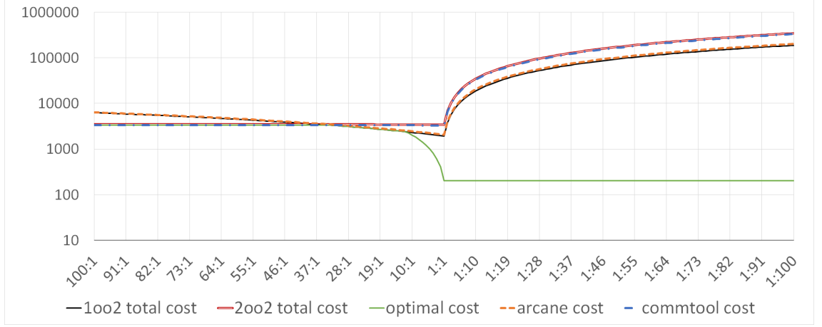
Figure 32: D1 total error costs
