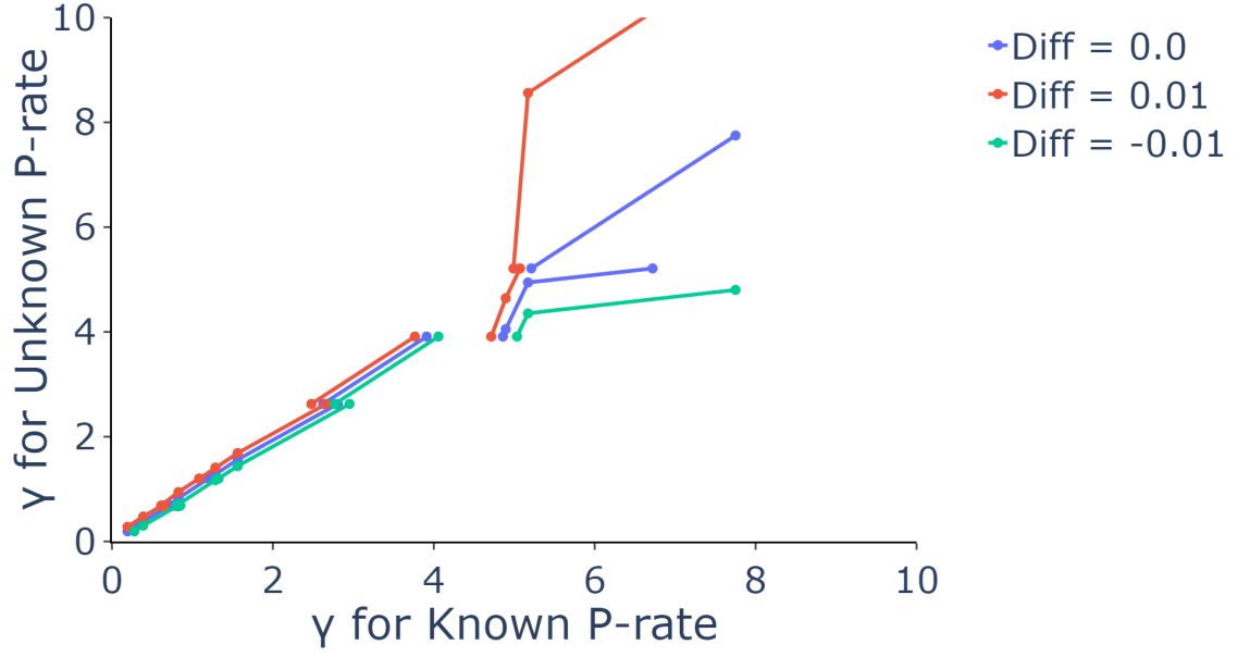
Figure 47: Ranges of \gamma for known and unknown P=rate, with different cost T cost differences (RNN models 30, 32 and 33)
