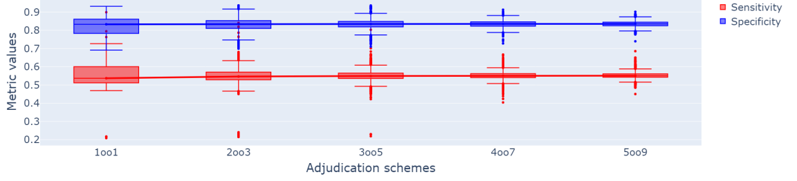
Figure 26: Sensitivity and Specificity for majority voting adjudication schemes
