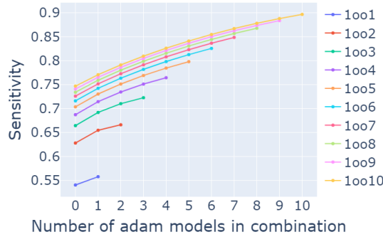
(a) Mean sensitivity based on optimiser combinations for 1ooN schemes
