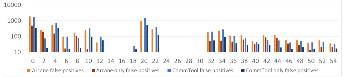
Figure 11: False positives by bytes sent for D2.
