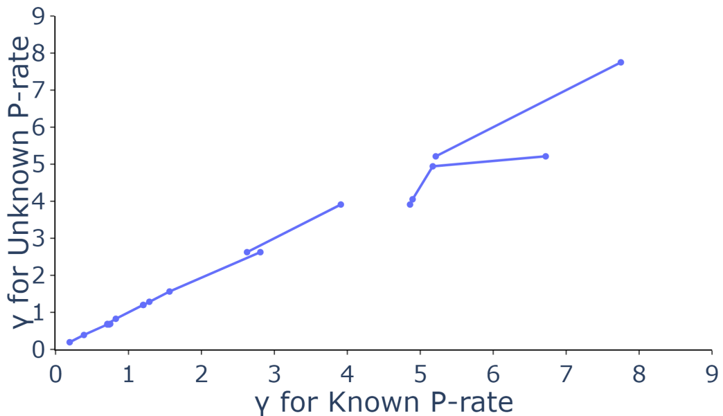
Figure 46: Ranges of \gamma for known and unknown P-rate (RNN models 30, 32 and 33)
