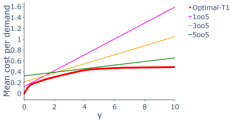
Figure 41: Mean cost per demand for optimal adjudicator T1, 1005, 3005 and 5005 ( n=5 )
