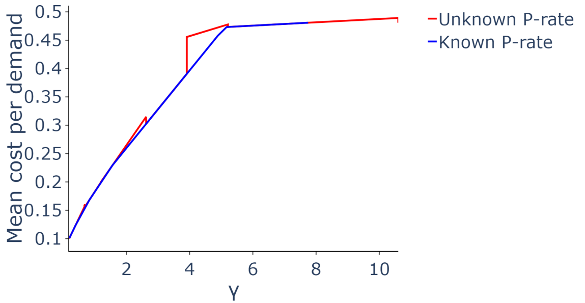
Figure 45: Mean cost per demand profile (RNN models 30, 32 and 33)
