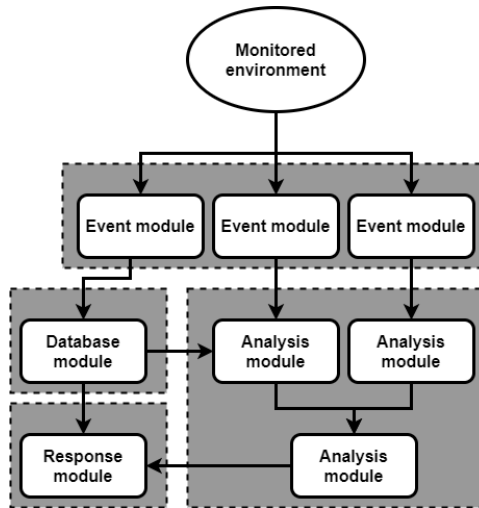
Figure 6: Common intrusion detection framework
