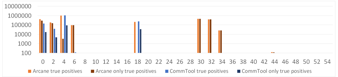
Figure 7: True positives by bytes sent for D1.
