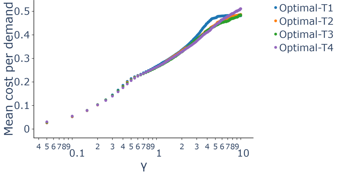
Figure 42: Mean cost per demand profile for optimal adjudicators T1, T2, T3 and T4 (log)
