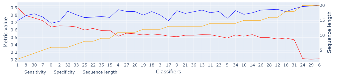
Figure 21: Single model metrics, ordered by sequence length
