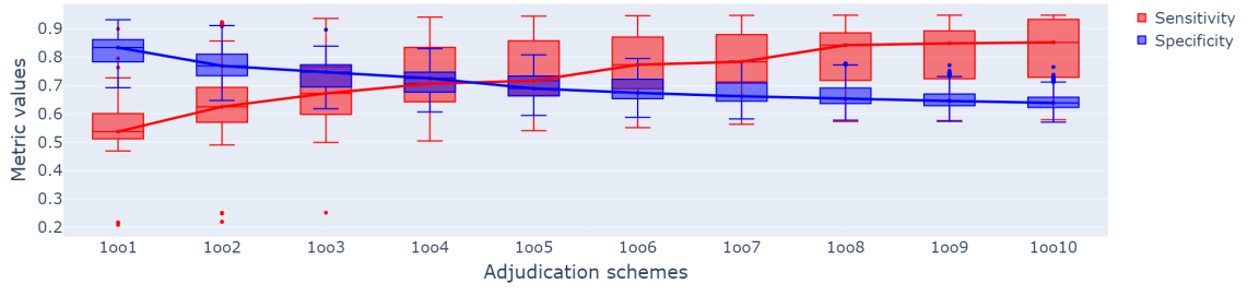
Figure 23: Sensitivity and Specificity for 100N adjudication schemes
