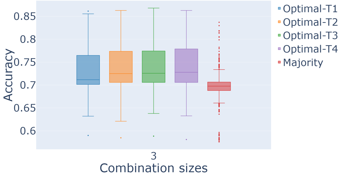
Figure 36: Accuracy for optimal adjudicators T1, T2 and T4
