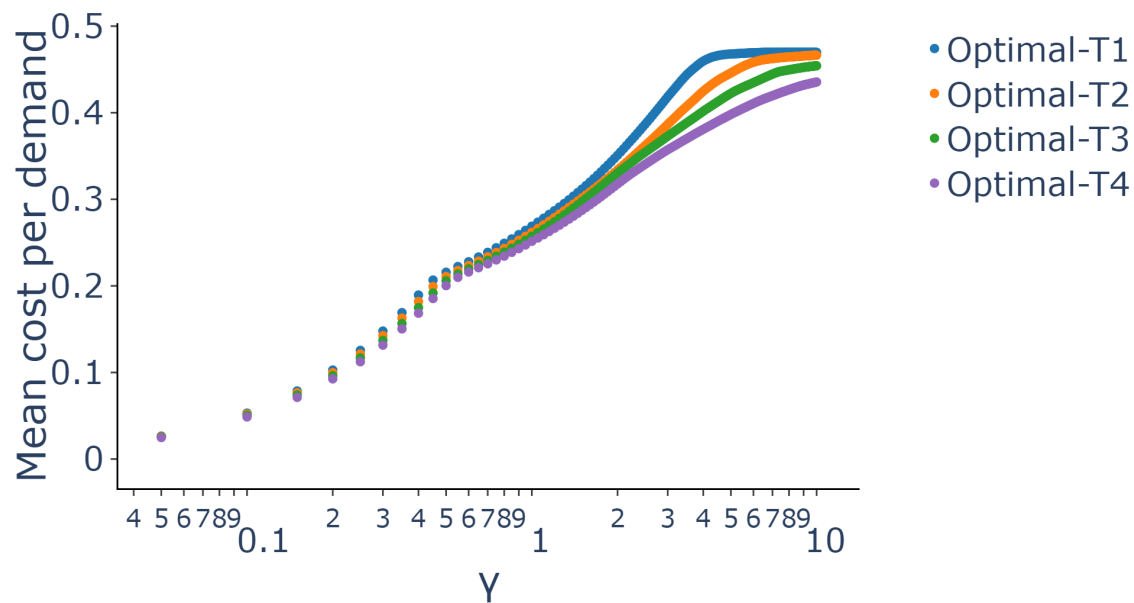
Figure 43: Mean cost per demand profile for optimal adjudicators T1, T2, T3 and T4 using testing data only (log)
