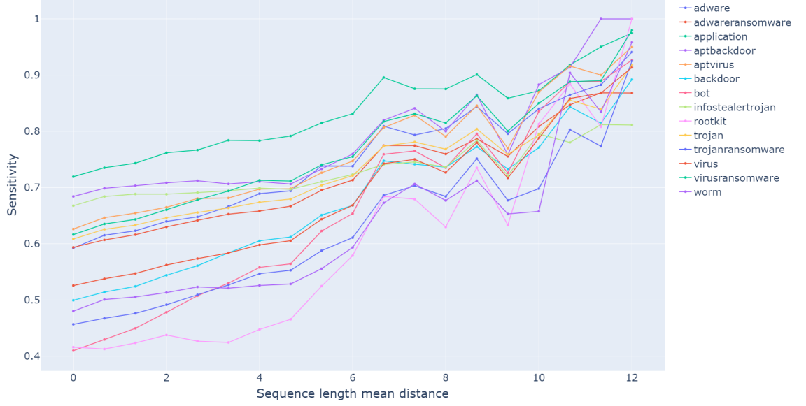
Figure 31: Mean sensitivity by malware type based on sequence length mean distance (1003)
