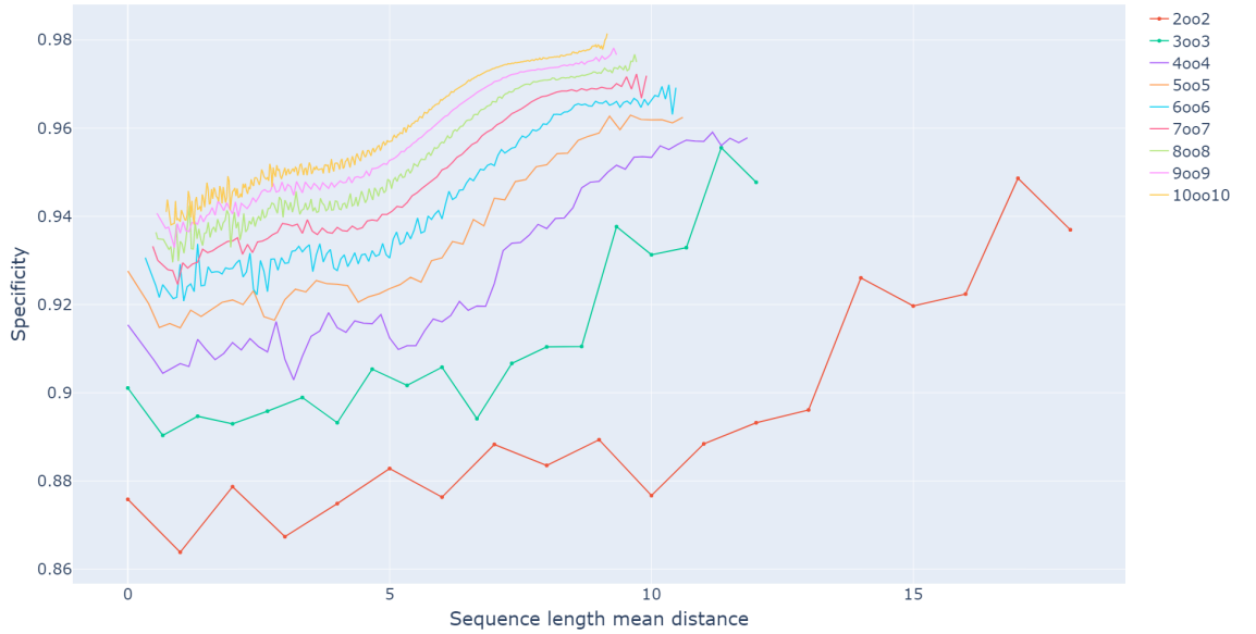
Figure 28: Mean specificity based on the mean distance between sequence length values of models in a particular combination
