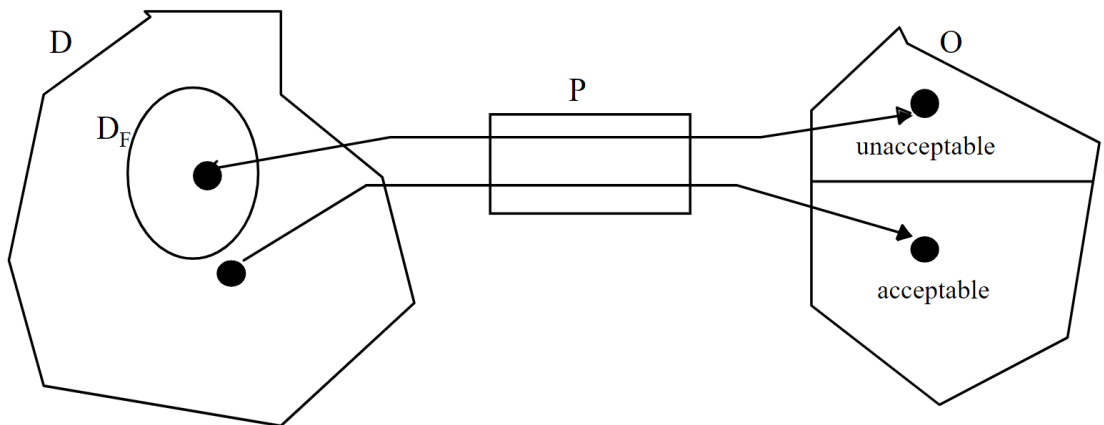
Figure 2: Software failure model [1]
