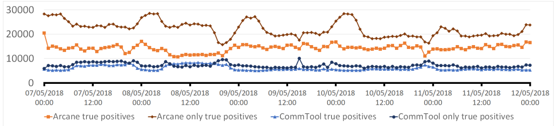
Figure 13: Average bytes sent for true positives for D1.
