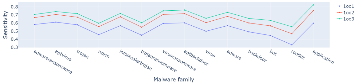
Figure 30: Mean sensitivity by malware type (ordered by largest improvement from 1oo1 to 1oo3)
