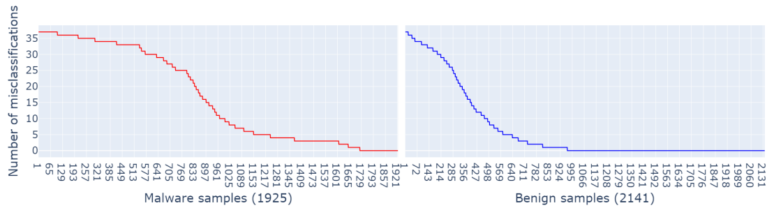
Figure 22: Sample difficulty for malware and benign samples
