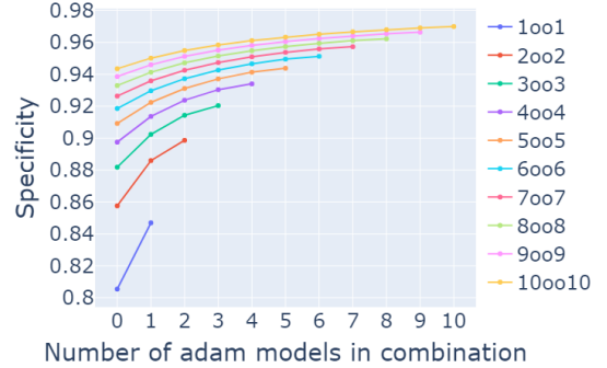
(d) Mean specificity based on optimiser combinations for NooN schemes
