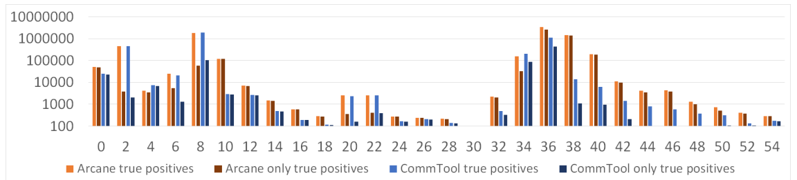
Figure 9: True positives by bytes sent for D3
