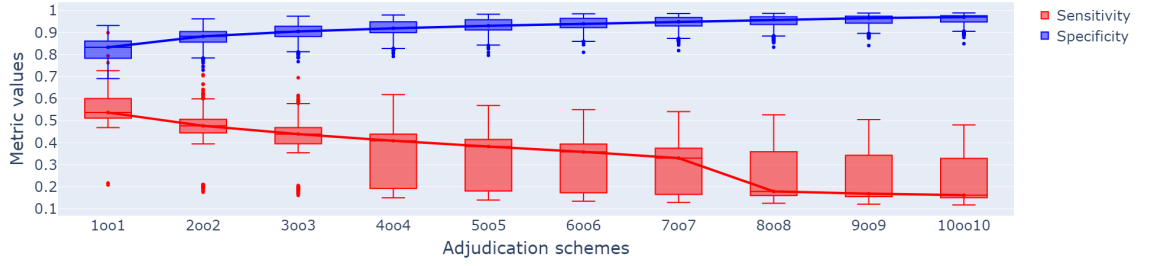
Figure 24: Sensitivity and Specificity for NooN adjudication schemes
