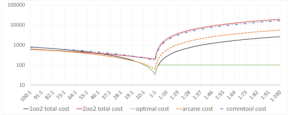
Figure 33: D2 total error costs
