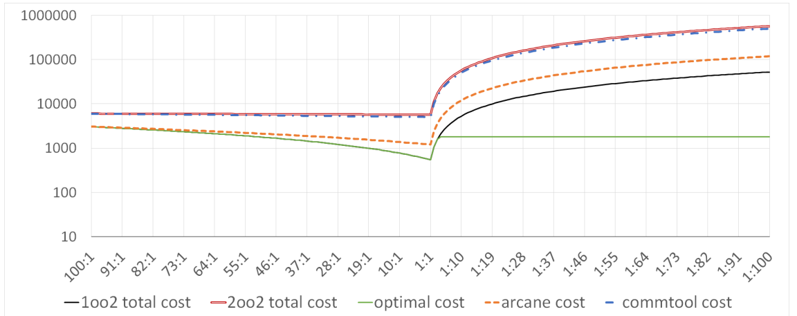
Figure 34: D3 total error costs
