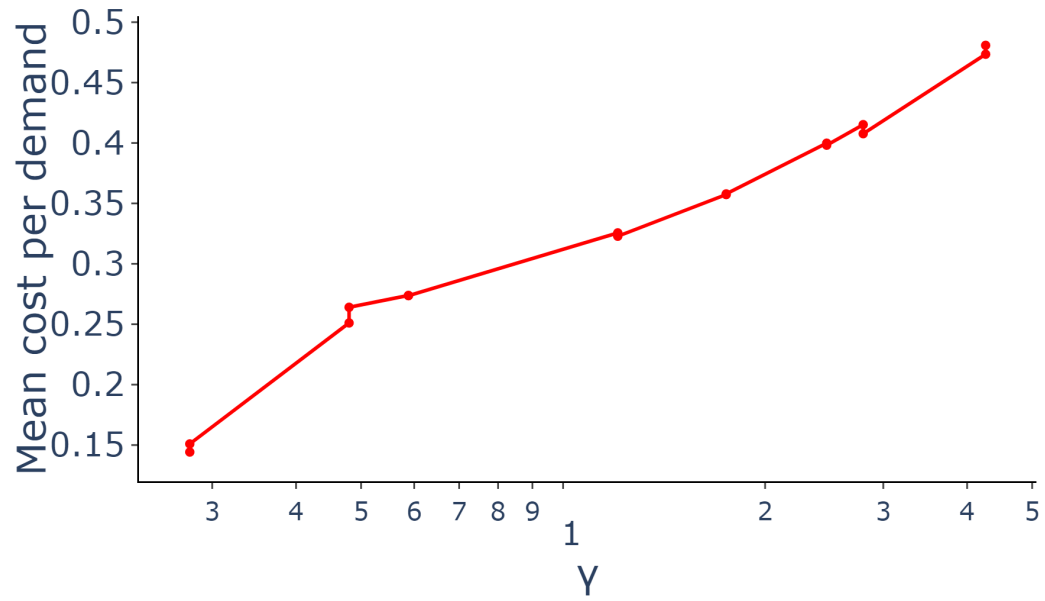
Figure 39: Mean cost per demand profile for a single optimal adjudicator (log)
