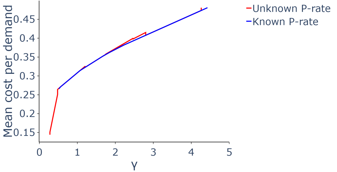
Figure 38: Mean cost per demand profile for a single optimal adjudicator - Known vs Unknown P-rates (RNN models 10, 12 and 23)
