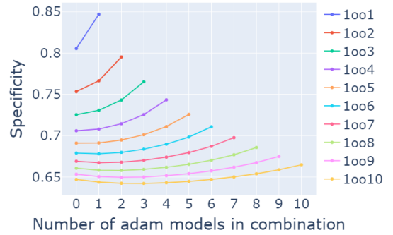
(b) Mean specificity based on optimiser combinations for 1ooN schemes
