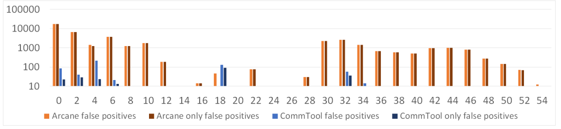
Figure 10: False positives by bytes sent for D1.
