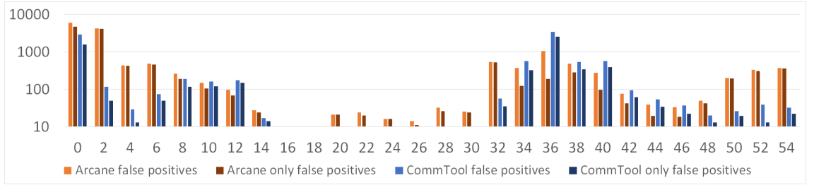
Figure 12: False positives by bytes sent for D3
