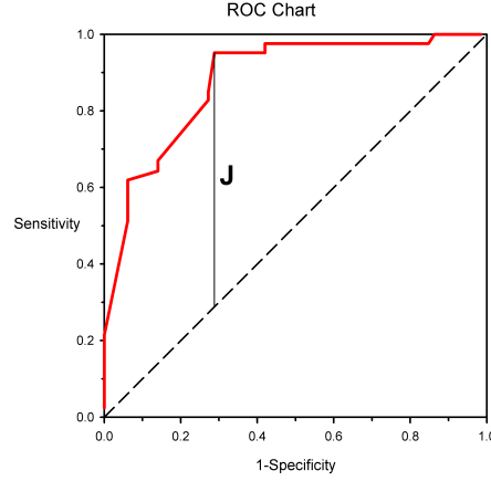
Figure 5: Informedness represented in a ROC curve
