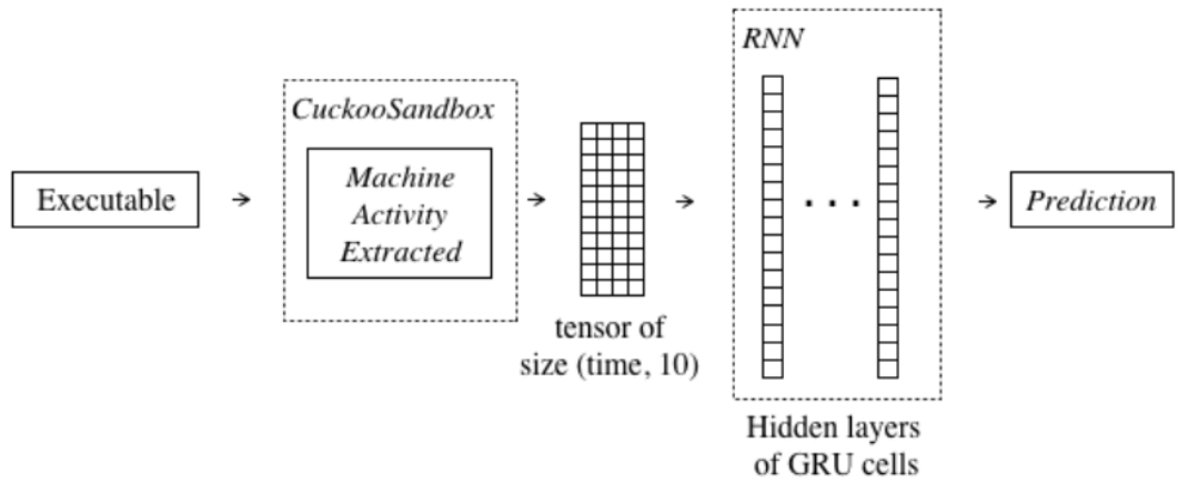
Figure 19: High-level model overview
