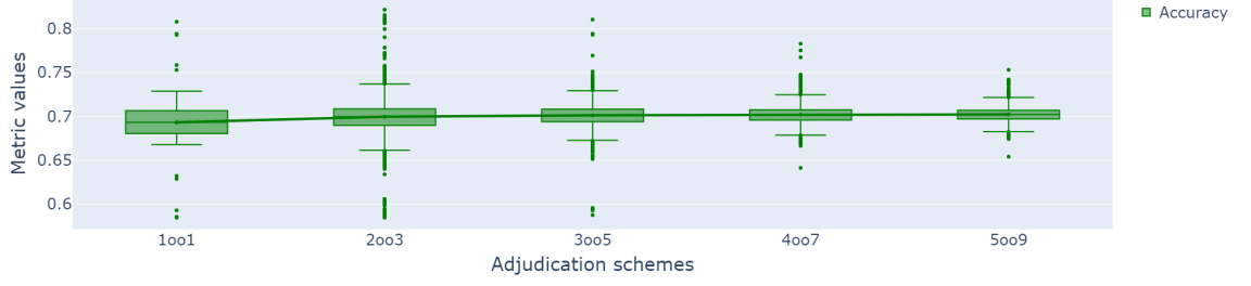
Figure 25: Accuracy for majority voting adjudication schemes
