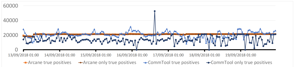
Figure 14: Average bytes sent for true positives for D2.
