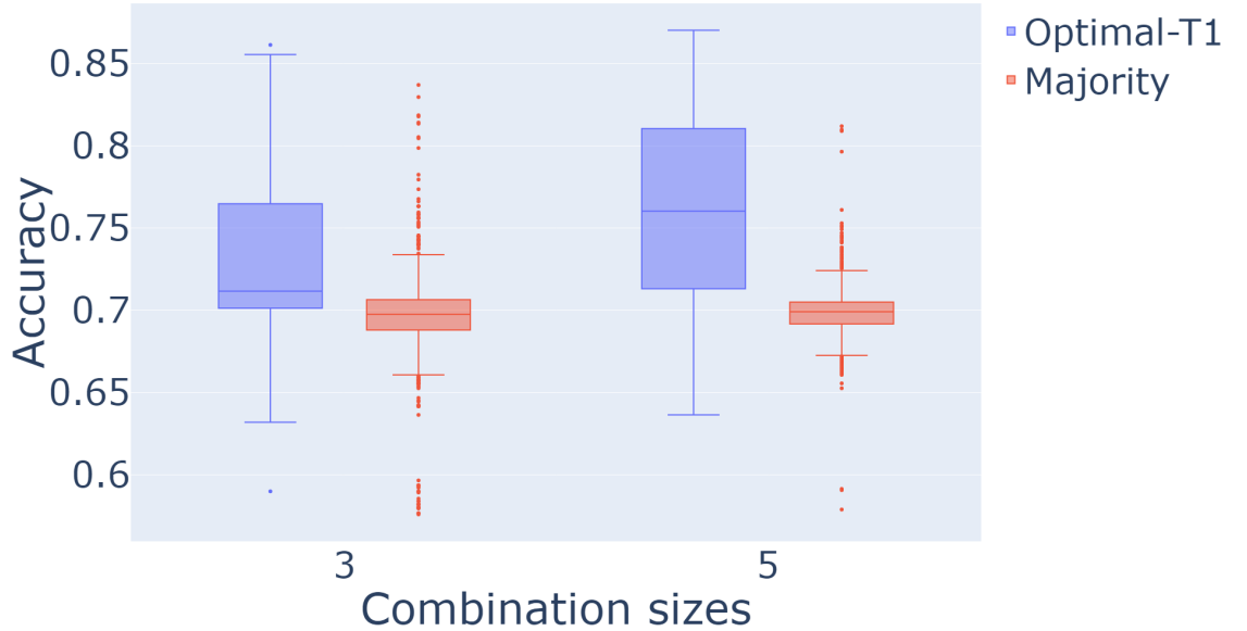
Figure 35: Accuracy for optimal adjudicators T1 and simple majority schemes
