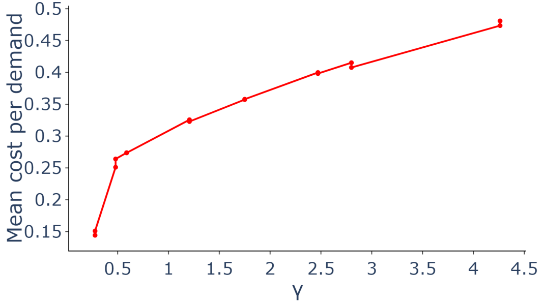
Figure 37: Mean cost per demand profile for a single optimal adjudicator (RNN models 10, 12 and 23)
