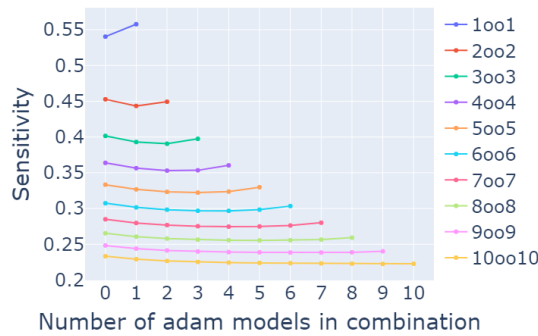
(c) Mean sensitivity based on optimiser combinations for NooN schemes
